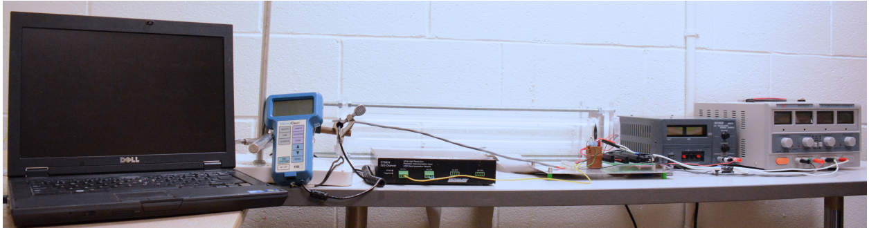
Figure A.2.1 Photo of the complete apparatus used to conduct LCSR tests on thermocouples in cross flow.
