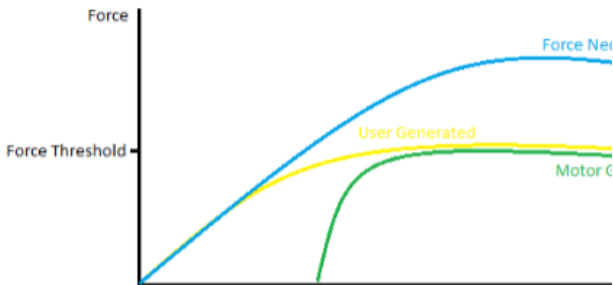
Figure 5: Graph of Expected Force by User Along with Motor
