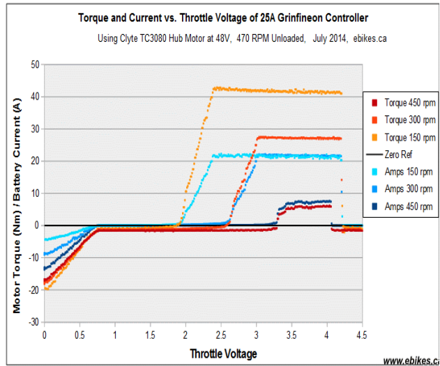
Figure 3: Relationship between driver throttle voltage and motor torque/battery current. [1]
