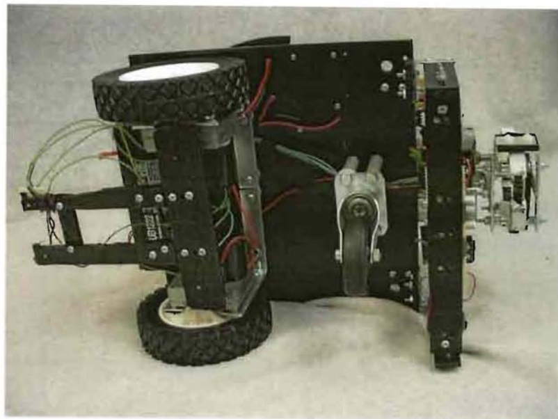
Figure 17: Line tracking platforms mounted beneath the robot
