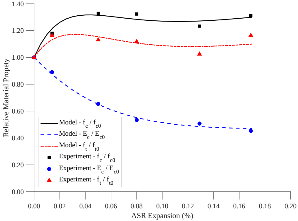
Figure 4.4: Calibrated curves for relative material property evolution
