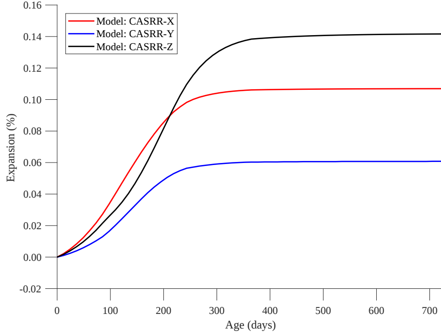
Figure 4.9: Simulated expansions of the rotated CASRR specimen with the casting direction in the X-axis
