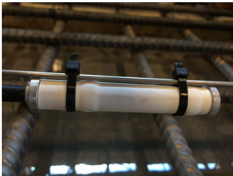
Figure A.9: KM-100B strain transducer attached to positioning bar within rebar cage
