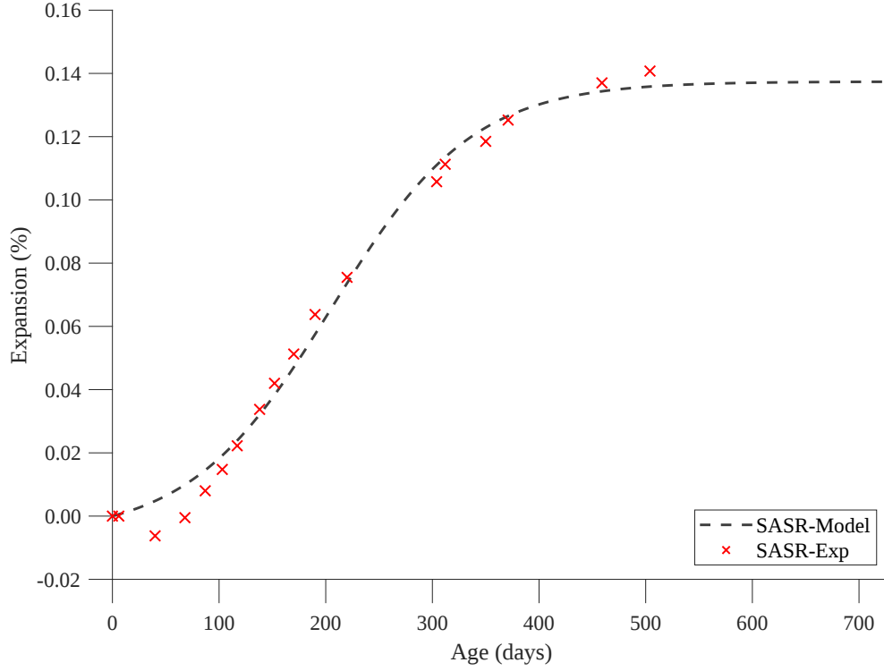
Figure 4.2: Modeled expansion of SASR specimen compared to experimental data
