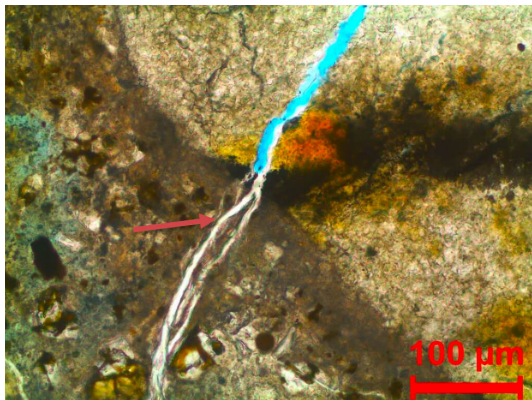
(c) Crack in aggregate and cement
