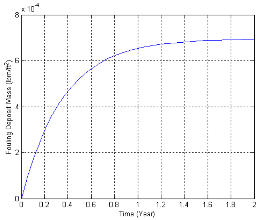
Figure 4.1. Fouling Deposit Mass Variation versus Time
