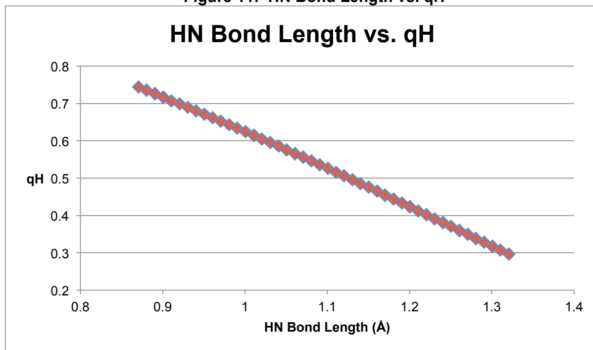
Figure 11: HN Bond Length vs. qH
