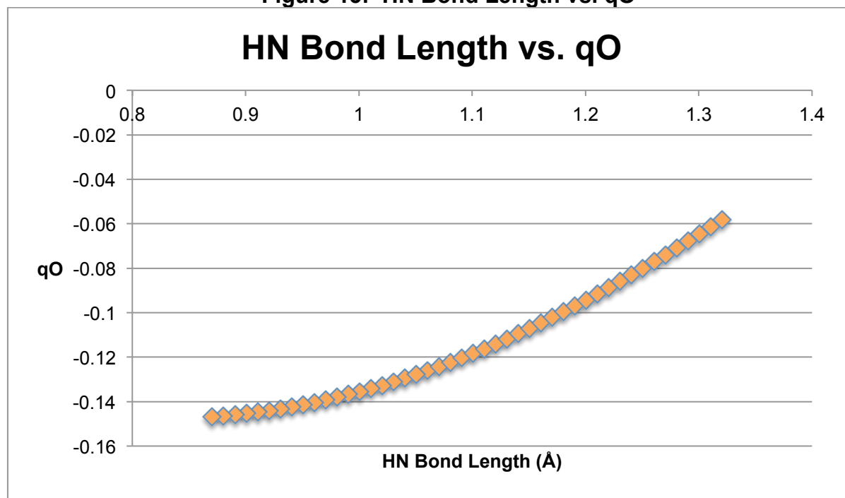
Figure 13: HN Bond Length vs. q_O
