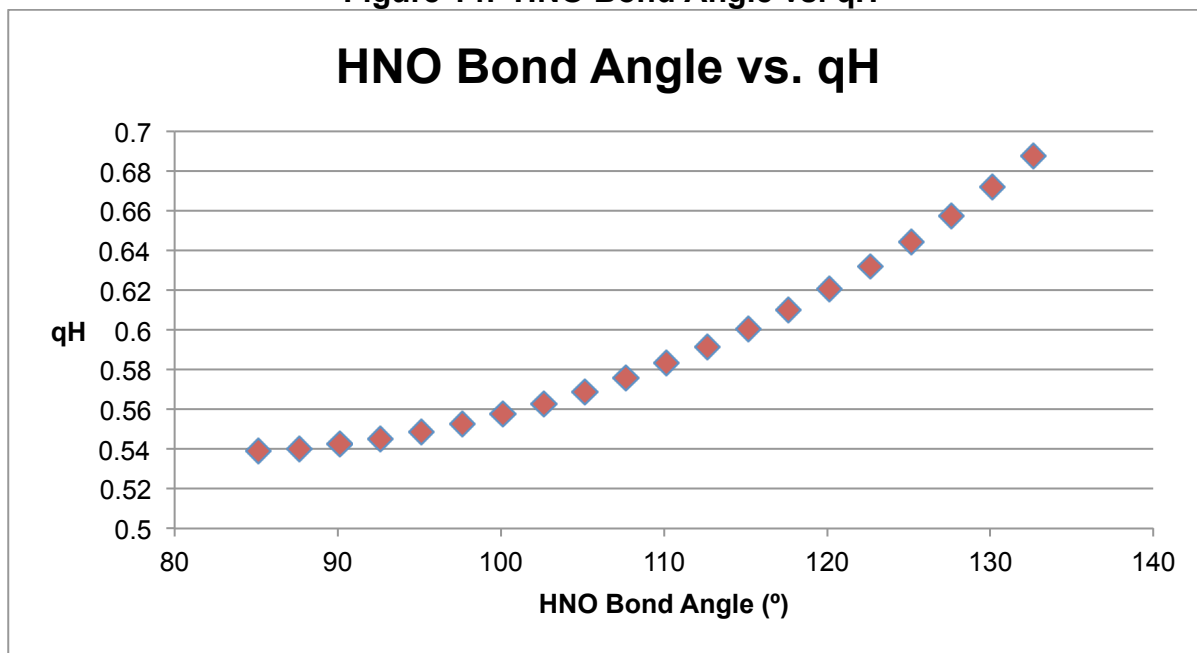
Figure 14: HNO Bond Angle vs. qH
