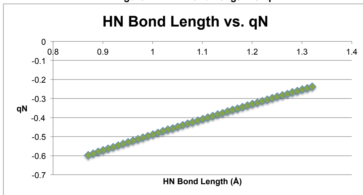
Figure 12: HN Bond Length vs. q_N
