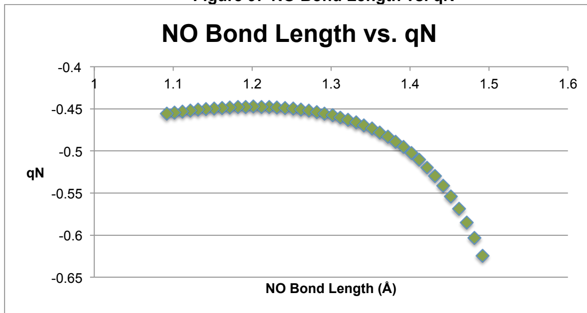
Figure 9: NO Bond Length vs. qN
