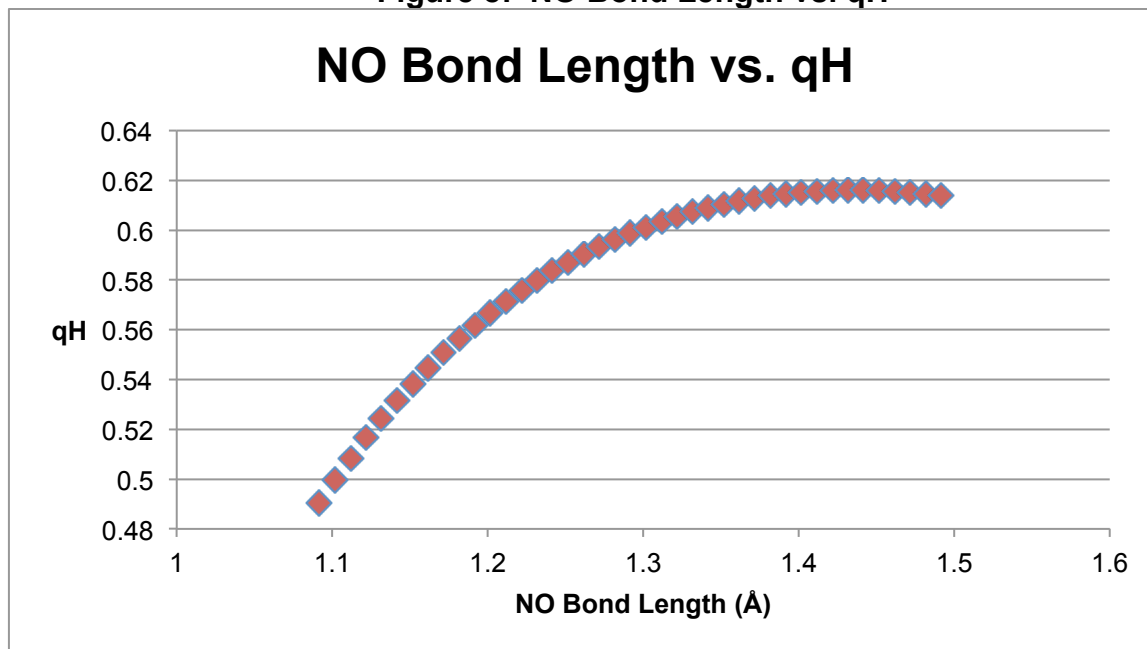
Figure 8: NO Bond Length vs. qH
