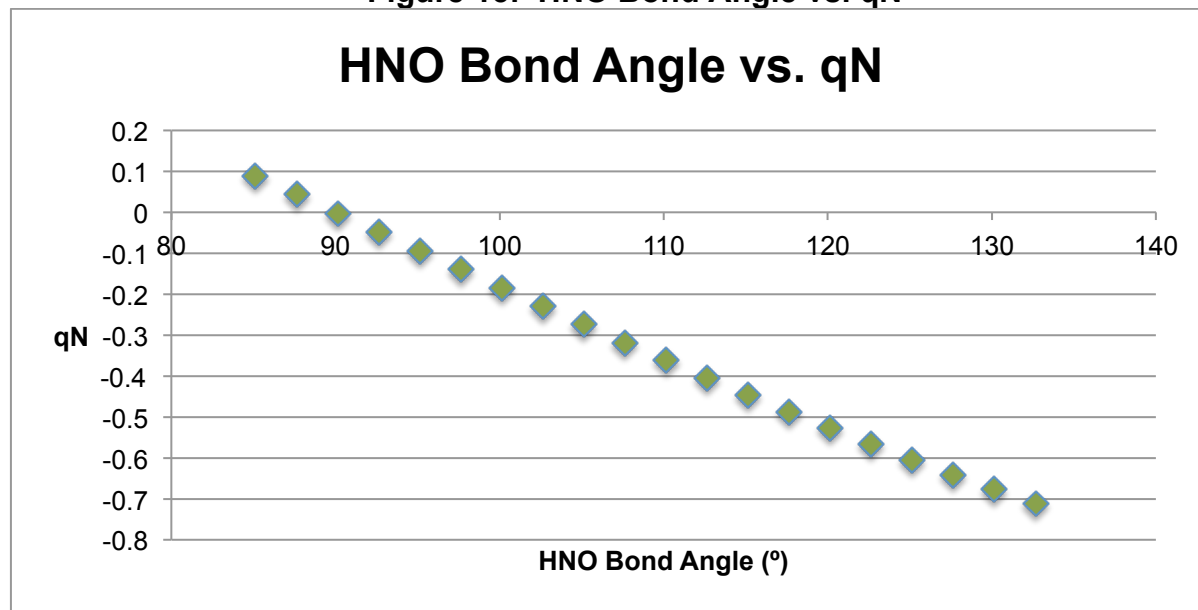
Figure 15: HNO Bond Angle vs. qN
