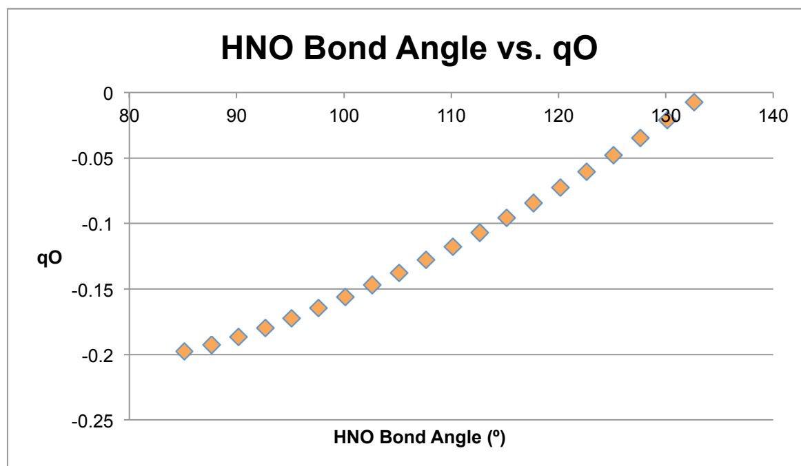
Figure 16: HNO Bond Angle vs. qO
