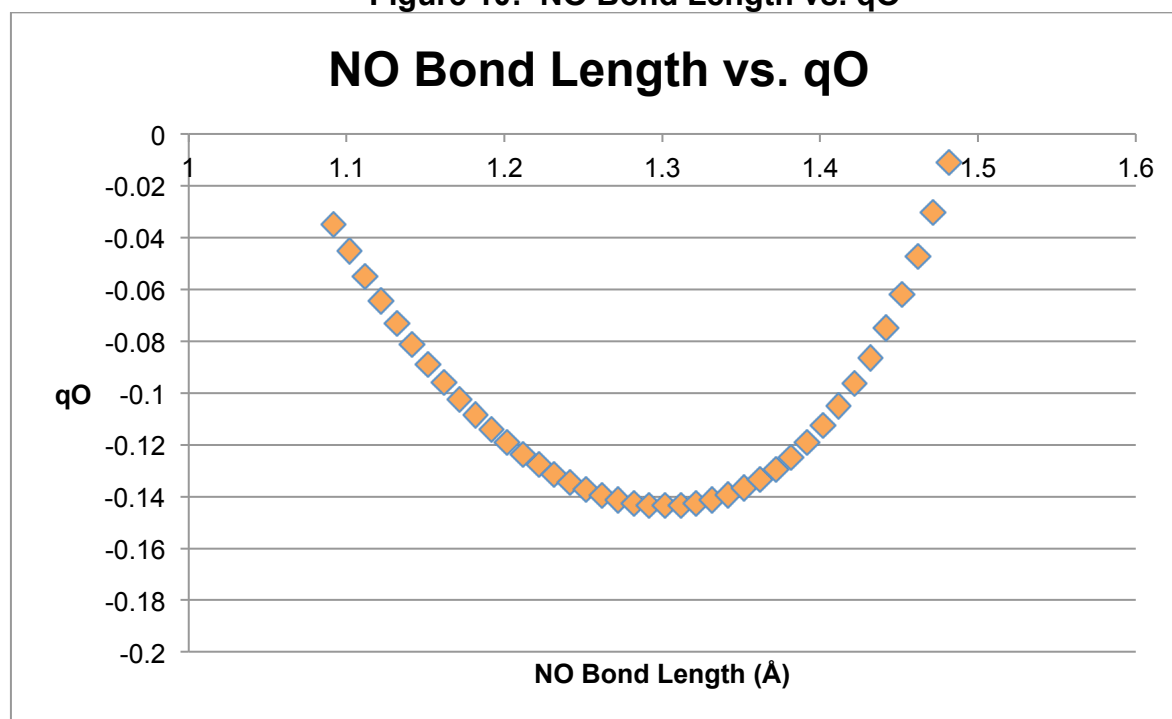
Figure 10: NO Bond Length vs. qO
