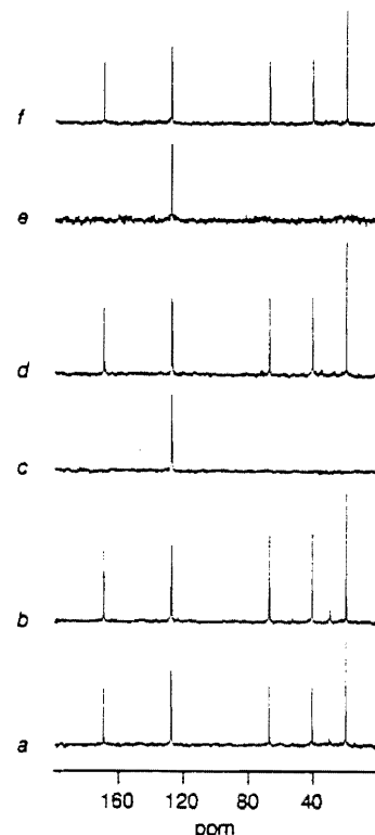
Figure 6. Natural abundance 100-MHz 13 C-NMR spectra, at 70 °C, of aqueous suspensions (D 2 O or H 2 O) of various artificial granule preparations. The peak in each spectrum at \delta 128 ppm is derived from a sealed benzene- d 6 capillary, which served as an internal intensity standard. Spectrum a was obtained from a freshly prepared sample of CTAB-coated, artificial PHB granules; spectrum b was obtained from the identical sample after 11 months' incubation at 30 °C. Spectrum c was obtained from a sample of CTAB-coated, artificial amorphous granules dialyzed exhaustively against distilled water. Spectrum d was collected from a sample of artificial amorphous PHB granules prepared using the detergent sodium cholate. Dialysis of these granules against distilled water causes crystallization and loss of NMR signals (e). Addition of solubilized soy phospholipids prior to dialysis protects the granules from crystallization, leaving the NMR spectrum intact (f).
