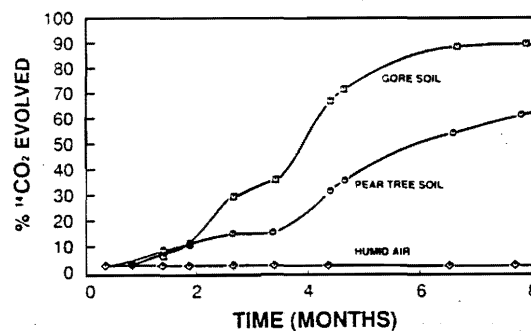
Gas Evolution During Aerobic Degradation of 'BIOPOL' resin in Various Soils
