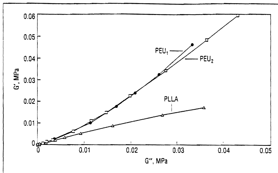
Figure 6. The poly(ester-urethanes) (PEU 1 and PEU 2 ) have greater melt elasticity than the linear polymeric structures (PLLA). The storage modulus ( G' ) versus loss modulus ( G'' ) is shown at 180 °C with rotational rheometry.
