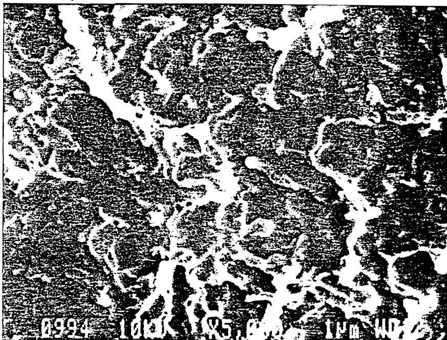
6. SEM of hot-pressed PHB/HV latex film with 21% HV after 12 days immersion in simulated activated sludge
