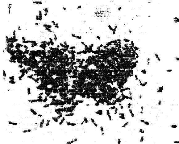
Figure 3: PHB stained granules in activated sludge bacteria ( Manual on the Causes and Control of Activated Sludge. David Jenkins )
