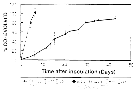
Figure 7(a) Gas Evolution During Aerobic Degradation in Activated Sewage Sludge
