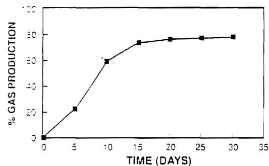
Gas Evolution During Anaerobic Degradation in Activated Sewage Sludge
