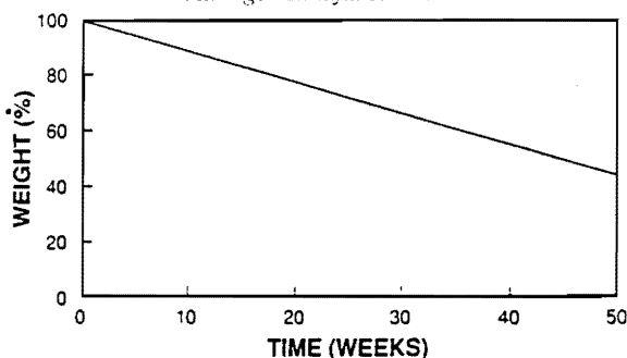
Degradation of BIOPOL Bottles in Managed Landfill Simulation
