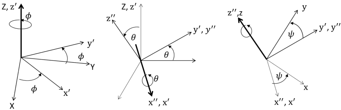
Figure 3.1: Example of rotation using Euler angles. The first rotation is \phi around the z axis transforming from the initial X, Y, Z system to the x', y', z' system, followed by a rotation of \theta around the new x' axis into the x'', y'', z'' system, and finally a rotation of \psi around the z'' into the x, y, z system.
