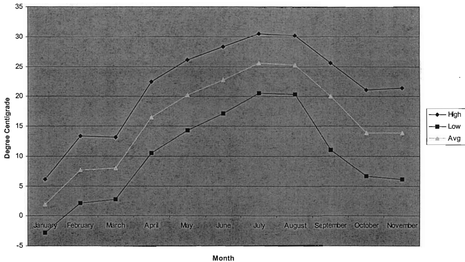
Figure 38: Weather data in the form of monthly high, low, and average temperatures.
