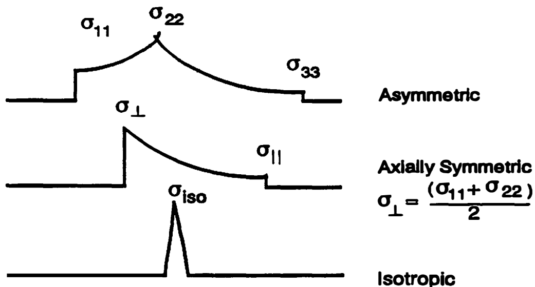
Figure 8 Schematic representation of ^{13}\text{C} chemical-shift-anisotropy powder patterns
