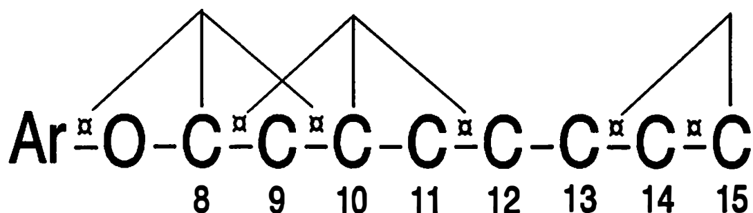
Figure 50 Bond conformations of the octyloxy chain below the K transitions. The bonds marked with the sign \propto are of the gauche character.
