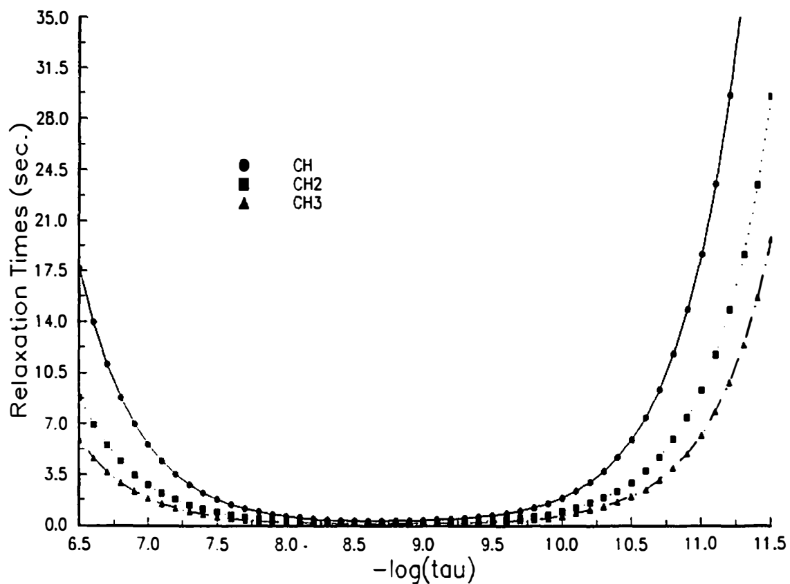
Figure 4 Spin-lattice relaxation times of a ^{13}\text{C} nucleus undergoing a random motion. The horizontal axis is the correlation time.
