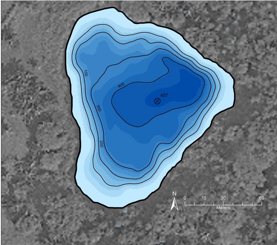
Figure 4.3. Bathymetry of Laguna Carse with coring location indicated. Lake depths (shown in cm) surveyed in July 2014 with bathymetry calculated using a spline function. Aerial Imagery modified from ESRI, DigitalGlobe.
