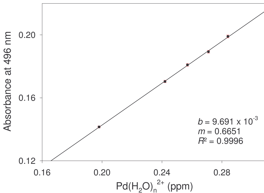
Figure C.1. Calibration plot from the analysis of \text{Pd}(\text{H}_2\text{O})_n^{2+} standard solutions.
