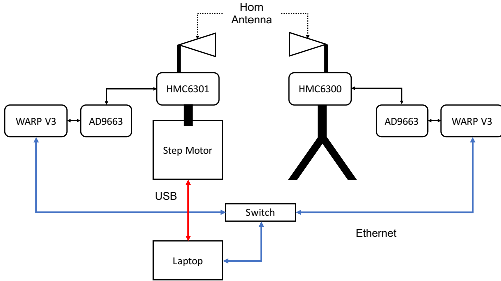
Figure 6.4: Scheme of Motorized mmWave Communication Testbed
