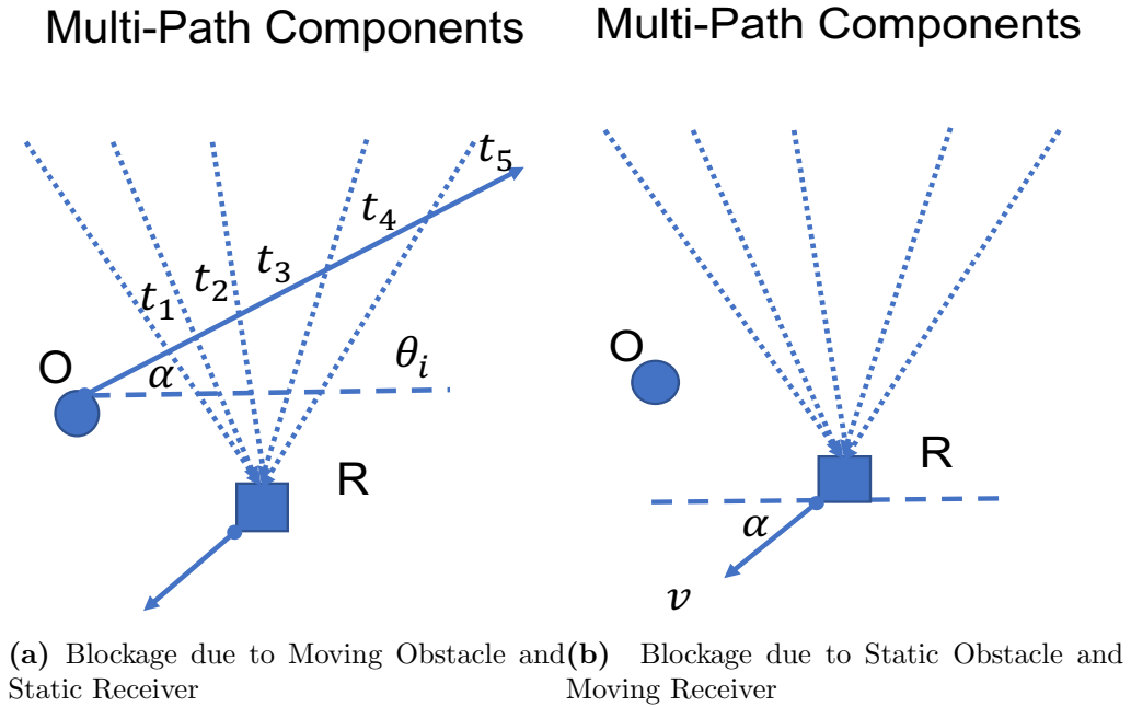
Figure 6.2: Two Approximately Equivalent Blockage Models
