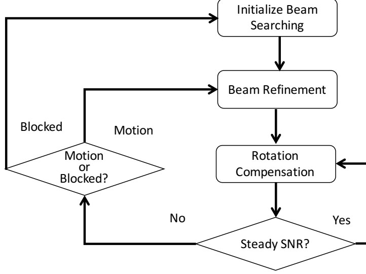
Figure 3.6: Proposed scheme of beam tracking
