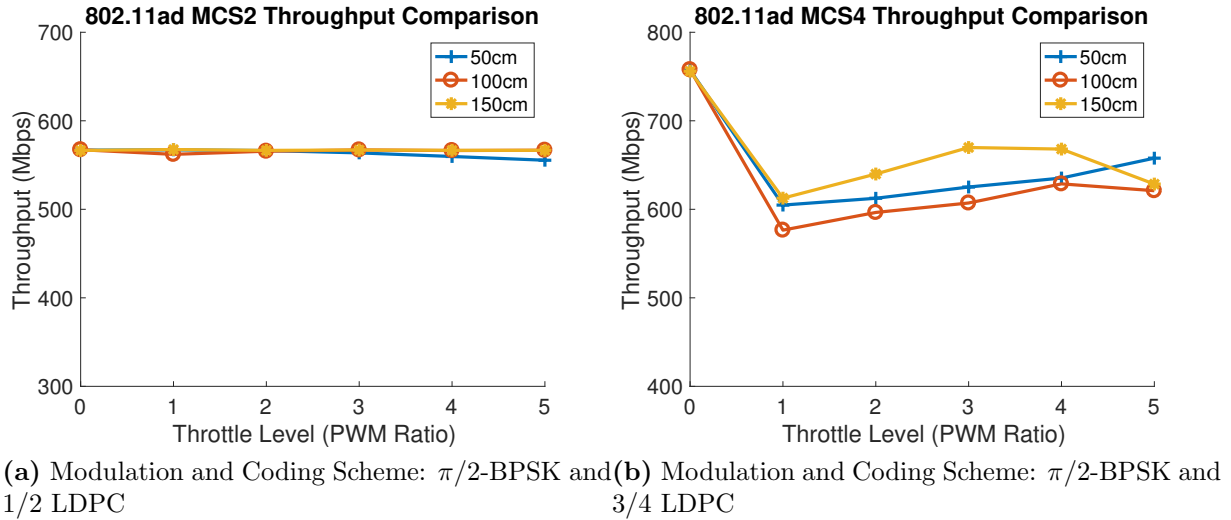
Figure 5.9: IEEE 802.11ad throughput test
