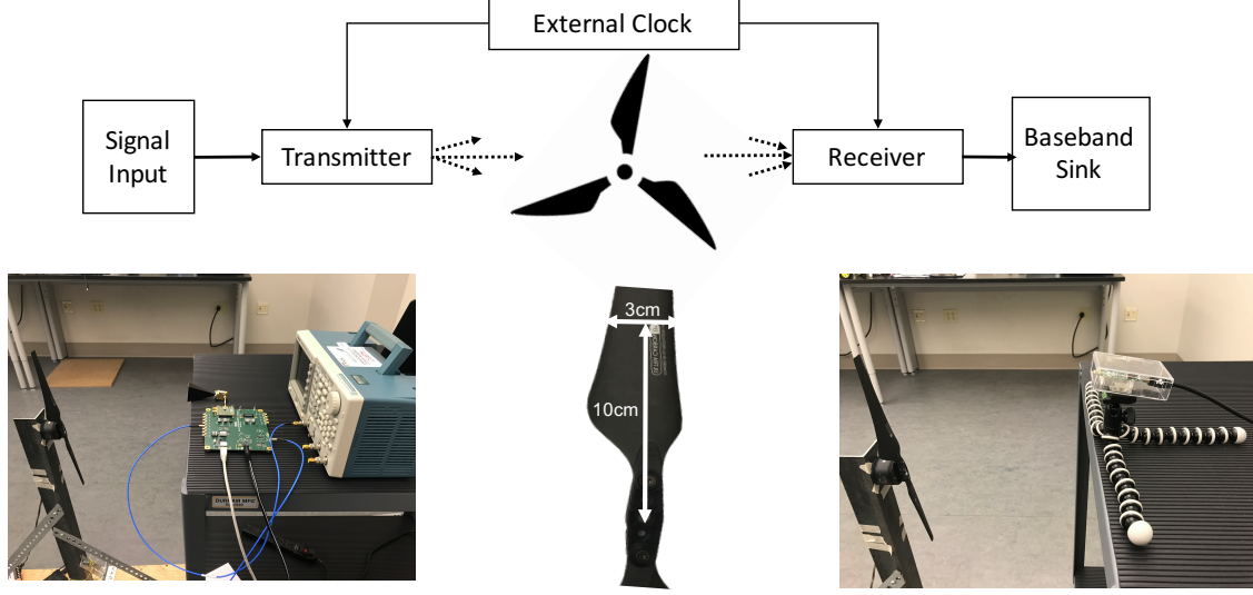
Figure 5.2: Experiment setup: the lower left figure shows the AD HMC 6300 transmitter and the UAV propeller. The lower right figure shows the Tensorcom Platform Test. In the middle is the dimension of the propeller.
