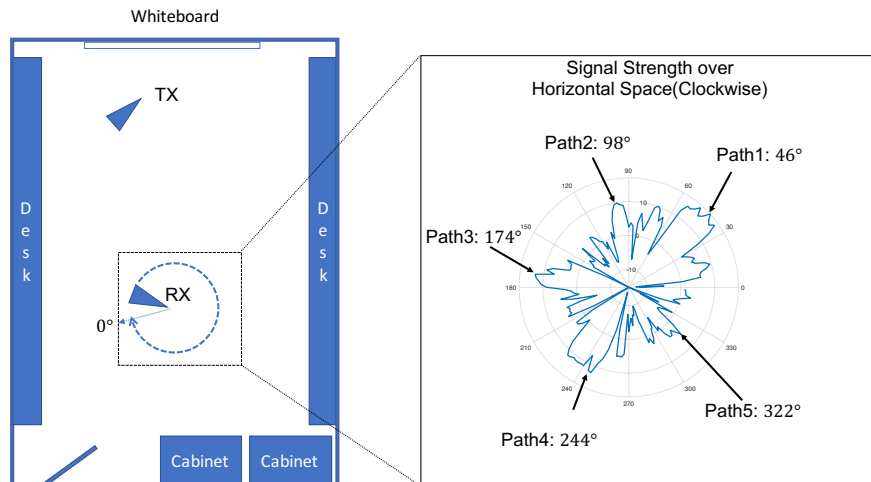
Figure 6.6: Floor Plan of the Lab and the Polar Plot of Multi-paths Signal Strength
