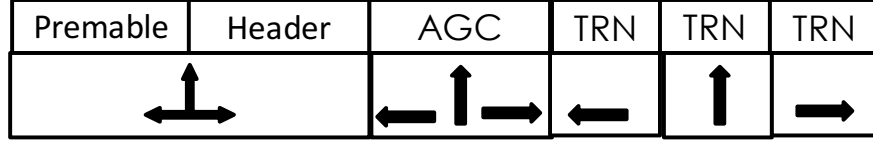
Figure 3.5: In-packet Training in the Beam Refinement of IEEE 802.11ad. (The arrows means the directions.)
