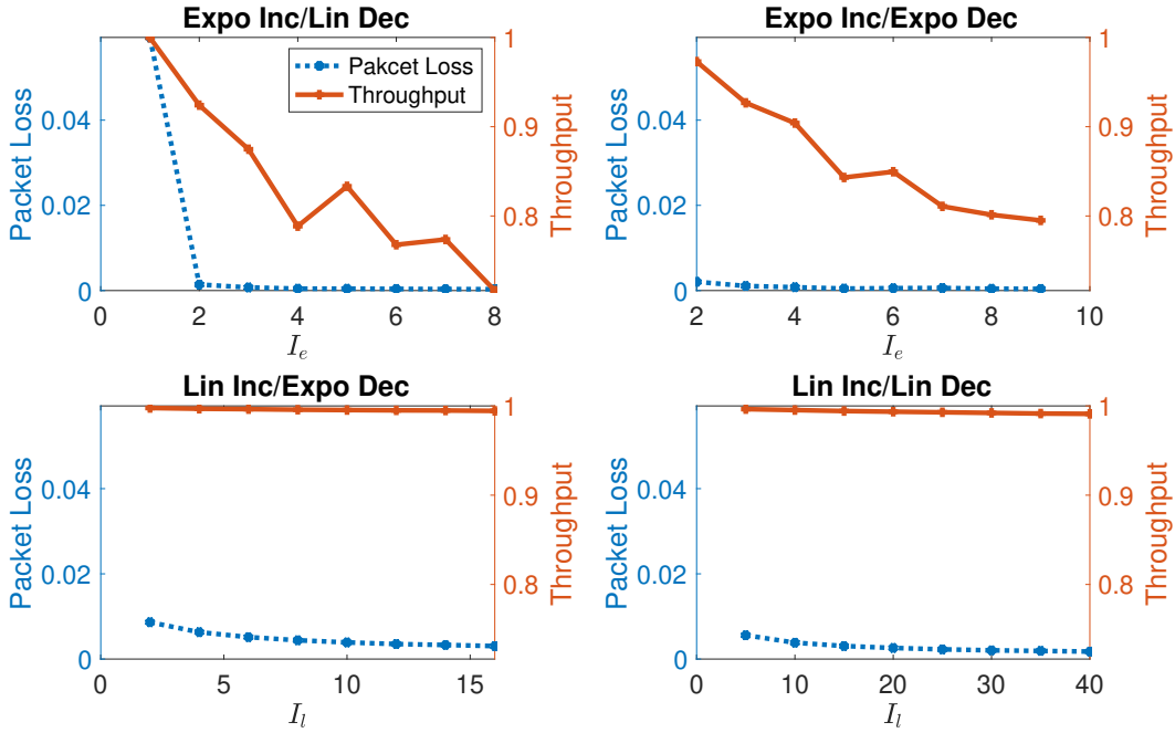
Figure 4.12: Performance comparison of four backoff schemes over different increasing functions f_{inc} . The f_{dec} is fixed in each figure.
