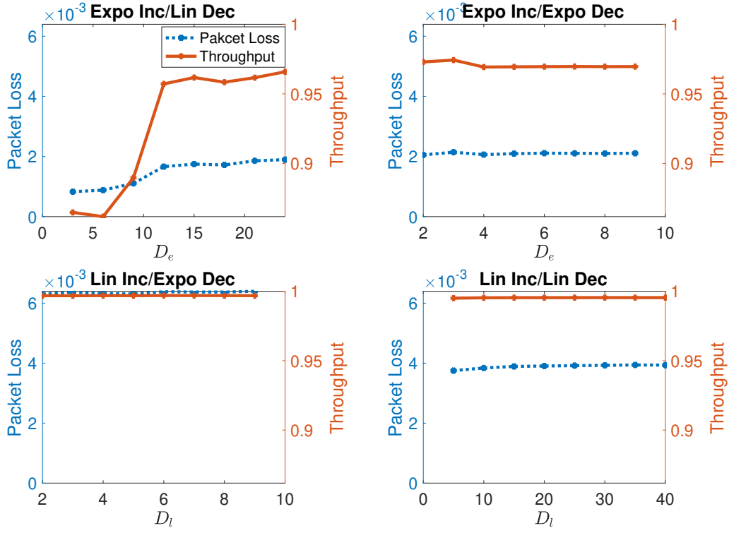
Figure 4.13: Performance comparison of four backoff schemes over different decreasing functions f_{dec} . The f_{inc} is fixed in each figure.
