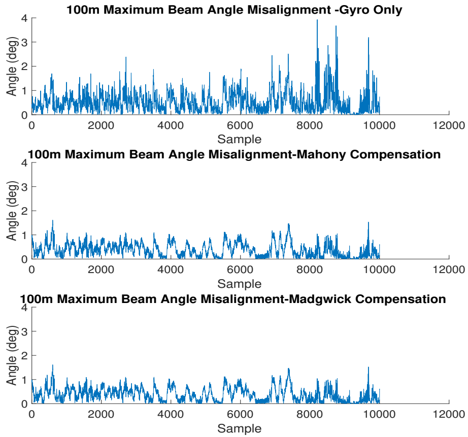
Figure 3.12: Comparison of Compensation using Different Filters
