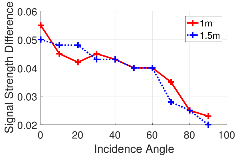
Figure 5.7: Signal Strength Difference between Blockage and LOS. (The legend shows the distance between propeller and transmitter. )
