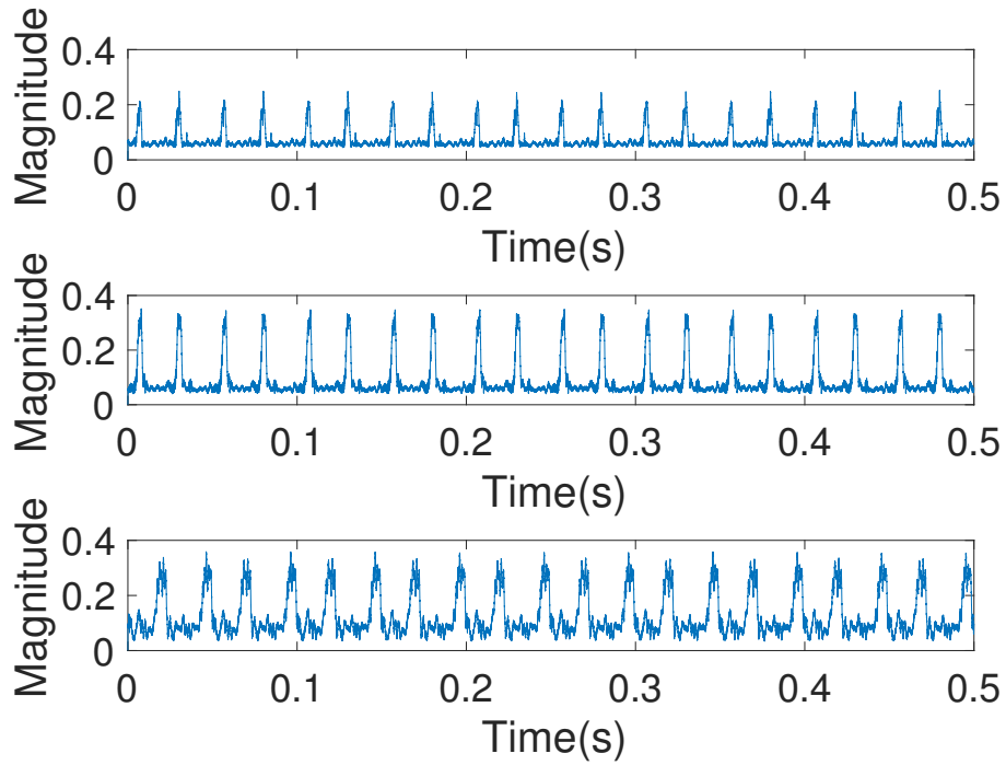
Figure 5.8: Reflected Signal Strength with Different Angles 60°, 45° and 30°.
