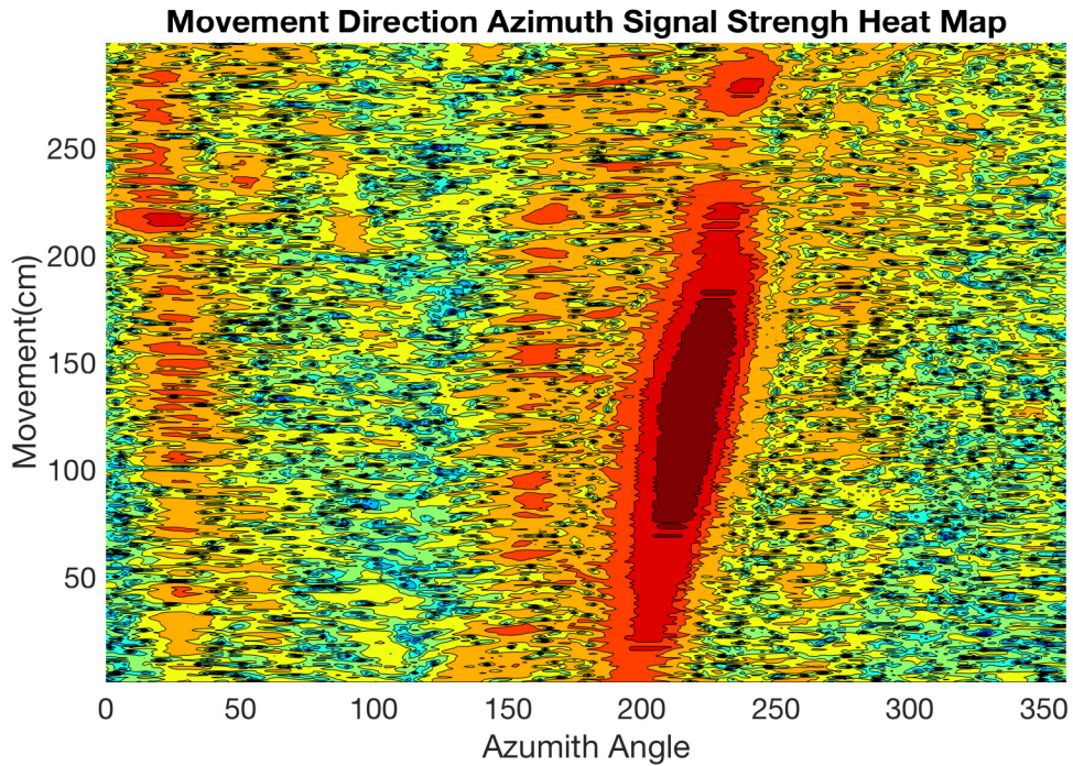
Figure 6.5: Signal Strength over Azimuth Angle and Movement
