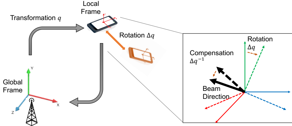
Figure 3.3: Beamforming Misalignment Compensation
