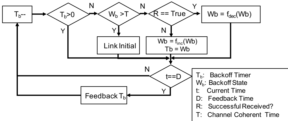
Figure 4.4: Dynamic data offloading: distributed encoding
