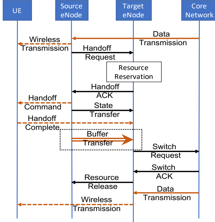
Figure 4.3: The time scheme of handoff procedure. The dotted block is optional.
