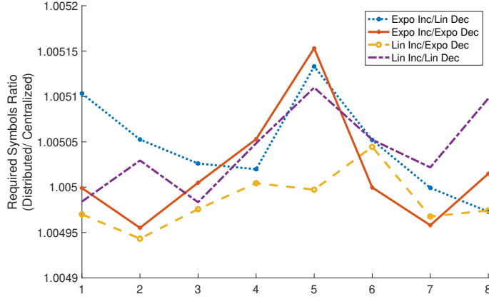
Figure 4.16: The ratio of averaged symbol numbers for successful decoding between distributed and centralized off-loading mechanisms.
