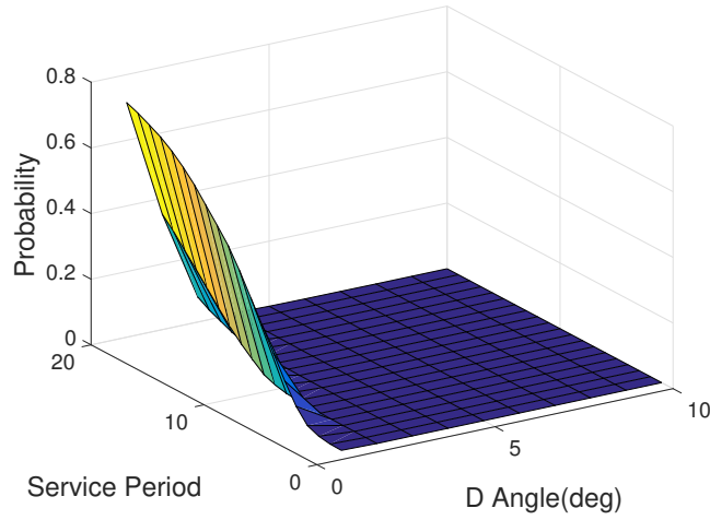
Figure 3.11: The probability of different hitting time of the angle deviation threshold (the loss of tracking) at different service periods in the outdoor walking condition.
