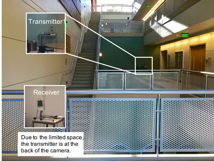
Figure 4.6: The Experiment in the Hall Way of Min Kao Building, University of Tennessee.
