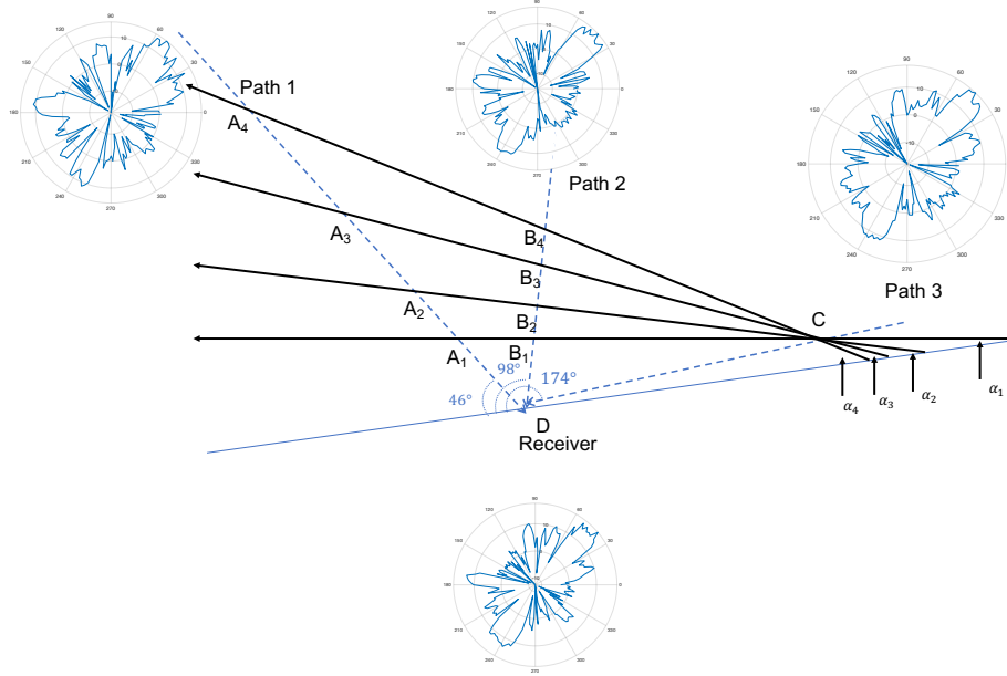
Figure 6.9: Blockage Prediction Scheme with Experiment Records
