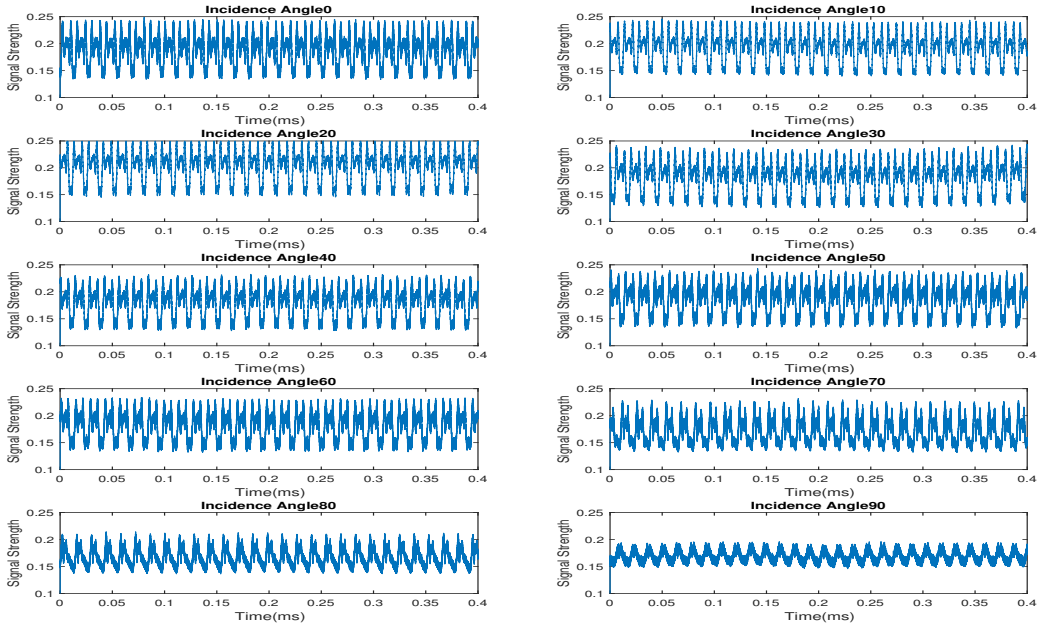
Figure 5.6: Blockage Pattern vs Incidence Angle. The Distance between Propeller and Transmitter is 1.5m.
