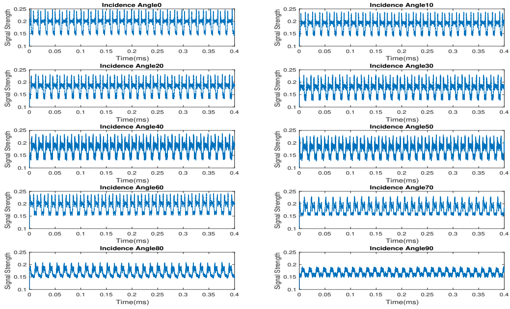
Figure 5.5: Blockage Pattern vs Incidence Angle. The Distance between Propeller and Transmitter is 1.0m.
