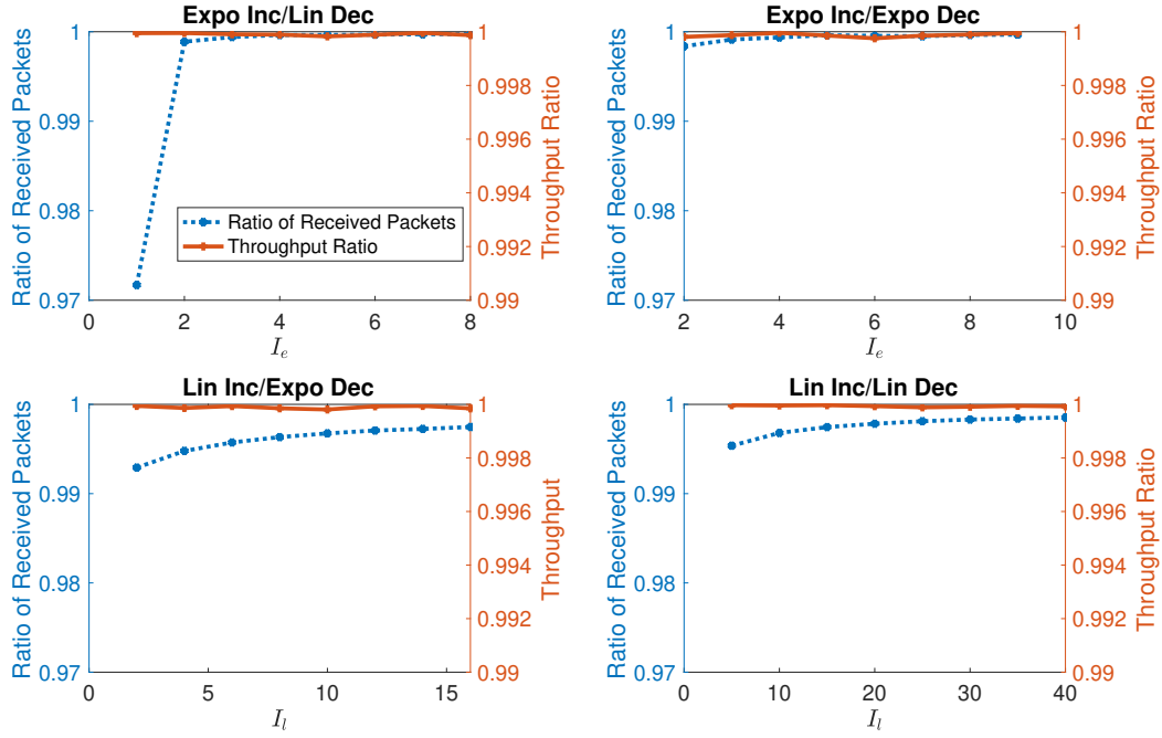
Figure 4.14: System performance comparison between instant feedback and feedback with 5ms latency with same parameters as Fig.4.12. All the ratios in figures are defined as 5ms Latency feedback over instant feedback.
