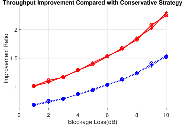
Figure 5.16: Throughput improvement
