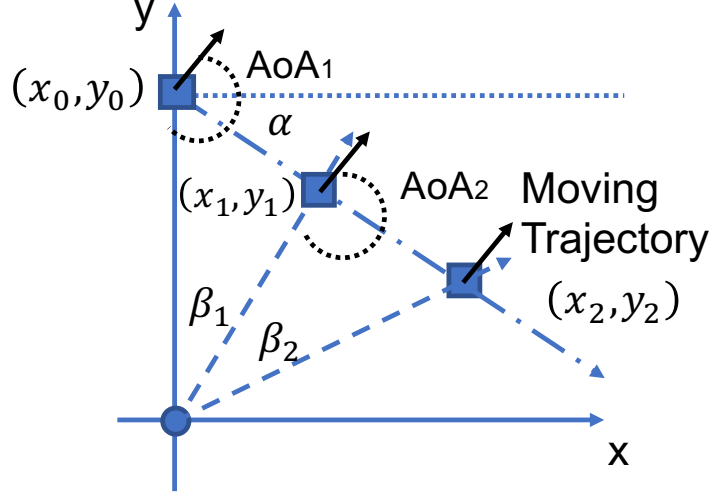
Figure 6.3: Estimation of Moving Direction \alpha Based on AoA \beta_i
