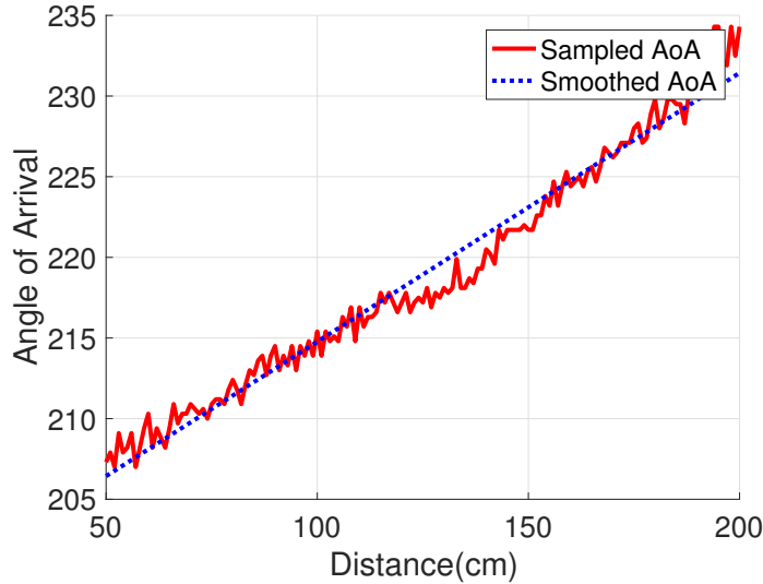
Figure 6.8: Comparison of Sampled AoA and Smoothed AoA with Linear Regression
