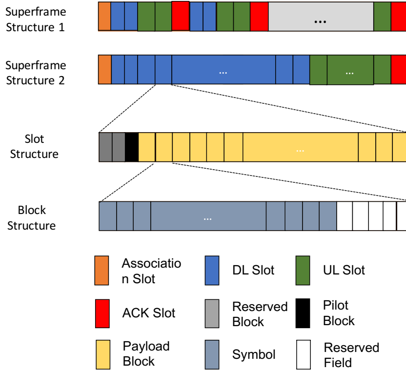
Figure 5.11: Illustration of superframe scheme
