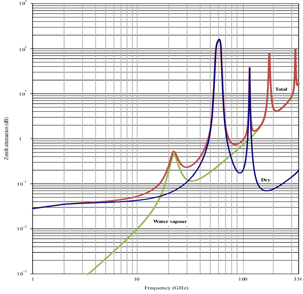
Figure 1.1: Total, dry air and water-vapour zenith attenuation from sea level from [86] (Pressure = 1 013.25 hPa ; Temperature = 15^{\circ}C ; Water Vapour Density = 7.5 g/m^3 )
