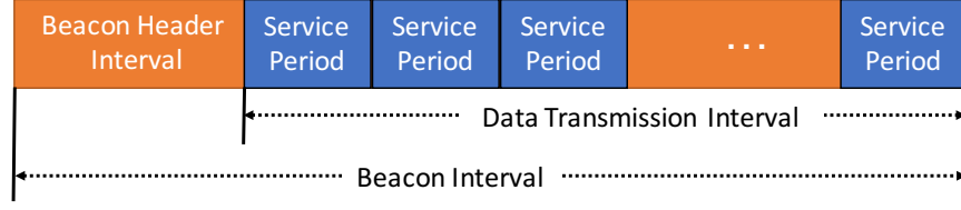
Figure 3.4: A Simplified Beacon Interval Frame of IEEE 802.11ad.
