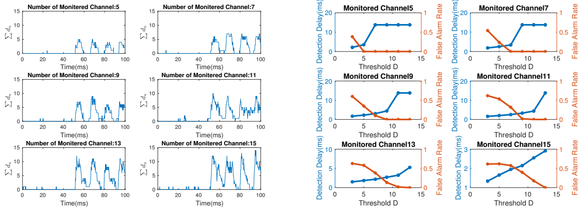
(a) Different Numbers of Subcarriers under 5dB Loss (b) Detection Delay and False Alarm Rate under with Noise of \mathcal{CN}(0, 5) and Rejection Level \alpha = 0.1 . Different Channel Numbers and Thresholds D .
