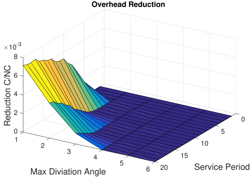
Figure 3.13: Overhead reduction for different thresholds
