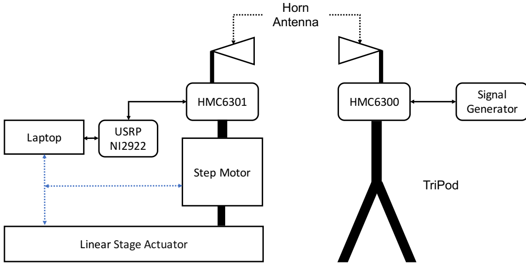
Figure 2.1: The Scheme of Two Degree of Freedom Motorized mmWave Communication Testbed.
