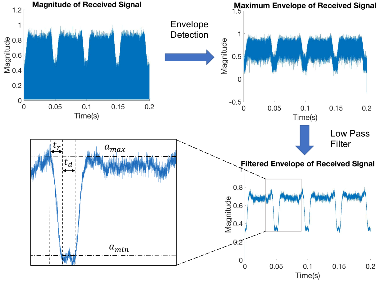
Figure 5.4: The Illustration of Blockage Pattern.
