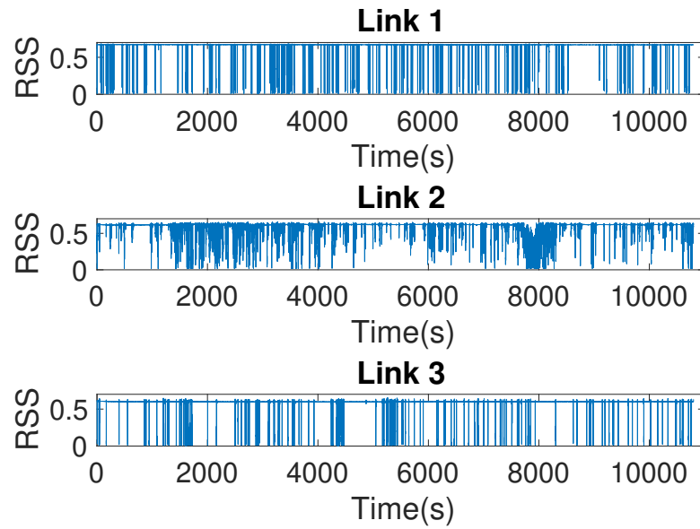
Figure 4.8: Received signal strength over 3 hours over three links.
