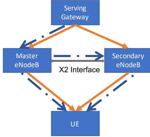
Figure 4.2: Two DC architectures, where the orange solid and blue dotted arrows correspond to architecture types 1 and 2, respectively.
