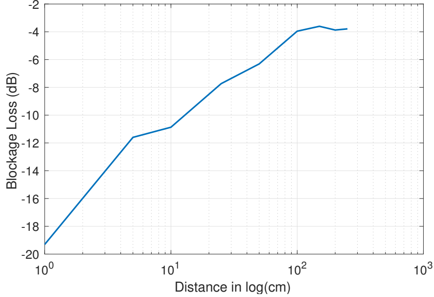
Figure 5.3: Blockage Loss due to the Rotating Propeller given Different Distances, where the x -axis is in the Logarithm Scale.
