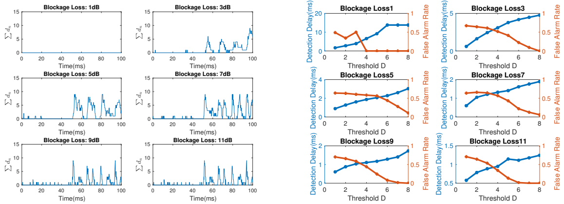
(a) 10 Subcarriers under Different Levels of Blockage (b) Detection Delay and False Alarm Rate under Loss with Noise of \mathcal{CN}(0, 5) and Rejection Level \alpha = 0.1 . Different Levels of Blockage Loss and Thresholds D .
