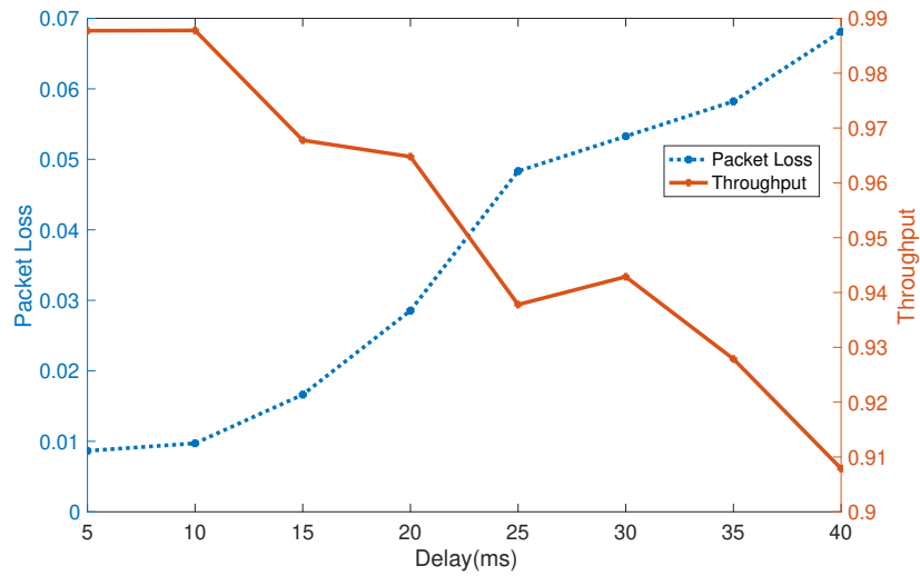
Figure 4.15: System performance comparison over different latencies.
