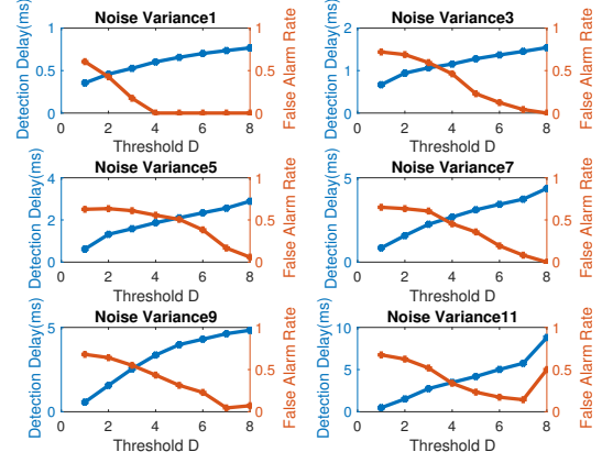
(a) 10 Subcarriers under 5dB Loss with Different Noise of \mathcal{CN}(0, \sigma^2) and Rejection Levels \alpha . (b) Detection Delay and False Alarm Rate under Different Noise Variance and Thresholds D .
