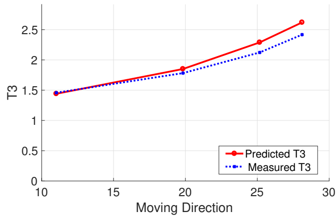
Figure 6.10: Predicted and Measured Lead Time of LOS Blockage T_3 as a Function of Moving Direction \alpha
