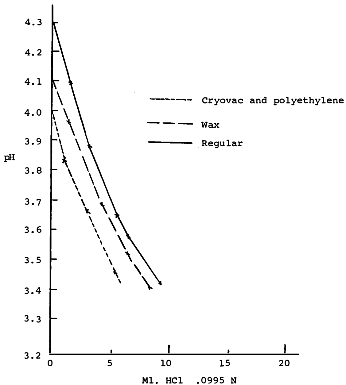
Figure 9. Neutralizing \text{NH}_3 absorbed by strawberries.
