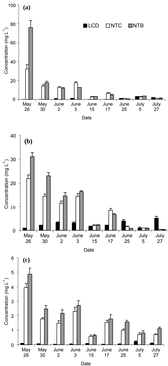
Figure 2.3. Concentrations of (a) Br, (b) NO 3 -N, and (c) PO 4 -P in runoff in 2004. Error bars indicate standard error.
