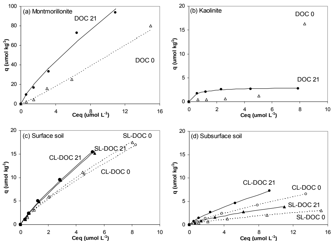
Figure 3.15. Dissolved organic carbon (DOC) effect on sulfamethazine (SMT) sorption. DOC= 21 mg L -1 . SL= sandy loam, CL= clay loam. Symbols represent experimental data and lines represent isotherm models for which parameters are listed in Table 3.9 and Table 3.10. The sorption data were obtained by equilibrating 6.5 g L -1 of Ca 2+ -saturated montmorillonite or 500 g L -1 of soils in 0.01 M Ca(NO 3 ) 2 containing 0.0006-0.016 mM SMT. Solution pH values were 4.2 (montmorillonite), 5.2 (kaolinite), 5.2 (CL-S), 5.3 (CL-SS), 5.4 (SL-S), and 5.5 (SL-SS) for both in the absence and in the presence of dairy manure DOC. The suspensions were equilibrated for 24 h at 20 to 22°C.
