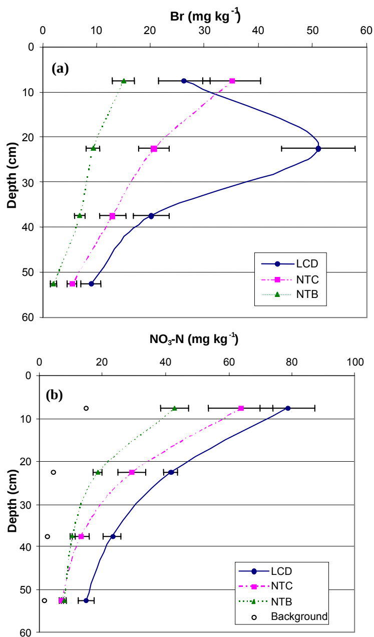
Figure 2.4. Residual concentration profiles for (a) Br and (b) NO 3 -N in LCD, NTC, and NTB, 30 days after fertilizers were applied. Error bars indicate \pm 1 standard error. Background nitrate concentration before fertilization is shown by an open circle.
