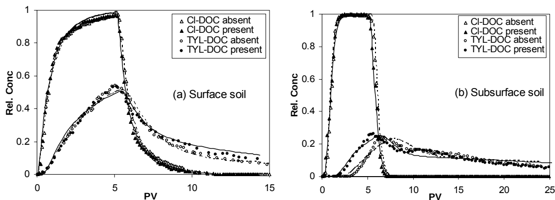
Figure 3.17. Dissolved organic carbon (DOC) effect on tylosin (TYL) mobility for Captina sandy loam. Concentration of DOC added to input solution was 63 \text{ mg L}^{-1} . Symbols represent measured breakthrough curves (BTCs) and lines represent fitted BTCs for which transport parameter estimates are listed in Table 3.12.
