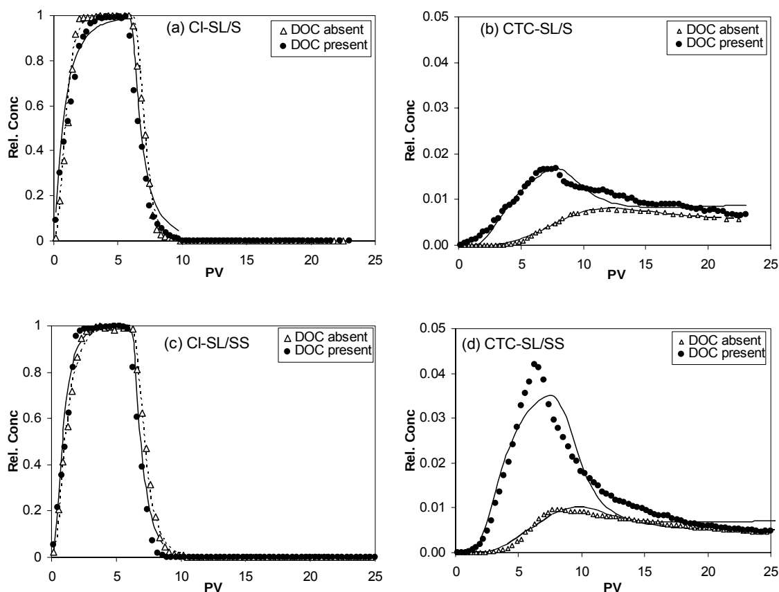
Figure 3.16. Dissolved organic carbon (DOC) effect on chlortetracycline (CTC) mobility. Cl - and CTC are chloride and chlortetracycline, respectively. SL/S and SL/SS are Captina sandy loam surface and subsurface soil, respectively. Concentrations of DOC added to input solution were 63 mg L -1 for surface soil and 21 mg L -1 for subsurface soil. Symbols represent measured breakthrough curves (BTCs) and lines represent fitted BTCs for which transport parameter estimates are listed in Table 3.11.
