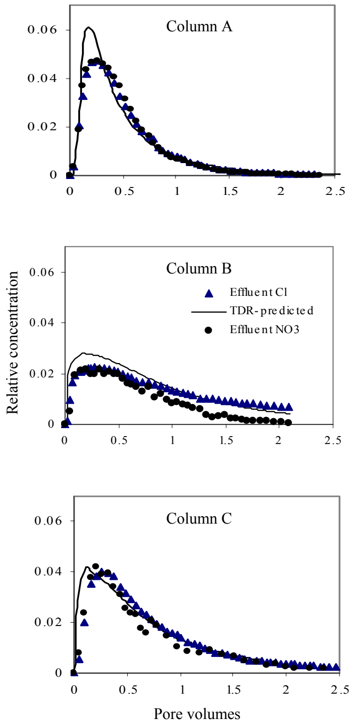
Figure 1.1. Measured effluent chloride and nitrate BTCs along with TDR-predicted BTCs. The “TDR-predicted” BTCs were obtained using TDR data and the CXTFIT program.
