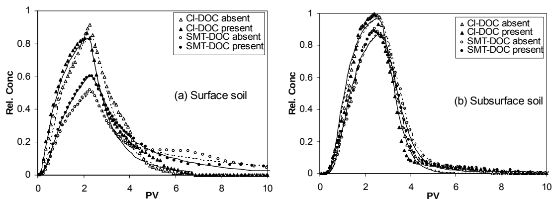
Figure 3.18. Dissolved organic carbon (DOC) effect on sulfamethazine (SMT) mobility for Captina sandy loam. Concentration of DOC added to input solution was 63 \text{ mg L}^{-1} . Symbols represent measured breakthrough curves (BTCs) and lines represent fitted BTCs for which transport parameter estimates are listed in Table 3.13.
