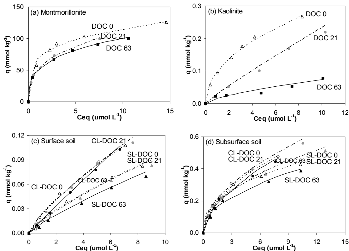
Figure 3.14. Dissolved organic carbon (DOC) effect on tylosin (TYL) sorption. DOC= 21 and 63 \text{mg L}^{-1} . SL= sandy loam, CL= clay loam. Symbols represent experimental data and lines represent isotherm models for which parameters are listed in Table 3.8. The sorption data were obtained by equilibrating 0.30 \text{ g L}^{-1} of \text{Ca}^{2+} -saturated montmorillonite, 6.0 \text{ g L}^{-1} of \text{Ca}^{2+} -saturated kaolinite, or 50 \text{ g L}^{-1} of soils in 0.01 \text{ M Ca(NO}_3)_2 containing 0.0008\text{-}0.059 \text{ mM TYL} . Solution pH values were 5.0 (montmorillonite), 5.2 (kaolinite), 5.3 (CL-S), 5.4 (CL-SS), 5.4 (SL-S), and 5.6 (SL-SS) in the absence of DOC and 5.6 (montmorillonite), 5.3 (kaolinite), 5.3 (CL-S), 5.5 (CL-SS), 5.5 (SL-S), and 5.6 (SL-SS) in the presence of dairy manure DOC. The suspensions were equilibrated for 24 h at 20 to 22^\circ\text{C} .
