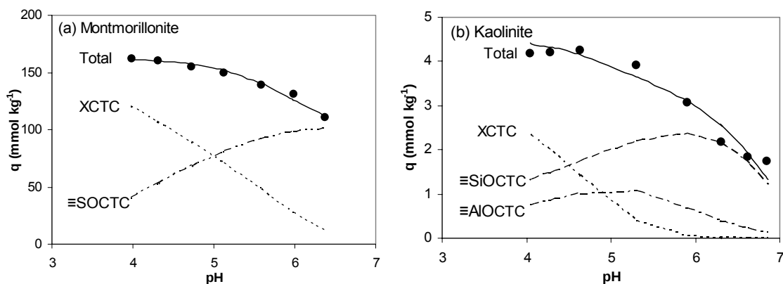
Figure 3.4. Effect of pH on chlortetracycline (CTC) sorption. Closed circles represent experimental data and lines represent modeled complexes. The sorption data were obtained by equilibrating 0.45 \text{ g L}^{-1} of \text{Na}^{+} -saturated montmorillonite or 3.6 \text{ g L}^{-1} of \text{Na}^{+} -saturated kaolinite in 0.01 \text{ M NaNO}_3 containing 0.072 \text{ mM CTC} . The suspensions were equilibrated for 48 h at 20 to 22^{\circ}\text{C} .
