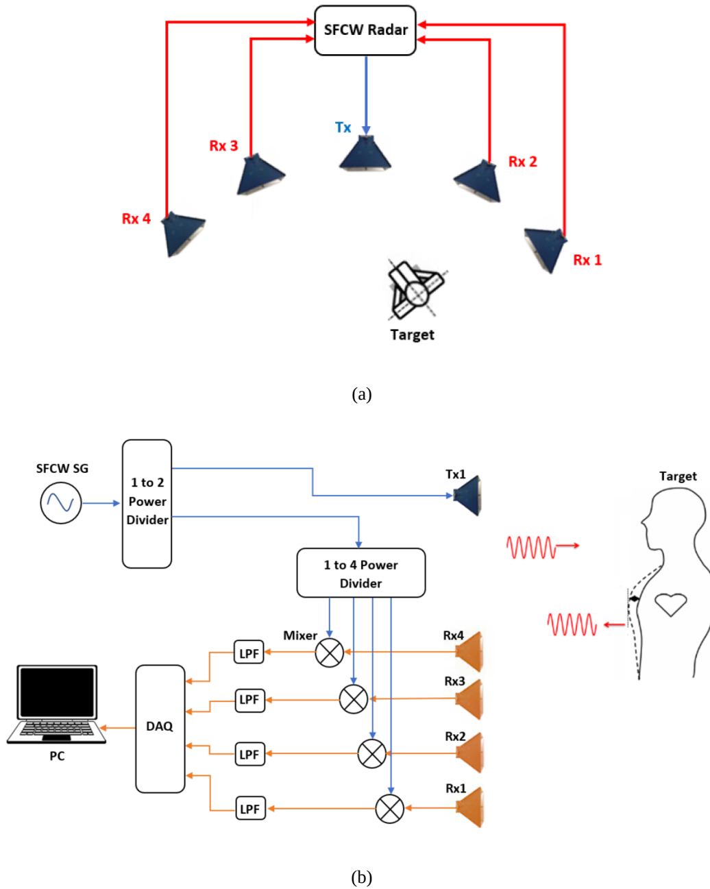
Figure 7.11 (a) MIMO SFCW radar system with one transmitter and four receivers (top view); (b) Block diagram of the MIMO SFCW radar with one transmitter and four receivers.
