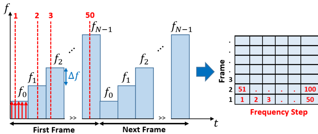
Figure 4.6 Time-frequency representation of SFCW and frame fitting.
