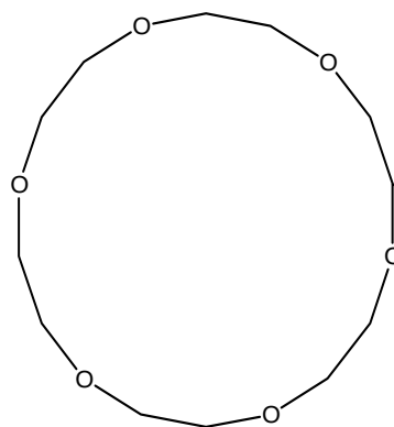
18-crown-6
