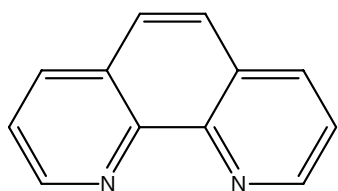
1,10-phenanthroline
