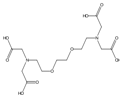
[ethylenebis(oxy-ethylenenitrilo)]tetraacetic acid
