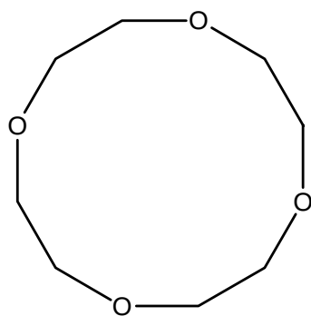
12-crown-4
