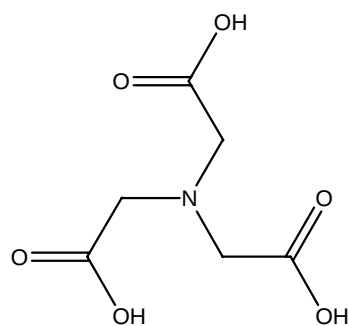
nitrilotriacetic acid
