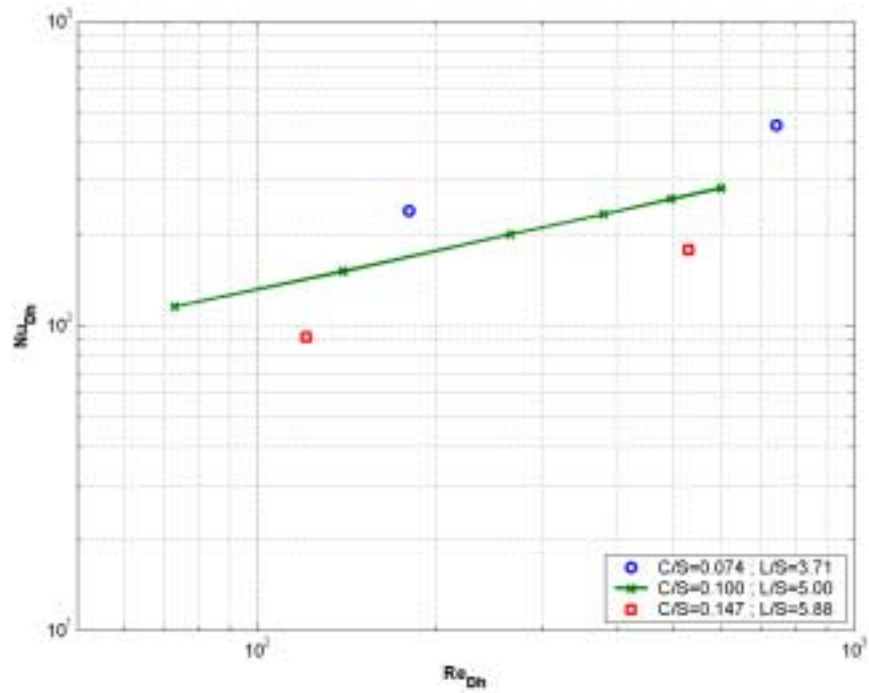
Figure 6.11. Nusselt number as a function of Reynolds number for optimal cases.
