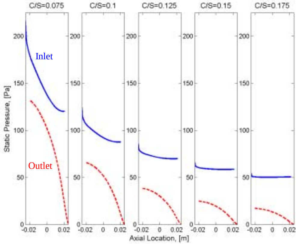
Figure 6.5. Effect of C/S on static pressure along inlet and outlet slots for L=0.05\text{m} , Re_K^*=0.1 , L/S=5 .
