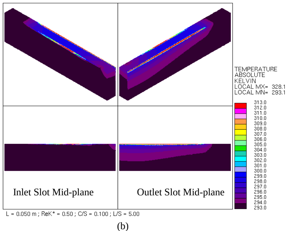
Figure 6.10. Three-dimensional temperature contours for L=0.05\text{m} , C/S=0.100 , L/S=5.00 , \text{Re}_K^*=0.10 (a) and \text{Re}_K^*=0.50 (b).
