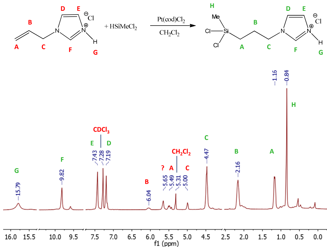
Figure 29: 1 H NMR spectrum of 1-DCMSP-Im Cl via diffusion (400 MHz, CDCl 3 , 23 °C)
