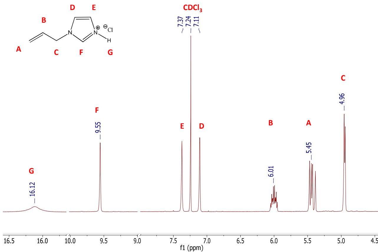
Figure 21: ^1\text{H} NMR spectrum of 1-All-Im Cl (400 MHz, \text{CDCl}_3 , 23 ^\circ\text{C} )
