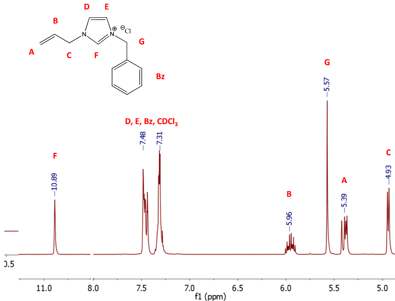
Figure 23: ^1\text{H} NMR spectrum of 1-All-3-Bz-Im Cl (400 MHz, \text{CDCl}_3 , 23 °C)
