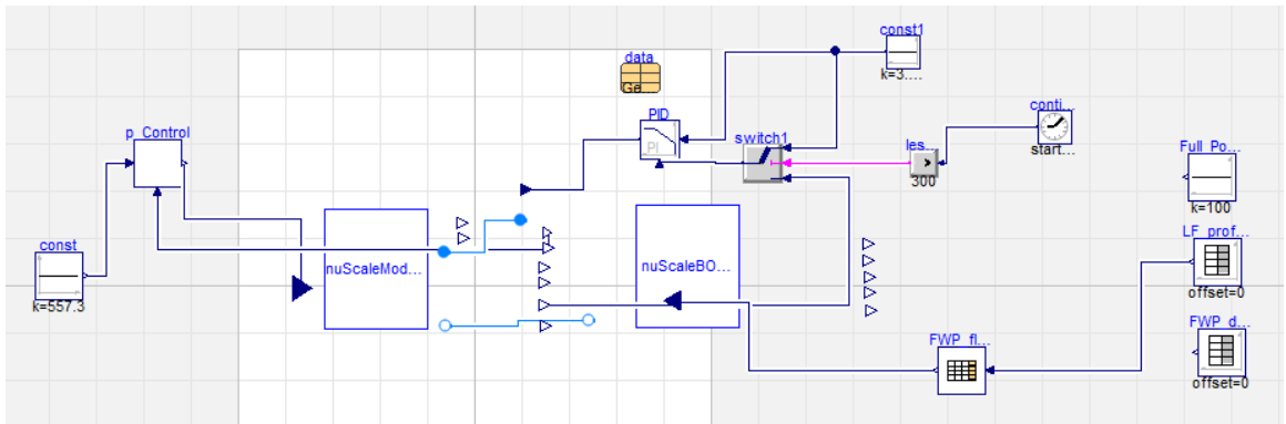
Figure 2.5: NPM model in Dymola Environment
