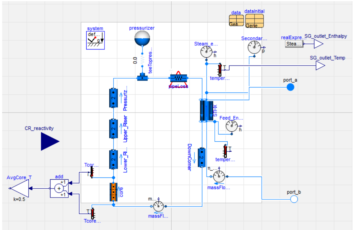
Figure 2.3: Reactor Model in Dymola Environment
