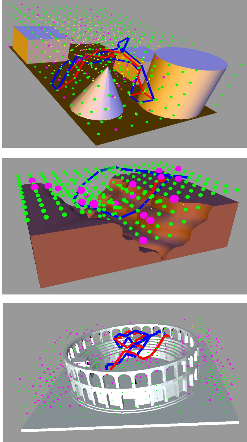
Figure 6.2: The PICRD algorithm in comparison to the naïve Dijkstra algorithm in Scenario 3 with 10% of the grid points removed. Note that the forbidden zones are designated in pink.
