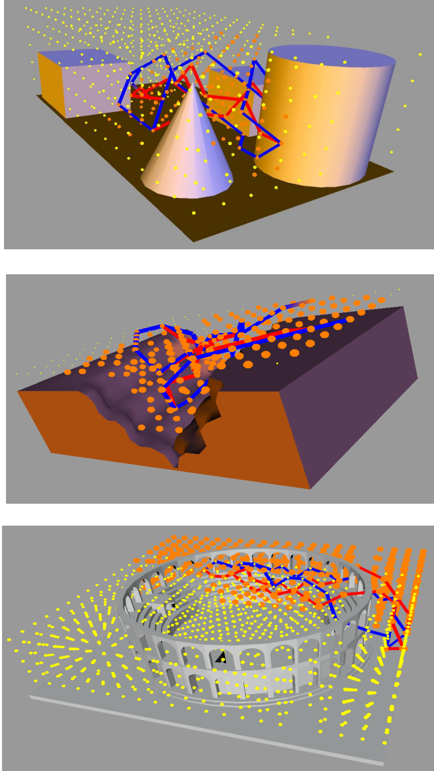
Figure 6.3: The k -means-moderated PICRD algorithm (red route) compared to the naïve Dijkstra algorithm (blue route) operating in circumstances described by Scenario 1.
