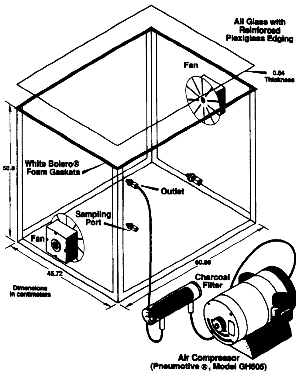
Figure III - 3. Glass exposure chambers used to regulate environmental conditions and quantify ^{14}\text{C} released by the plants in whole plant experiments.
