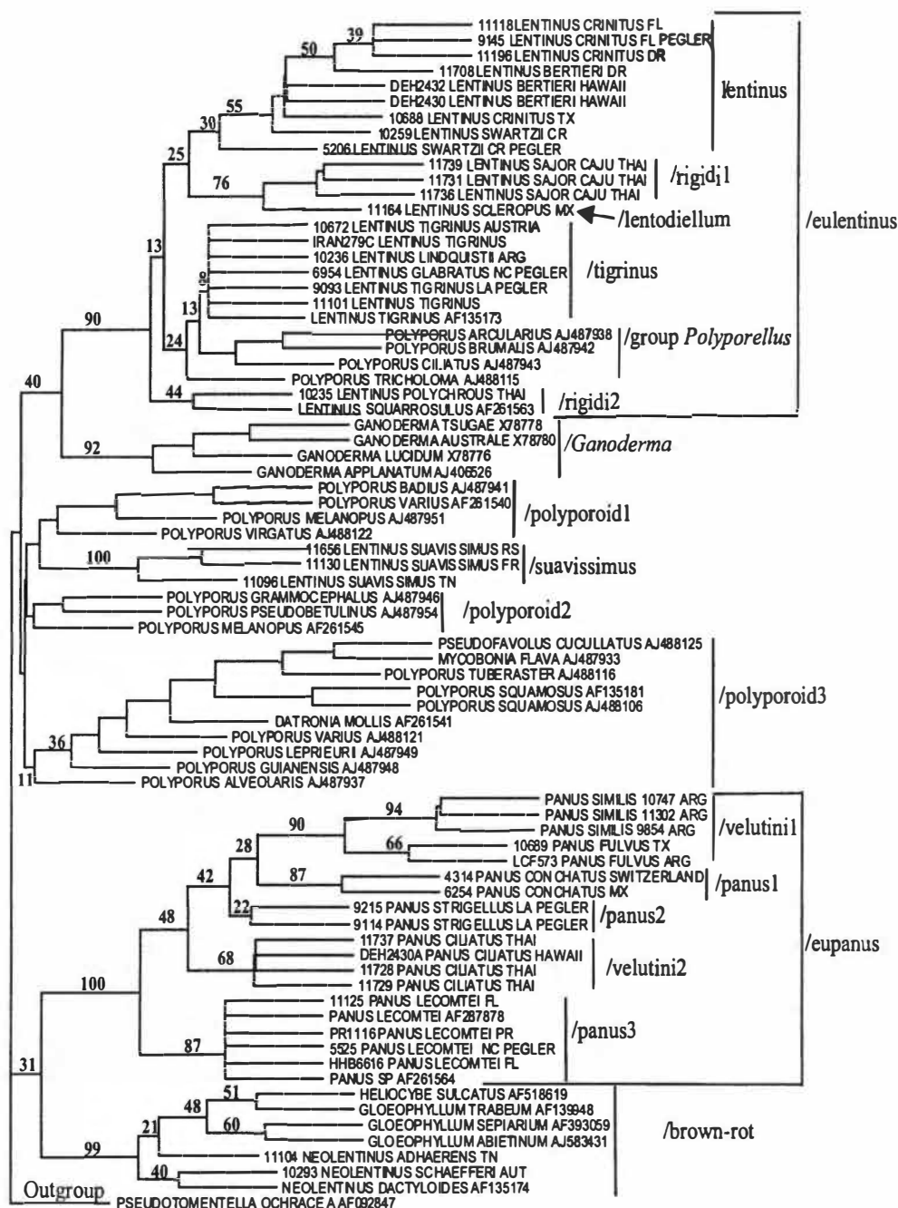
Fig. 1 - Maximum parsimony 50 % majority rule consensus LSU phylogeny. Bootstrap values are proportional to branch lengths and reported on branches preceding clades. 1000 bootstrap replicates were performed. Tree length = 537, consistency index (CI) = 0.4525, homoplasy index (HI) = 0.5475, retention index (RI) = 0.8344.
