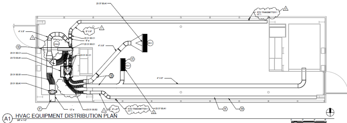
Fig. 4.1. Ducting Layout
