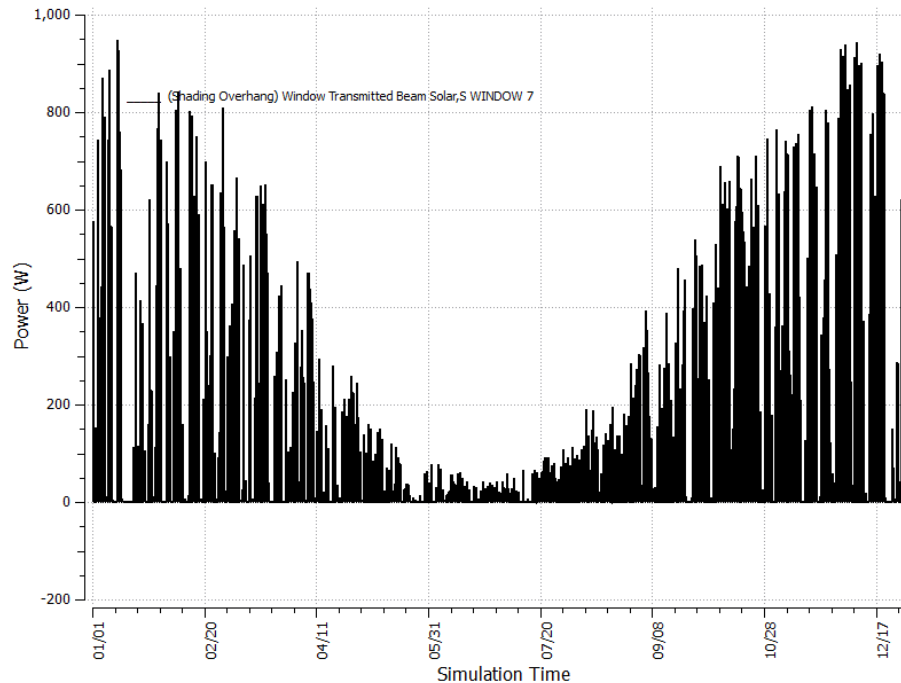
Figure 4.6. Transmitted Beam Solar through a South Façade Window with No Overhang
