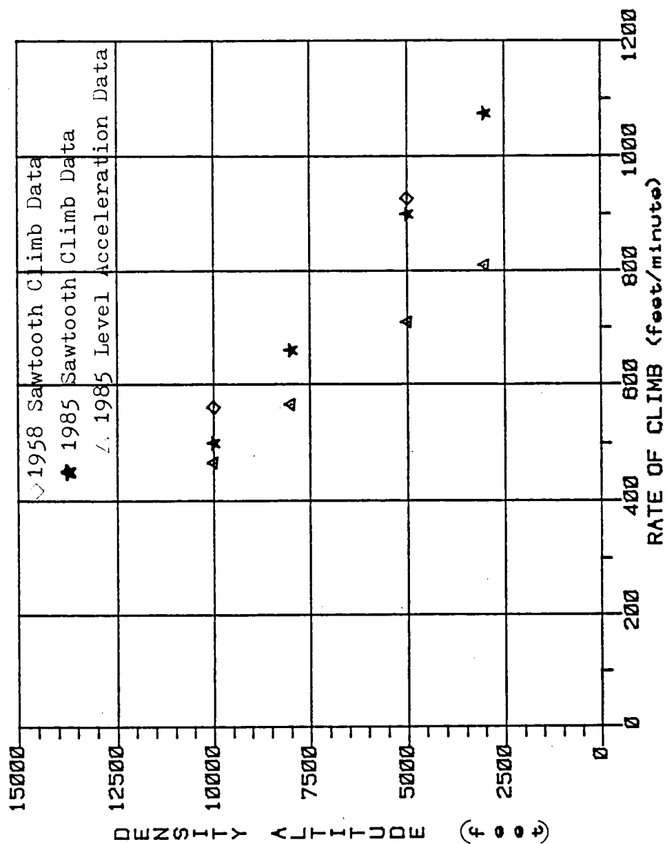
Figure 28. Density Altitude versus Rate of Climb - with Sawtooth Climb and Level Acceleration Results Compared
