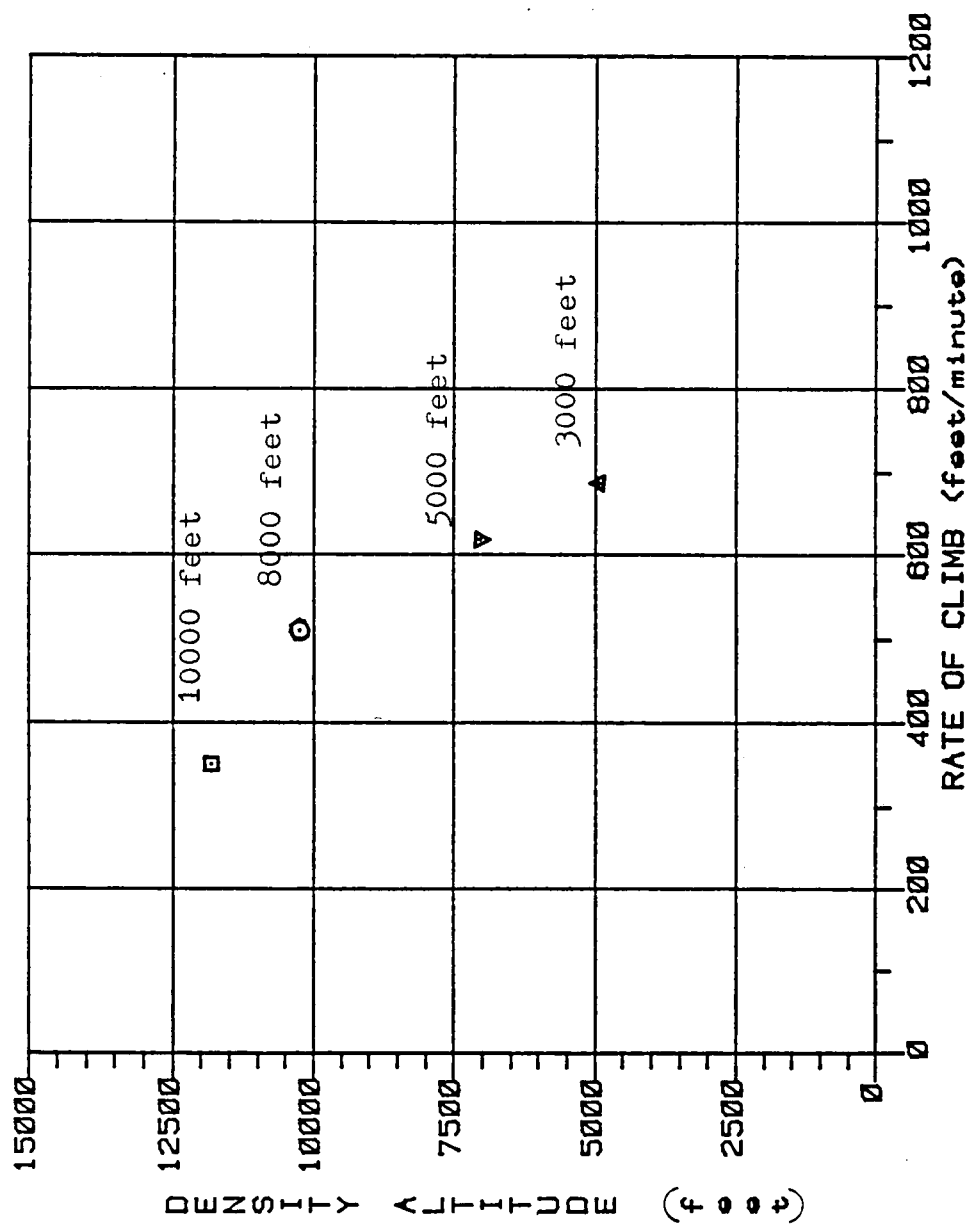
Figure 27.. Density Altitude versus Rate of Climb as Demonstrated by the Level Acceleration Method (Raw Data)
