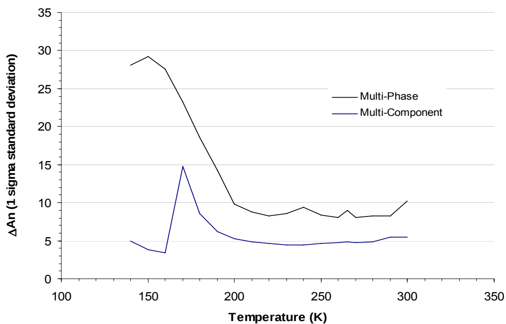
Figure A.4. Anorthite variation (1 \sigma std. dev.) for multi-phase and multi-component mixture deconvolutions vs. temperature (K). \Delta An begins to degrade for both sets of mixtures in the 180-200K range.
