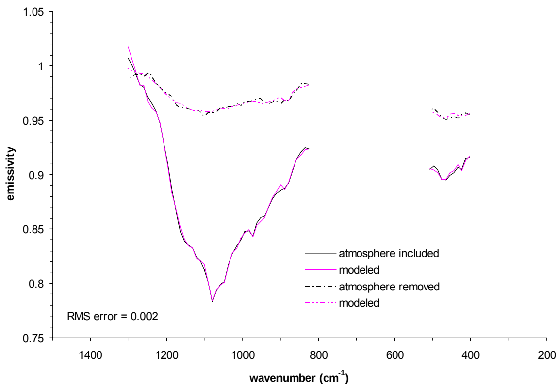
Figure 33. Actual (black) vs. modeled (purple) average TES emissivity spectrum for the Opportunity landing site. Solid lines are spectra with the atmospheric component included, while dashed line spectra have atmospheric components removed.
