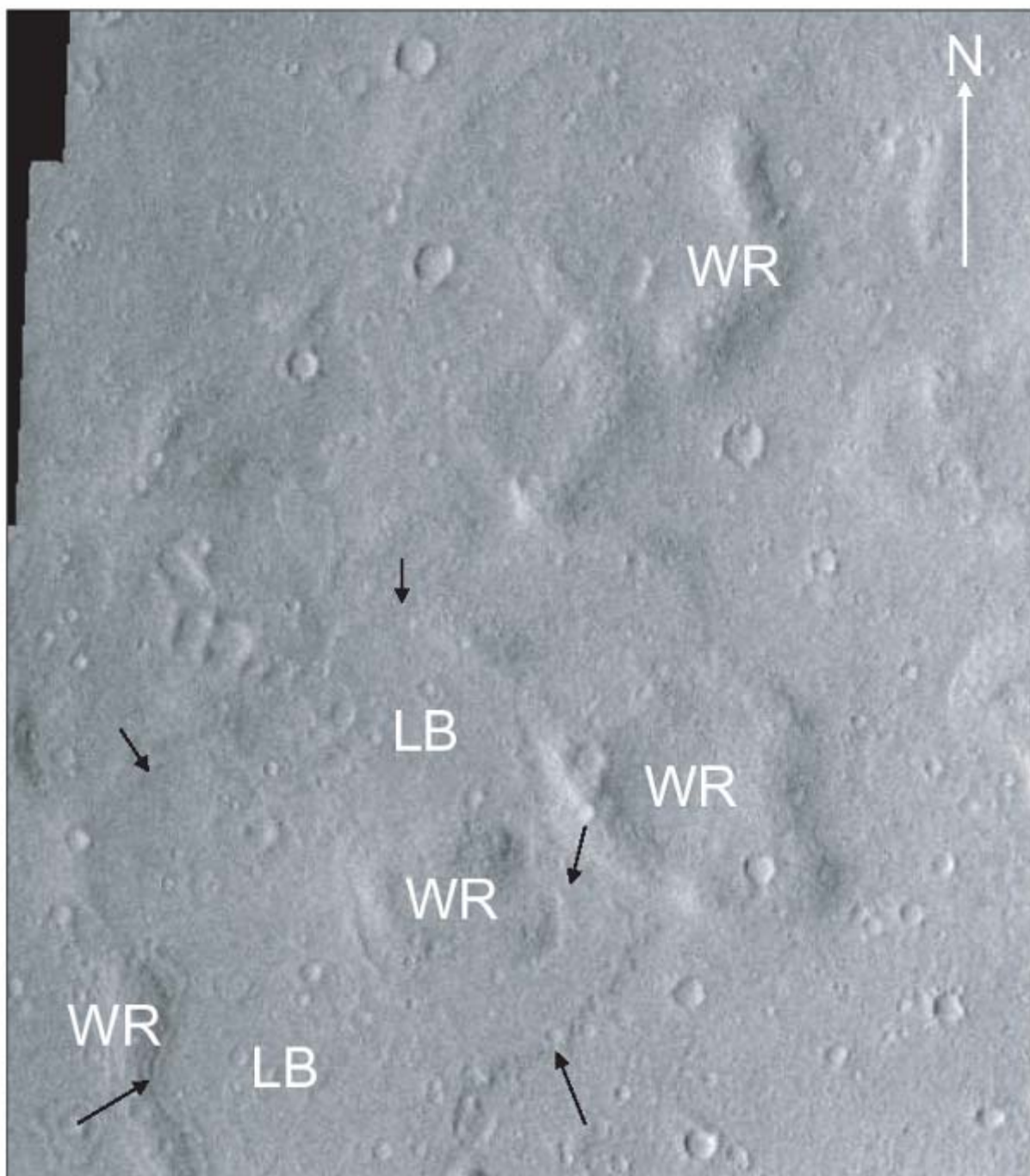
Figure 18. LB deposited against and between ridges of WR in north central Gusev (THEMIS-V-01580003).
