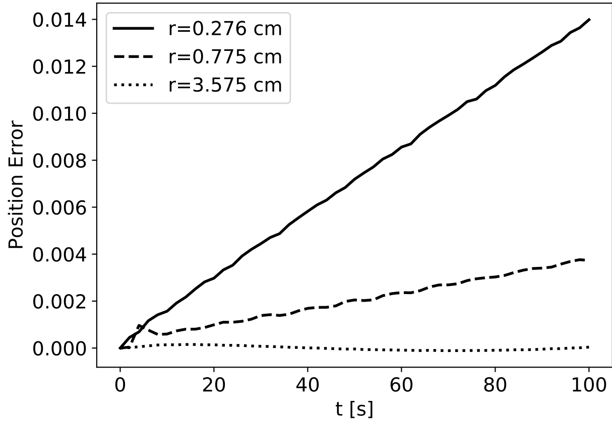
Figure 2.5: Particle trajectory errors ( [r(t) - r(0)]/[r(0)] ) for three specific particles in the isentropic vortex test problem. The solid line is the inner particle, dashed line is the middle particle, and dotted line is the outer particle.
