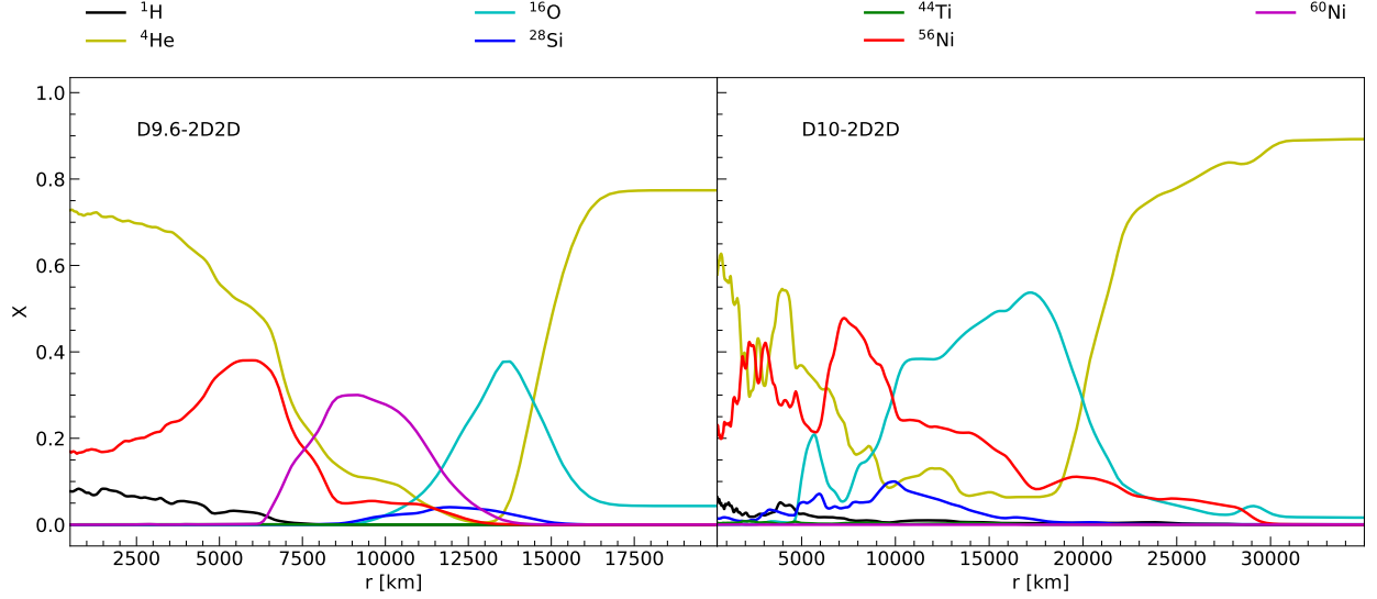
Figure 2.6: Angle-averaged mass-fractions of inner ejecta for D9.6–2D2D (left) and D10–2D2D (right) at t_{\text{map}} .
