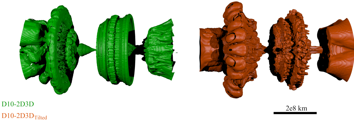
Figure 3.24: External coating X_{56\text{Ni}+\text{IG}} = 0.1\% isosurface for the D10–2D3D (green, left) and D10–2D3D Tilted (orange, right) bullets at shock breakout. Note, the D10–2D3D Tilted isosurface has been realigned in post-processing (i.e. rotated clockwise about its y-axis 90^\circ ) to match the orientation of the other model. The open ended “caps” are due to the poles evolving off the grid much earlier in the simulation.
