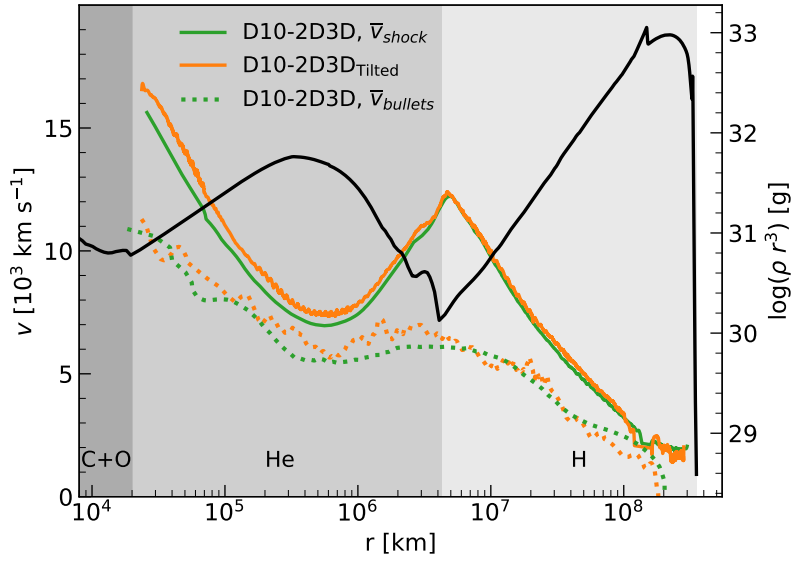
Figure 3.20: Angle-averaged shock velocity (colored, solid lines) and angle-averaged bullet velocity of the X_{^{56}\text{Ni}+\text{IG}} = 3\% isosurface (colored, dashed lines) for the D10 models as functions of their respective angle-averaged shock or bullet radii. Density profile of the D10 progenitor prior to bounce (black, solid) displays the change of \rho r^3 and spans the right axis. Grey shaded sections highlight the regions of the (C+O), He, H shells up to the defined R_{\text{Int}} in Table 2.1.
