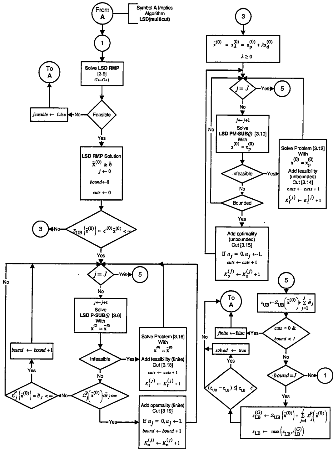
Figure 3.3: Procedure LSD(multicut)-Initialize Flowchart
