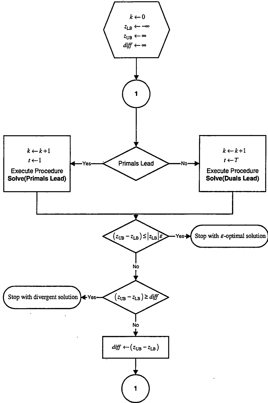
Figure B.1: Algorithm MDPCA Flowchart
