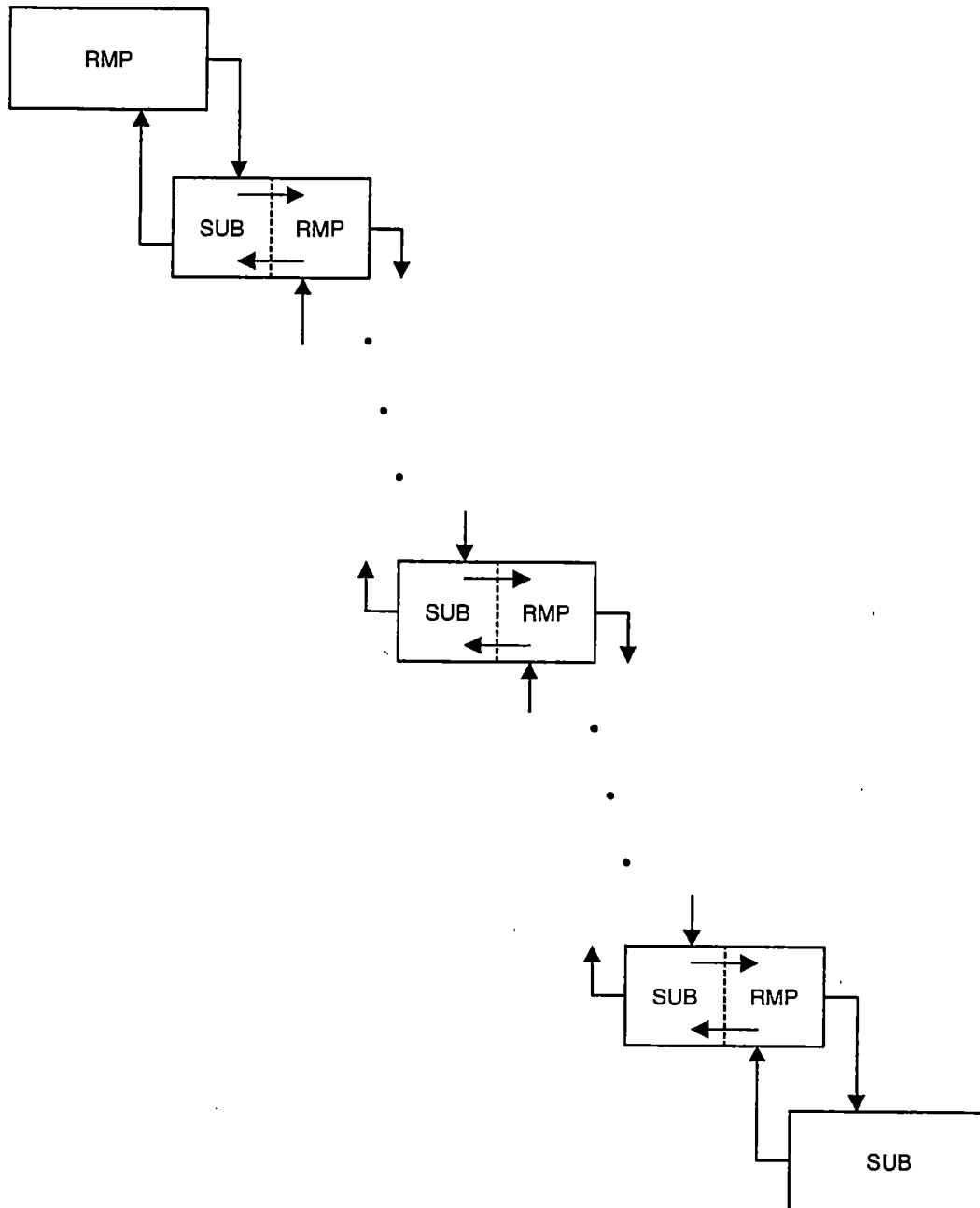
Figure 4.2: Nested Decomposition Work Flow – First Period RMP \rightleftharpoons Final Period SUB
