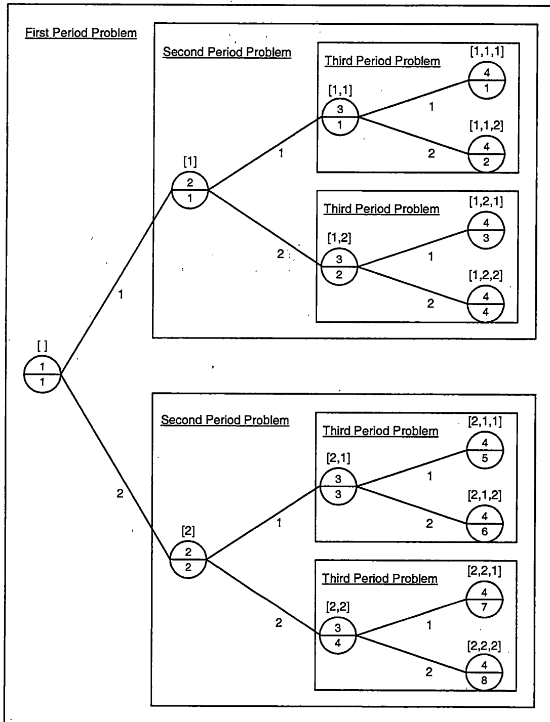
Figure 4.1: Four-Period Binary Outcomes Decision Tree - Nested Two-Period Problems
