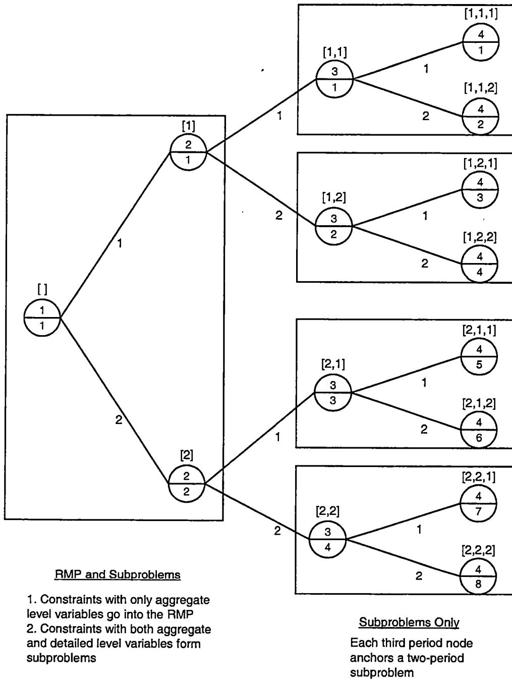
Figure 4.3: Four Period Block-Separable Problem With \bar{t} = 2
