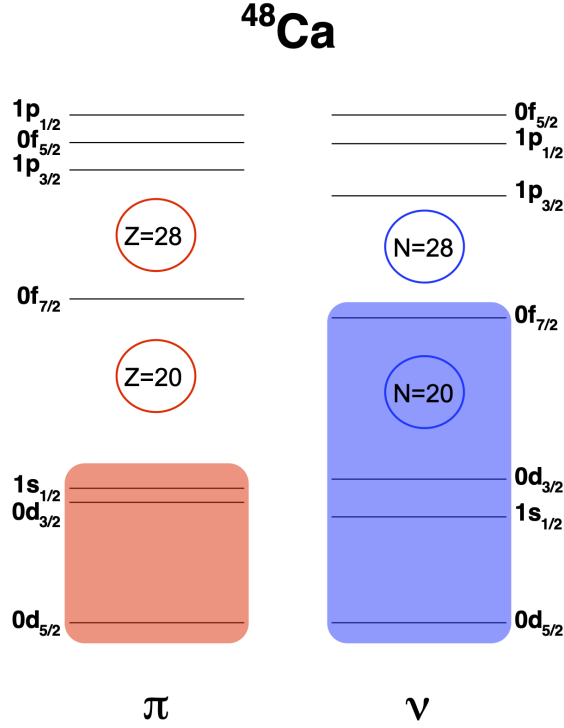
Figure 1.1: Orbitals for ^{48}\text{Ca} , where the protons ( \pi ) fill up the sd -shell shown as the red block consisting of the d_{5/2} , d_{3/2} , and s_{1/2} orbitals and the neutrons ( \nu ) occupy up to the f_{7/2} orbital, shown as the blue block on the right.
