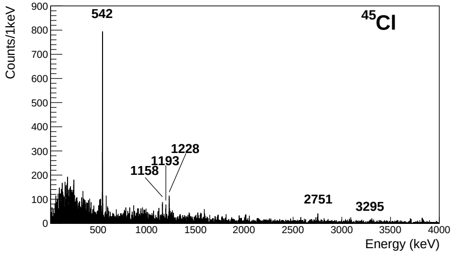
Figure 5.10: The negative-time subtracted HPGe discrete \gamma -ray spectrum for ^{45}\text{Cl} .
