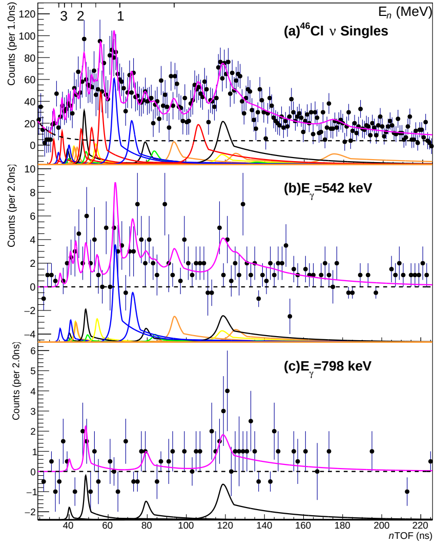
Figure 5.20: Neutron time-of-flight deconvolution from the decay of ^{46}\text{Cl} .
