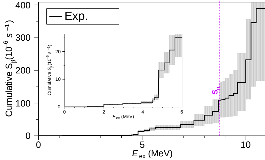
Figure 5.7: The cumulative \beta -decay strength for ^{44}\text{Cl} , with the inset plot zoomed into the range of previous \beta -decay measurements, < 6 \text{ MeV} . The neutron separation energy, S_n = 8.73 \text{ MeV} is shown as the purple dashed line.
