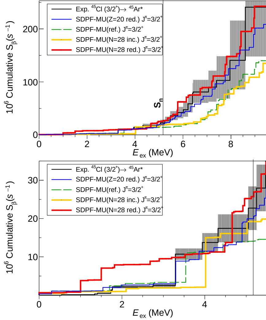
Figure 6.4: Comparing the effect on the cumulative S_\beta distribution for ^{45}\text{Cl} due to the modification of the N = 28 shell gap in the SDPF-MU interaction. The red (yellow) curve represents the reduced (increased) N = 28 modified SDPF-MU predictions.
