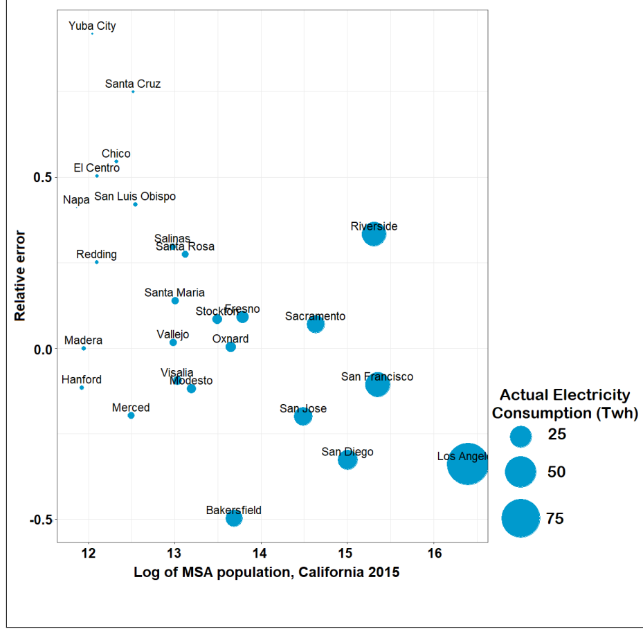
Figure 5.3: Relative errors for California MSAs.
