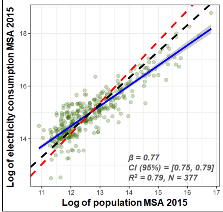
Figure 5.5: Scaling of urban electricity consumption and population, MSAs 2015.
