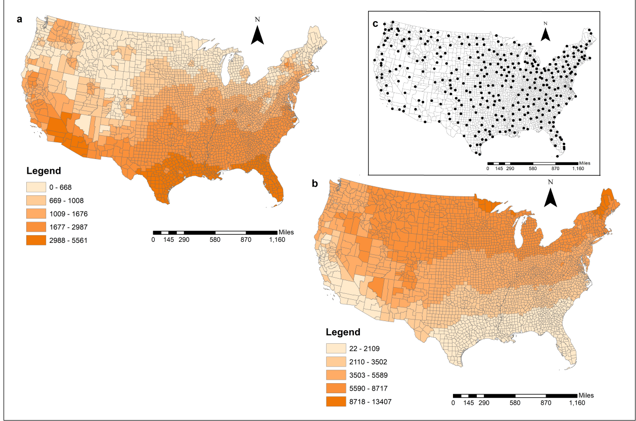
Figure 5.2: Estimated (a) CDDs and (b) HDDs at county level. (c) NOAA weather station locations are shown in the inset.
