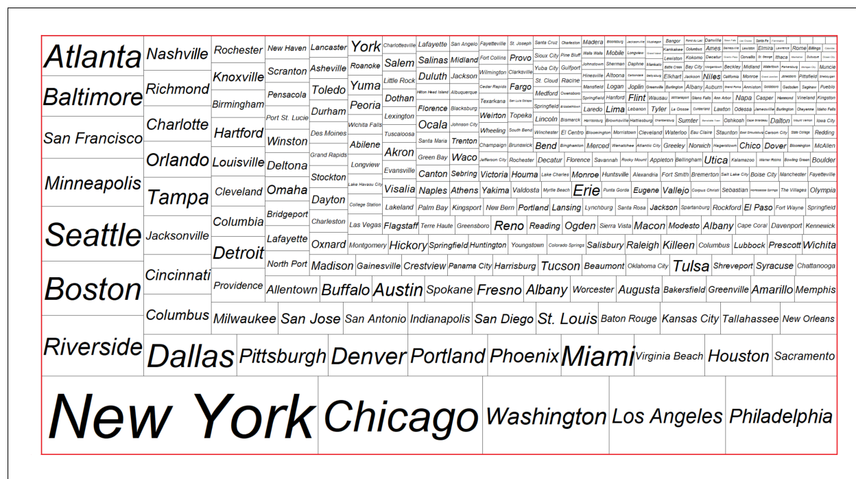
Figure 5.4: Estimated electricity consumption in MSAs. Each small square is proportional to consumption, the rectangle circumscribed in thick red line represents total 2015 urban electricity consumption.
