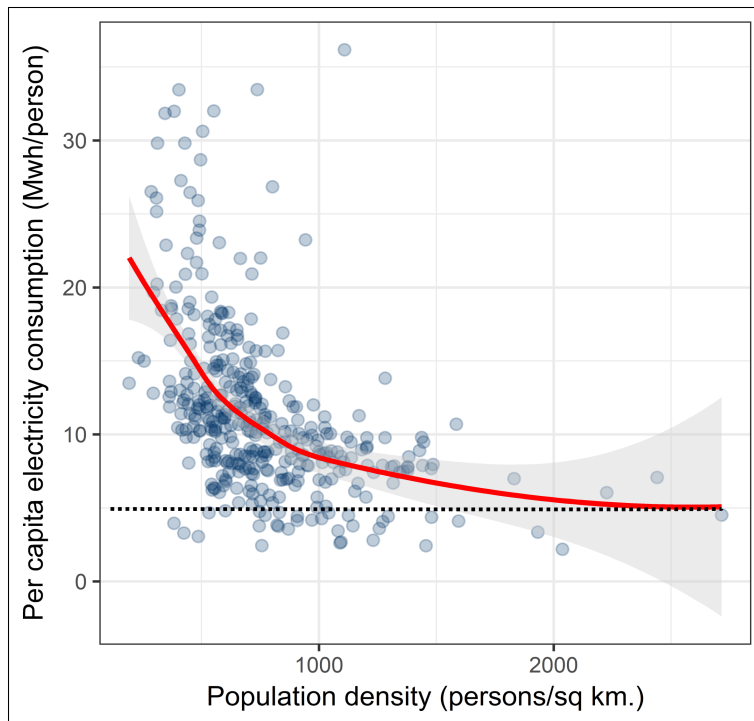
Figure 5.6: Per capita electricity consumption and population density, MSAs in the United States 2015. The black dashed line at y \approx 5 indicates the lower limit of per-capita electricity consumption.
