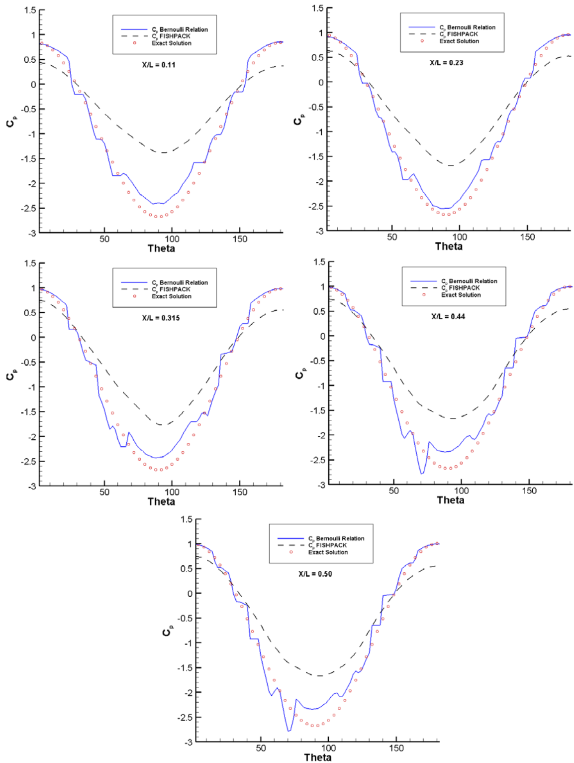
Figure 4-11. Pressure Coefficient, cross planes, 90^\circ incidence, inviscid surface model.
