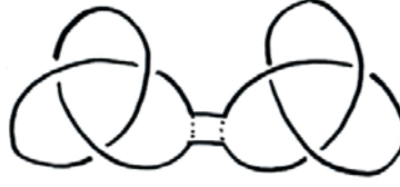
Figure 1.2: The composition of two trefoil knots
