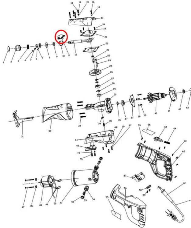
Figure 10. Location of ball cover
