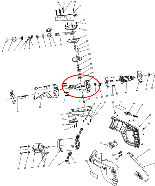
Figure 23. Location of gear housing
