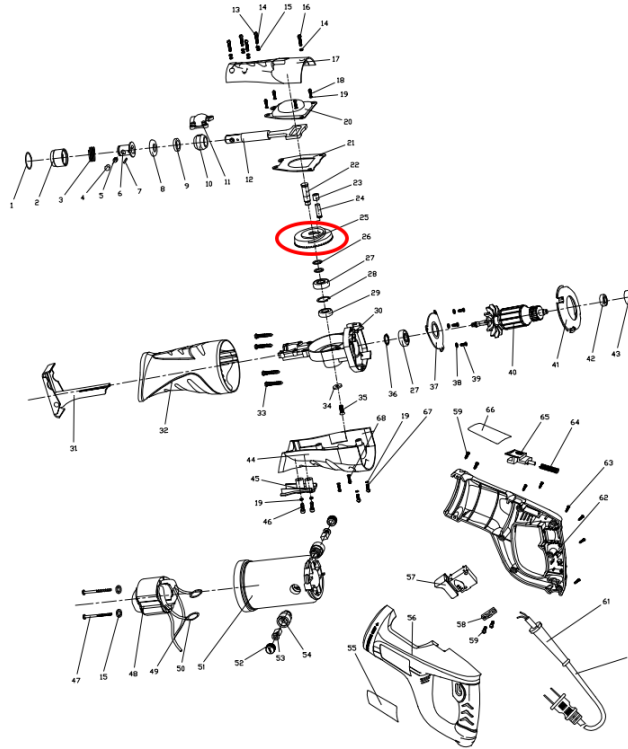
Figure 20. Location of gear
