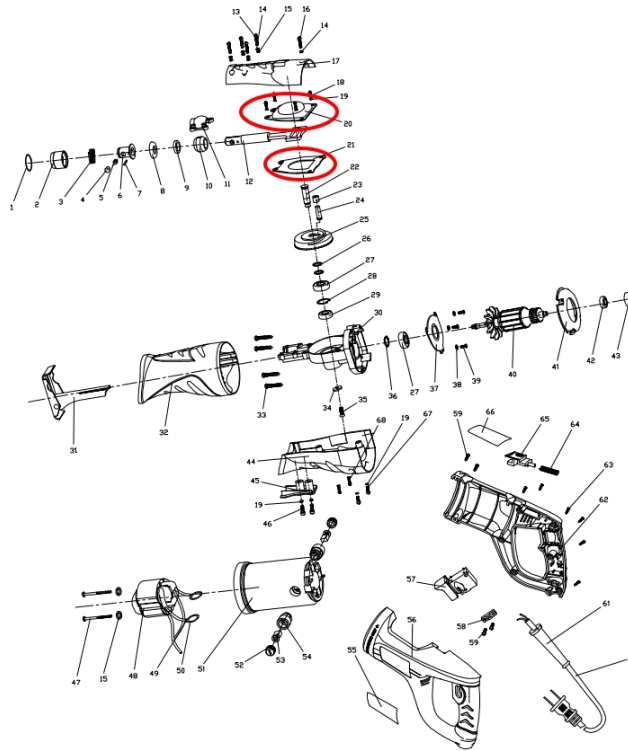
Figure 17. Location of gasket and covering plate
