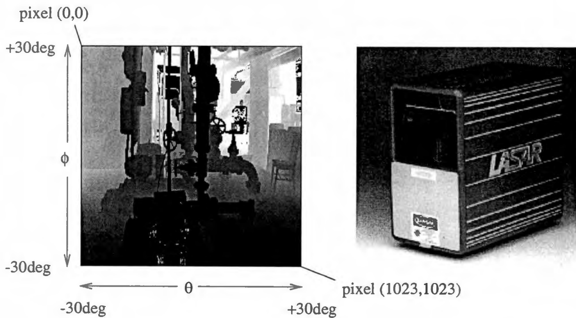
Figure 2: Field of view for a typical range image and the commercially available laser range camera from Percepton [29] which captured this image.
