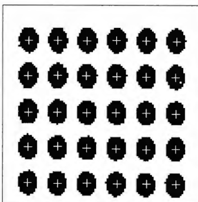
Centroids Found
