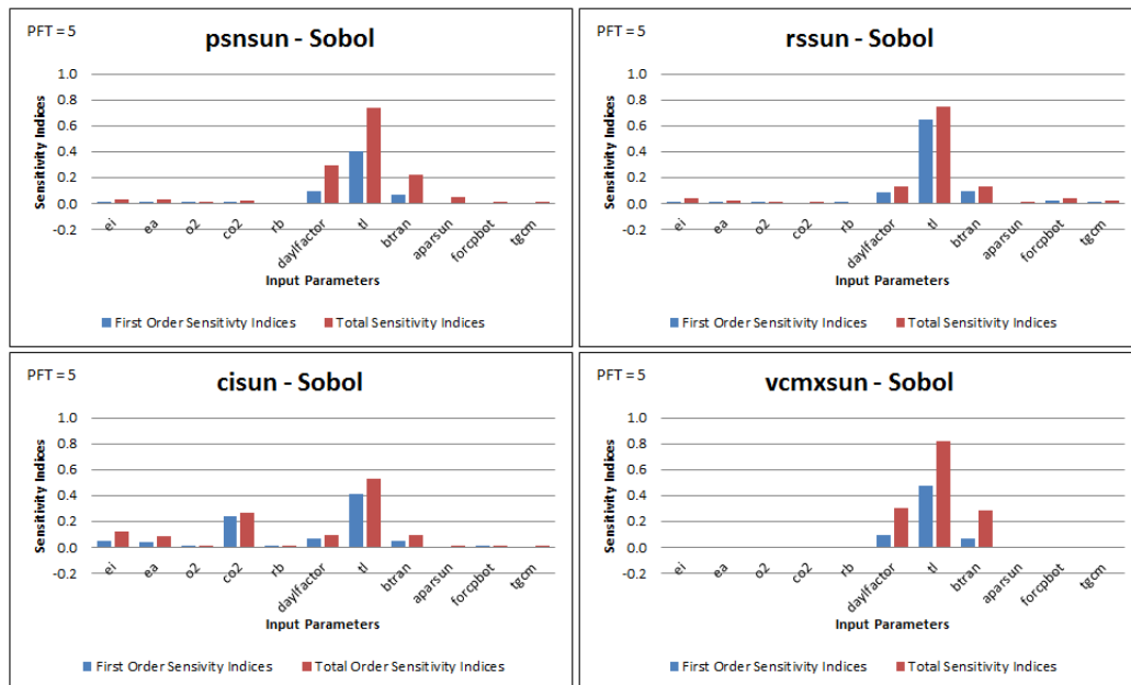
Figure 19. The Sobol Method
