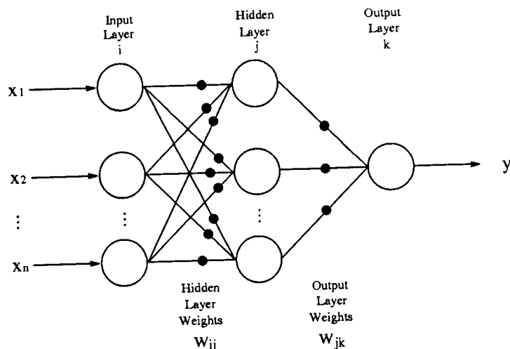
Figure 1.1: Fully-Connected Multi-Layer n - n-1 Artificial Neural Network with Three Layers of Neurons and Two Layers of Trainable Weights.
