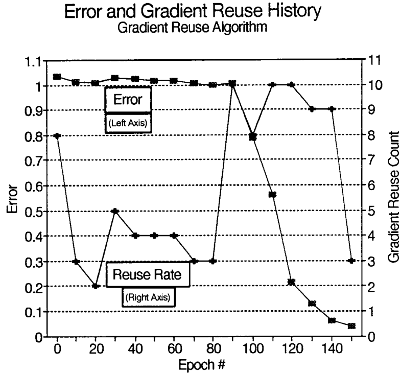
Figure 5.2: Overall System Error and Gradient Reuse Rates for the 2-Bit XOR Problem Using the GRA.
