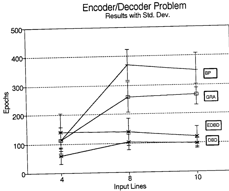
Figure 5.11: Graph of Best Average Convergence Times with Std. Dev. (from Sets of Runs with 100% Convergence) for the Encoder/Decoder Problem.
