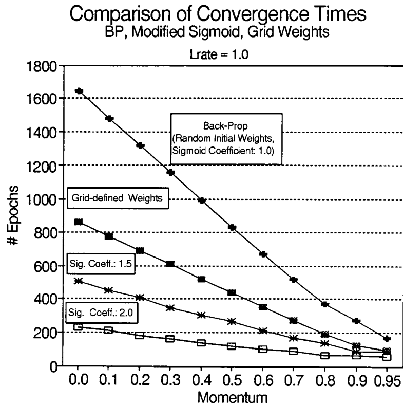
Figure 5.7: Graph of Convergence Times using Random and Predefined Initial Weights, and Modified Sigmoid Coefficients with the BP Algorithm on the 2-Bit XOR Problem.
