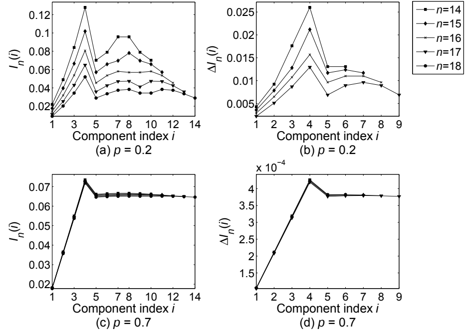
Figure 2.6: The changes of BIs for Lin/Con/4/n:F systems for n = 14, 15, 16, 17 , and 18
