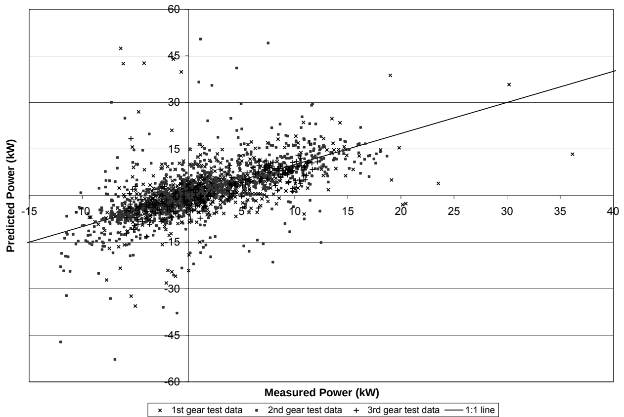
Figure 45: The discrete predicted mobility power values from the Trimble 132 GPS receiver during uncontrolled compared to the measured drivewheel power
