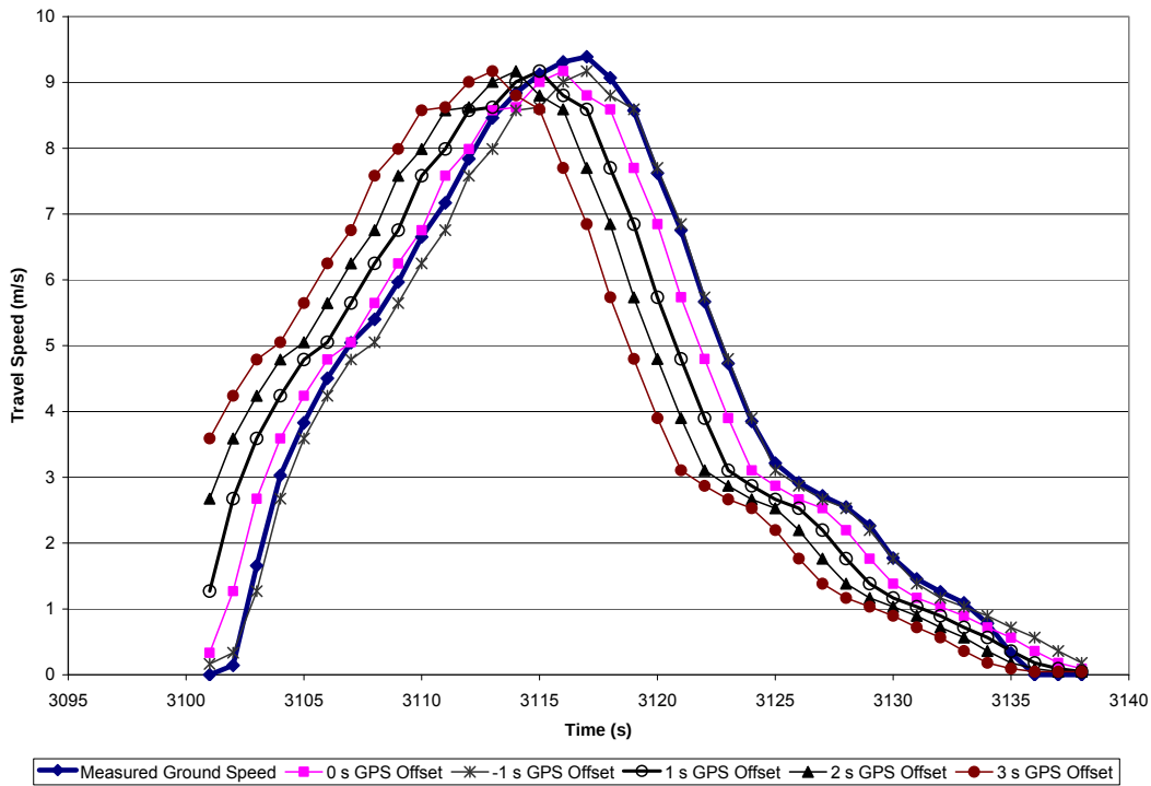
Figure 68: Vehicle travel speed at various Trimble 132 GPS offsets during a medium inertia test
