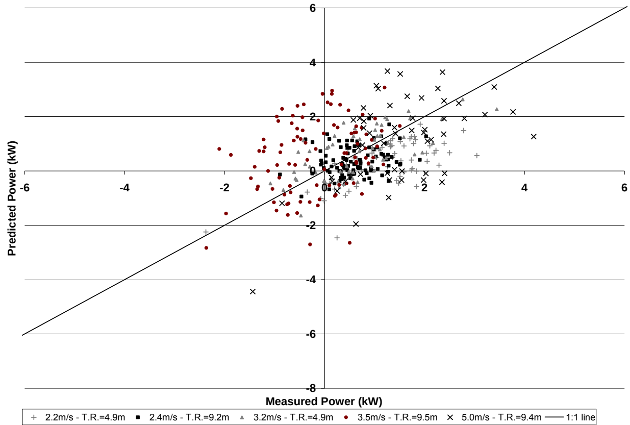
Figure 26: The discrete predicted mobility power values from the Trimble 132 GPS receiver during five constant turning radius motion resistance tests compared to the measured drivewheel power
