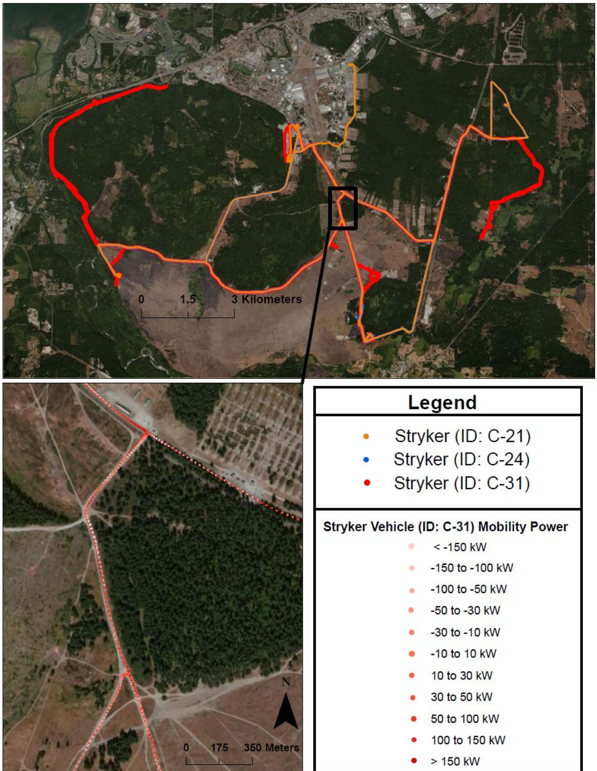
Figure 58: The maneuvers of the three Stryker vehicles at Fort Lewis, Washington along with a single vehicle's mobility power requirements
