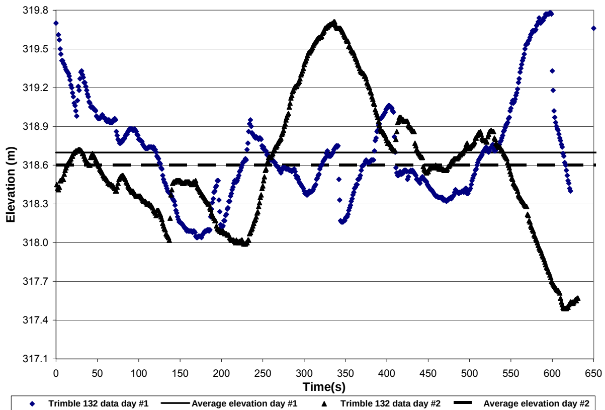
Figure 20: Static Trimble 132 elevation data during two different days at the grade test location
