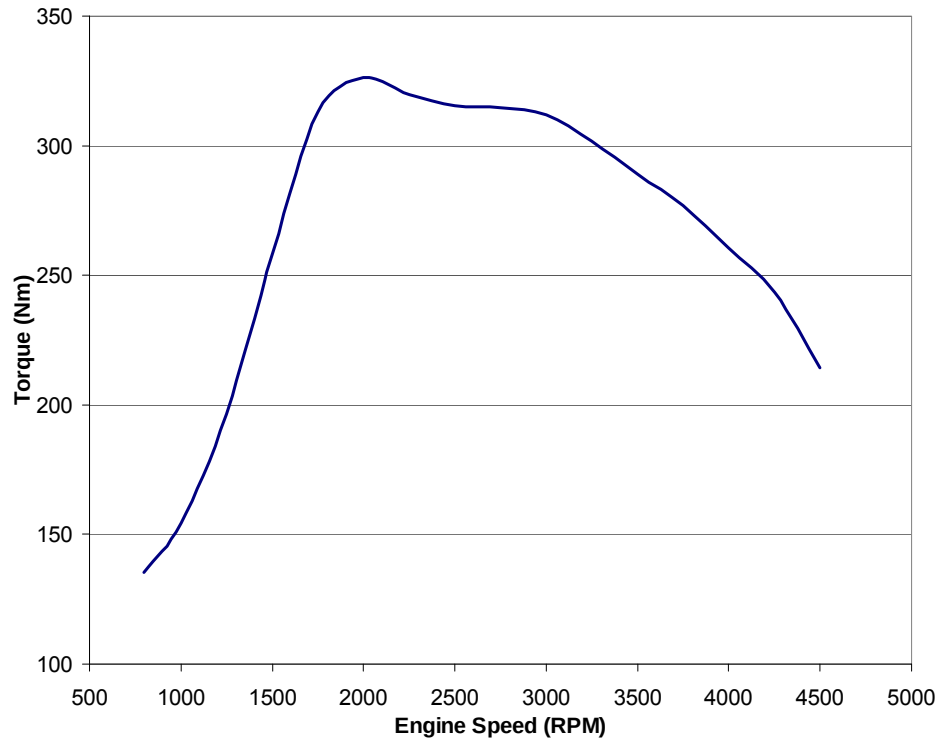
Figure 64: The 1.9L Fiat diesel engine's torque curve
