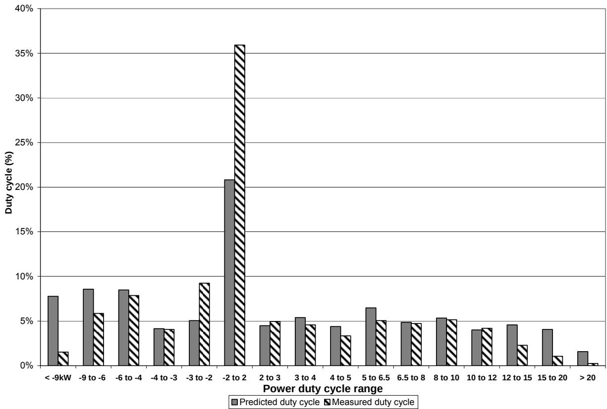
Figure 53: The predicted power duty cycle values from the Garmin 18 receiver compared to the measured duty cycle values
