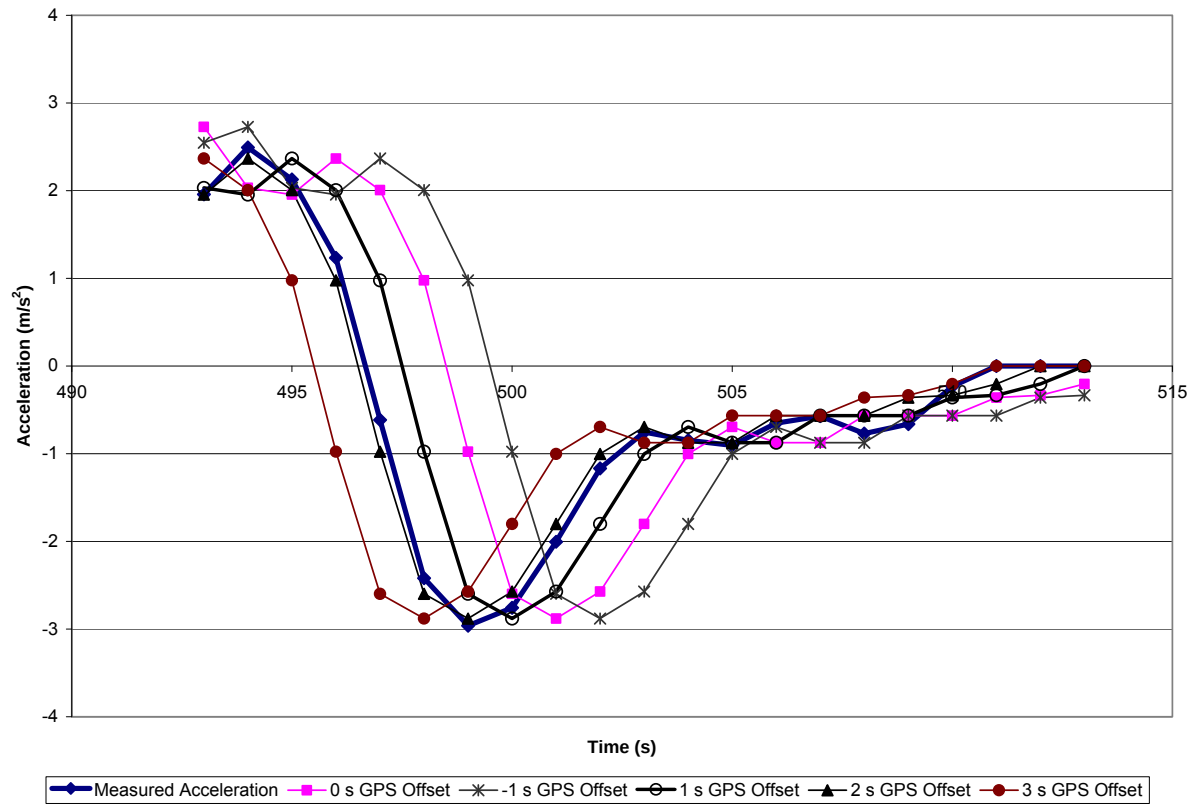
Figure 75: Vehicle acceleration at various Garmin 18 GPS offsets during a fast inertia test
