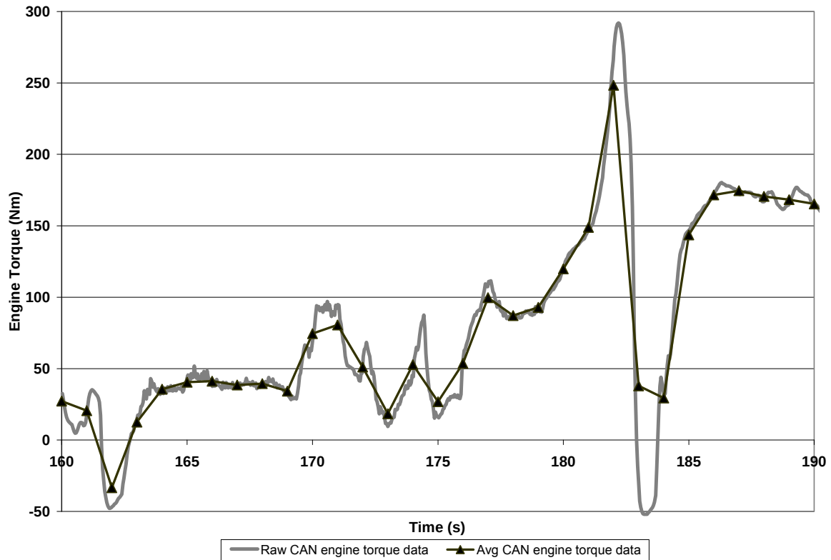
Figure 15: Raw 25 Hz CAN engine torque data and the averaged 1 Hz engine torque data
