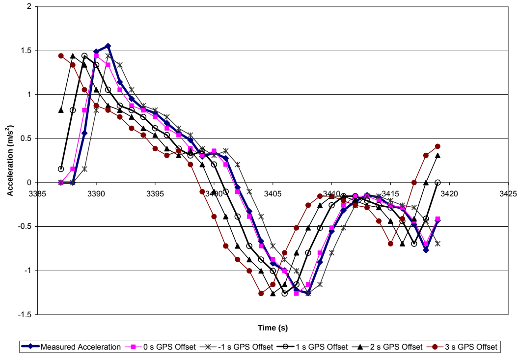
Figure 71: Vehicle acceleration at various Garmin 18 GPS offsets during a medium inertia test
