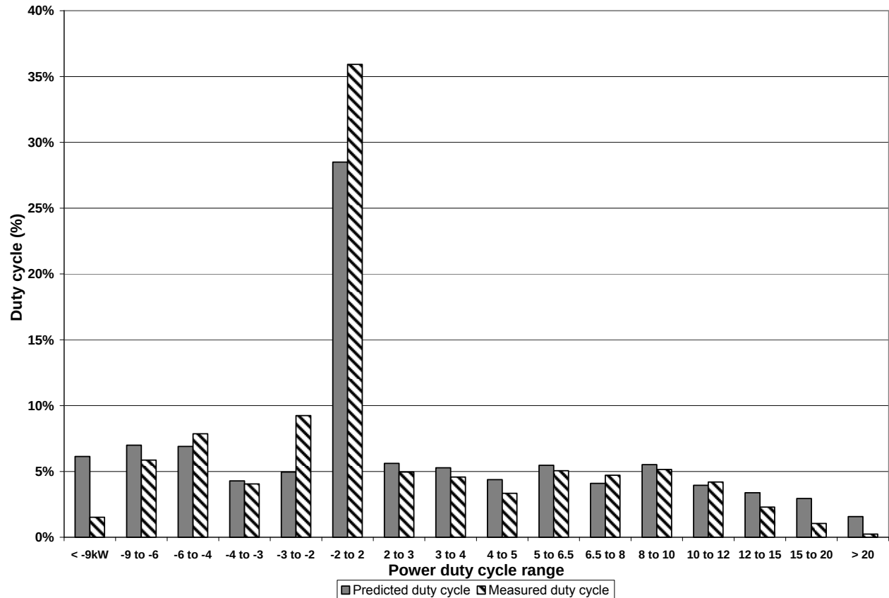
Figure 50: The predicted power duty cycle values from the Trimble 132 receiver compared to the measured duty cycle values
