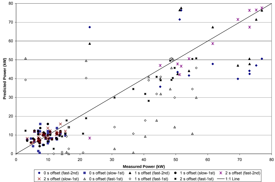
Figure 76: A comparison of predicted and measured mobility power at various GPS speed and acceleration offsets during nine inertia tests for the Garmin 18 GPS receiver
