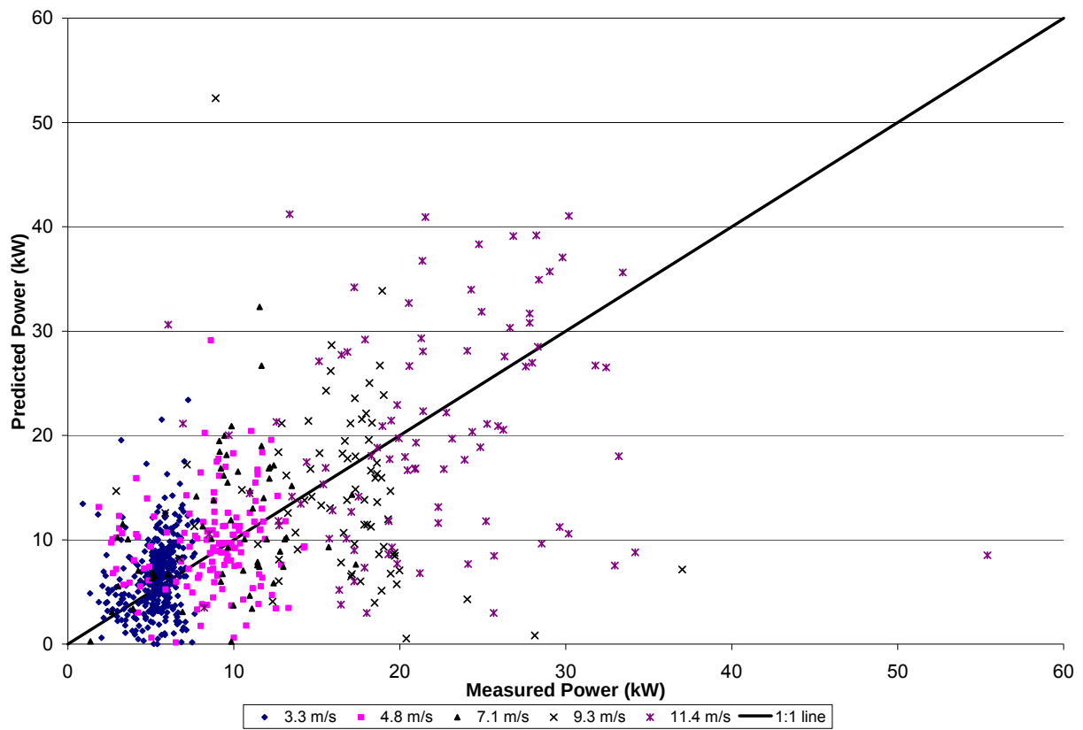
Figure 35: The discrete predicted mobility power values from the Garmin 18 GPS receiver during nine grade tests compared to the measured drivewheel power
