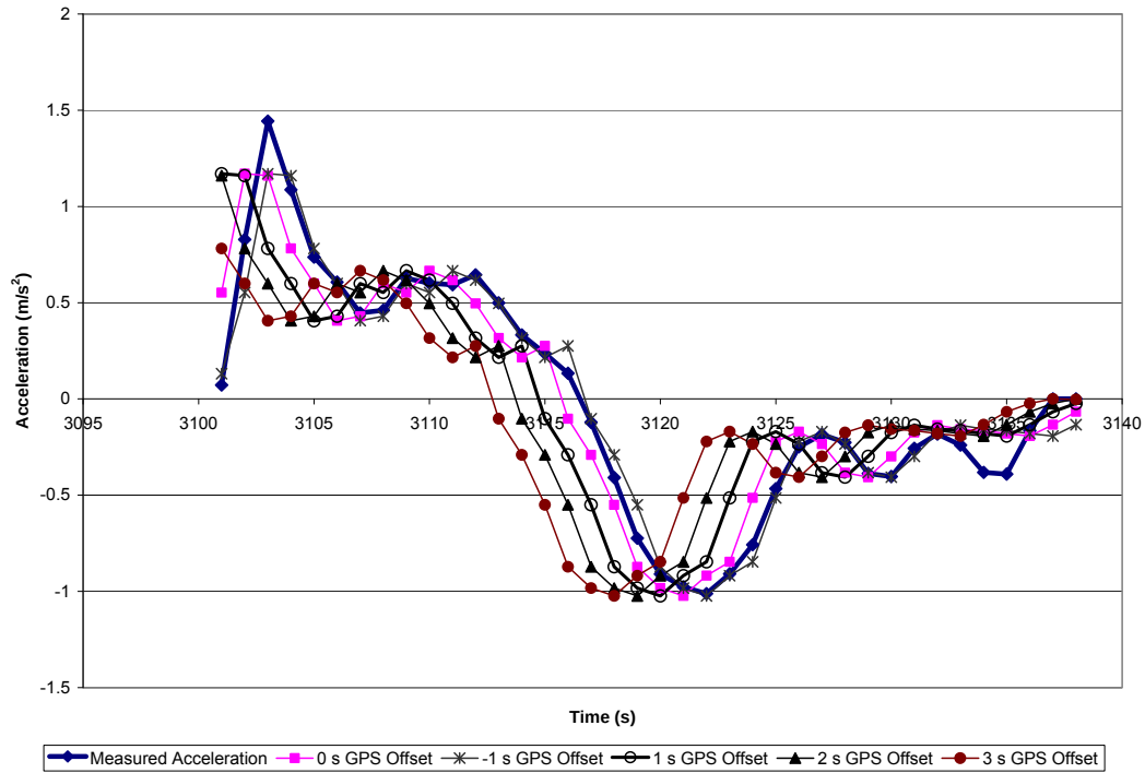
Figure 69: Vehicle acceleration at various Trimble 132 GPS offsets during a medium inertia test
