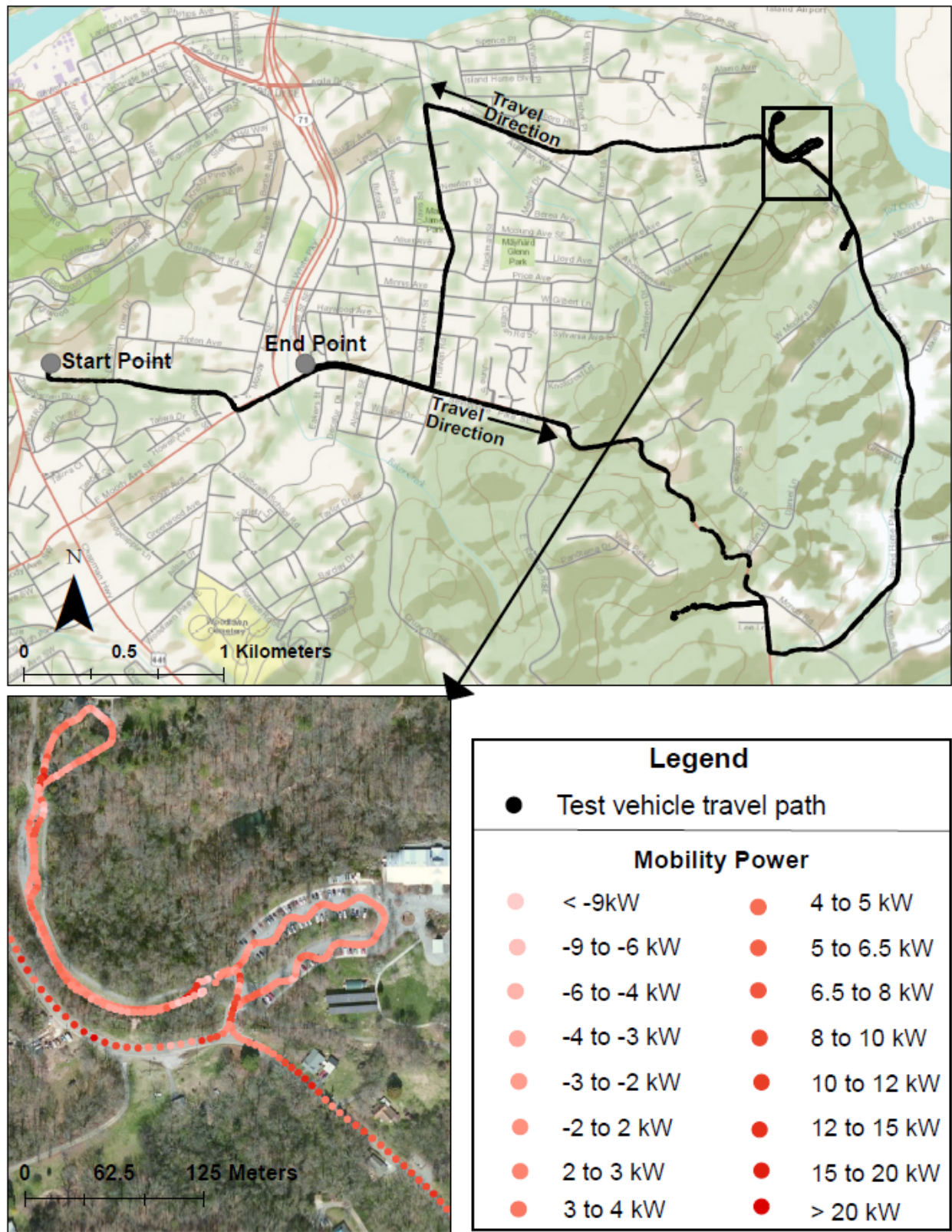
Figure 8: The uncontrolled test travel path along with the discrete predicted mobility power values from the Trimble 132 GPS receiver for a section of the test
