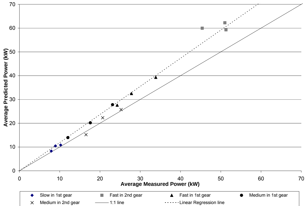
Figure 42: The predicted average mobility power from the Garmin 18 GPS receiver during 15 inertia tests compared to the measured average drivewheel power
