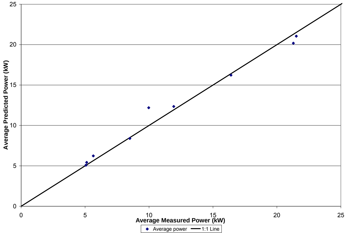
Figure 34: The predicted average mobility power from the Trimble 132 GPS receiver during nine grade tests compared to the measured average drivewheel power
