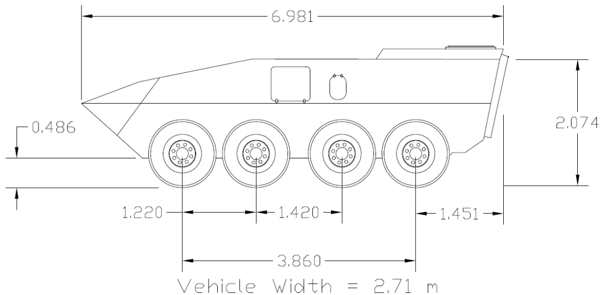
Figure 56: Stryker vehicle geometry (units: meters)
