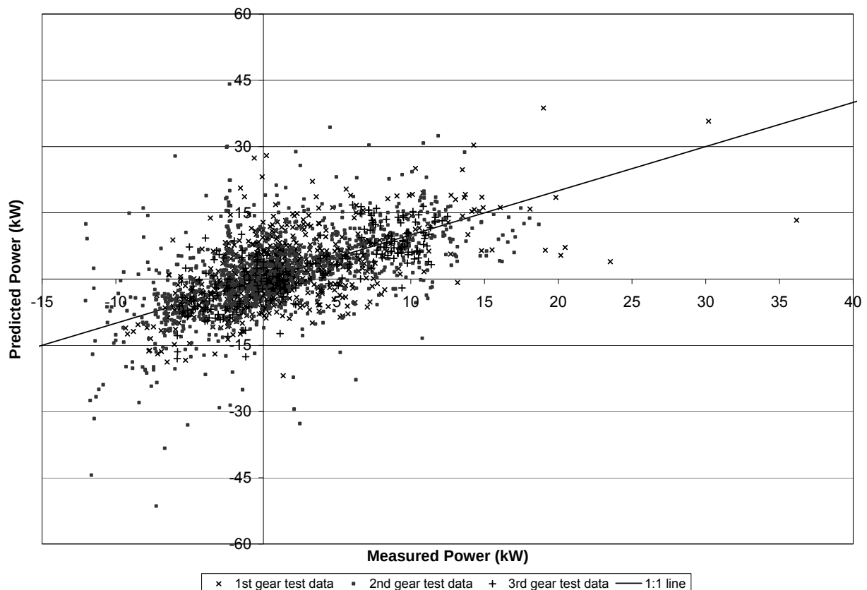
Figure 52: The discrete predicted mobility power values from the Garmin 18 GPS receiver during uncontrolled compared to the measured drivewheel power
