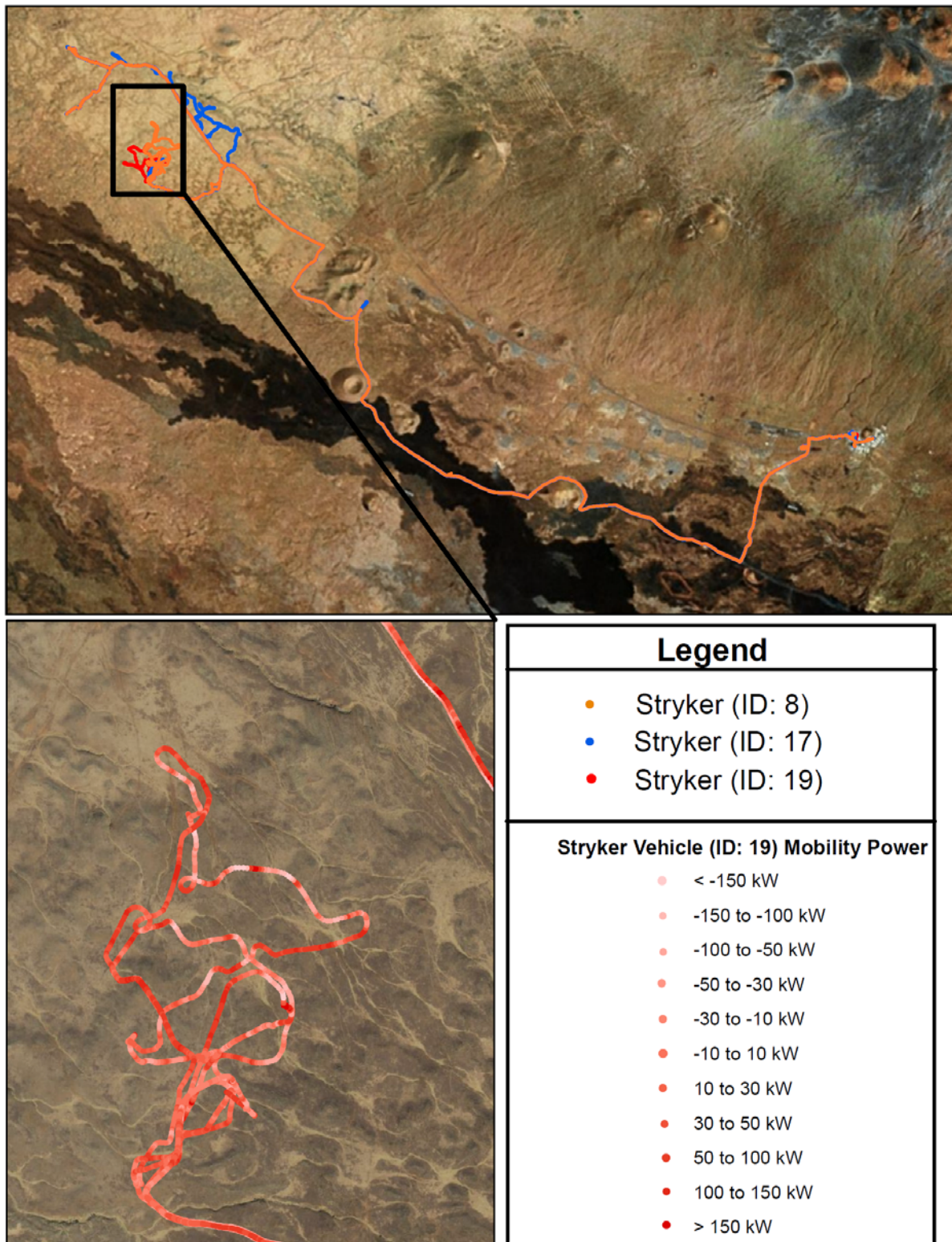
Figure 59: The maneuvers of the three Stryker vehicle at the Pohakuloa Training Area (PTA), Hawaii along with a single vehicle's mobility power requirements during off-road maneuvers at the Keamuku parcel
