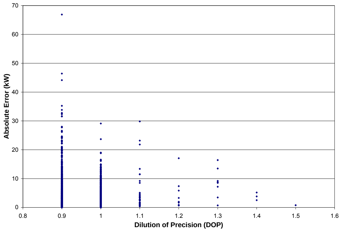
Figure 49: The predicted mobility power absolute error as a function of the Garmin 18 GPS receiver's Dilution of Precision (DOP) values
