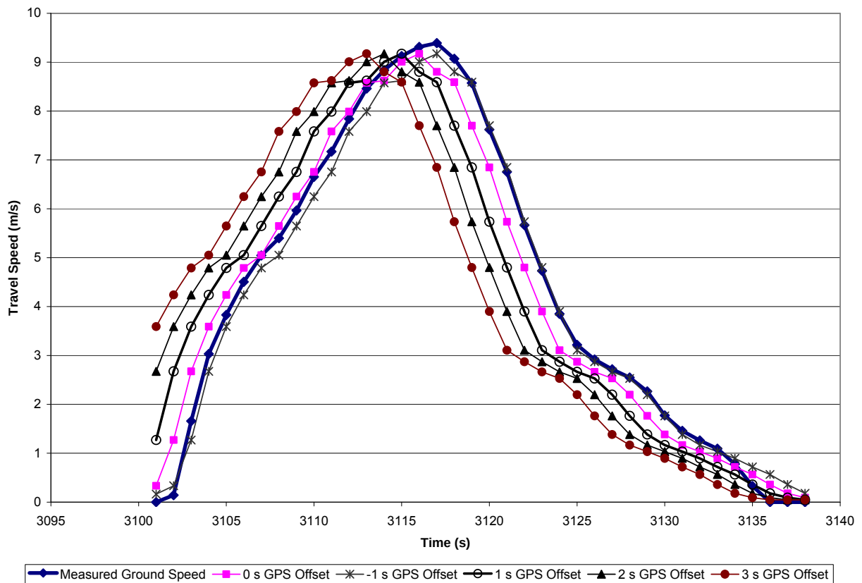
Figure 18: Vehicle travel speed at various Trimble 132 GPS offsets during a slow inertia test
