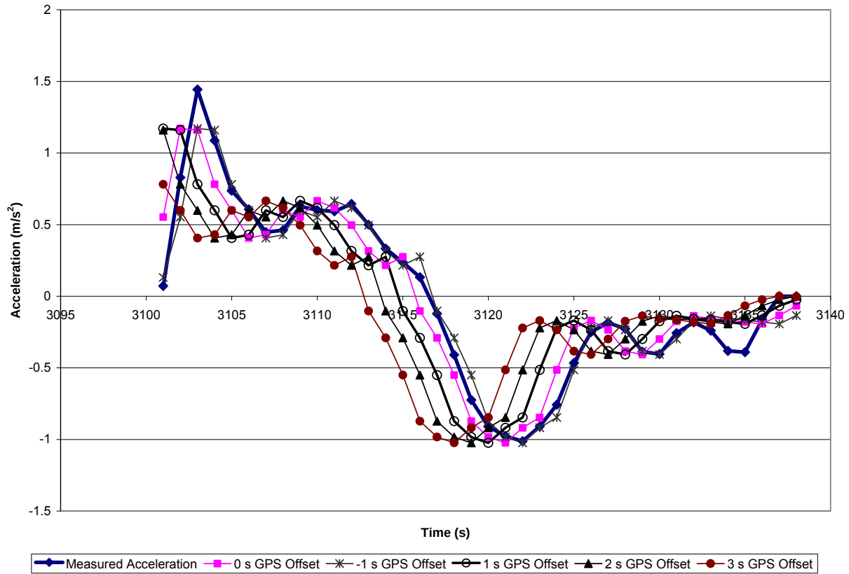
Figure 19: Vehicle acceleration at various Trimble 132 GPS offsets during a slow inertia test
