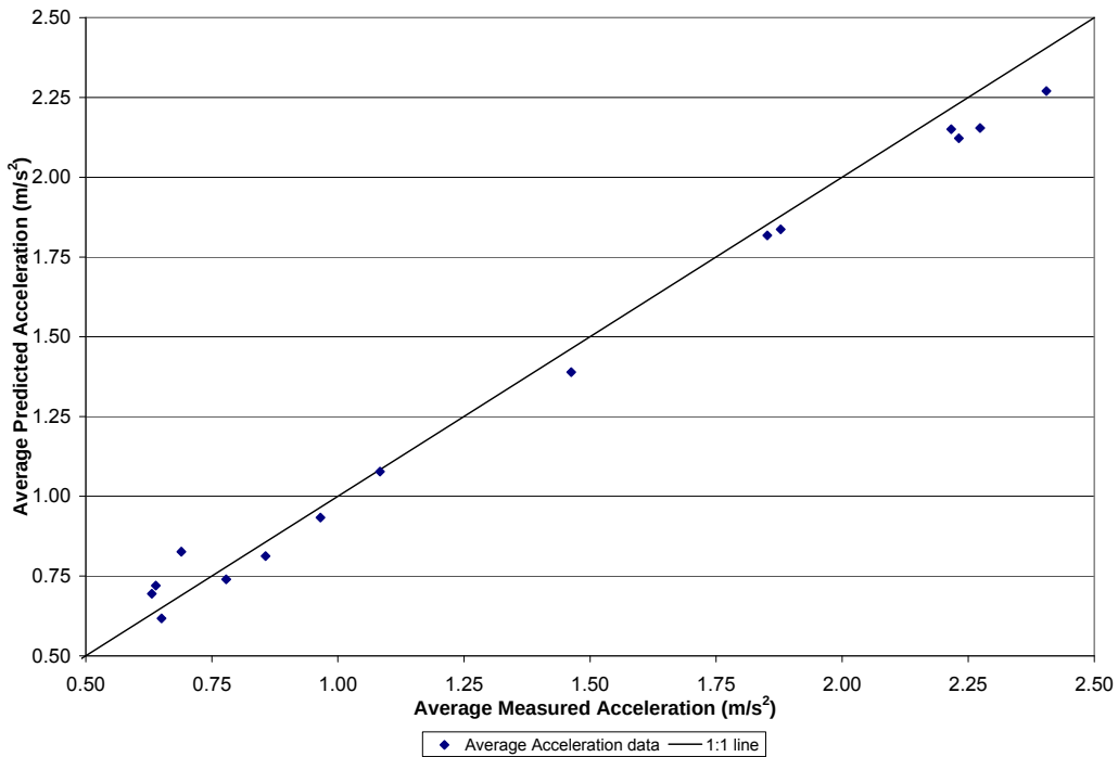
Figure 38: The average predicted vehicle acceleration from the Garmin 18 GPS receiver during 15 inertia tests compared to the measured acceleration
