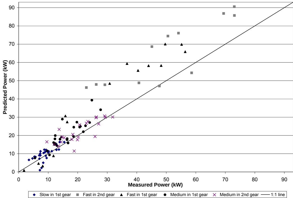
Figure 39: The discrete predicted mobility power values from the Trimble 132 GPS receiver during 15 inertia tests compared to the measured drivewheel power
