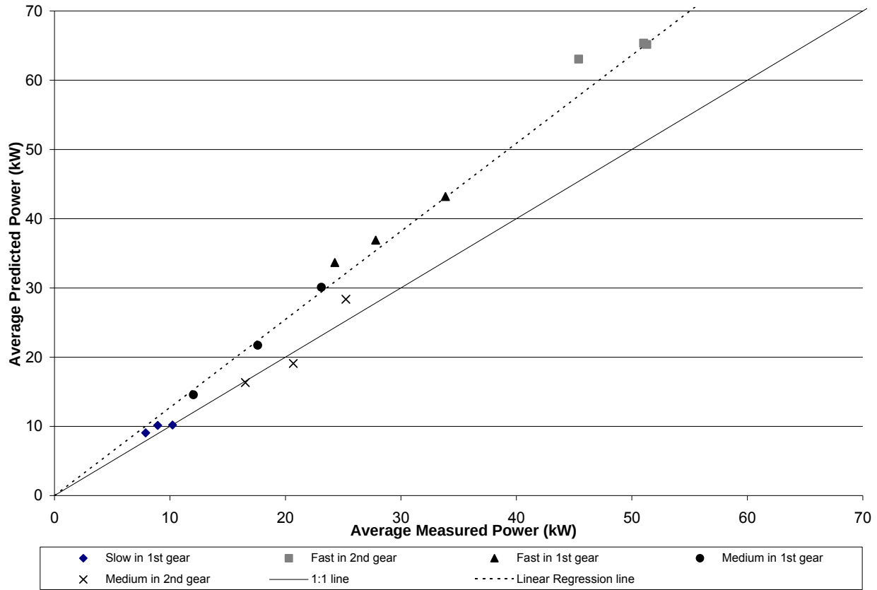
Figure 40: The predicted average mobility power from the Trimble 132 GPS receiver during 15 inertia tests compared to the measured average drivewheel power
