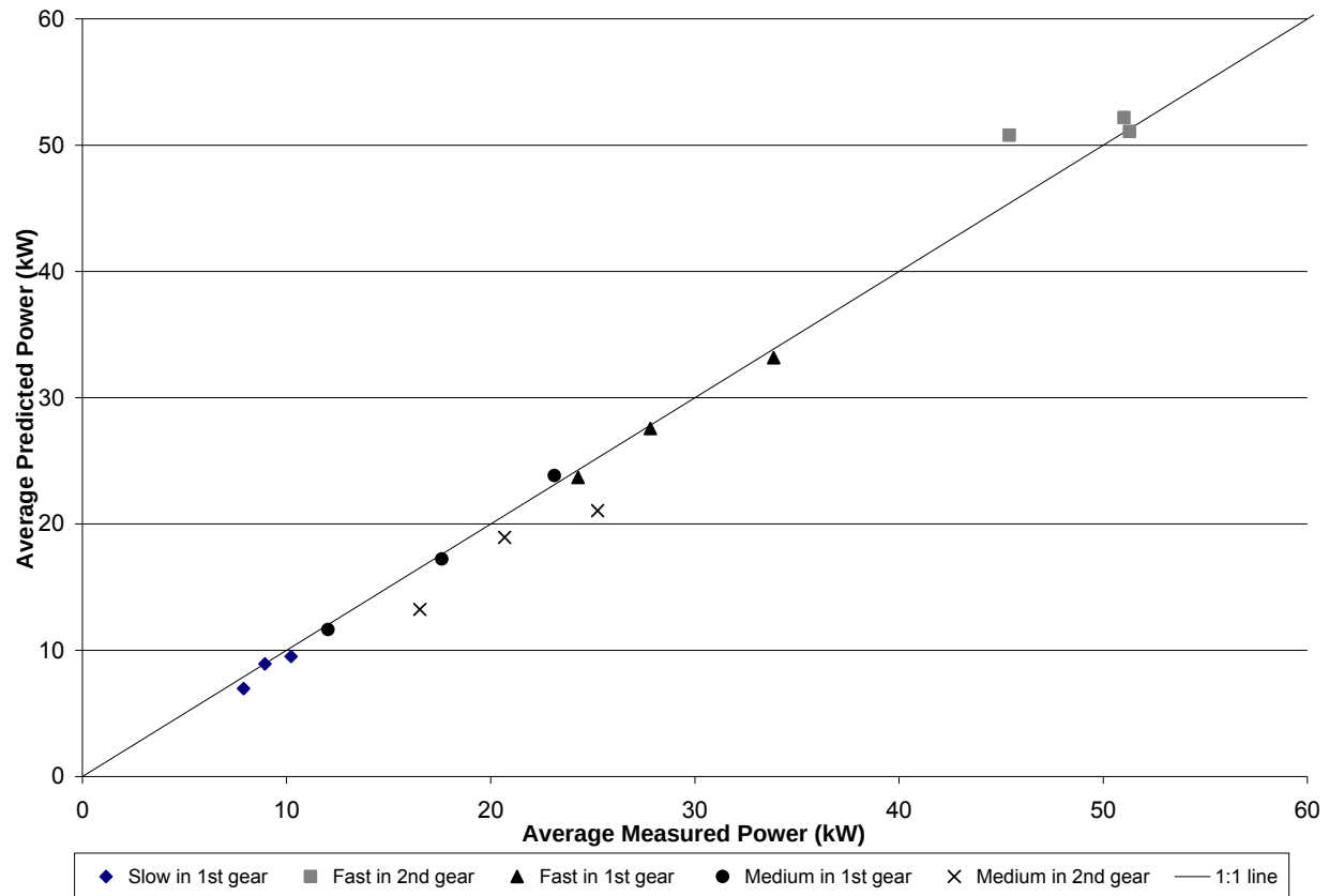
Figure 44: The predicted average mobility power from the Garmin 18 GPS receiver using calibrated drivetrain gamma ( \gamma ) values during 15 inertia tests compared to the measured average drivewheel power
