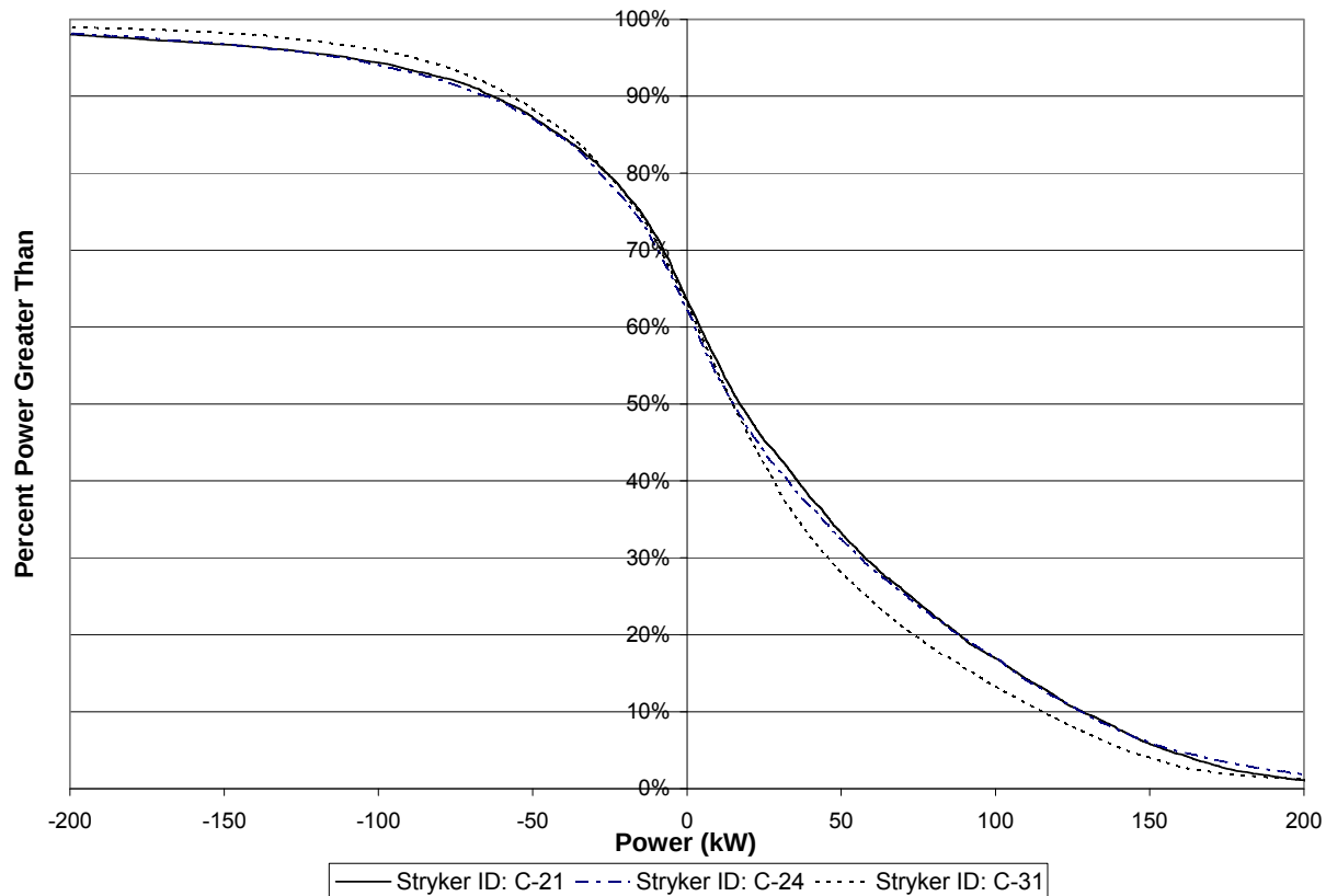
Figure 60: The mobility power duty cycle curves for the three Stryker vehicles performing live-fire, urban operations, and security training missions at Fort Lewis, Washington
