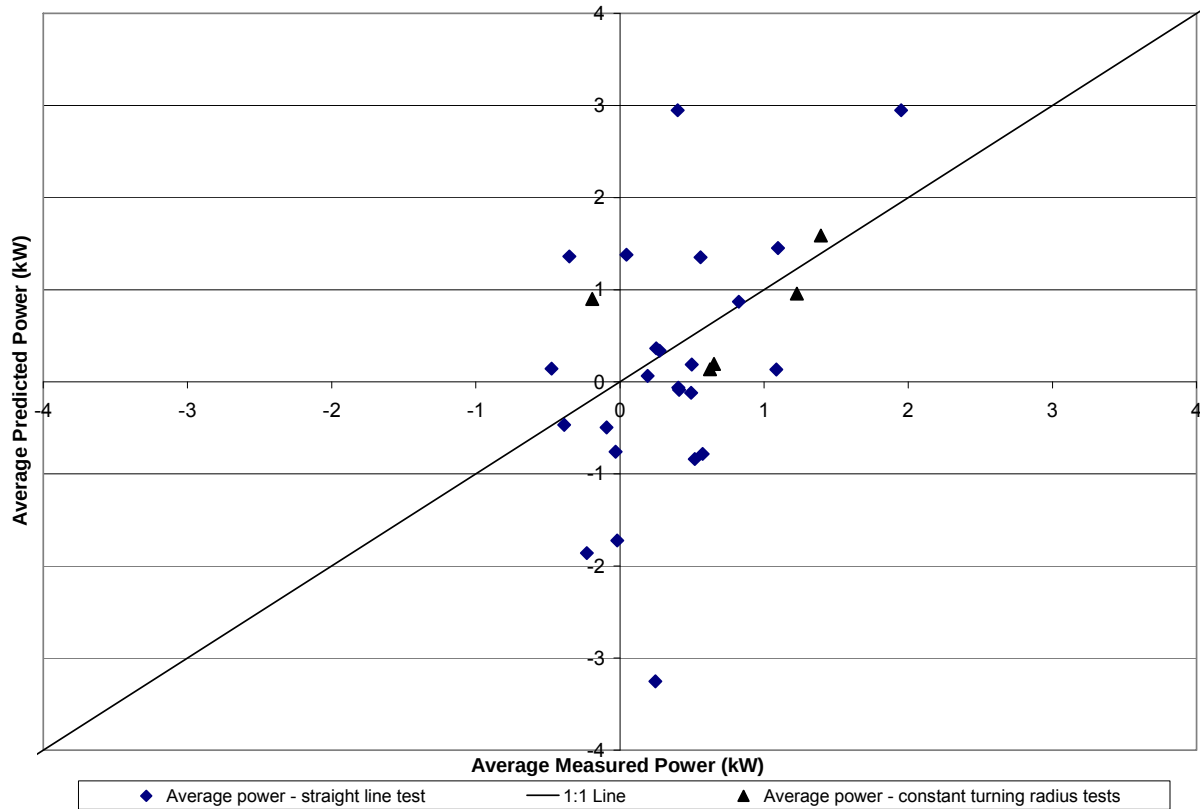
Figure 29: The predicted average mobility power from the Garmin 18 GPS receiver compared to the measured average drivewheel power during the 24 straight-line and five constant turning radius motion resistance tests
