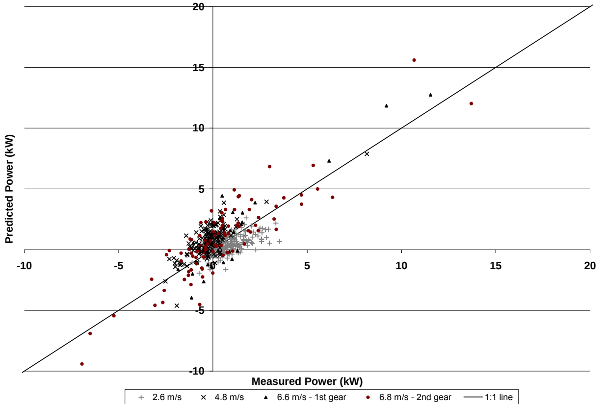
Figure 24: The discrete predicted mobility power values from the Trimble 132 GPS receiver during 20 straight-line motion resistance tests compared to the measured drivewheel power
