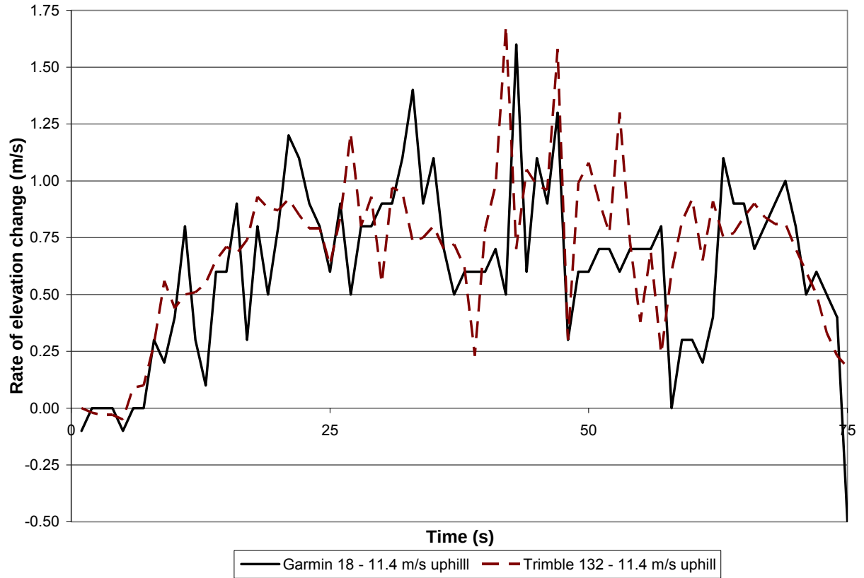
Figure 30: Elevation change estimated from the Garmin 18 and Trimble 132 GPS receivers during a 11.4 m/s uphill grade test
