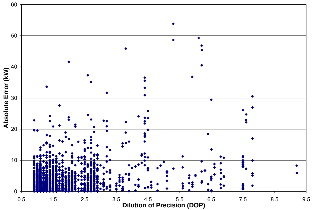
Figure 48: The predicted mobility power absolute error as a function of the Trimble 132 GPS receiver's Dilution of Precision (DOP) values
