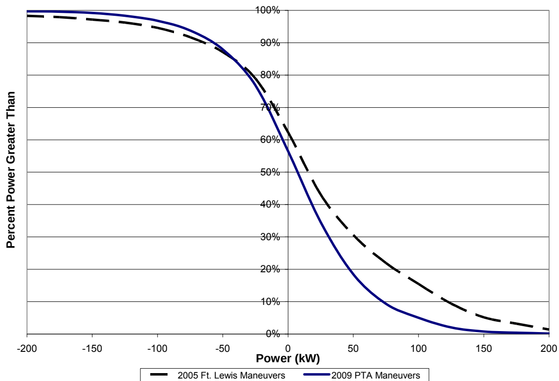
Figure 62: The average mobility power duty cycle curves for the Stryker vehicles operating at Fort Lewis, Washington and the Pohakuloa Training Area, Hawaii
