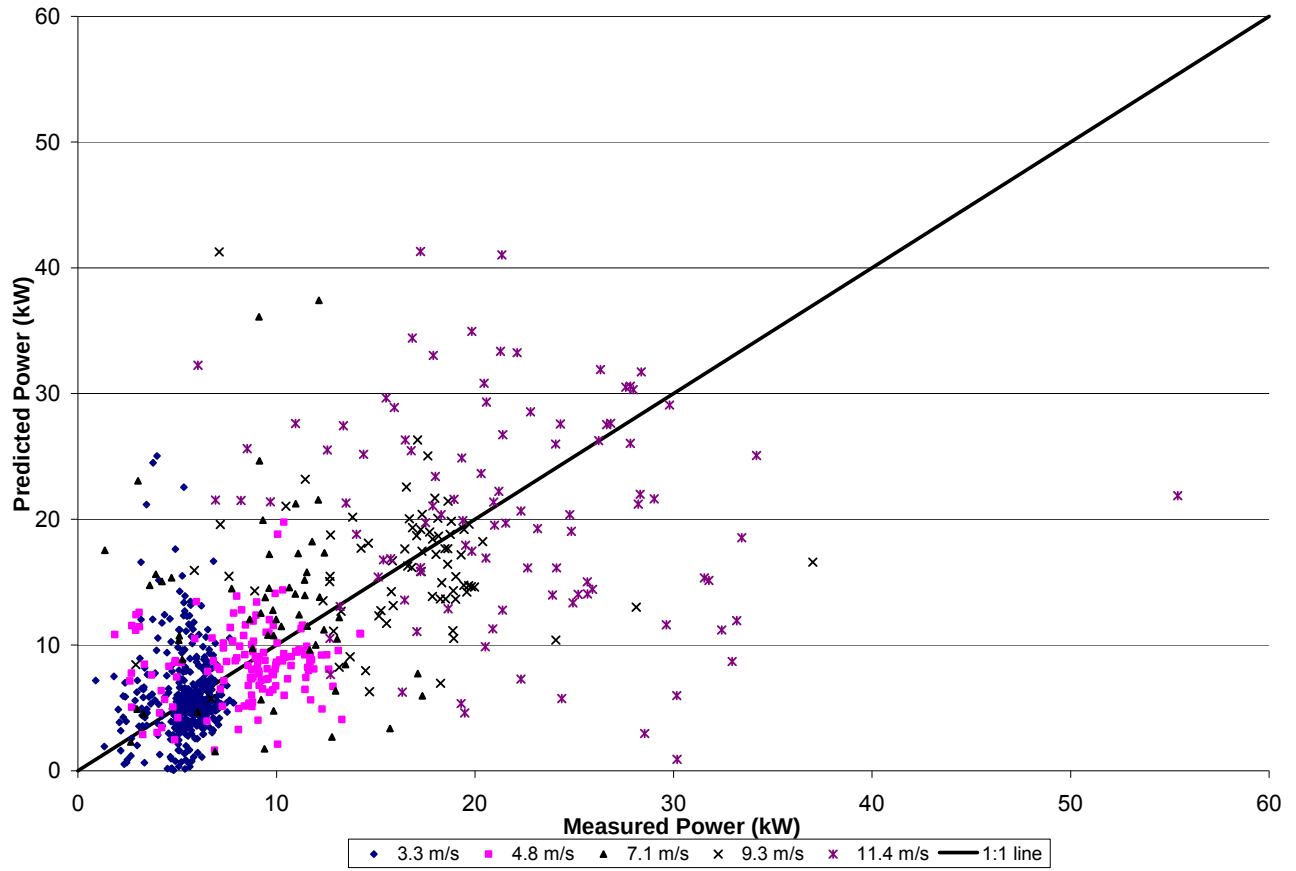
Figure 33: The discrete predicted mobility power values from the Trimble 132 GPS receiver during nine grade tests compared to the measured drivewheel power
