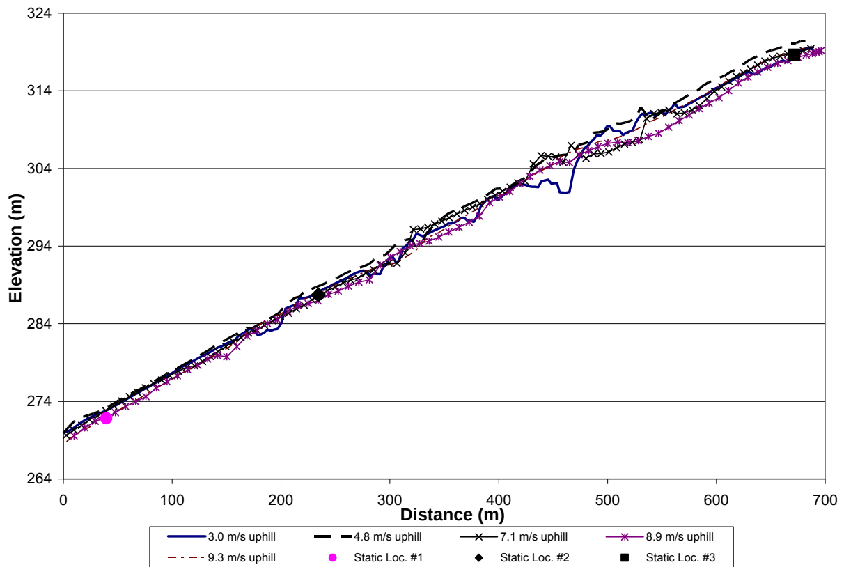
Figure 22: The change in elevation of the test vehicle as a function of distance traveled from the Trimble 132 data during uphill grade tests at different travel speeds
