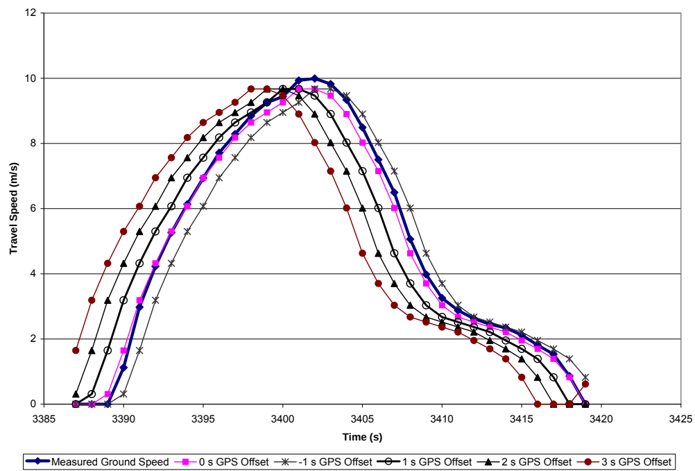
Figure 70: Vehicle travel speed at various Garmin 18 GPS offsets during a medium inertia test
