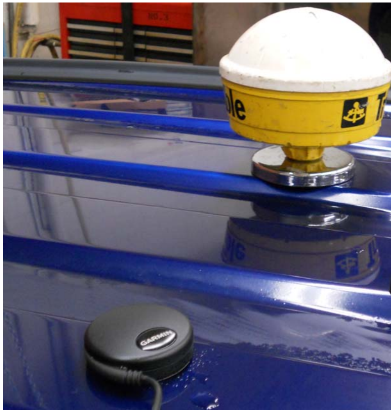
Figure 10: The Garmin 18 and Trimble 132 GPS receivers mounted on the test vehicle
