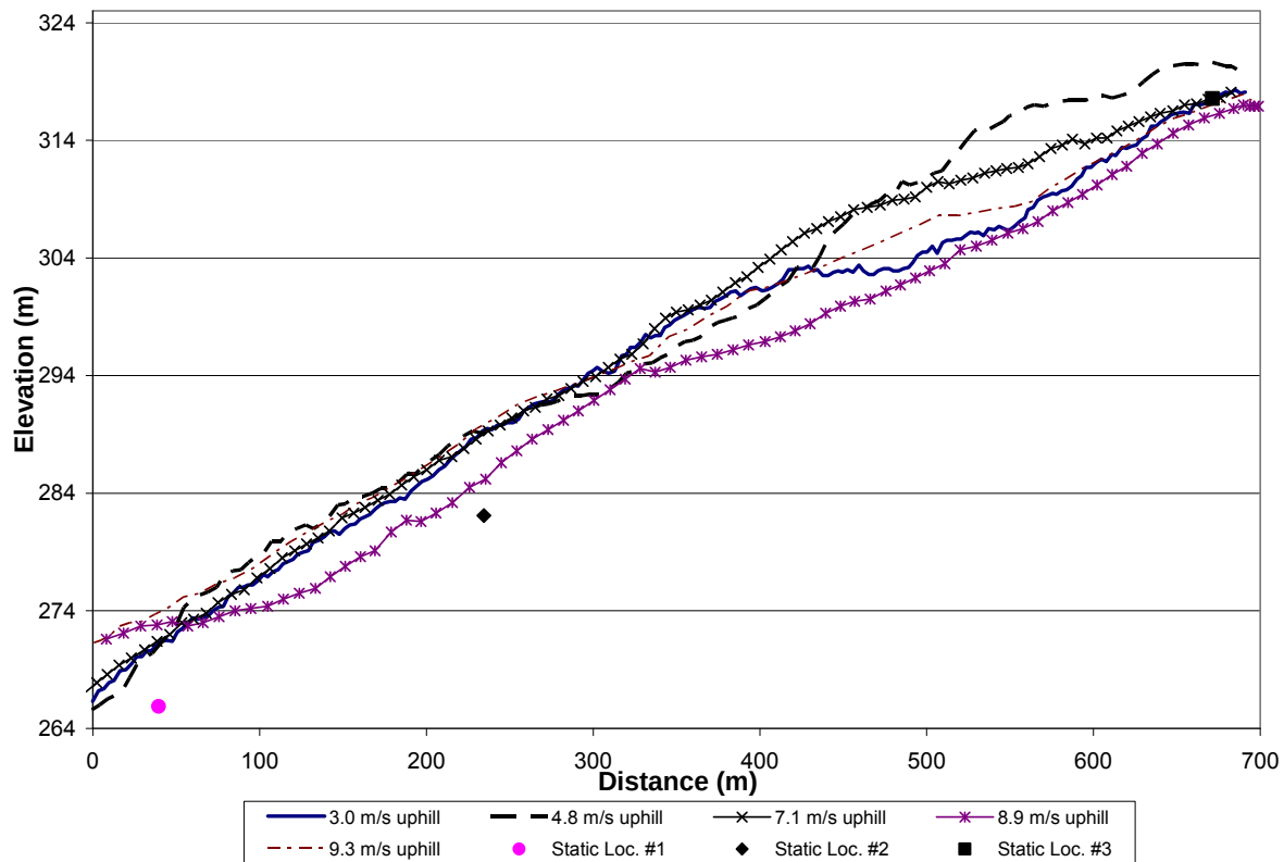
Figure 23: The change in elevation of the test vehicle as a function of distance traveled from the Garmin 18 data during uphill grade tests at different travel speeds
