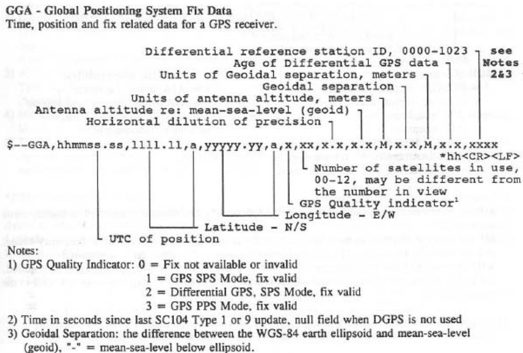
Figure 1: A description of the $GPGGA string (Source: NMEA Standard, 1995)
