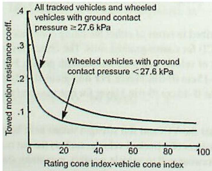
Figure 4: Motion resistance coefficient as a function of the excess soil strength (Source: Wong, 2010)
