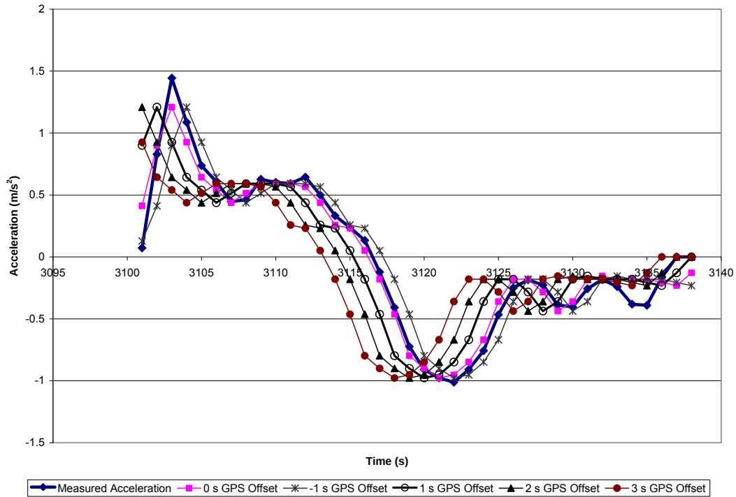
Figure 67: Vehicle acceleration at various Garmin 18 GPS offsets during a slow inertia test
