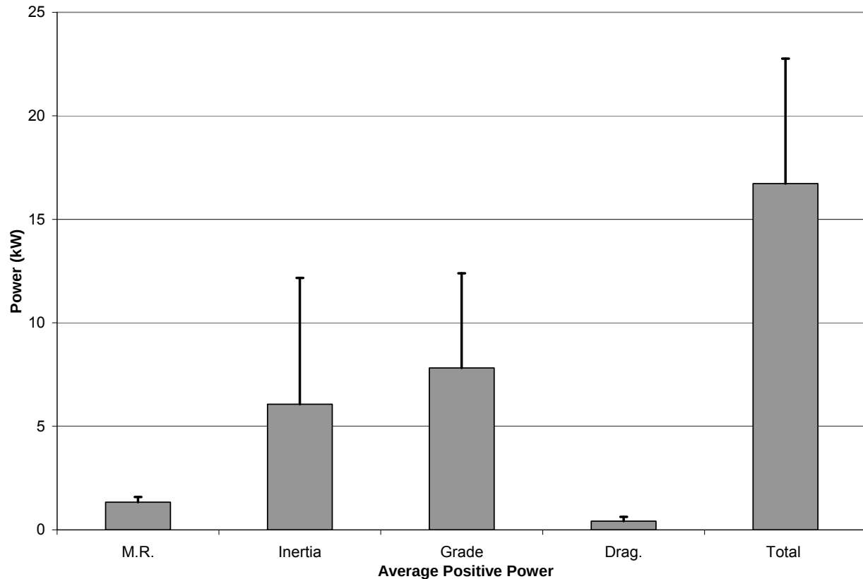
Figure 54: The predicted peak 20% average positive power requirement of the components of the model and the total average positive power with one standard deviation the bars from the Garmin 18 GPS receiver during the uncontrolled test
