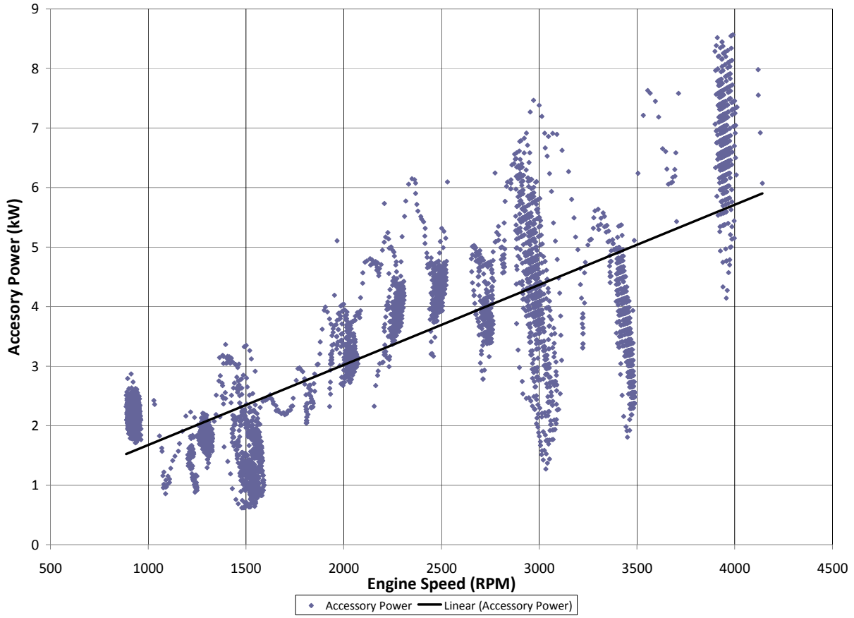
Figure 16: The Fiat engine's accessory power demand data as a function of engine speed and the least-squares linear fit of the accessory power
