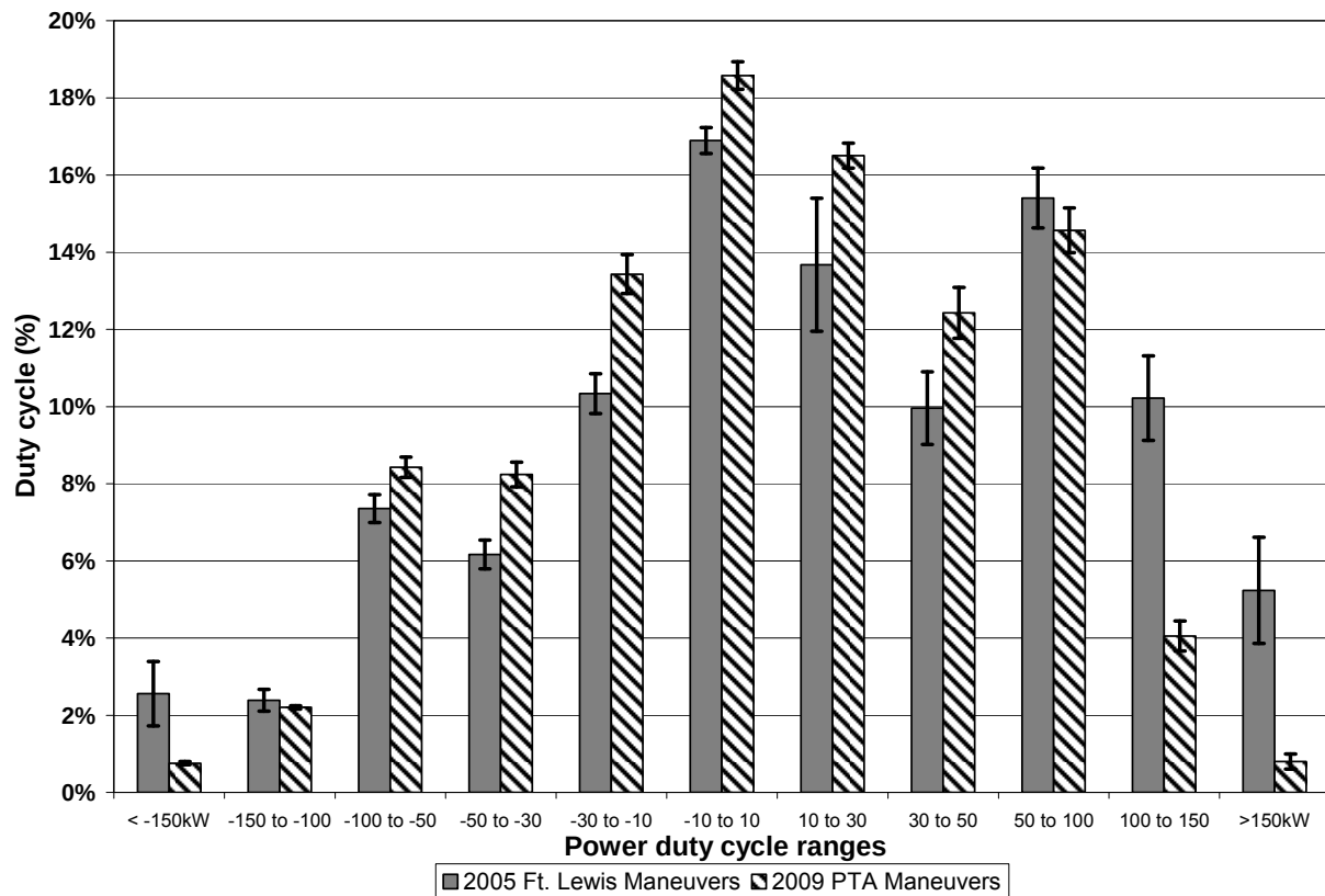
Figure 63: A comparison of the average mobility power duty cycles for three Stryker vehicles operating at Fort Lewis, Washington and the Pohakuloa Training Area, Hawaii along with the associated standard deviation between the vehicles
