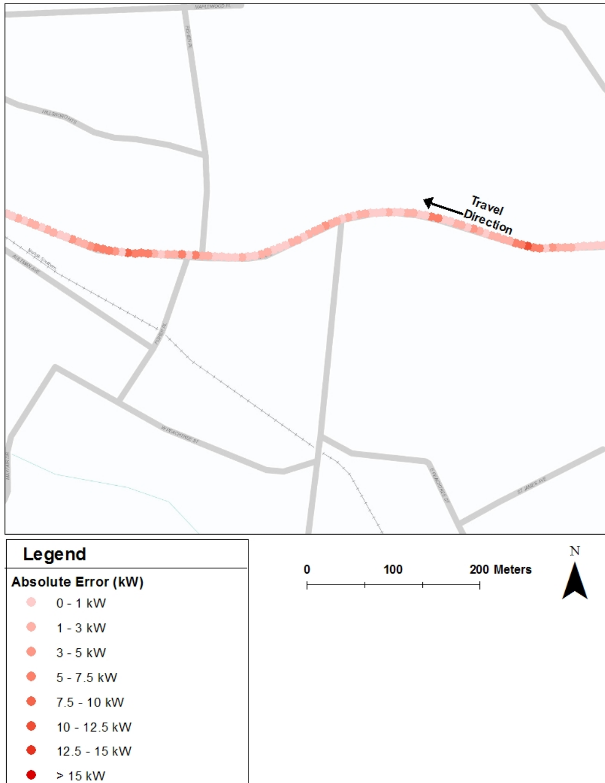
Figure 46: The absolute error of the model's predicted mobility power requirement from the Trimble 132 data compared to the measured drivewheel power during the uncontrolled test
