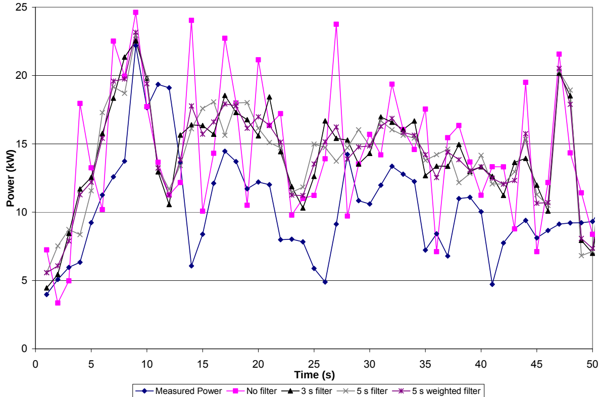
Figure 32: The predicted mobility power using different change in elevation filters Garmin 18 GPS data during a 7.1 m/s travel speed grade test
