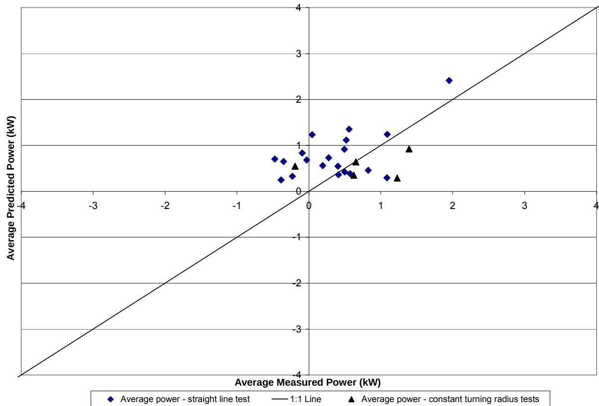
Figure 27: The predicted average mobility power from the Trimble 132 GPS receiver compared to the measured average drivewheel power during the 20 straight-line and five constant turning radius motion resistance tests
