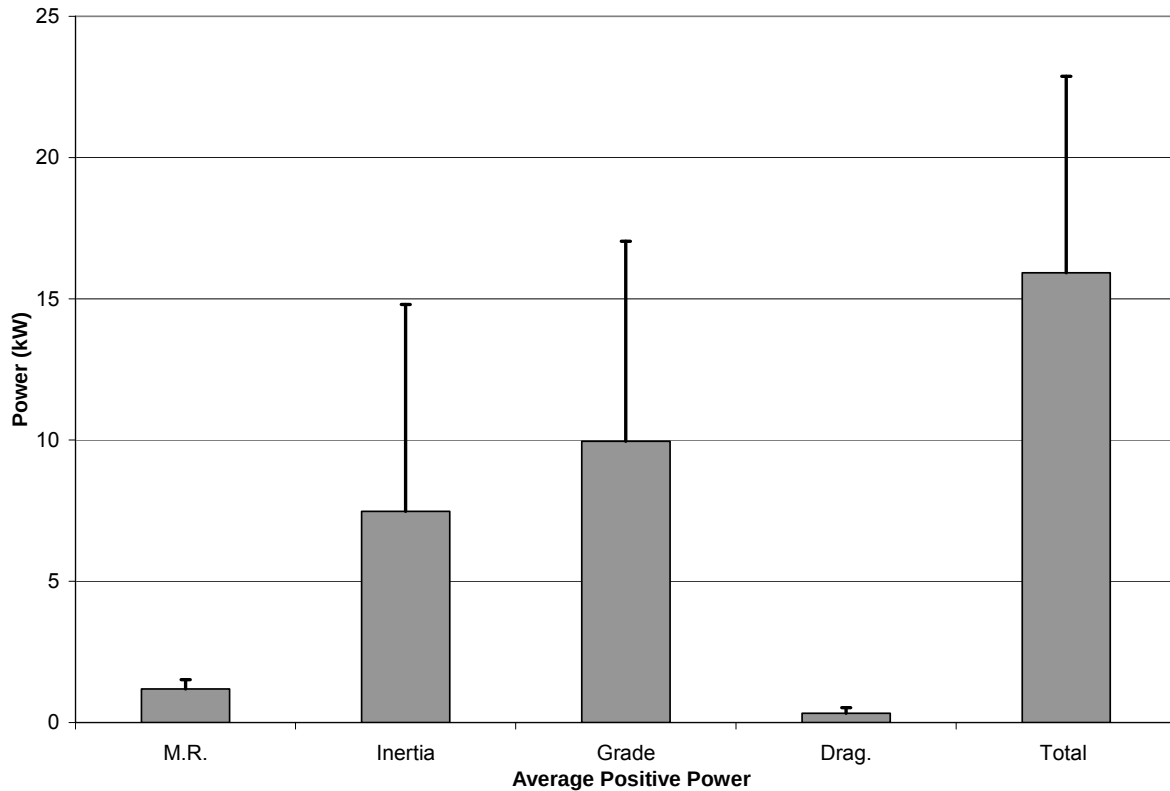
Figure 51 : The predicted peak 20% average positive power requirement of the components of the model and the total average positive power with one standard deviation the bars from the Trimble 132 GPS receiver during the uncontrolled test
