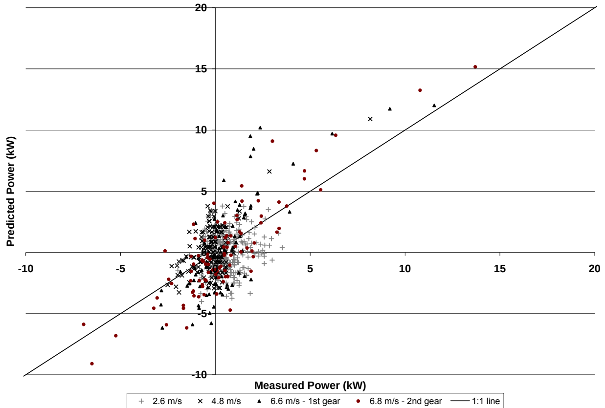
Figure 25: The discrete predicted mobility power values from the Garmin 18 GPS receiver during 24 straight-line motion resistance tests compared to the measured drivewheel power
