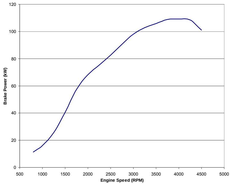
Figure 65: The 1.9L Fiat diesel engine's brake power curve
