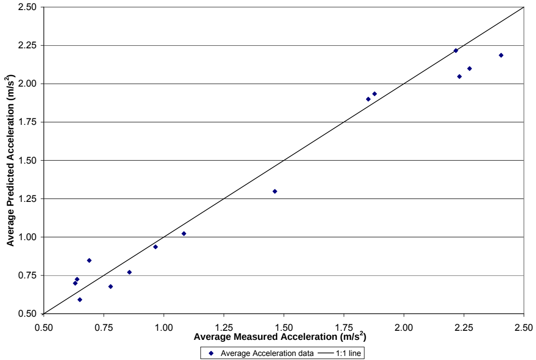
Figure 37: The average predicted vehicle acceleration from the Trimble 132 GPS receiver during 15 inertia tests compared to the measured acceleration
