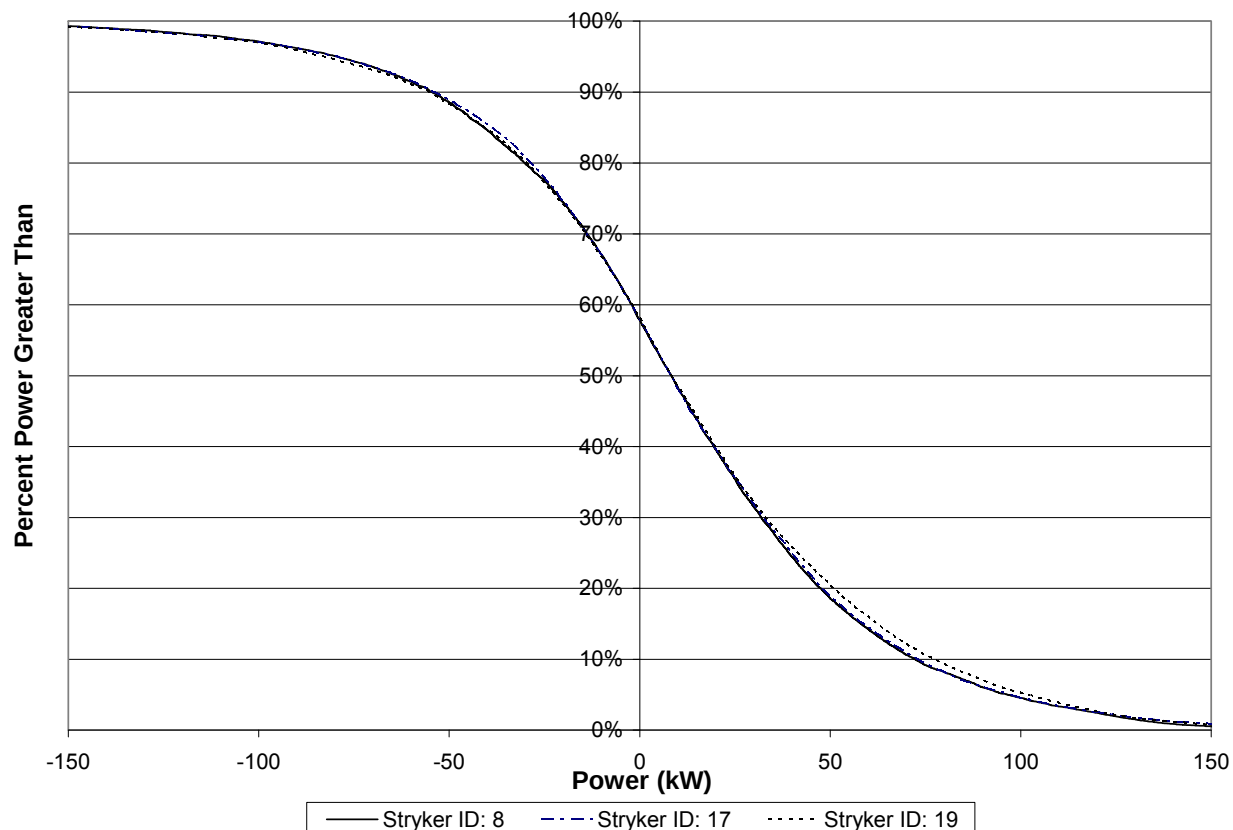
Figure 61: The mobility power duty cycle curves for the three Stryker vehicles performing a proofing mission at the Pohakuloa Training Area, Hawaii
