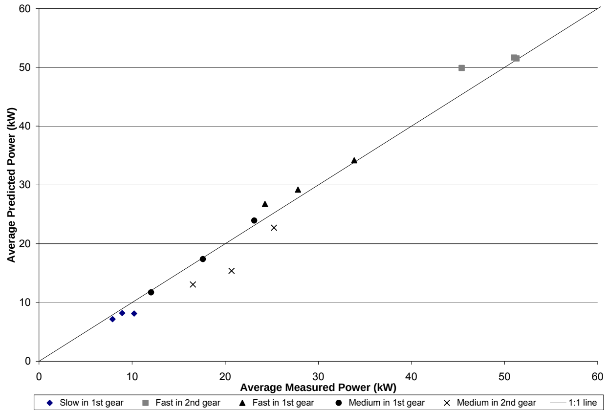
Figure 43: The predicted average mobility power from the Trimble 132 GPS receiver using calibrated drivetrain gamma ( \gamma ) values during 15 inertia tests compared to the measured average drivewheel power
