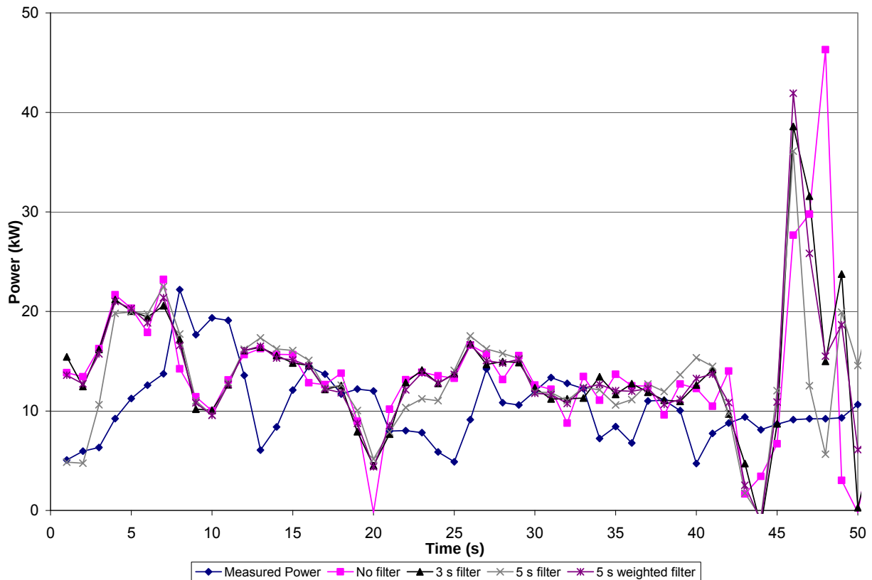
Figure 31: The predicted mobility power using different change in elevation filters Trimble 132 GPS data during a 7.1 m/s travel speed grade test
