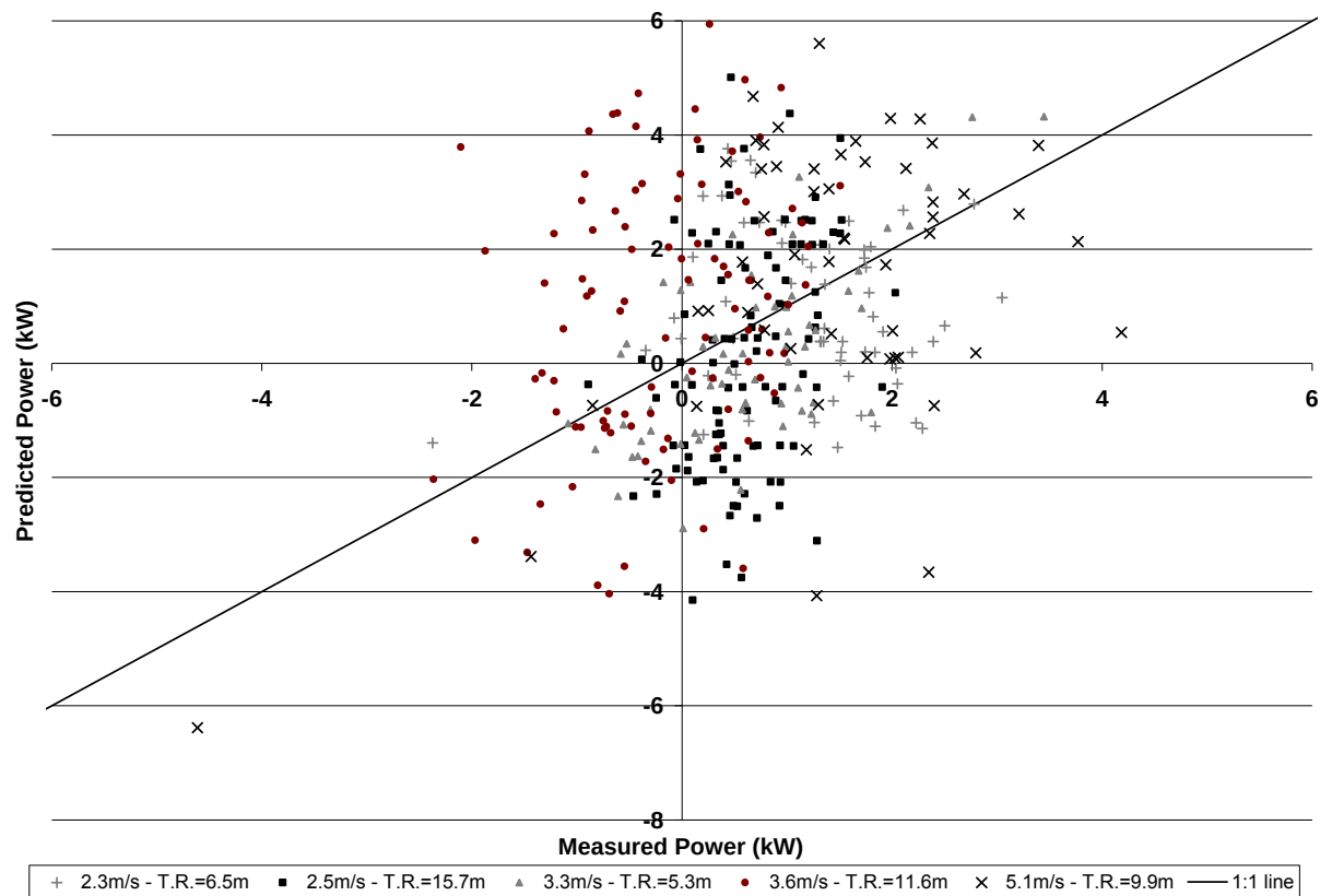
Figure 28: The discrete predicted mobility power values from the Garmin 18 GPS receiver during five constant turning radius motion resistance tests compared to the measured drivewheel power
