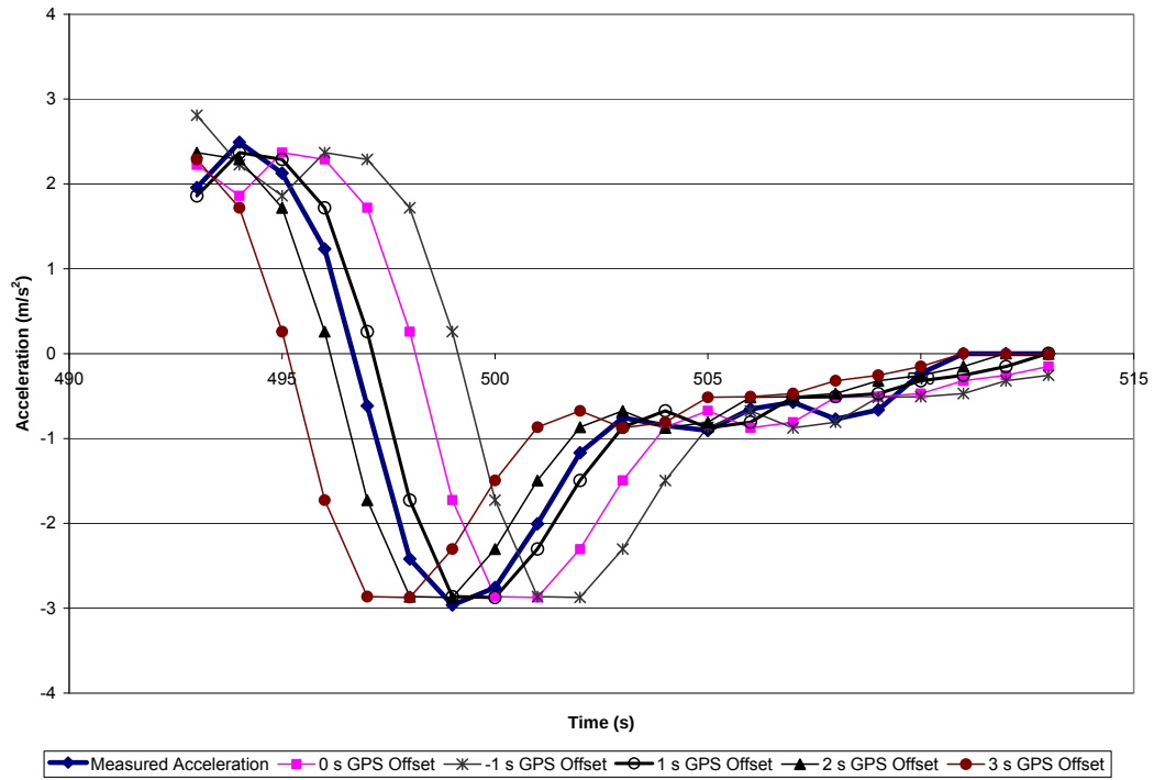
Figure 73: Vehicle acceleration at various Trimble 132 GPS offsets during a fast inertia test
