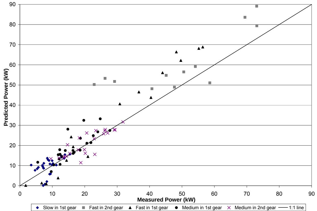
Figure 41: The discrete predicted mobility power values from the Garmin 18 GPS receiver during 15 inertia tests compared to the measured drivewheel power
