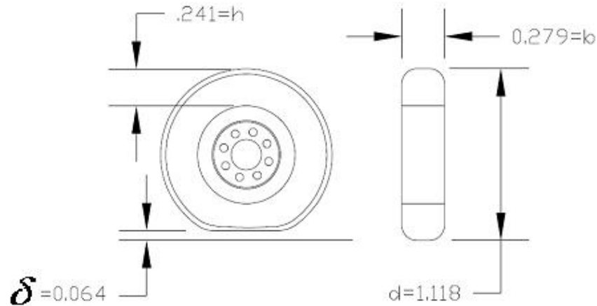
Figure 57: The geometry of the Michelin X tire on the Stryker vehicle (units: meters)
