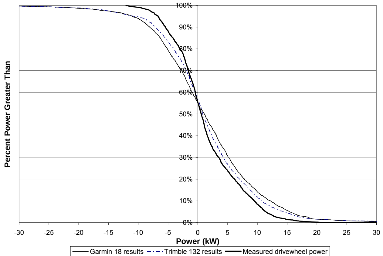
Figure 55: The predicted mobility power duty cycle curves from the Trimble 132 and Garmin 18 GPS data compared to the measured drivewheel power duty cycle during the uncontrolled test
