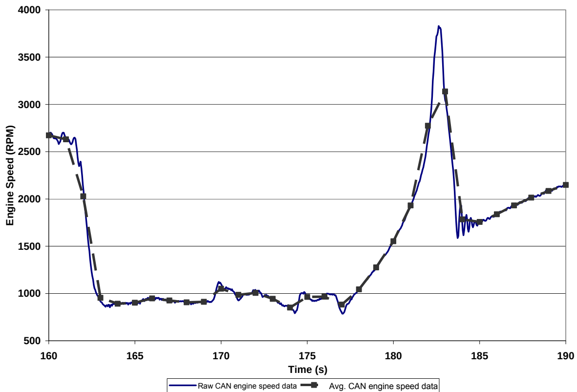
Figure 14: Raw 25 Hz CAN engine speed data and the averaged 1 Hz engine speed data
