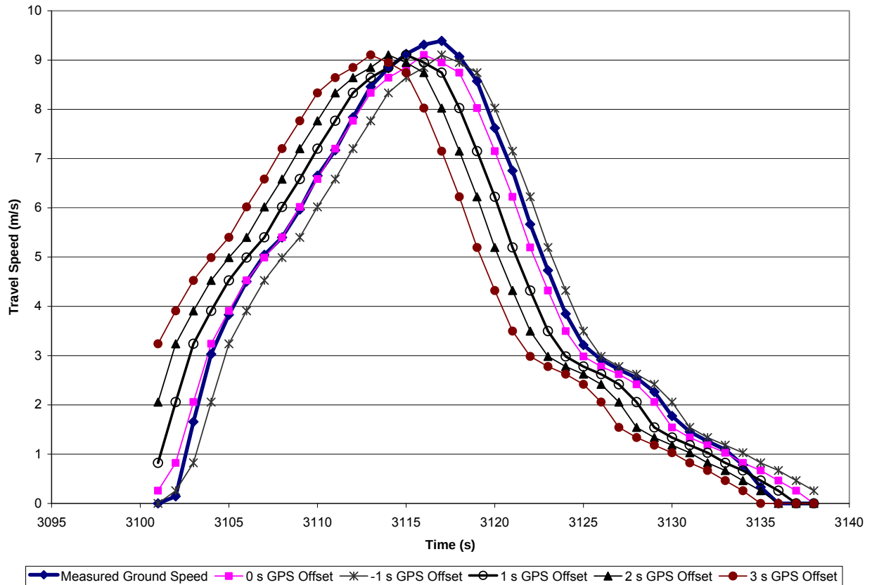
Figure 66: Vehicle travel speed at various Garmin 18 GPS offsets during a slow inertia test
