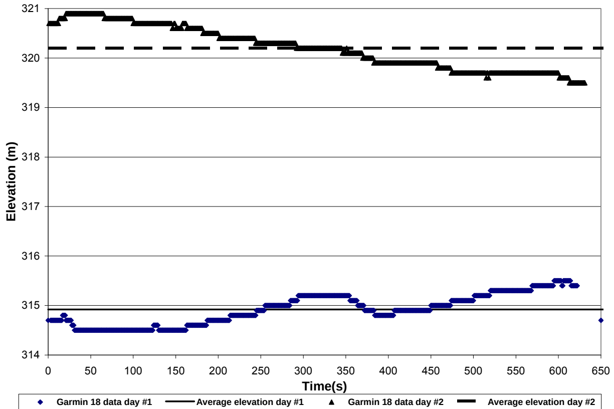
Figure 21: Static Garmin 18 elevation data during two different days at the grade test location
