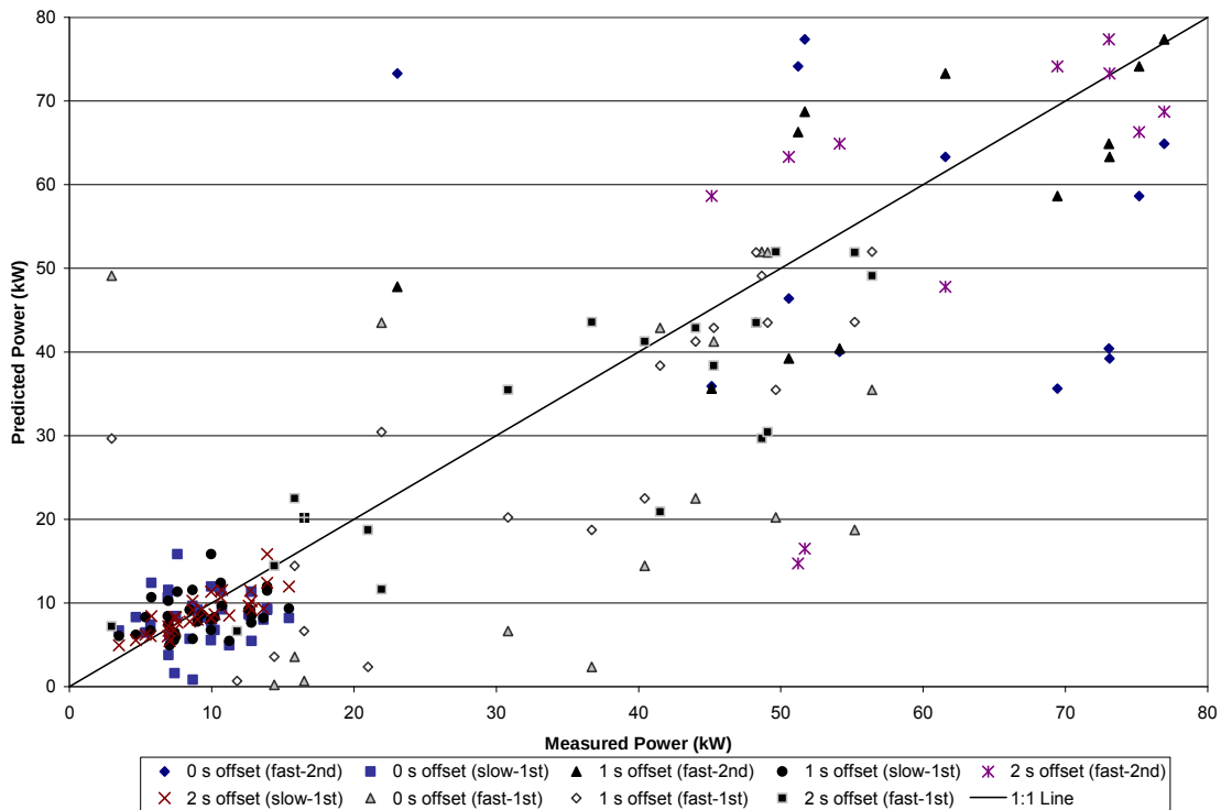
Figure 77: A comparison of predicted and measured mobility power at various GPS speed and acceleration offsets during nine inertia tests for the Garmin 18 GPS receiver
