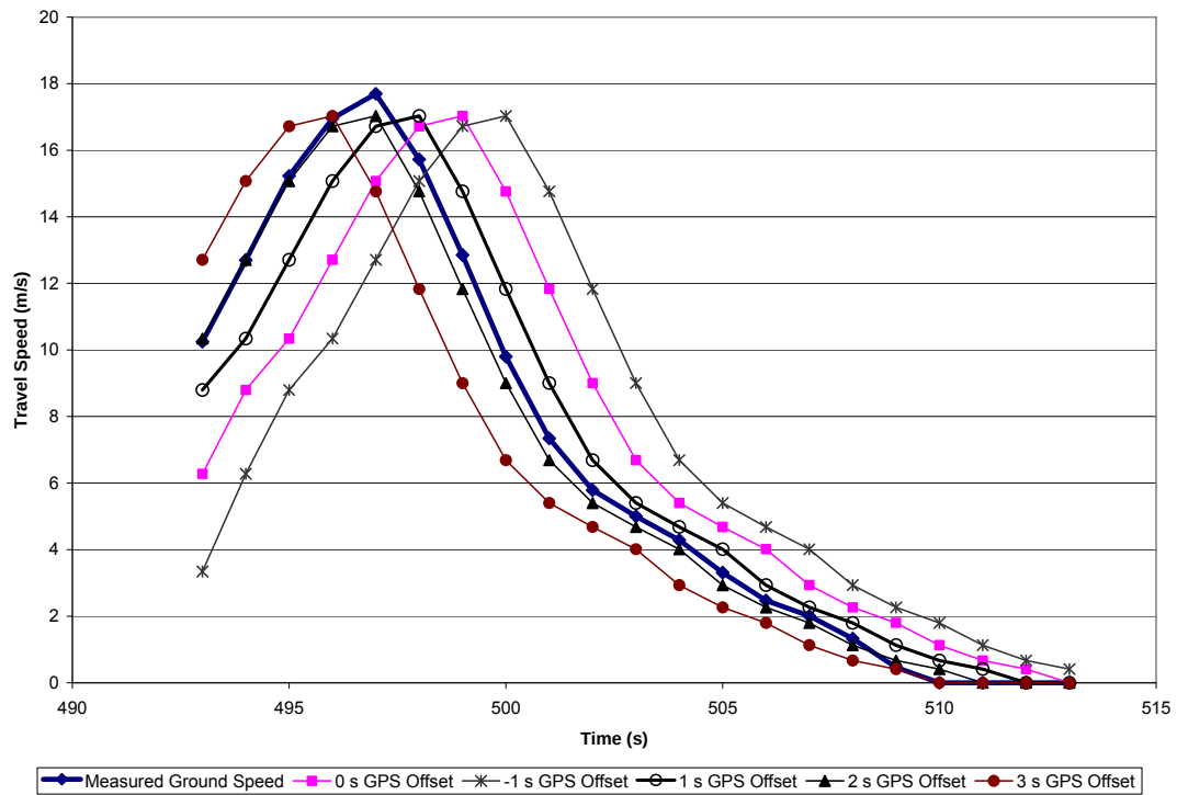
Figure 74: Vehicle travel speed at various Garmin 18 GPS offsets during a fast inertia test
