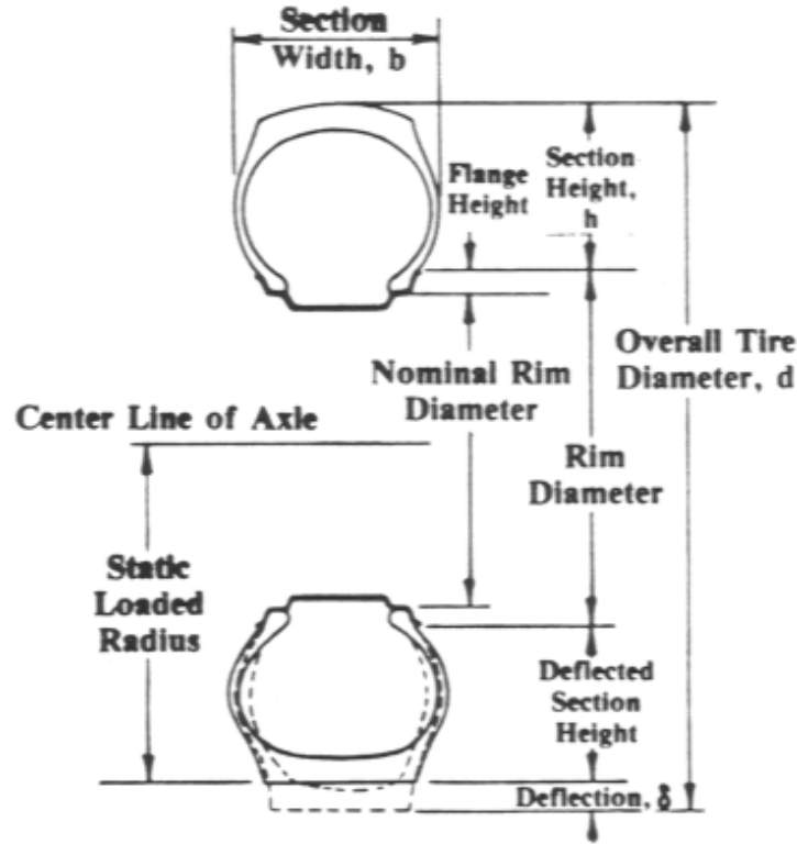
Figure 3: Tire parameters used to calculate dimensionless wheel numeric (Source: Brixius, 1987)
