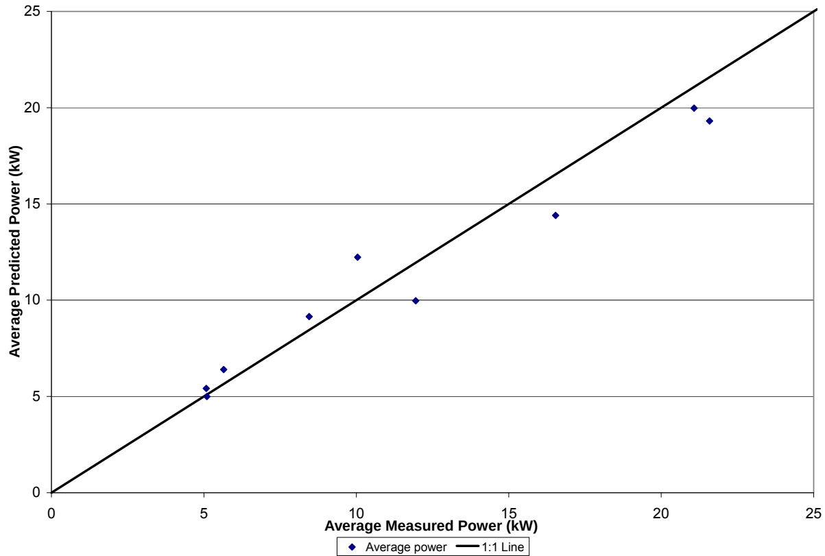
Figure 36: The predicted average mobility power from the Garmin 18 GPS receiver during nine grade tests compared to the measured average drivewheel power
