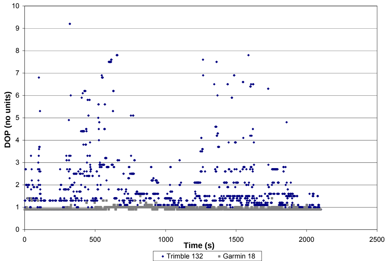
Figure 47: The Dilution of Precision (DOP) from the Trimble 132 and Garmin 18 GPS receivers during the uncontrolled test
