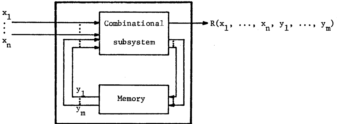
Figure 6.2. The conventional model of a sequential system.
