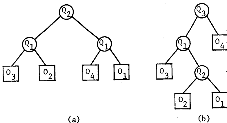
Figure 2.6. The two identification procedures of Example 2.14.
