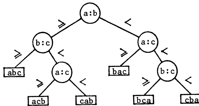
Figure 1.1. A decision tree for sorting three elements.
