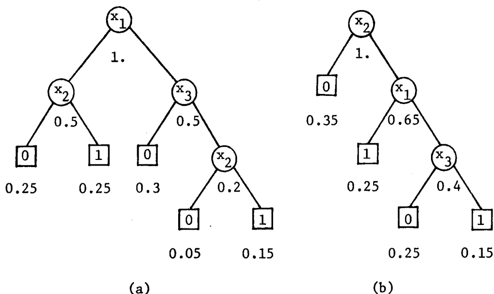
Figure 2.4. The two decision trees of Figure 2.1 with their node probabilities.
