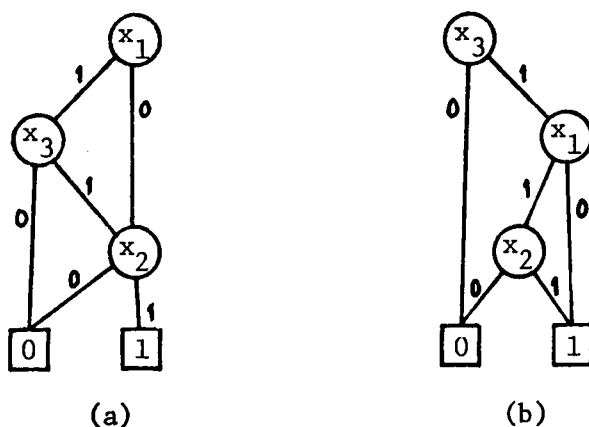
Figure 2.3. The two free Boolean graphs of Example 2.8.
