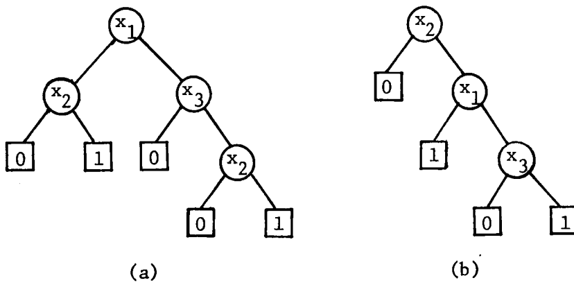
Figure 2.1. Two decision trees for the function of Example 2.6.
