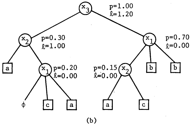
Figure 5.1. The two trees for Example 5.2 with the probability ( p ) and loss ( \ell ) at each internal node.
