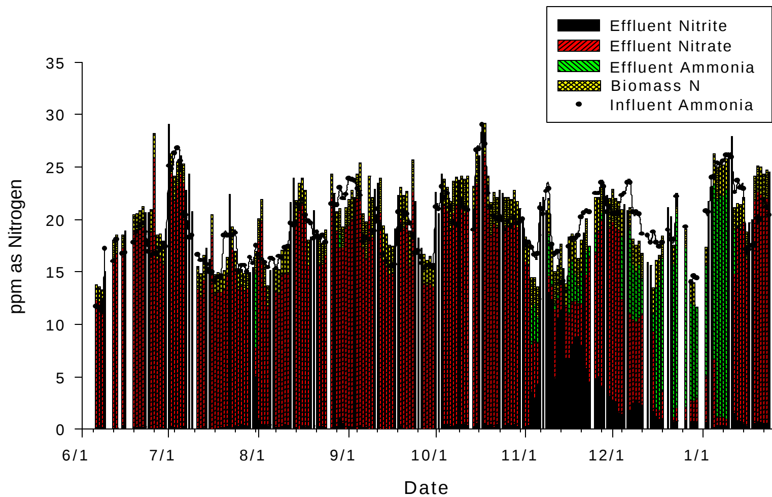
Figure 15 A balance of influent ammonia, effluent ammonia, effluent nitrite, effluent nitrate, and reactor biomass nitrogen used to confirm the occurrence of complete nitrification in the 5 day BSRT reactor.
