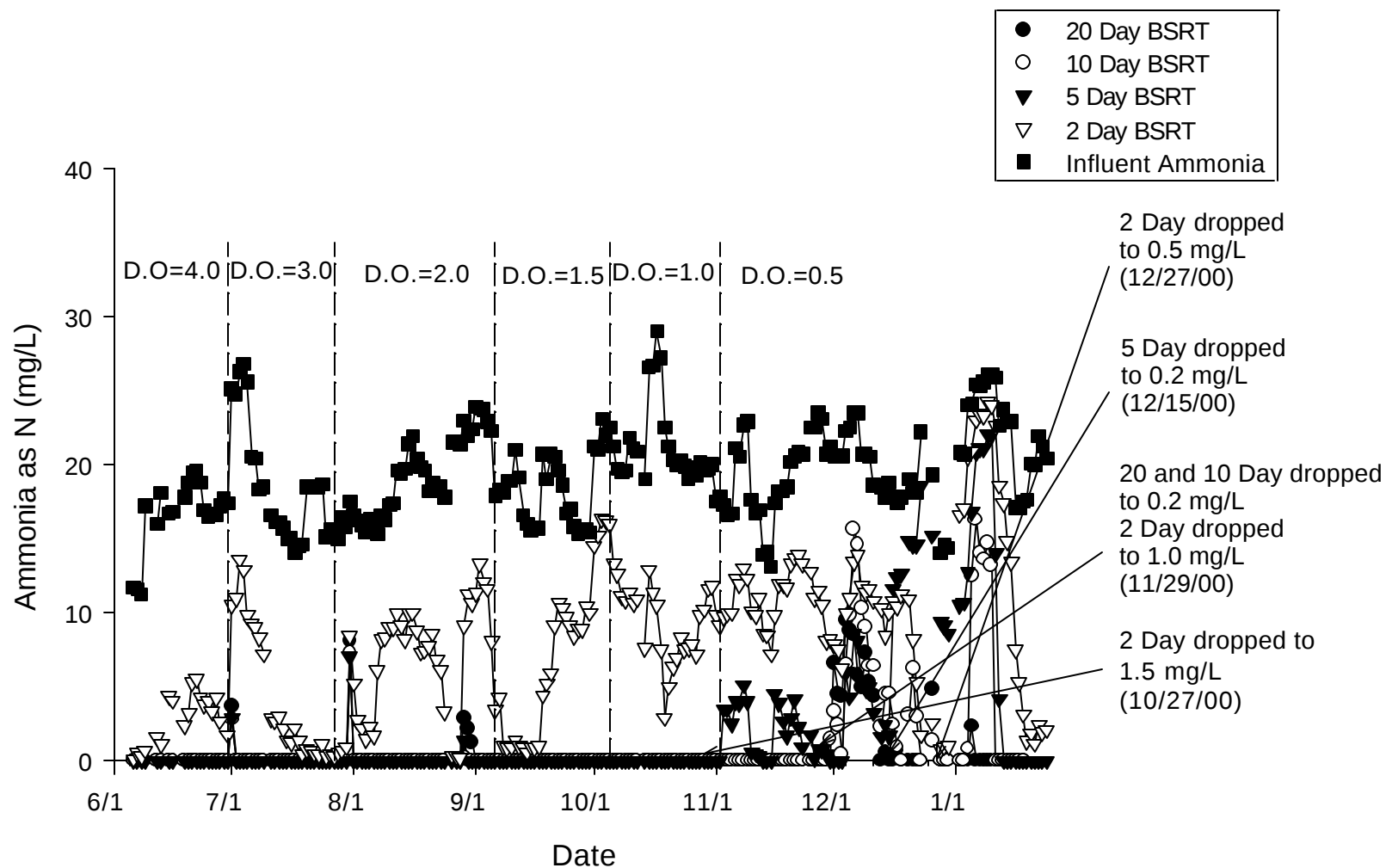
Figure 12 Ammonia removal as a function of DO concentration over the course of the treatability study.
