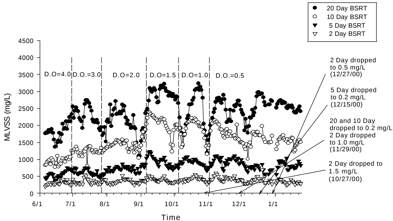
Figure 8 Fluctuations in MLVSS concentration due to changing influent COD concentrations during the treatability study.
