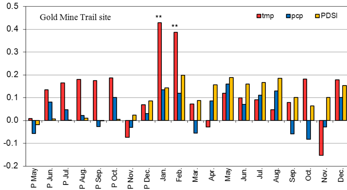
Figure 29. Correlations between the Gold Mine Trail chronology and monthly temperature (tmp), precipitation (pcp), and PDSI from previous May to current December (1895–2006) (*: P<0.05 ; **: P<0.01 ).
