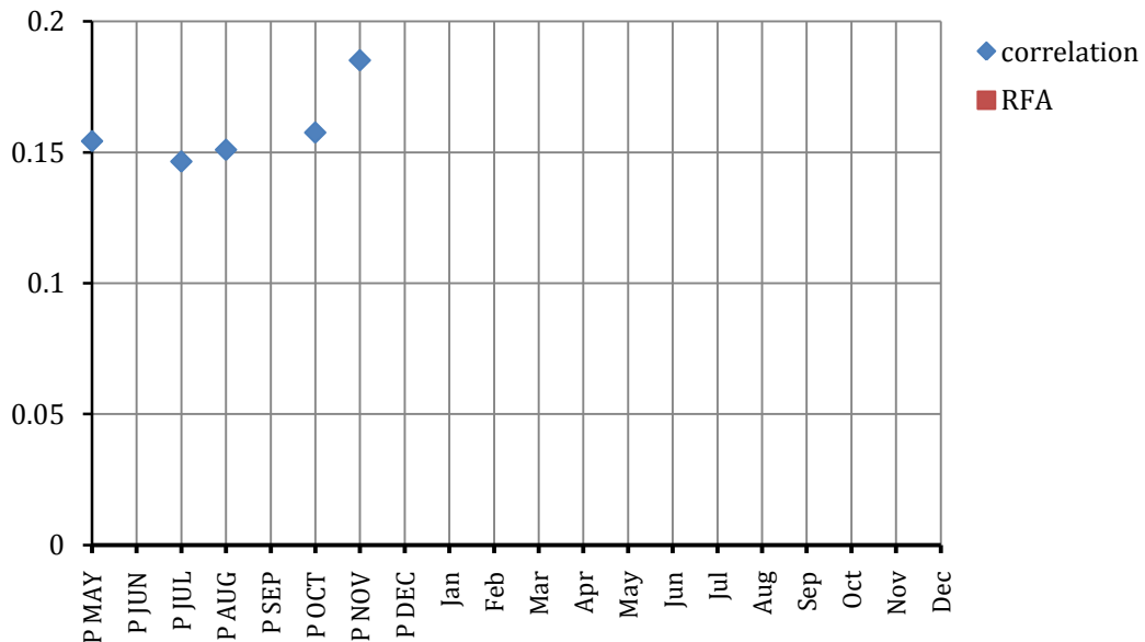
Figure 40. Correlation and response function significant coefficients between the composite chronology and monthly AMO index from the previous May to the current December (1856-2003). Coefficients with significant level higher than 5% are marked using colors, and all non-significant coefficients are marked equal to zero.
