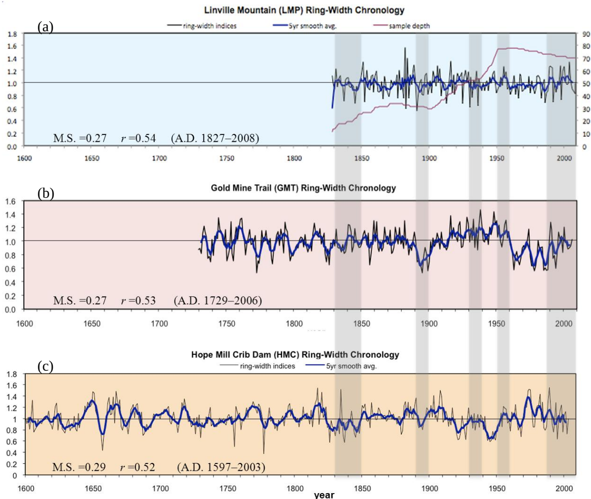
Figure 7(a). Standard chronology of the Linville Mountain site, and sample depth is indicated in red line; Figure 7(b). Standard chronology of the Gold Mine Trail site; Figure 7(c). Standard chronology of the Hope Mills site. Note: The highlighted columns are the periods (1830s–1840s, 1890s, 1930s, 1950s, post-1990s) with extreme climatic events. The horizontal line cross the chronologies is the average ring width index value of 1.0.
