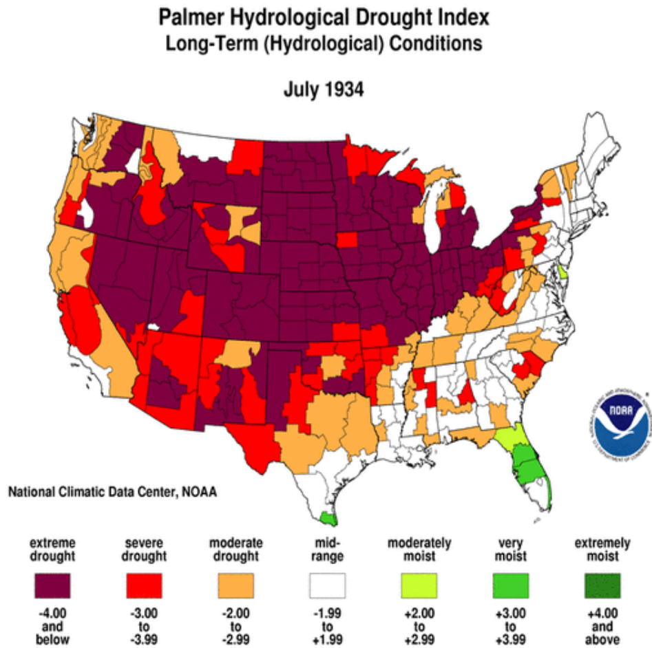
Figure 43. The Palmer Hydrological Drought Index map of 1934. As the most severe year during the Dust Bowl of 1930s, this map shows the areas with different levels of drought across the U.S. (from National Climatic Data Center, NOAA)
