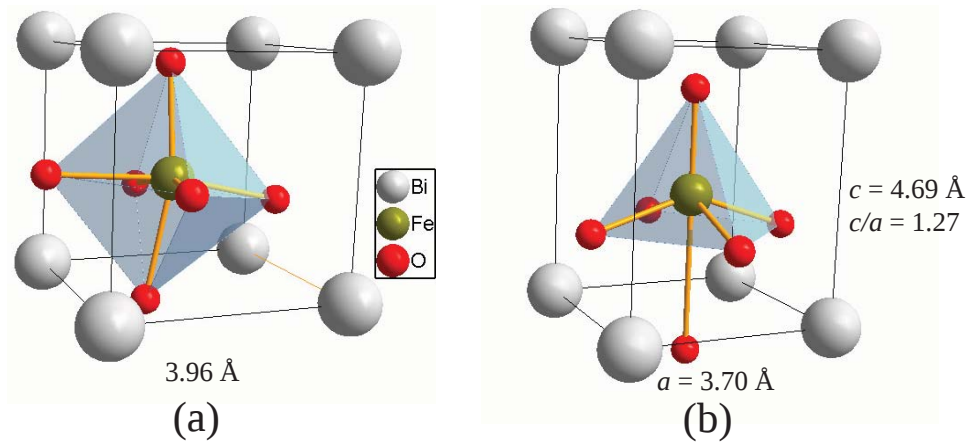
Figure 4.6: (Color online) Schematic view of the local structure around the \text{Fe}^{3+} center of (a) rhombohedral [124] and (b) tetragonal [143] \text{BiFeO}_3 . (after Ref. [105])
