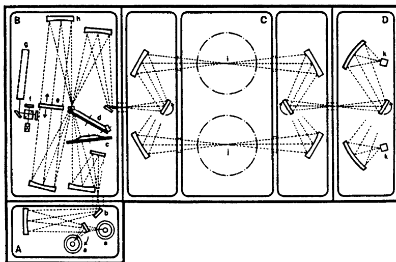
Figure 3.2: Optical layout of the Bruker 113V FTIR spectrometer.
