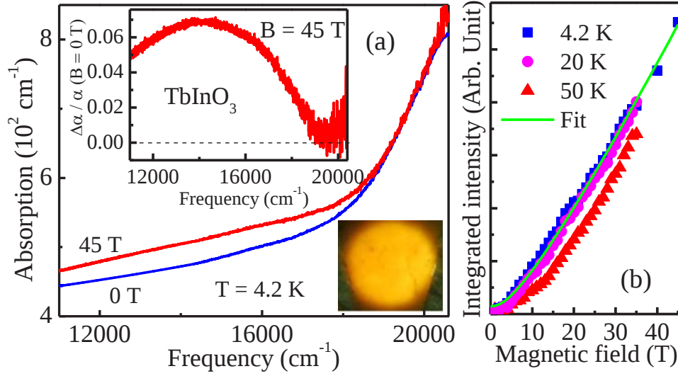
Figure 7.2: (Color online) (a) Absorption coefficient, \alpha(E) , of \text{TbInO}_3 in the field of 0 and 45 T at 4.2 K. Top inset: Absorption difference spectra [\frac{\Delta\alpha(B)}{\alpha(0\text{ T})} = \frac{\alpha(45\text{ T}) - \alpha(0\text{ T})}{\alpha(0\text{ T})}] . Bottom inset: Transmittance image of a polished \sim 100\text{ }\mu\text{m} sample. (b) Integrated intensity in the range of excitation edge (12000 - 17000 \text{cm}^{-1} ) as a function of magnetic field at selected temperatures: 4.2, 20 and 50 K. The integrated magnetization C_1 \int M(B)dB fits well with the integrated intensity trend, where M(B) is the magnetization and C_1 is a constant.
