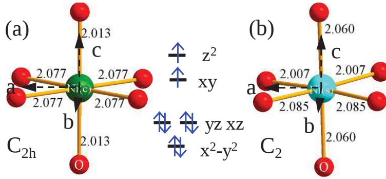
Figure B.1.1: The local structure of the (a) cross-tie NiO 6 and (b) distorted spine NiO 6 octahedron [87]. The local coordinate system is also indicated. The central diagram illustrates the electron configuration of Ni 2+ ( d 8 ).
