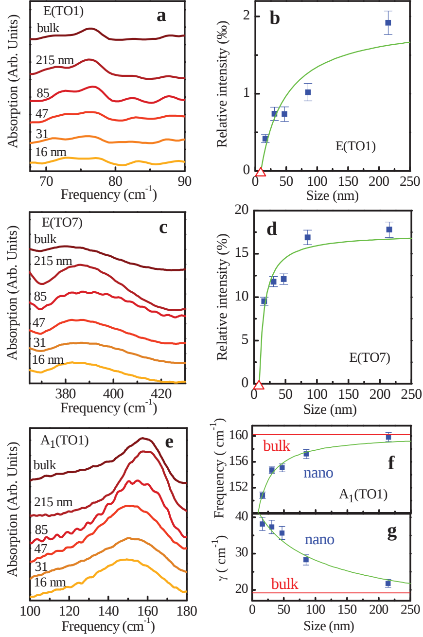
Figure 4.3: (Color online) Close-up view of selected phonon modes of \text{BiFeO}_3 as a function of size (diameter) at 300 K. These modes include features of (a) E(\text{TO1}) , (c) E(\text{TO7}) , and (e) A_1(\text{TO1}) symmetries. Important trends quantified include (b) the relative intensity of the E(\text{TO1}) mode vs. size, (d) the relative intensity of the E(\text{TO7}) mode vs. size, (f) the frequency of the A_1(\text{TO1}) mode vs. size and (g) the damping of the A_1(\text{TO1}) mode vs. size. The green solid lines are the calculated curves fit to the data, described in the text. Red triangles mark the critical size 13.5 nm and 8.1 nm for E(\text{TO1}) and E(\text{TO7}) modes respectively. (after Ref. [10])
