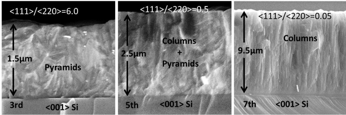
Figure 4-39. SEM images of the cross-sections of the 3rd, 5th and 7th samples involved in of XRD count ratio versus film thickness plot. The evolution of the morphology is: pyramids → Pyramids+columns → columns. This trend matches well with the XRD results.
