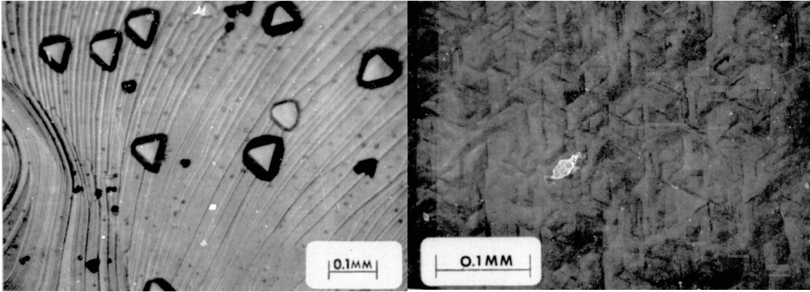
Figure 2-6. Oriented BP crystallites deposited on the Si-face of a hexagonal SiC substrate, early stage planview on the left and the surface of the 40µm film on the right. The triangular crystallites of opposite orientations indicate different stacking possibilities. [19]
