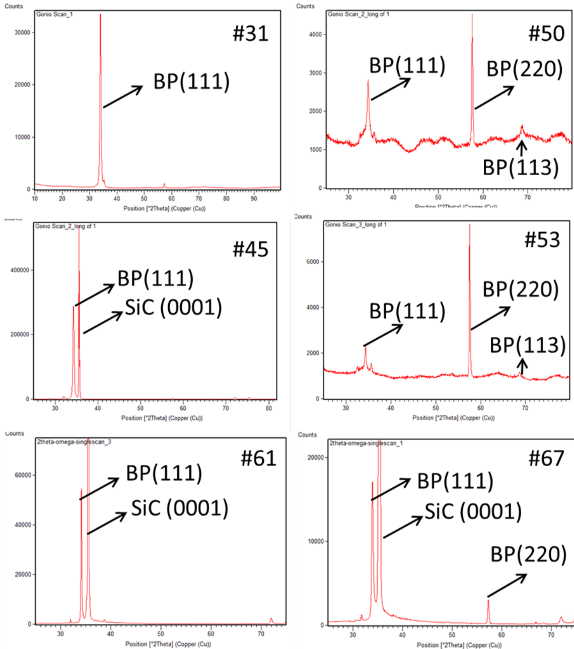
Figure 4-12. XRD examinations of the samples of the offcut angle study. Apparently, film grown on the 4° offcut wafers all have a large epitaxial component since the XRD patterns are all dominated by the BP (111) diffractions. However, the 8° offcut wafers do not yield epitaxial growth. Note that sample 67 performs better than sample 50 and 53, this should be due to the temperature adjustment. TEM analysis will be necessary.
