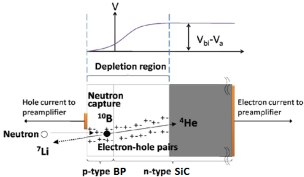
Figure 1-1. Device structure of a semiconductor neutron detector. [4]
