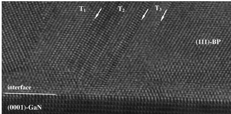
Figure 2-5. High-resolution TEM image of (111)-BP layer grown on (0001) GaN. Grain boundaries in the (111)-BP layer are indicated with arrows (↓). [42]
