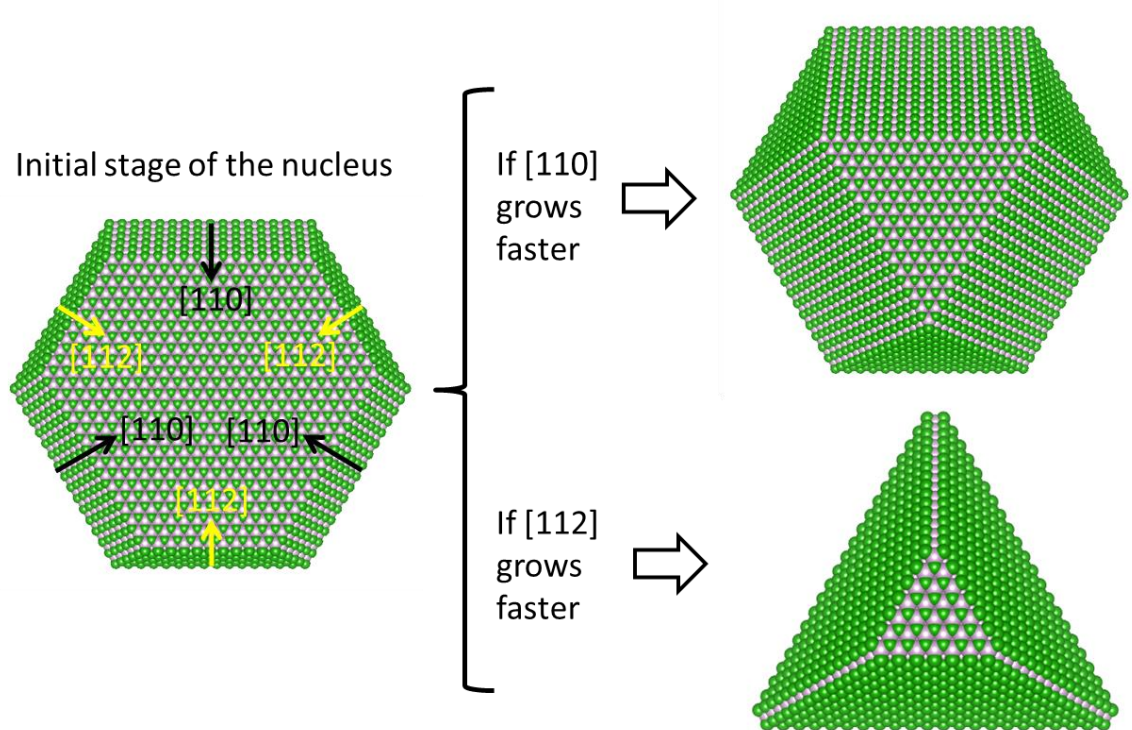
Figure 4-41. Effect of facet growth rate on the shape evolution of a nucleus.
