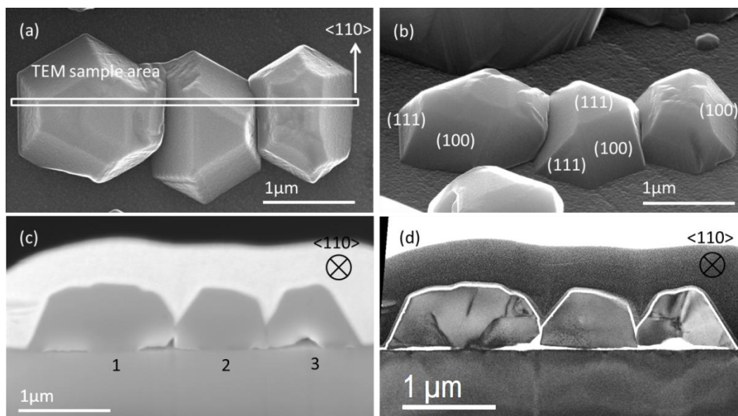
Figure 4-42. SEM and STEM overview of the truncated octahedral nuclei. (a). SEM image of the planview of the nuclei. TEM sampling area is labeled. (b). 54° tilted view of the nuclei. Some of the facet planes are indexed. (c). SEM image of the cross-section sample. This TEM sample is cutted via FIB. (d) STEM image of the cross-section. Features such as grain boundaries and stacking faults can be seen.
