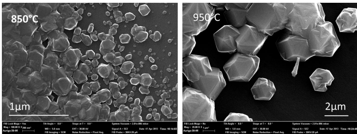
Figure 4-17. SEM Comparison of between the nuclei formed at 850°C and 950°C. The average nucleus size of the 850°C sample is smaller. It is consistent with what was concluded from Figure 4-16.
