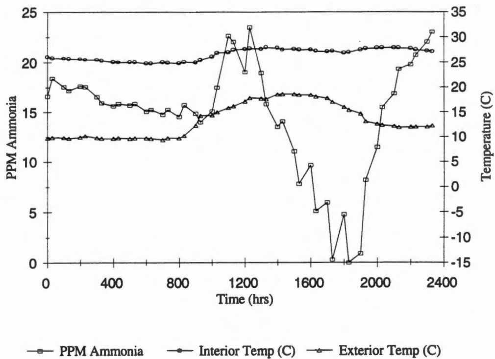
Figure 4. Ammonia levels and temperatures October 25, 1994 at Farm A (naturally ventilated).
