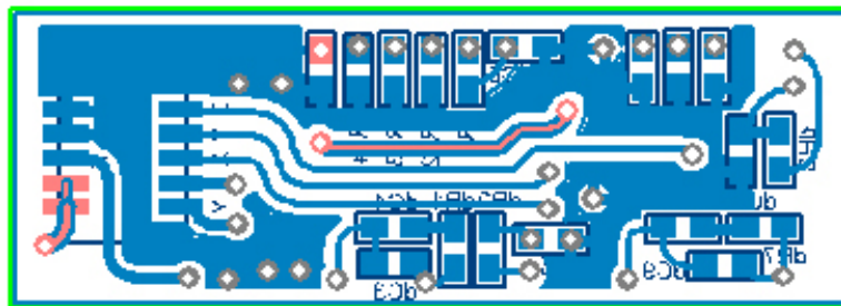
Figure B-10: Layout for accelerometers and gyroscopes sensor strip (Bottom Copper)
