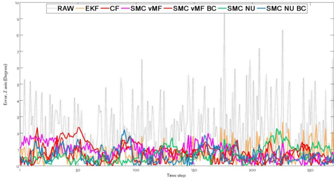
Figure 7-2 – Error between different algorithms and the intended motion
