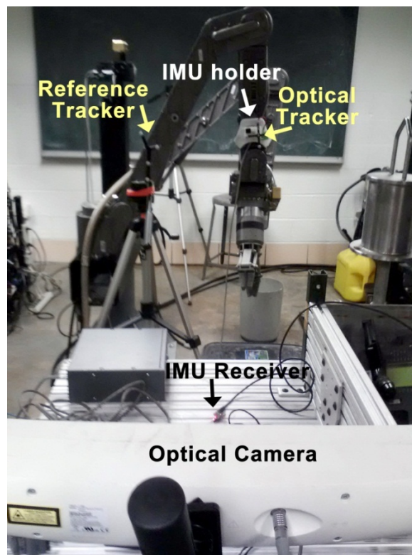
Figure 7-6 – Experimental setup with robotic manipulator
