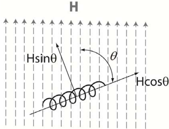
Figure 3-6 - Principle of magnetometer. The dash arrows represent the direction of the magnetic field H , and angle \theta is the deviation angle between the coil and the magnetic field
