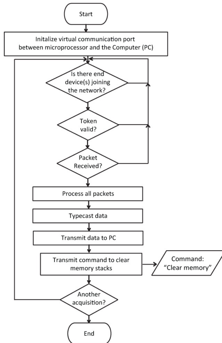
Figure 5-8 -Firmware instruction flow for Access Point
