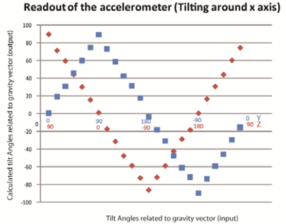
Figure 4-6 - Calibrated tilt angle output of Y and Z around the x axis
