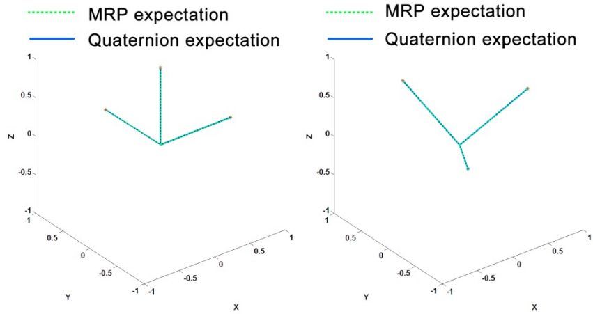
Figure C-1: Expectations between quaternion and MRP converted quaternion; (Left) no offsets, (Right) offset rotation [45 45 45]
