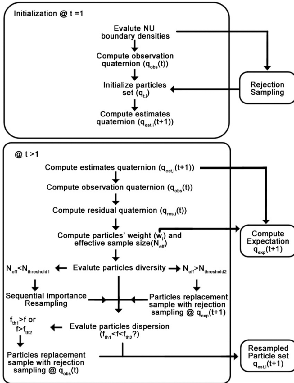
Figure 6-7 - Functional block diagram of the PF algorithm with non-uniform density
