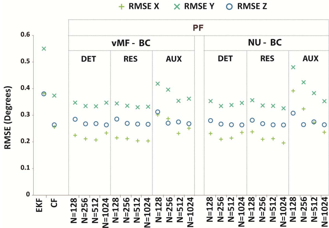
Figure 7-21 – RMSE of PF with BC against benchmark algorithms in static experiment
