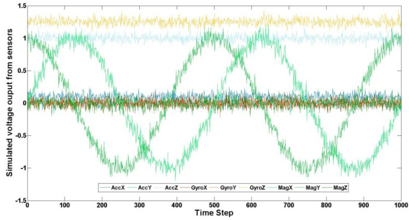
Figure 7-1 - Synthetic signal simulated raw output of the sensors
