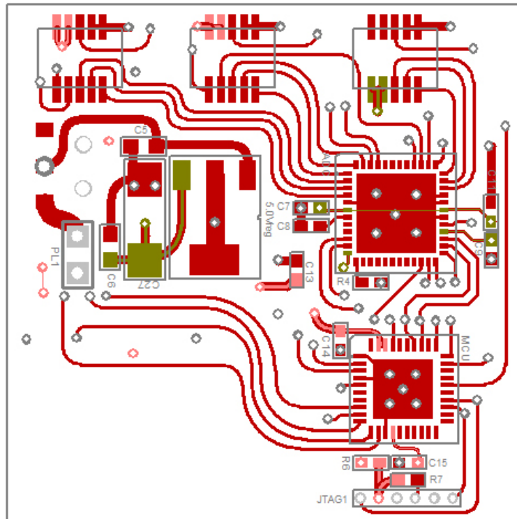
Figure B-1: Layout for signal processing board (Top Copper)
