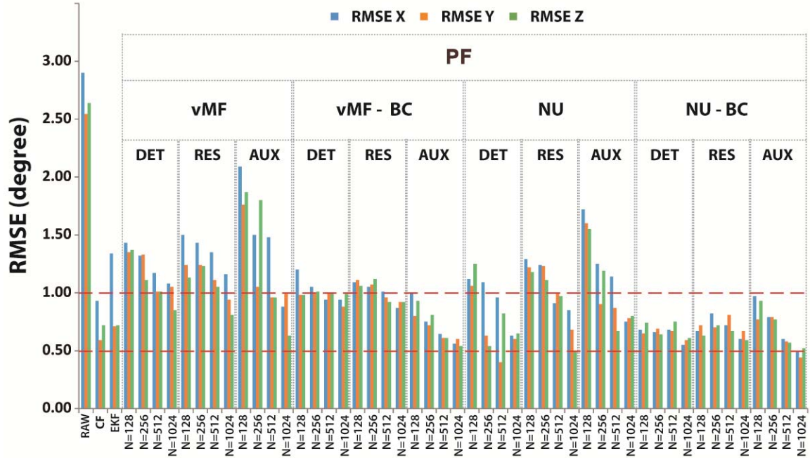
Figure 7-3 – RMSE of the testing algorithms for synthetic signal
