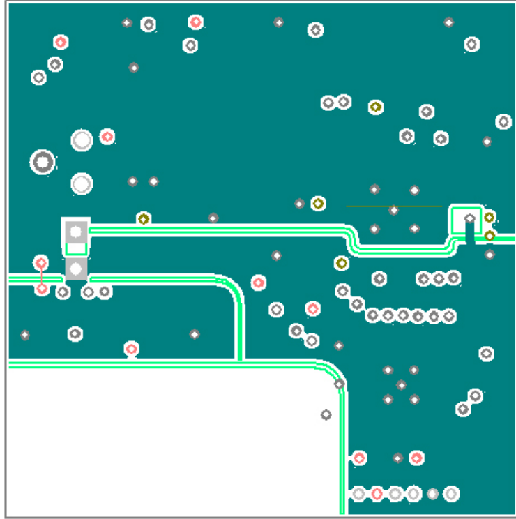
Figure B-7: Layout for signal processing board (Inner Layer: Ground)
