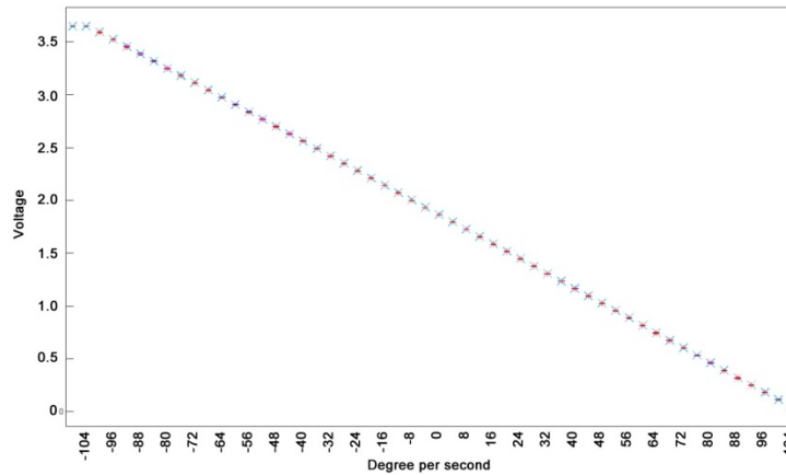
Figure 5-1 Box plot of the X-axis of the gyroscopes (LPR510-AL) undergoing rotations at different angular velocities
