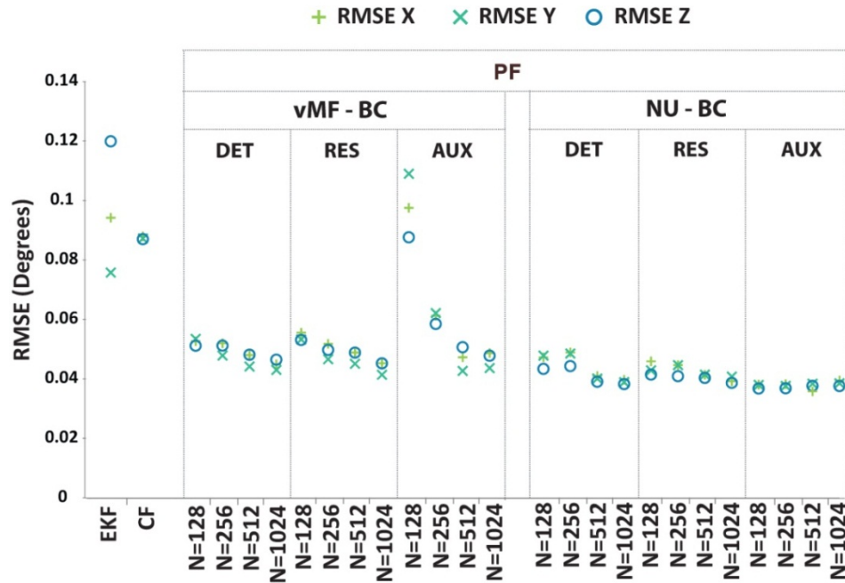
Figure 7-9 – RMSE of PF with BC against benchmark algorithms for static experiment
