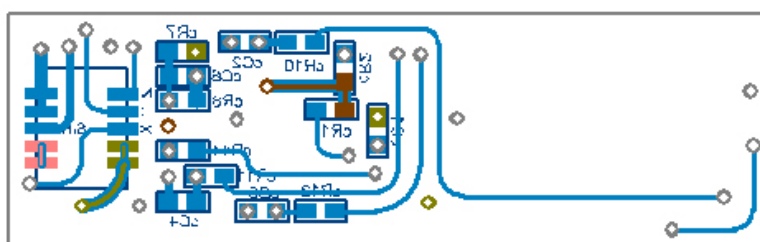
Figure B-4: Layout for magnetometer sensor strip (Bottom Copper)
