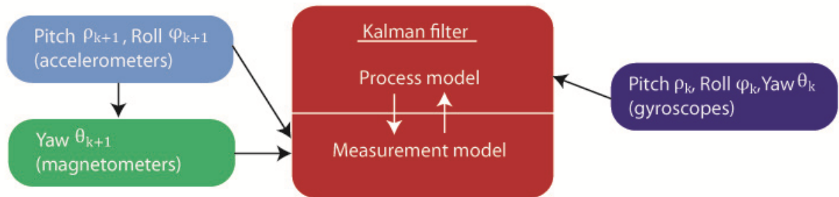
Figure 4-10 - Kalman filter models for IMU
