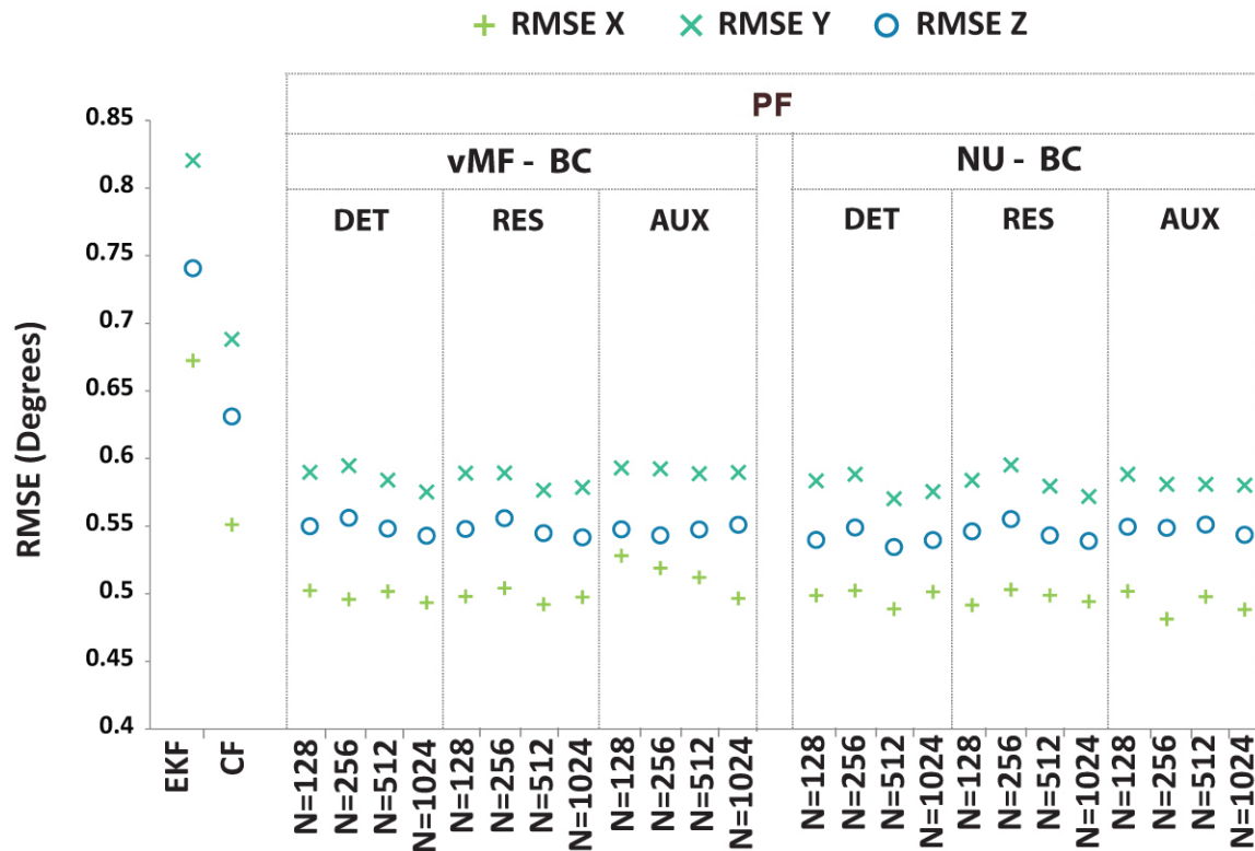
Figure 7-23 – RMSE of PF with BC against benchmark algorithms in dynamic experiment
