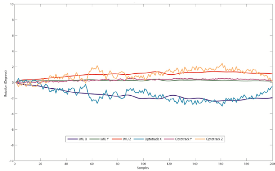
Figure 4-15 - IMU vs optical outputs (Standing, Thigh) Light blue: Optical X, Purple: Optical Y, Yellow: Optical Z; Dark blue: IMU X, Green: IMU Y, Red: IMU Z
