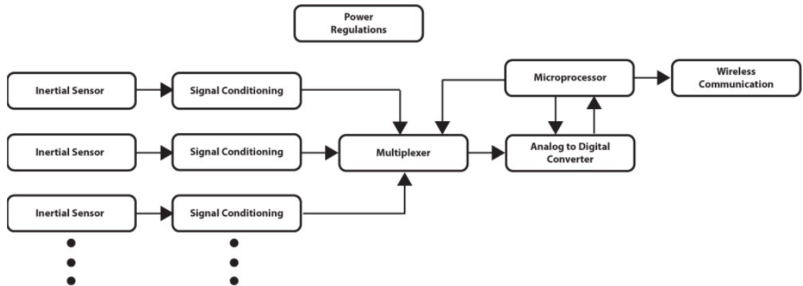
Figure 5-2 - System Architecture for Prototype IMU
