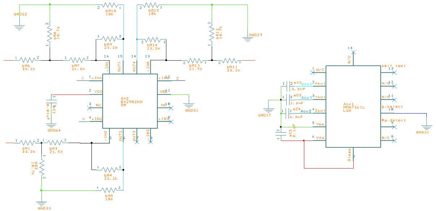
Figure A-4: Schematic for Accelerometers and its signal conditioning circuit (1.5g setup)
