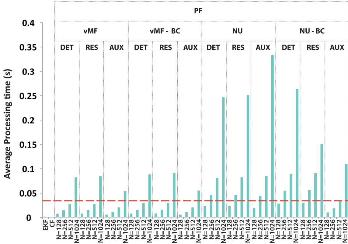
Figure 7-24 – Average processing time of the testing algorithms for free hand activities
