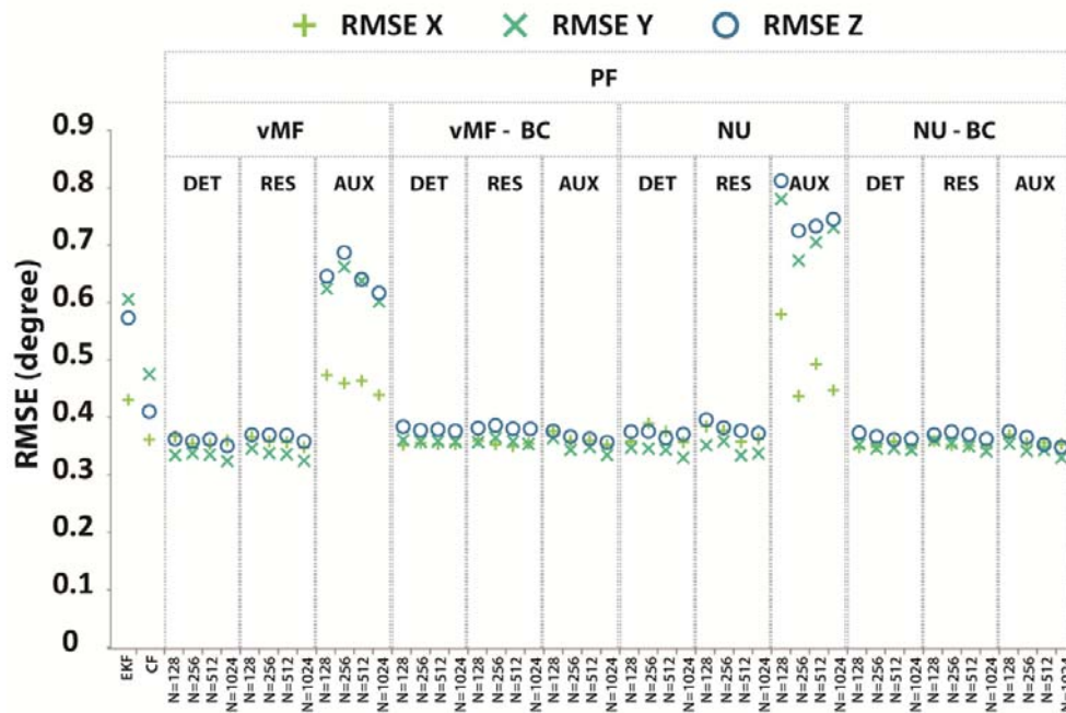
Figure 8-5 — Comparison between the RMSE of PF and the benchmark algorithms for shank during knee joint activities
