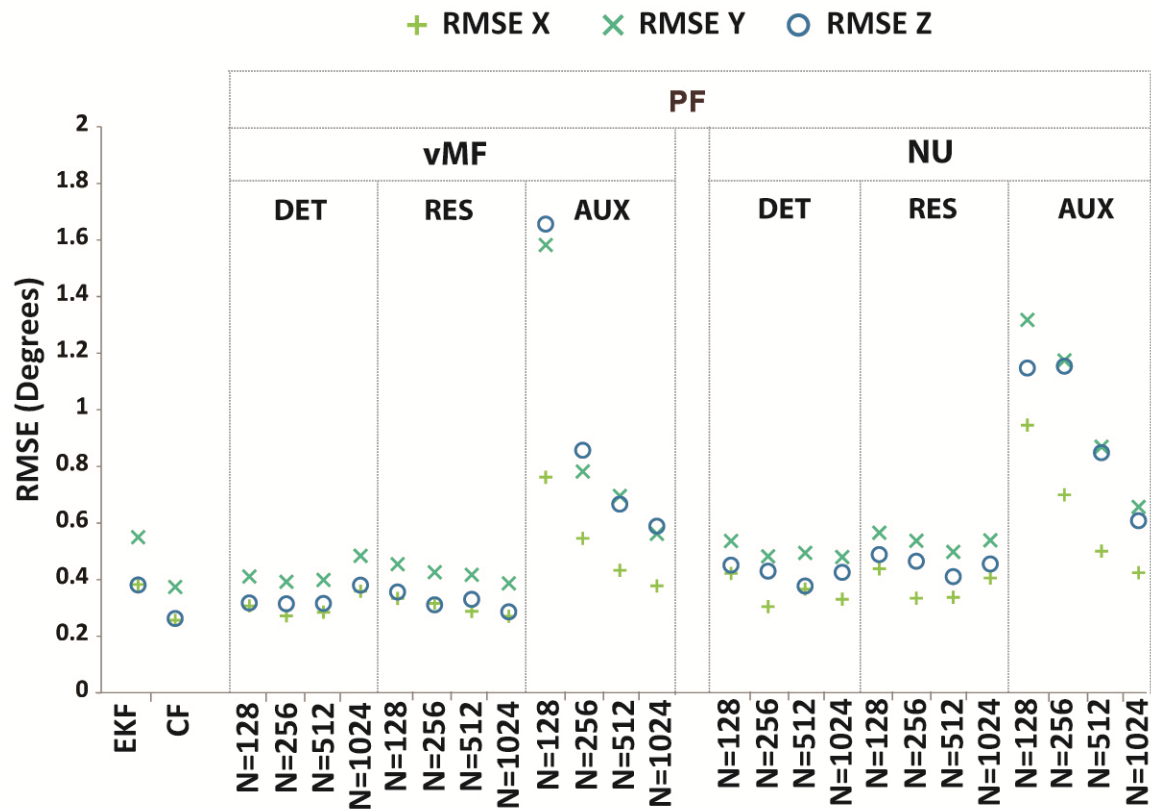
Figure 7-20 – RMSE of PF without BC against benchmark algorithms in static experiment
