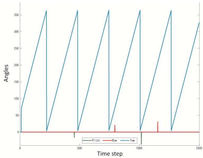
Figure 4-12 - Output after EKF
