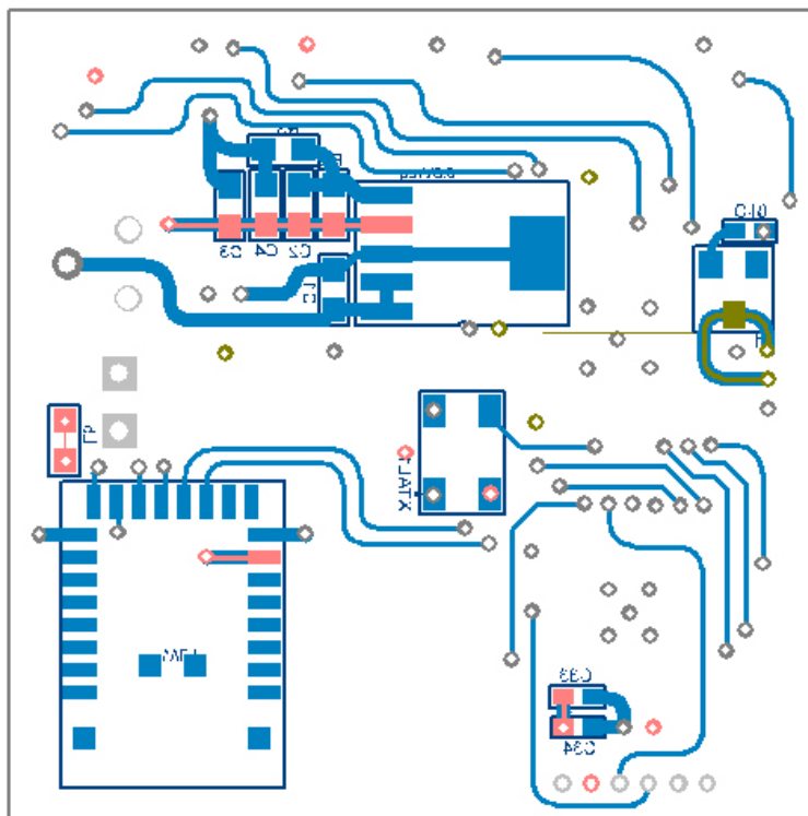
Figure B-3: Layout for signal processing board (Bottom Copper)
