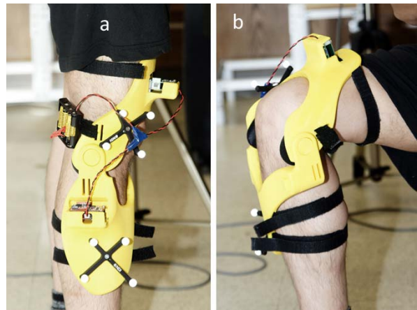
Figure 4-14 - Static testing with IMU brace. (a) Standing still; (b) Sitting still
