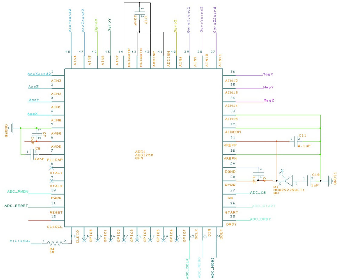
Figure A-3: Schematic for ADC and clock
