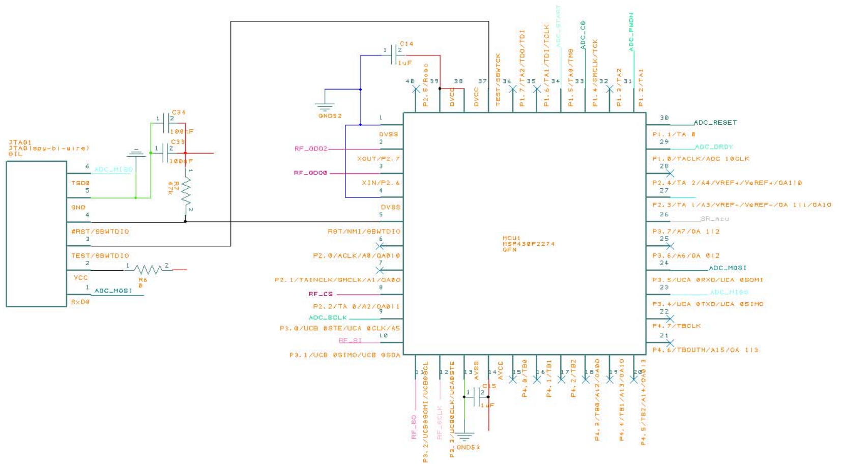
Figure A-2: Schematic for Microcontroller and JTAG setup
