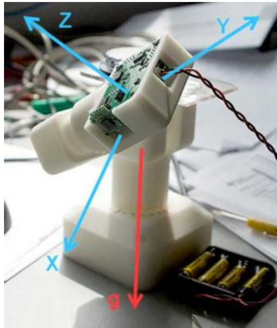
Figure 4-2 - Plastic arm for accelerometer calibration
