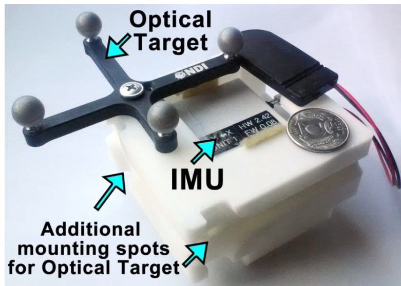
Figure 7-13 – Plastic container for both the IMU and optical systems for free hand motion
