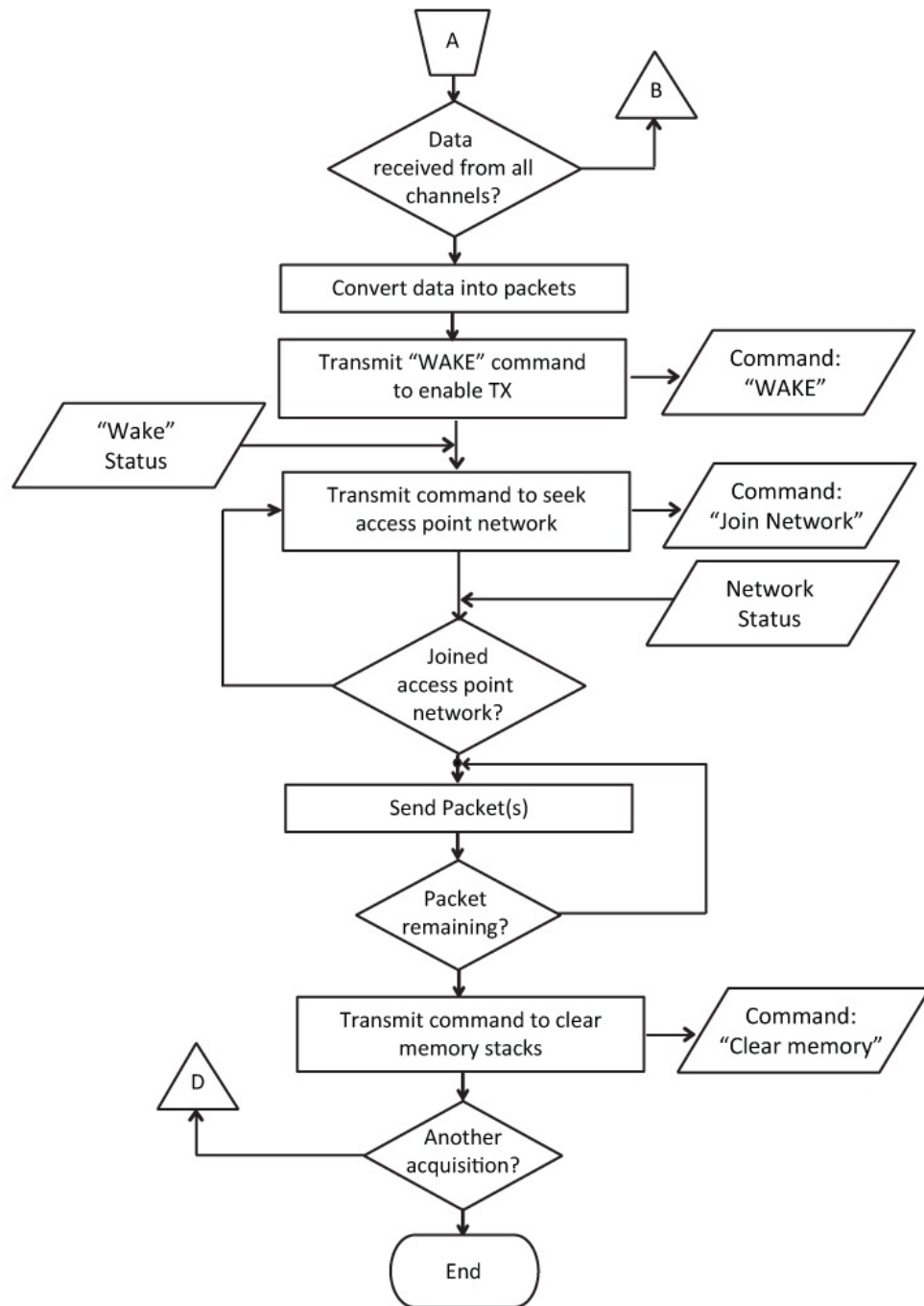
Figure 5-7 - Firmware instruction flow for end devices (B)
