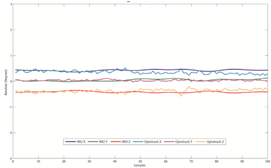
Figure 4-17 - IMU vs optical outputs (Sitting, Thigh) Light blue: Optical X, Purple: Optical Y, Yellow: Optical Z; Dark blue: IMU X, Green: IMU Y, Red: IMU Z
