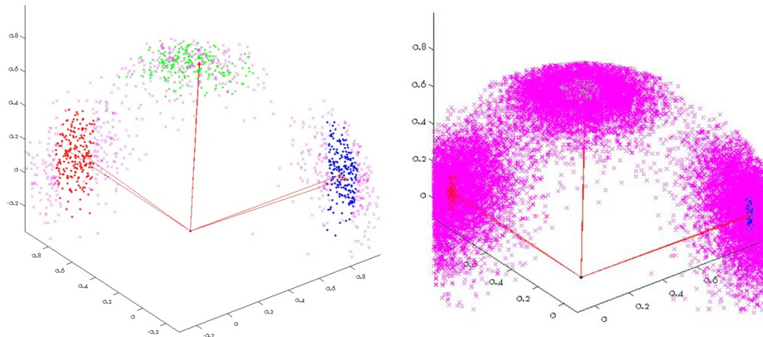
Figure 7-5 - Difference in Rejection Rate for PF with (Left) and without (Right) BC. Magenta indicates rejected particles
