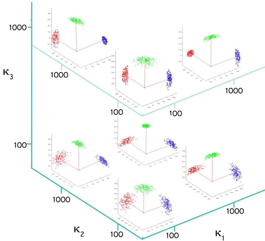
Figure 6-3 – Randomly sampled quaternions with non-uniform distributions with different density proportion in K . The samples are projected to 3-sphere with identity matrix. The red lines indicate the mean direction of the samples.
