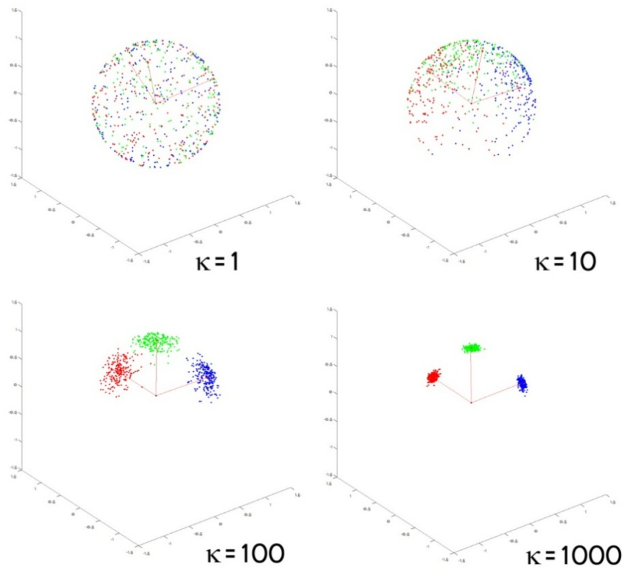
Figure 6-2 – Randomly sampled quaternions with von Mises-Fisher distributions with different dispersion factor. The samples are projected to 3-sphere with identity matrix. The red lines indicate the mean direction of the samples.
