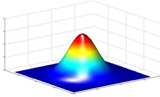
Figure 6-1- Generic 3D distribution
