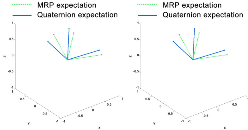
Figure C-2: Comparison between the expectations of the original quaternion sampled from vMF density and the quaternion converted from the MRP expectation; (Left) offset rotation: [0 4 359], (Right) offset rotation: [355 0 5]
