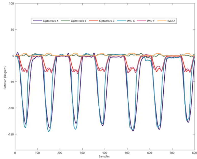
Figure 4-23 - IMU vs optical outputs (Chair RiseThigh). Dark blue: Optical X, Green: Optical Y, Red: Optical Z; Light blue: IMU X, Purple: IMU Y, Yellow: IMU Z
