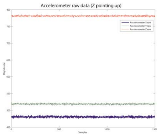
Figure 4-3 - Raw data from the accelerometer
