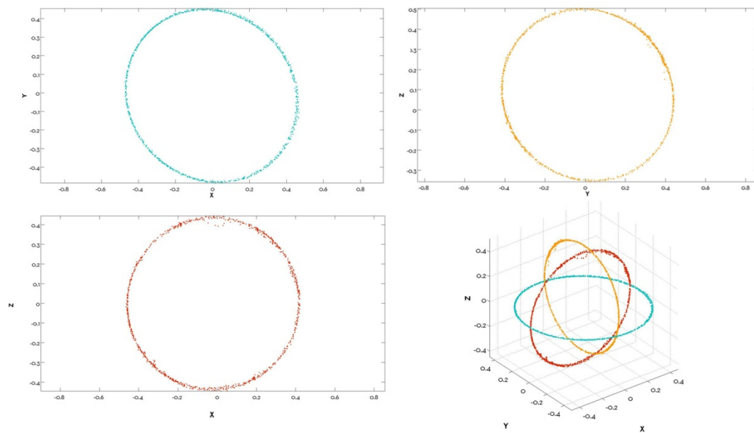
Figure 7-25 – Raw magnetometers output (Blue: Z axis, Red: Y axis, Orange: X axis)
