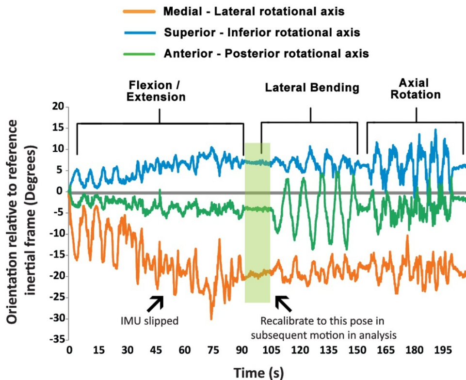
Figure 8-14 – Orientations of IMU located at L5 relative to the reference inertial frame for degenerative subject
