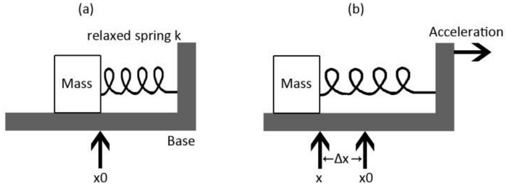
Figure 3-2 - Conceptual illustration of accelerometers
