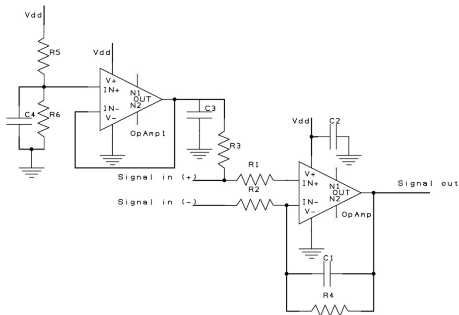
Figure 5-5 – Signal conditioning circuit for Magnetometers
