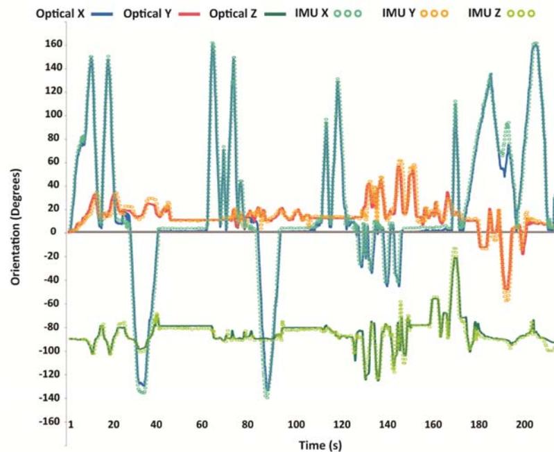
Figure 7-17 – Activity in Figure 7-16 processed with PF (NU density, BC, RES, 256 particles)
