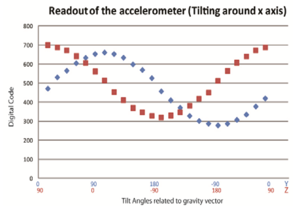
Figure 4-4 - Readout of the accelerometer tilting around the x axis
