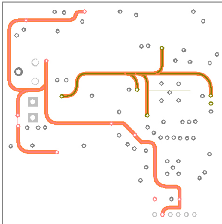
Figure B-5: Layout for signal processing board (Inner Layer: Power)
