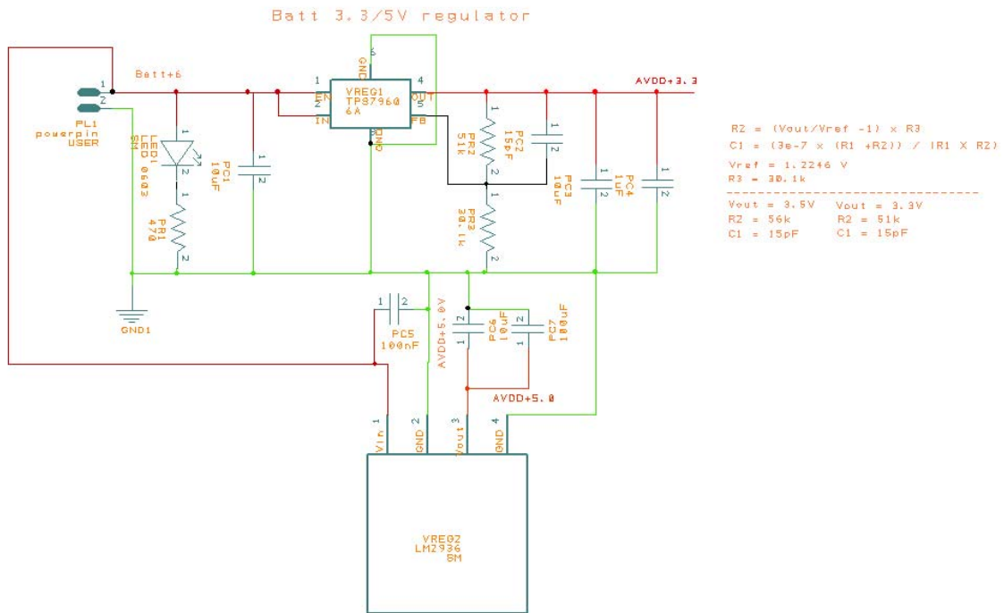
Figure A-1 - Schematic for powering circuit
