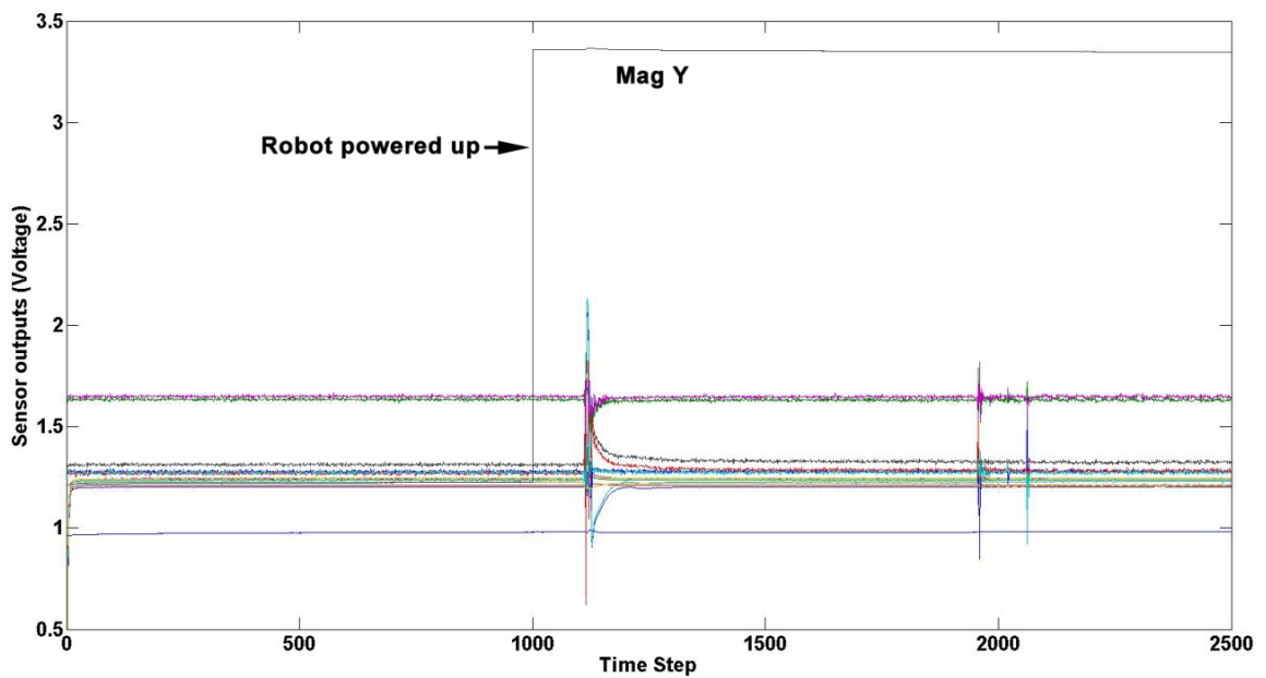
Figure 7-7 – Raw sensor output showing the magnetic interference of the robot to the magnetometer
