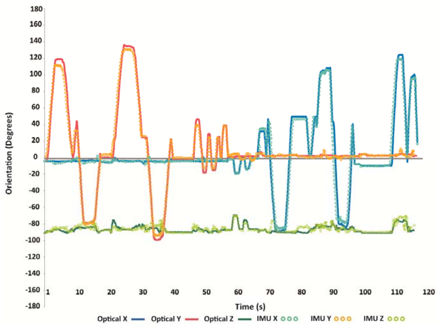
Figure 7-19 – Activity in Figure 7-18 processed with PF (NU density, BC, RES, 256 particles)
