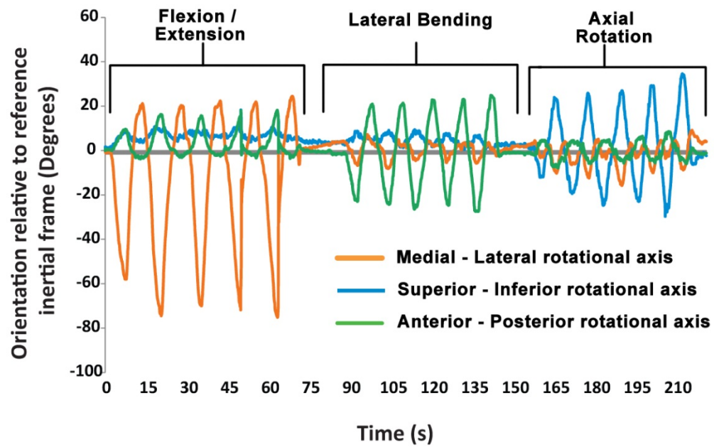
Figure 8-11 – Orientations of IMU located at L1 relative to the reference inertial frame for healthy subject
