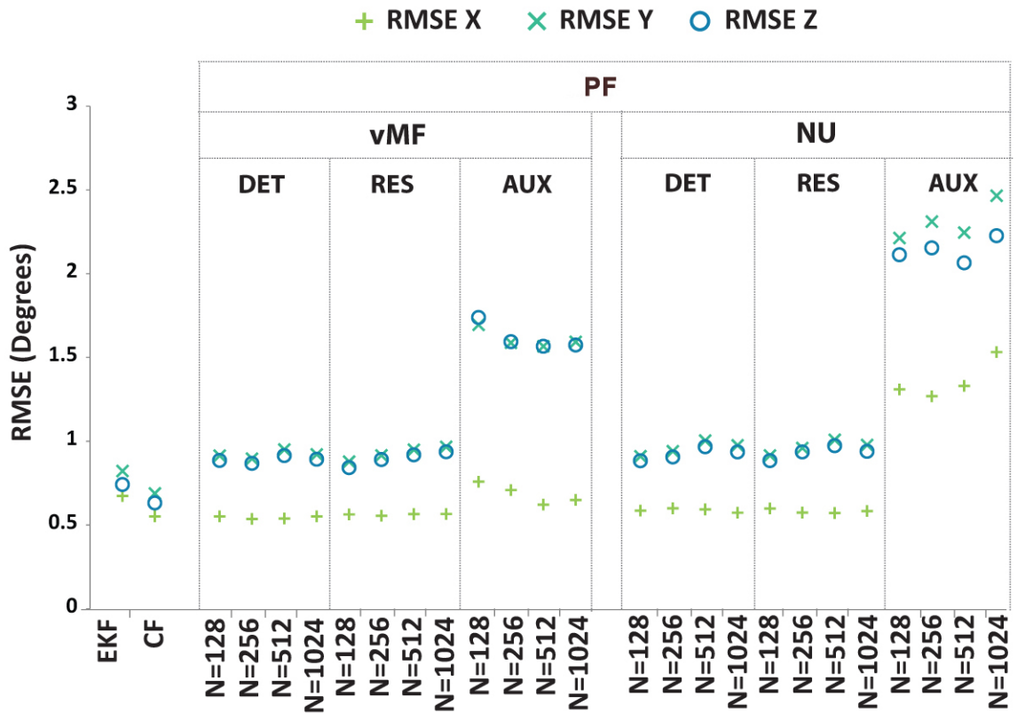
Figure 7-22 – RMSE of PF without BC against benchmark algorithms in dynamic experiment
