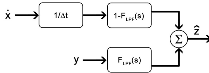
Figure 2-3 - Principle of Complementary Filter for IMU system
