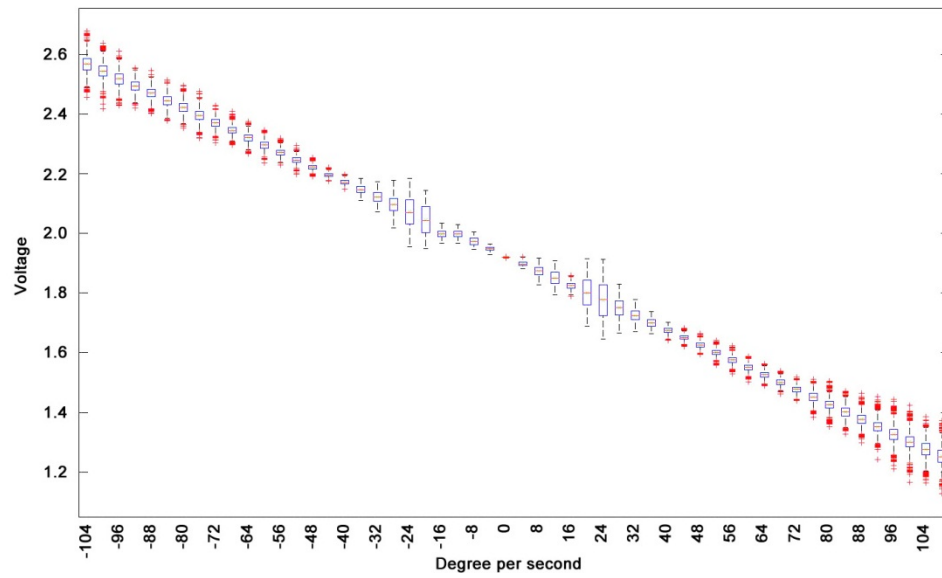
Figure 4-25 - Box plot of the X-axis of the gyroscopes undergoing rotations at different angular velocities
