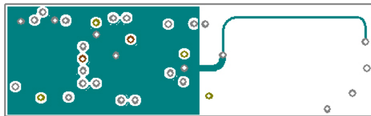
Figure B-8: Layout for magnetometer sensor strip ((Inner Layer: Ground)
