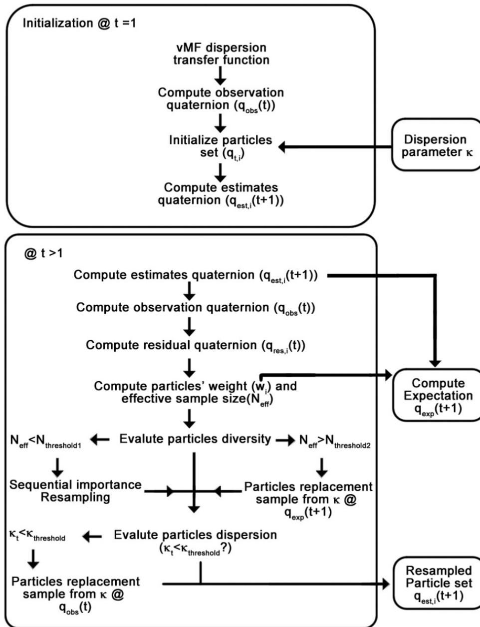
Figure 6-4 – Functional block diagram of the PF algorithm with von Mises-Fisher density
