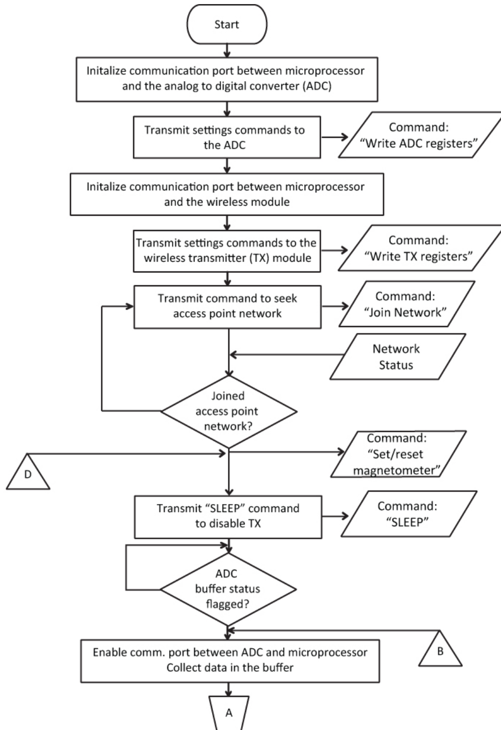
Figure 5-6 - Firmware instruction flow for end devices (A)
