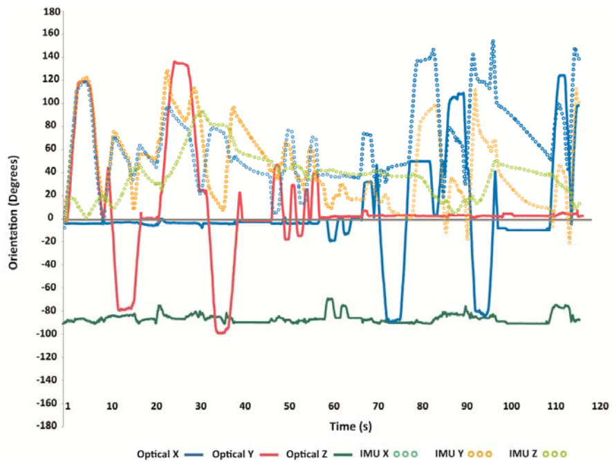
Figure 7-18 – Activity showing the instability of EKF during human motion testing
