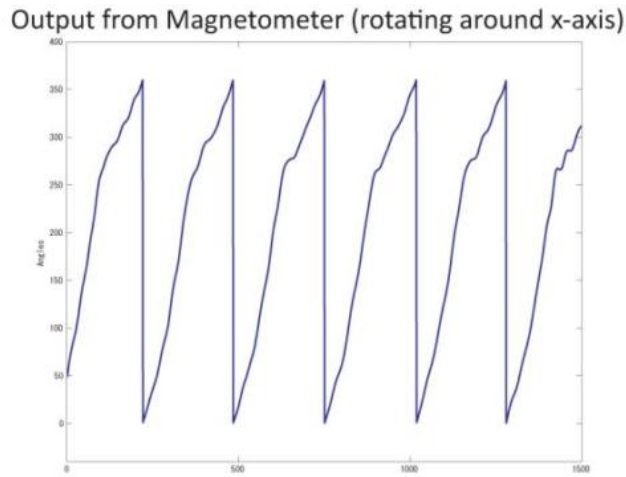
Figure 4-9 - Deviation angle between the sensors to true north calculated from magnetometer rotating around x-axis
