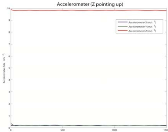
Figure 4-5 - Calibrated static output
