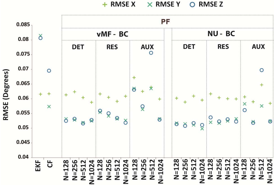
Figure 7-12 – RMSE of PF with BC against benchmark algorithms in dynamic experiment
