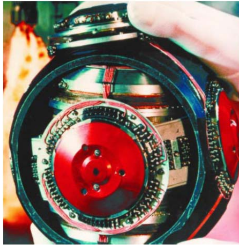
Figure 3-7 - Gimbaled inertial platform by Marconi Electronics (now BAE systems) shows the instrumentation are surrounded by 3 gimbal rings
