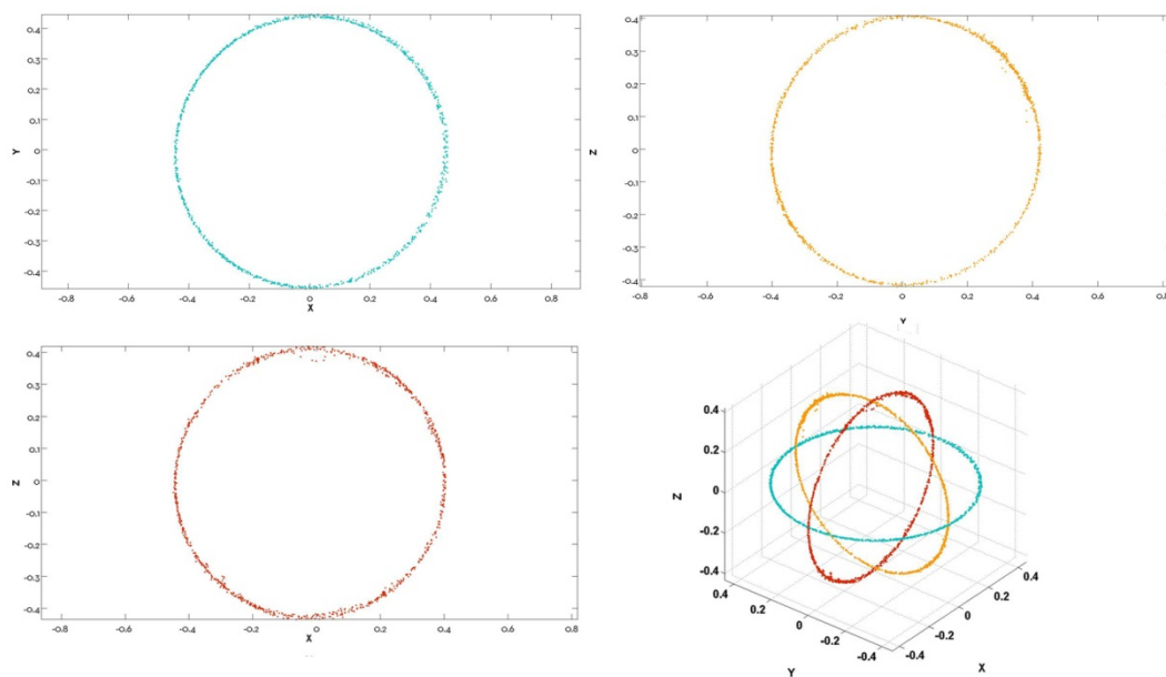
Figure 7-26 – Corrected magnetometers output (Blue: Z axis, Red: Y axis, Orange: X axis)
