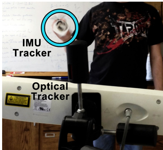
Figure 7-14 – Free hand motion testing
