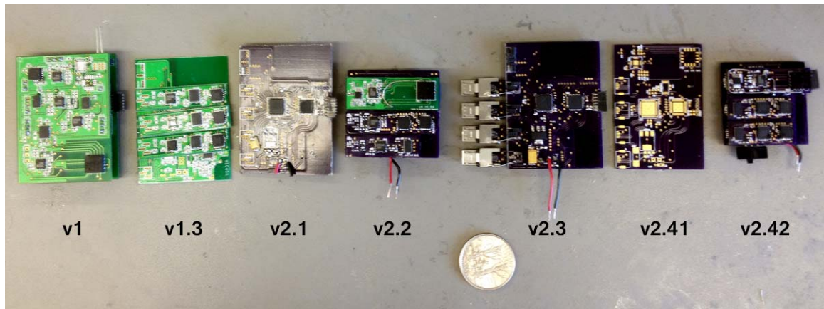
Figure 5-10 - The evolution of the IMU circuit designs
