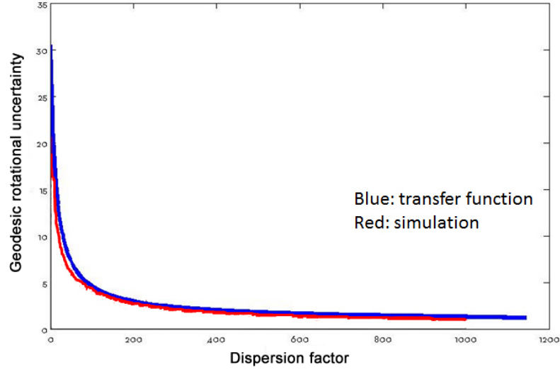
Figure 6-5 – Estimation function between particles uncertainty and dispersion factor
