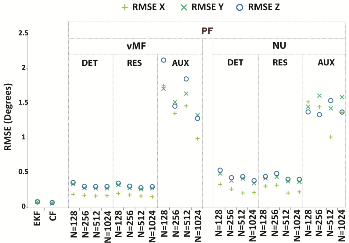
Figure 7-11 – RMSE of PF without BC against benchmark algorithms in dynamic experiment
