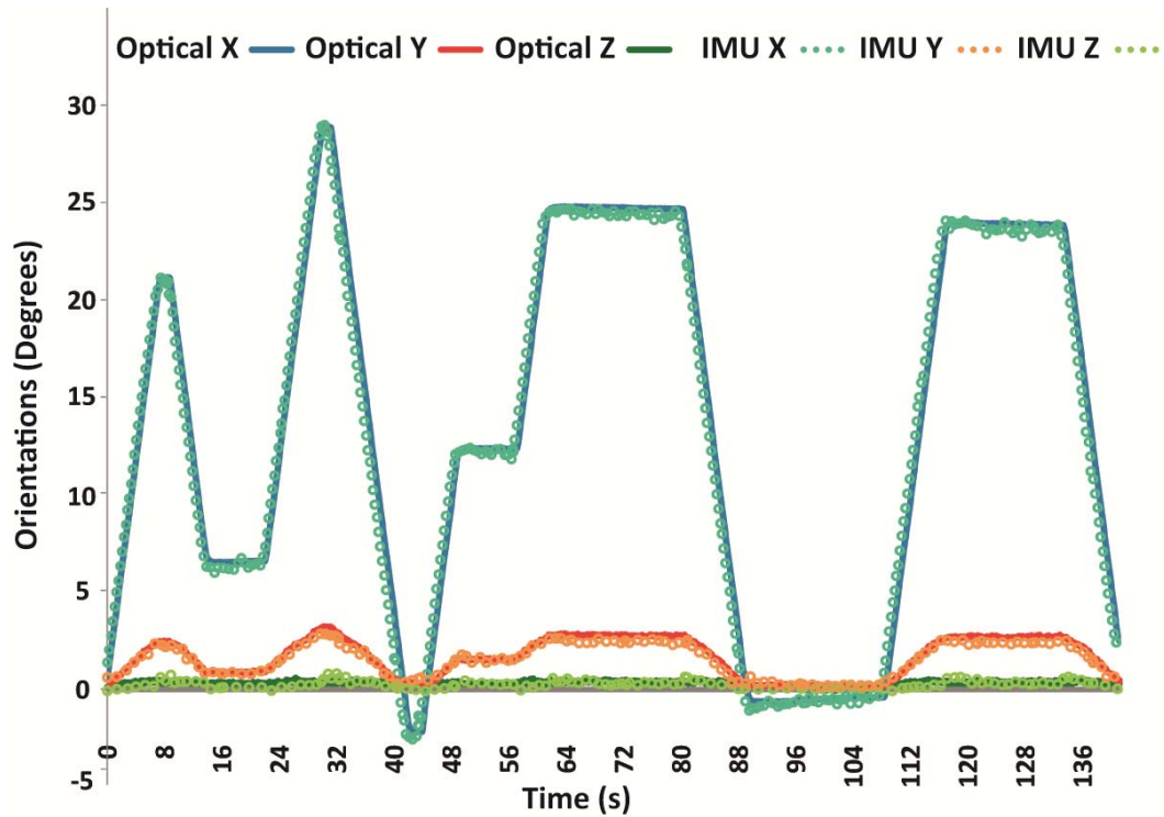
Figure 7-10 – Comparison between IMU data reconstructed with PF with the combination of NU density, BC and 256 particles population and the optical data.
