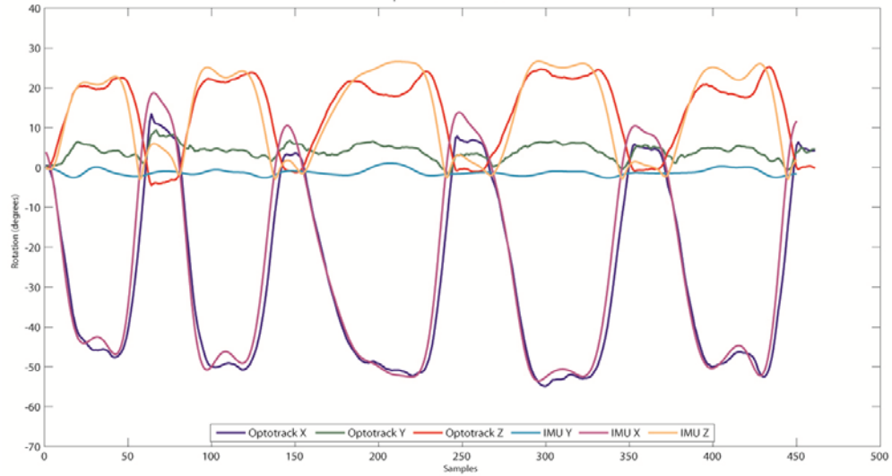
Figure 4-22 - IMU vs optical outputs (Deep Knee Bend, Shank). Dark blue: Optical X, Green: Optical Y, Red: Optical Z; Purple: IMU X, Light blue: IMU Y, Yellow: IMU Z
