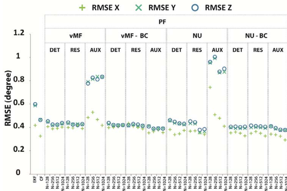
Figure 8-4 — Comparison between the RMSE of PF and the benchmark algorithms for IMU located at thigh during knee joint activities
