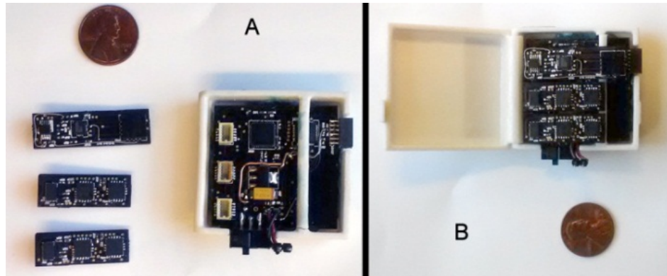
Figure 5-11 – The sensing strips and electronic board of the modular IMU design (A). The assembled IMU system (B)
