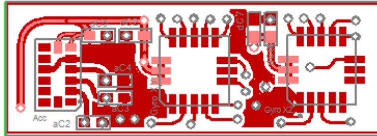
Figure B-9: Layout for accelerometers and gyroscopes sensor strip (Top Copper)
