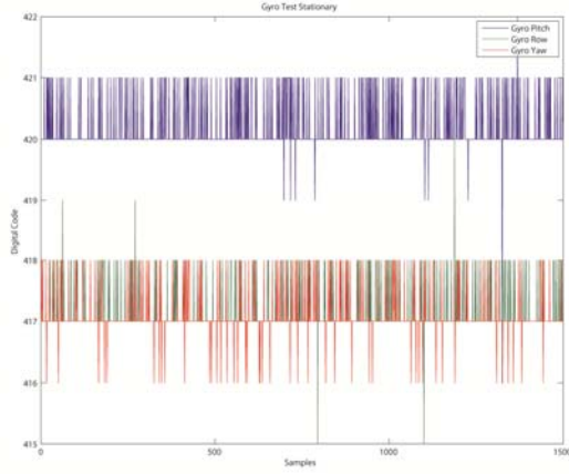
Figure 4-7 - raw data from the gyroscopes
