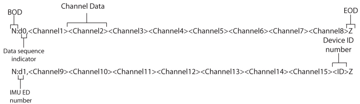
Figure 5-9 – Wireless transmission data format
