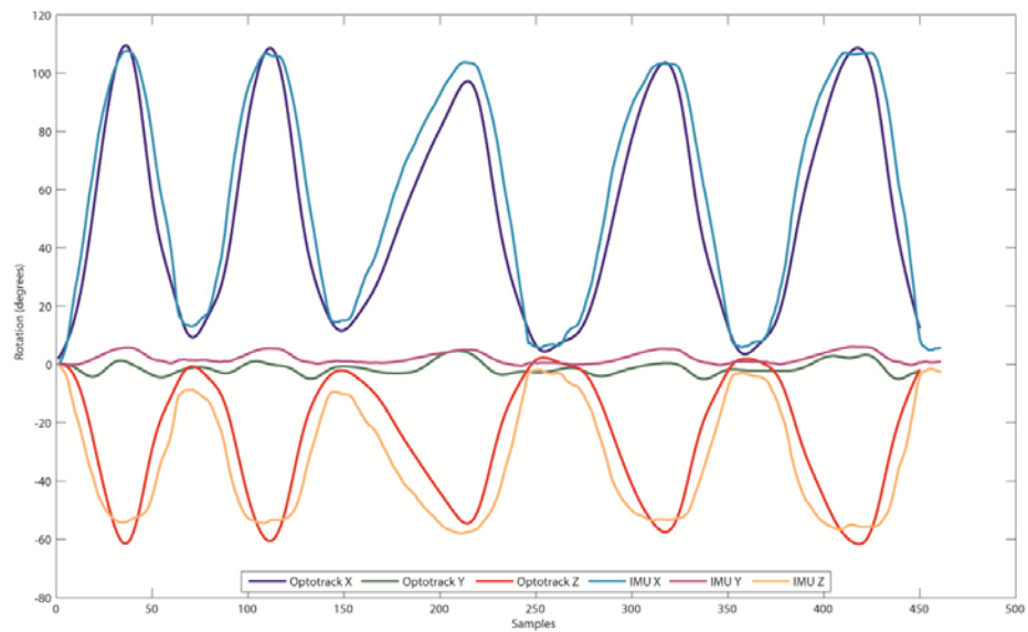
Figure 4-21 - IMU vs optical outputs (Deep Knee Bend, Thigh). Dark blue: Optical X, Green: Optical Y, Red: Optical Z; Light blue: IMU X, Purple: IMU Y, Yellow: IMU Z
