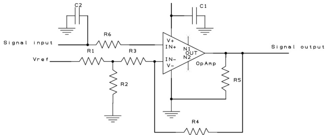
Figure 5-3 - Signal conditioning circuit for accelerometers and gyroscopes
