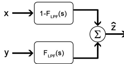
Figure 2-2 - Principle of Complementary Filter ( F_{LPF}(s) is a low pass filter)
