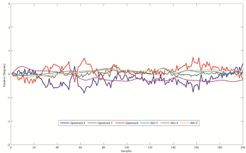
Figure 4-18- IMU vs optical outputs (Sitting, Shank) Dark blue: Optical X, Green: Optical Y, Red: Optical Z; Purple: IMU X, Light blue: IMU Y, Yellow: IMU Z
