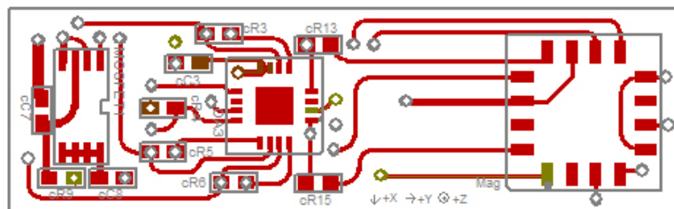
Figure B-2: Layout for magnetometer sensor strip (Top Copper)
