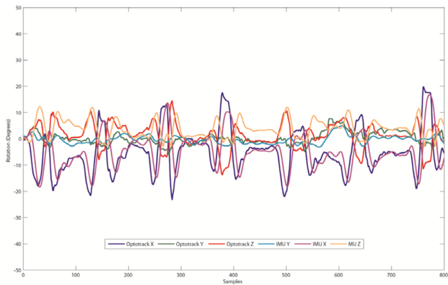
Figure 4-24 - IMU vs optical outputs (Chair Rise, Shank). Dark blue: Optical X, Green: Optical Y, Red: Optical Z; Purple: IMU X, Light blue: IMU Y, Yellow: IMU Z
