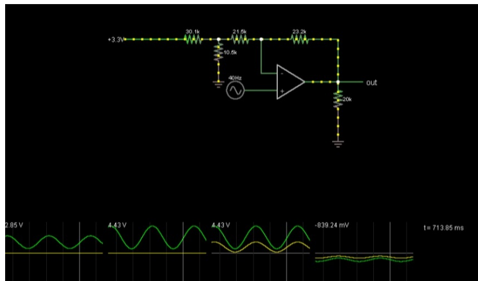
Figure 5-4 - Circuit simulation for the signal conditioning circuit
