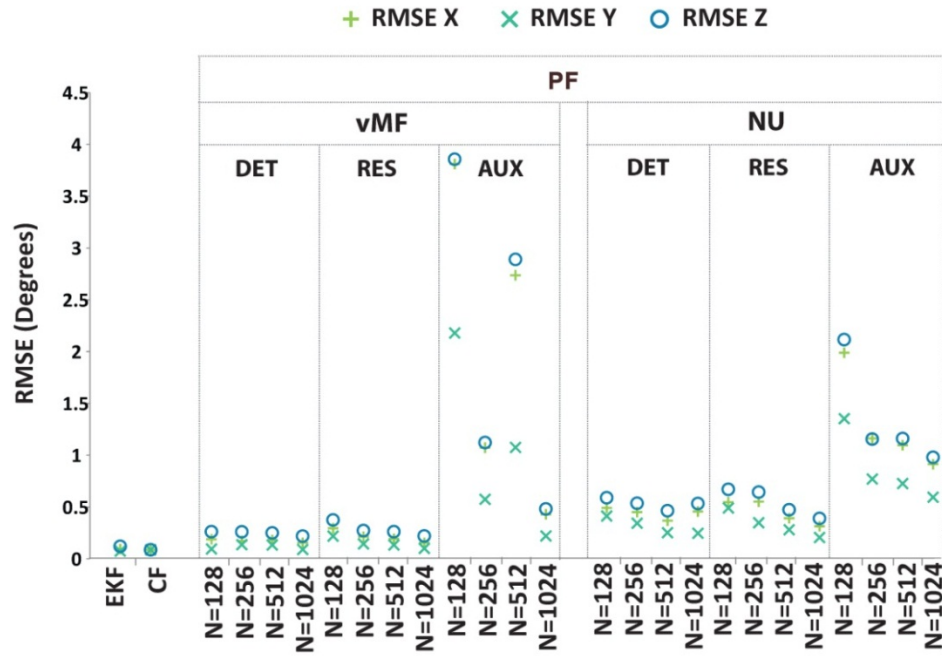
Figure 7-8 – RMSE of PF without BC against benchmark algorithms in static experiment
