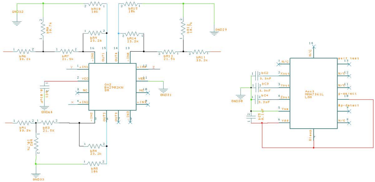
Figure A-5: Schematic for Accelerometer and its signal conditioning circuit (6g setup)
