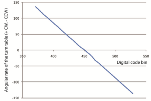
Digital output of the gyroscope rotating around axis X
