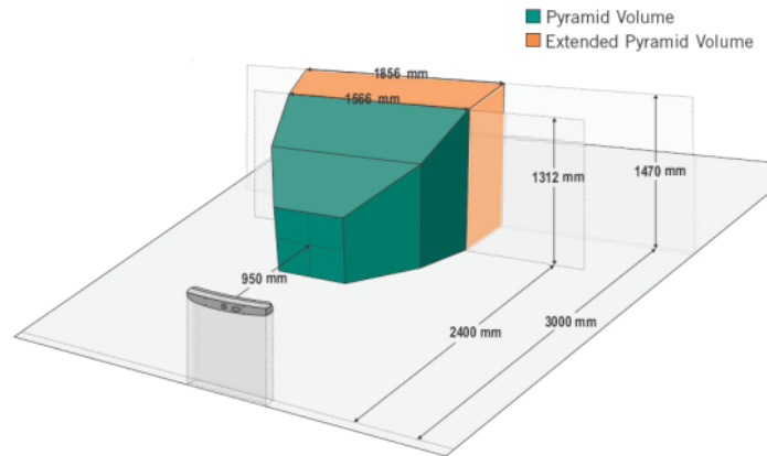
Figure 1-3: NDI Polaris Spectra view volume with 2.050 m in the z-direction and an in-plane area of 1.856 x 1.470 m 2 at a z distance of 3.000 m [5]
