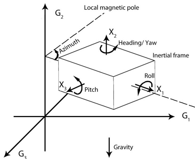
Figure 3-1 - Reference frames and axes of the IMU system
