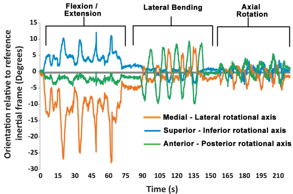
Figure 8-12 – Orientations of IMU located at at L5 relative to the reference inertial frame for healthy subject
