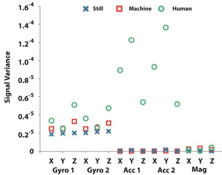
Figure 7-15 – Signal variance of the IMU tracker during still, static (robot), static (human)
