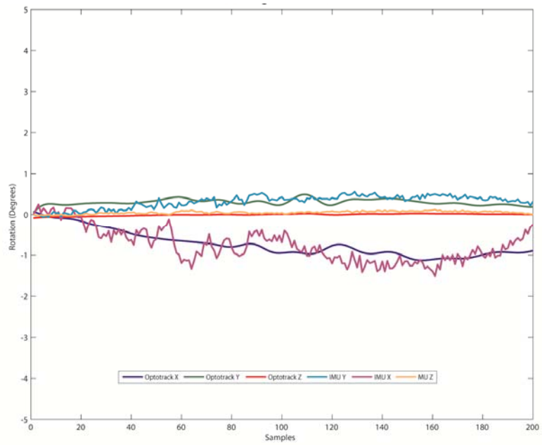
Figure 4-16 - IMU vs optical outputs (Standing, Shank) Dark blue: Optical X, Green: Optical Y, Red: Optical Z; Purple: IMU X, Light blue: IMU Y, Yellow: IMU Z
