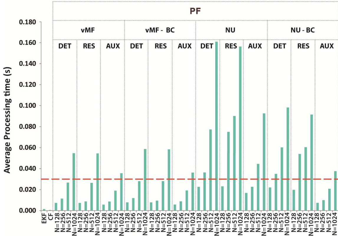
Figure 7-4 – Average processing time of the testing algorithms
