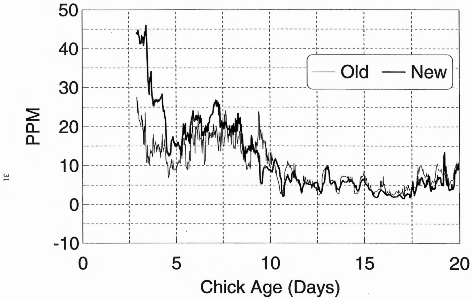
Figure 5. Carbon monoxide concentrations measured during the first half of the November grow-out.
