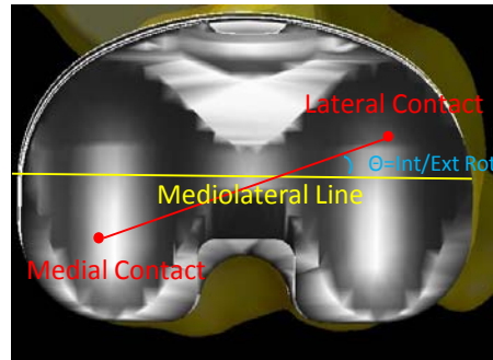
Figure 109: Description of internal/external rotation calculation in Figure 108
