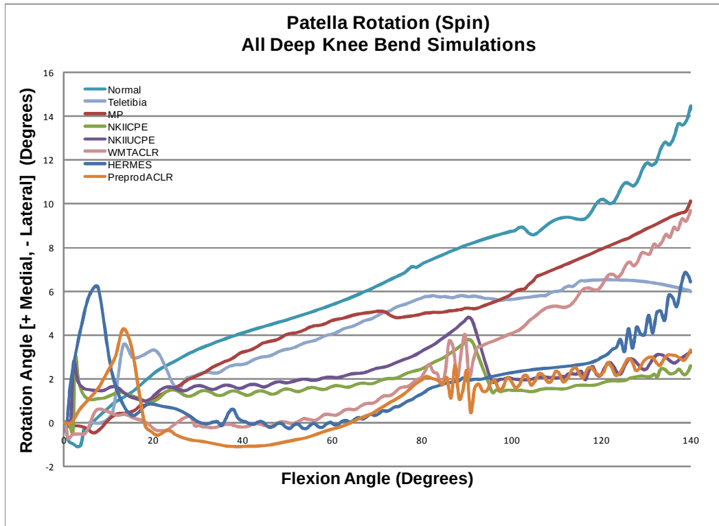
Figure 90: Patella rotation or spin (rotation about PAT1> axis) for the normal knee simulation and all TKA simulations.
