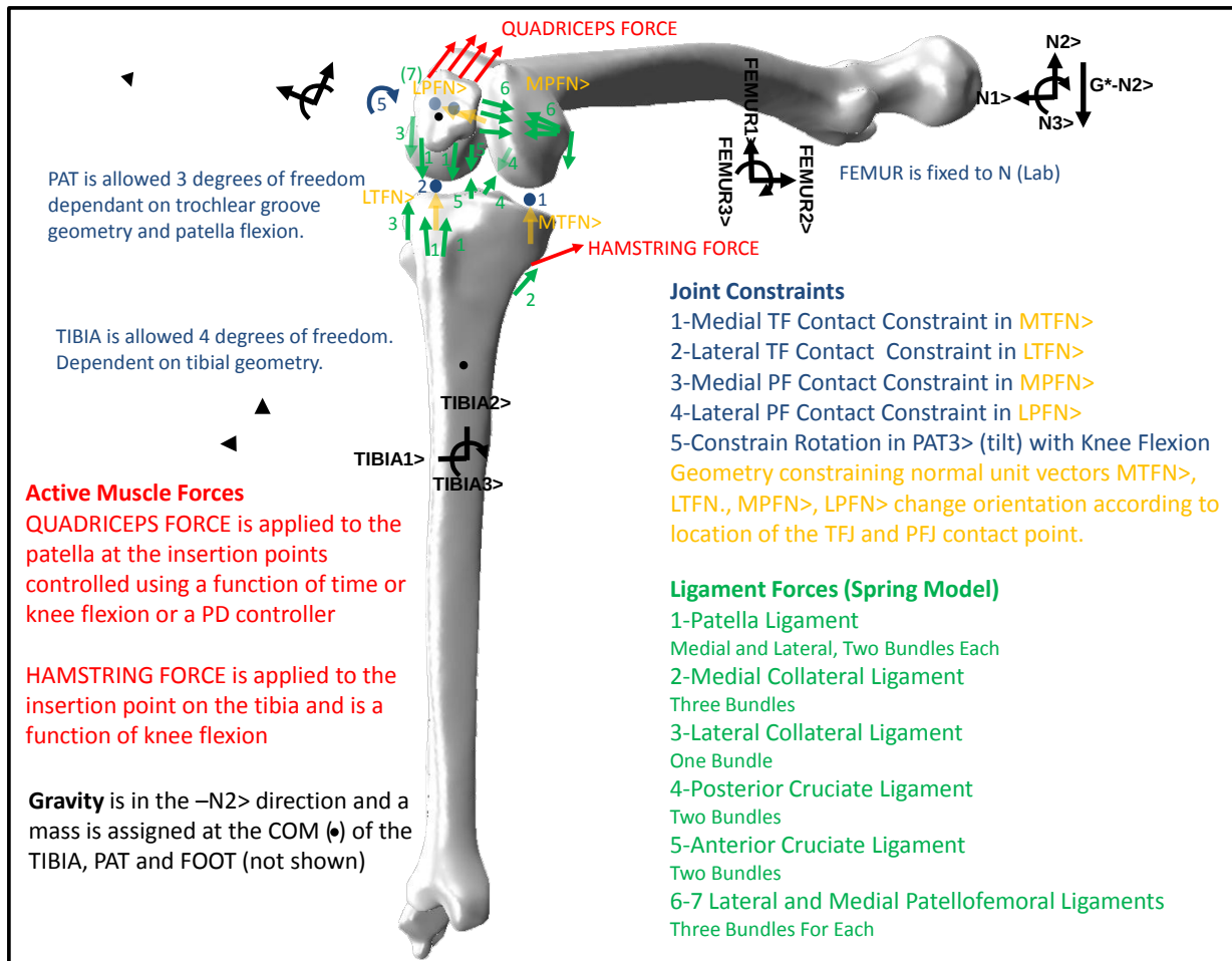
Figure 119: Free body diagram of extension model with articulating geometry. The TFJ and PFJ contact constraints were constrained using normals from the tibial or polyethylene insert and trochlear groove geometry.
