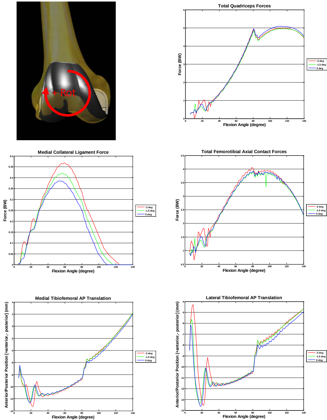
Figure 110: Sensitivity analysis of the coronal alignment of the femoral component.
