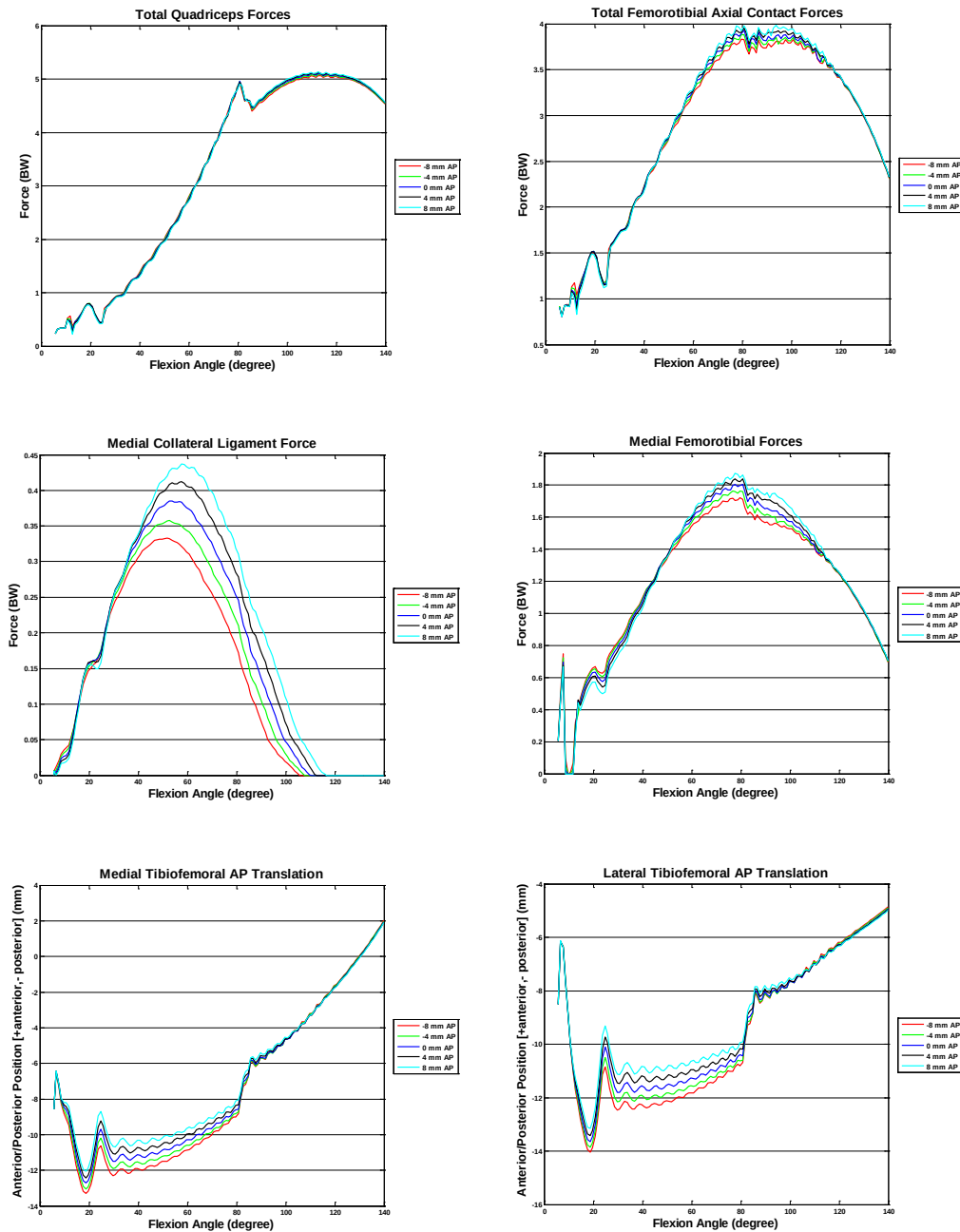
Figure 124: Sensitivity analysis of the attachment point of the MCL on the tibia. All three bundle attachments were moved in the anterior/posterior direction relative to the original position.
