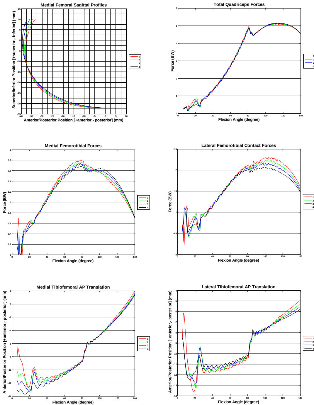
Figure 106: Sensitivity analysis of the medial sagittal femoral curvature. The curvatures simulated are shown in the upper left with data set 1 being the actual curvature of the Teletibia TKA.
