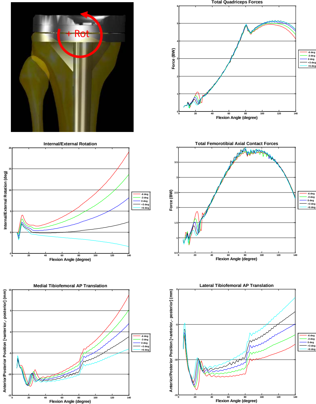
Figure 108: Sensitivity analysis of the rotation of the tibial component in the coronal plane (image in upper left describes rotational direction). The data sets are described by the rotation from the original orientation used for the validation. Internal/External rotation (middle plot on the left) in this case is calculated as the angle between the line connecting the contact points and the mediolateral line of the tibial component.
