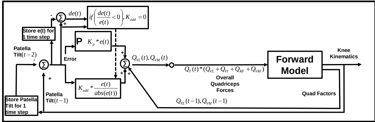
Figure 17: Diagram of the controller for patella stabilization. e(t) in this diagram is e_{PAT_2}(t) and Patella Tilt is \theta_{PAT_2} , discussed in the text. This is implemented in line with the flexion controller (Figure 16).
