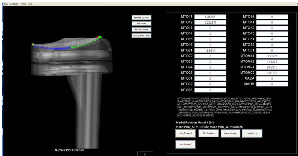
Figure 11: View of software developed to edit the multivariate polynomial and view the estimated geometry compared to actual geometry of the implant. The implant in this figure is the Teletibia TKA. The estimated geometry for the lateral insert is shown with the colored dots. Notice that the estimated sagittal curvature matches well with the actual curvature of the implant.
