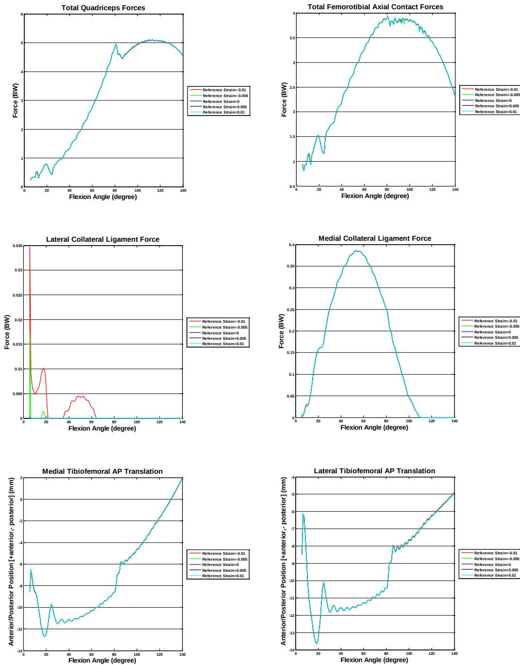
Figure 123: Sensitivity analysis of the lateral collateral ligament reference strain which adjusts the LCL slack length, calculated by multiplying the length of the ligament at full extension with the reference strain.
