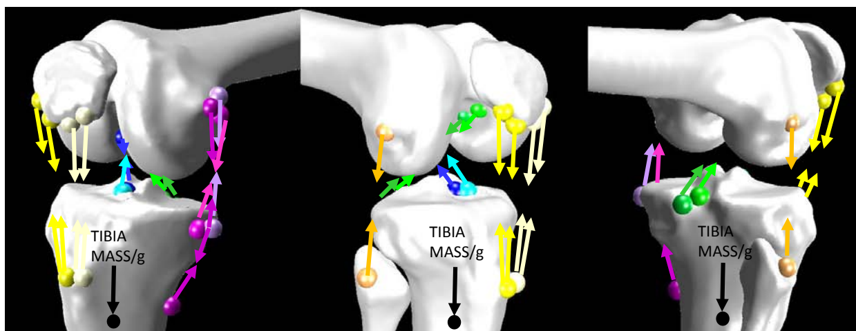
Figure 21: Close up view of the force vectors acting on the tibia from the various bundles of the ligaments of the knee and extensor mechanism. Each arrow represents two force vectors used in the calculation of ligament preloads. The goal is to find the force value for each ligament group which counter acts the mass of TIBIA and the FOOT (not shown). The spheres in this picture represent the actual attachment points used.
