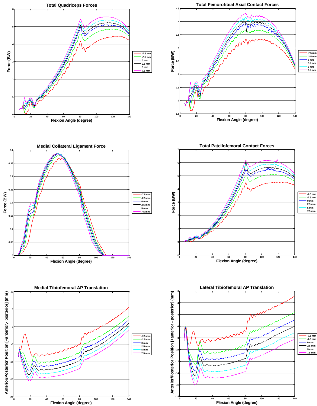
Figure 130: Sensitivity analysis of the tibial component location relative to the tibia in the Anterior/Posterior direction (+anterior,-posterior). The femur and femoral component and patella locations were adjusted so that the relative starting position to the tibial component was the same at each new location.
