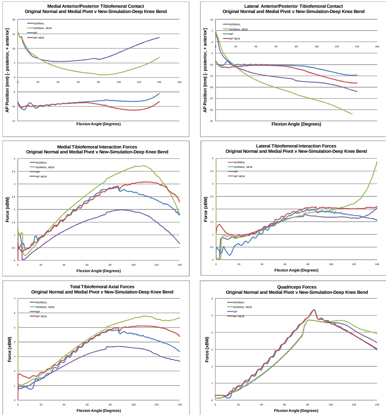
Figure 97: Tibiofemoral kinematics, kinetics and quadriceps force comparison for the original normal knee and Medial Pivot TKA implanted knee deep knee bend simulation and simulations with tightened ligaments.
