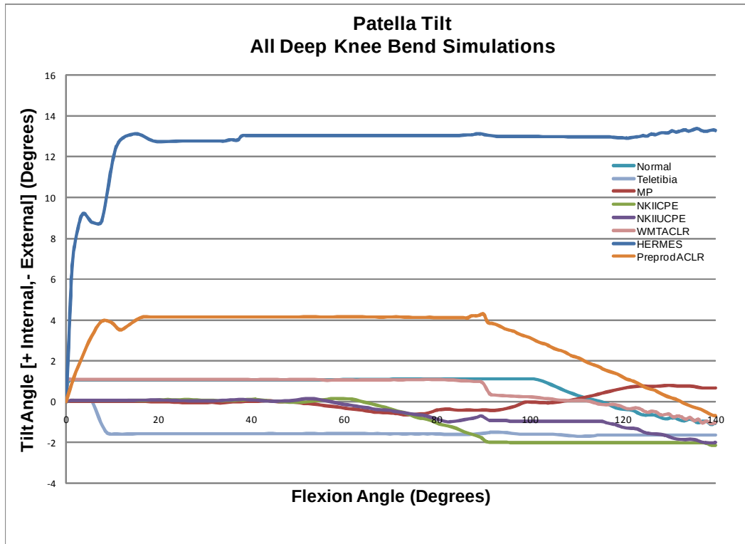
Figure 89: Patella tilt (rotation about PAT2> axis) controlled by a controller which adjusts the Vastus Medialis and Vastus Lateralis to stabilize the patella for the normal knee simulation and all TKA simulations.
