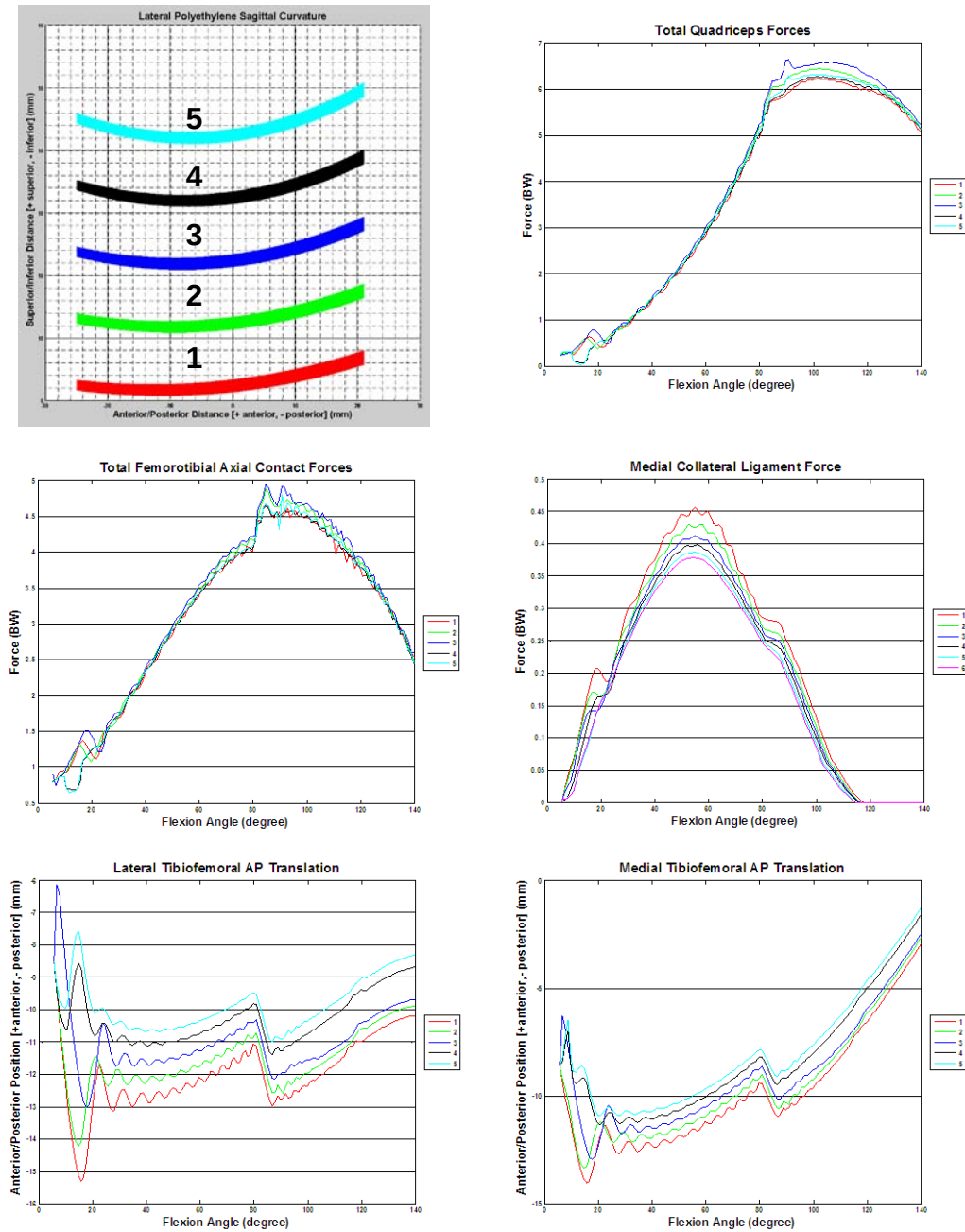
Figure 103: Sensitivity analysis of the lateral tibial tray curvature. The average curvatures simulated are shown in the upper left with data set 4 being the actual curvature of the Teletibia TKA. The “well point” changed moving more anterior in the more conforming design (5) and more posterior in the less constrained curvature (1-3).
