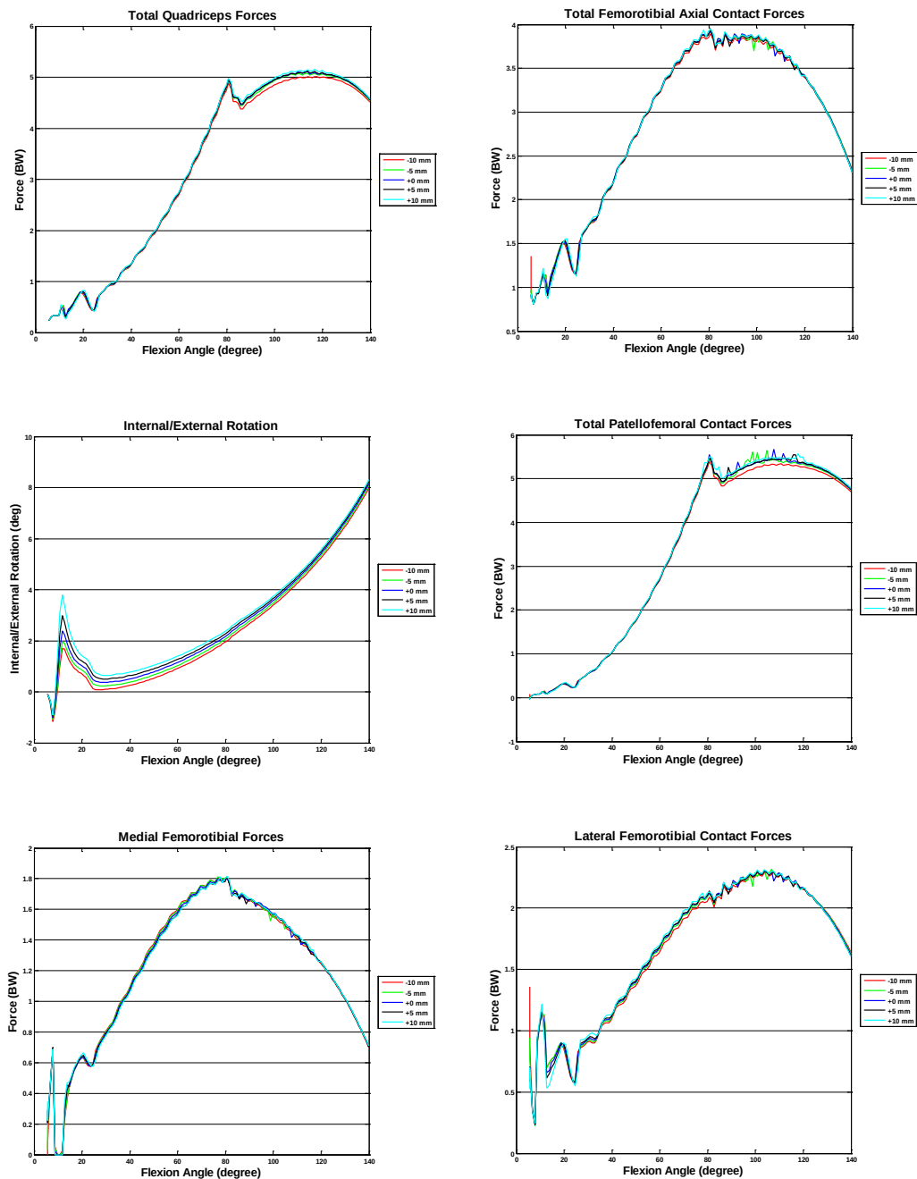
Figure 135: Sensitivity analysis of moving the attachment of the patella ligament on the tibia in the medial or lateral direction from the chosen position on the CAD models built by CT scans. For these simulations no adjustment of the slack length from simulation to simulation was made.
