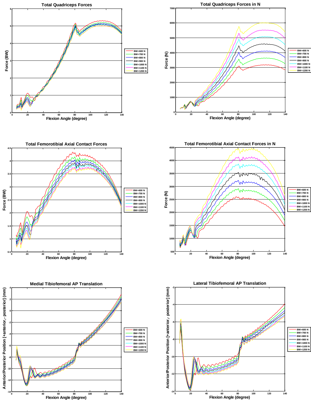
Figure 107: Sensitivity analysis of the total body weight parameter. The original body weight is 900 N. The quadriceps and total axial forces are in the top two rows in units of BW on the left and N on the right.
