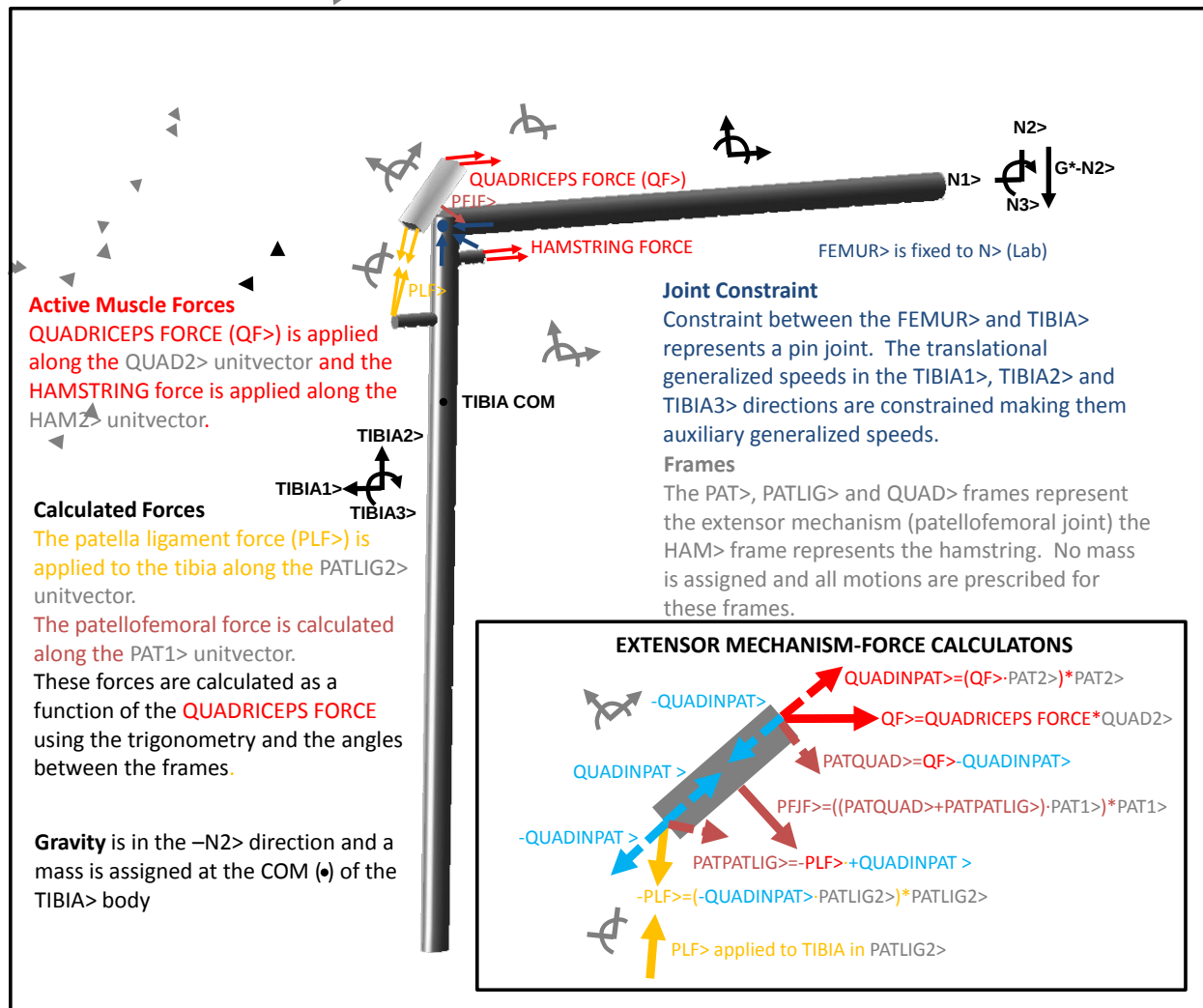
Figure 113: Description of a simple extension model with an idealized pin joint representing the TFJ and frames with specified motions representing the extensor mechanism. The inlay shows the calculations for the patellar mechanism forces including the patellar ligament force and patellofemoral force which are represented using massless frames. This model includes one body (TIBIA) free to rotate in all three directions with one tibiofemoral contact point with the femur fixed to the Newtonian reference frame. Active quadriceps and hamstring forces are applied along unitvectors in their respective reference frames.
