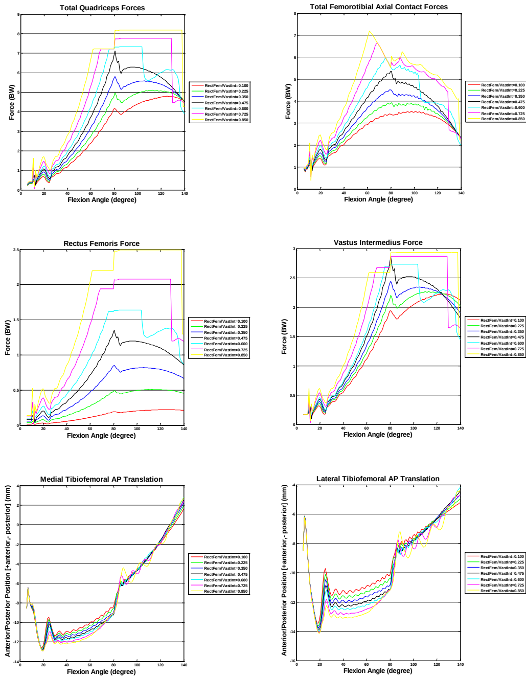
Figure 98: Sensitivity analysis results from increasing the Rectus Femoris / Vastus Intermedius force ratio. The model used for validation had a ratio of 0.225.
