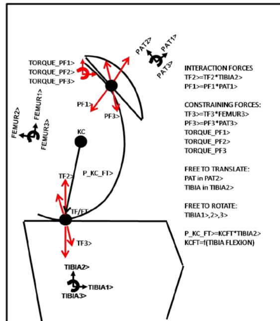
Figure 114: Schematic of the contact points and constraining forces for an initial model of extension. The patella is a body as is the tibia. The femorotibial and patellofemoral contact points are prescribed on the femur as a function of tibial flexion. Interaction forces keep the patella and tibia from penetrating the femur, constraining forces constrain the motion of the bodies. Ligaments and muscles are not shown.
