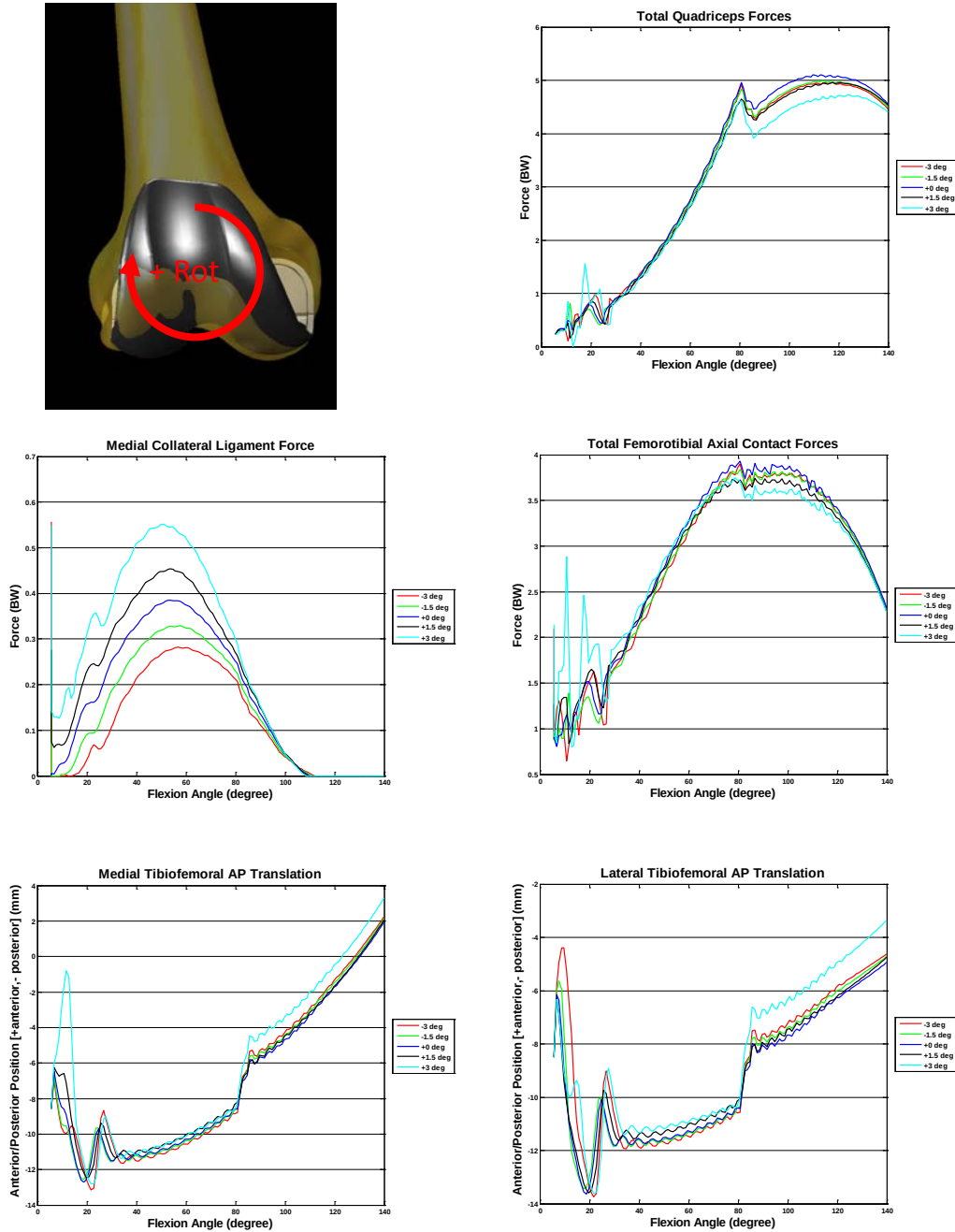
Figure 129: Sensitivity analysis of the femoral component orientation in the coronal plane (see figure in upper left for rotation direction). Adjustments were made from the original orientation (0 deg). Unlike the results Figure 110 the ligament slack lengths were kept the same for each orientation of the components.
