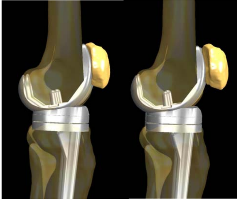
Figure 101: Although the “patellar button” is not visible in the above images the thickness is changed by keeping the patellofemoral contact points on the trochlear groove and moving the patella anterior from the femur. On the left is the thinnest patellar button analyzed, 9mm, and on the right the thickest, 19 mm.
