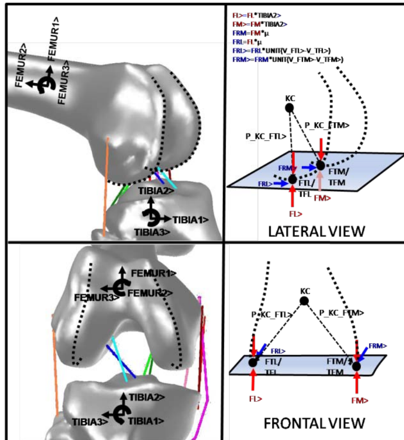
Figure 116: Diagram showing how tibiofemoral contact is modeled in early models. The geometry of the medial and lateral femur is expressed as a point on the medial (FTM) and lateral (FTL) condyle. FTM and FTL change position in the femoral reference frame as a function of flexion. TFL and TFM are the tibial contact points. The distance between TFL and FTL and TFM and FTM is set to 0>. TFL and TFM can translate relative to the tibia in the TIBIA3> and TIBIA1> directions. Medial (FM>) and lateral (FL>) contact forces are in the TIBIA2> direction. FRL> and FRM> are friction forces.
