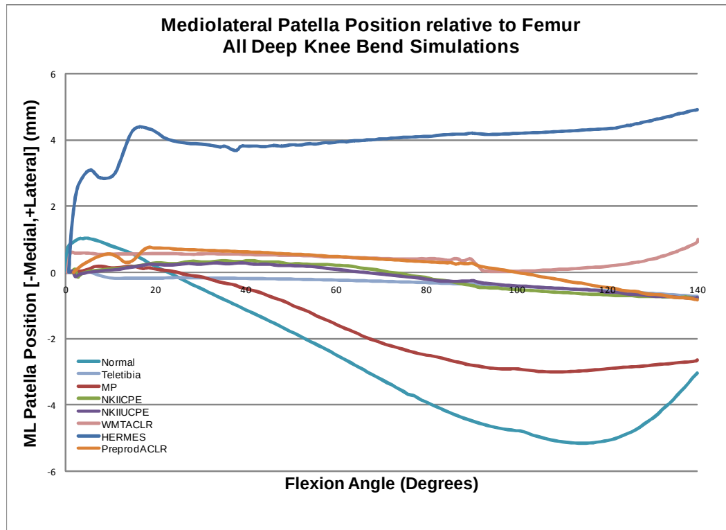
Figure 91: Mediolateral patella position relative to the femur for the normal knee simulation and all TKA simulations.
