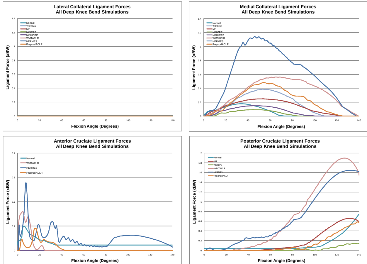
Figure 94: Ligament forces from all bundles for the LCL, MCL, ACL and PCL for the normal knee simulation and all TKA simulations.
