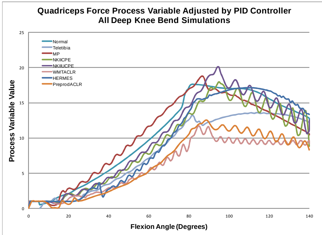
Figure 77: The quadriceps force process variable values adjusted by the PID controller for the normal knee simulation and all of the TKA design simulations.
