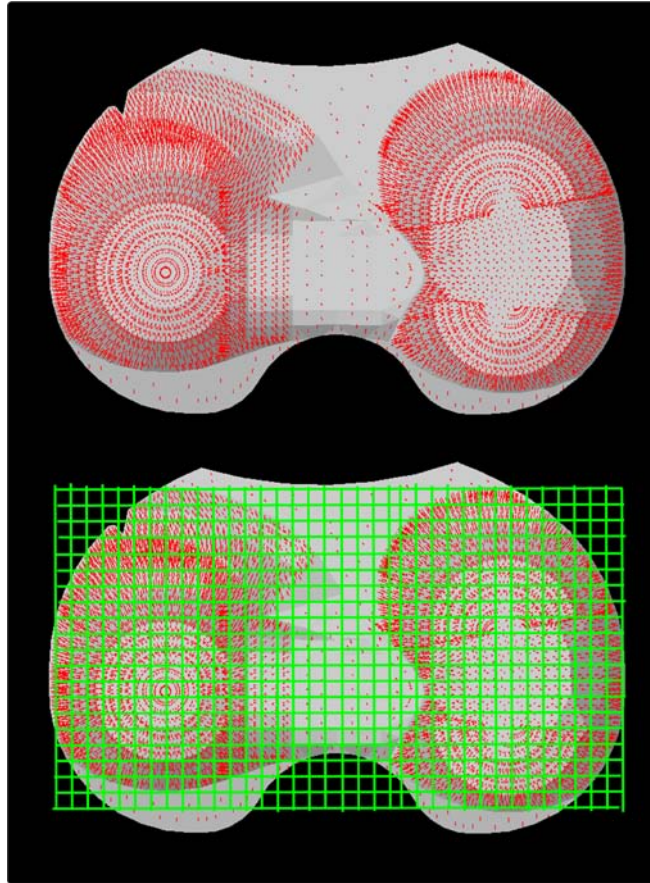
Figure 9: Normal vectors from the faces of a Medial Pivot® TKA polyethylene insert from Wright Medical Technology, Inc. These vectors can be mapped in the AP (up/down in this diagram) and ML (left/right) and a function can be fit to represent the two angles needed to find the orientation of the normal vectors.
