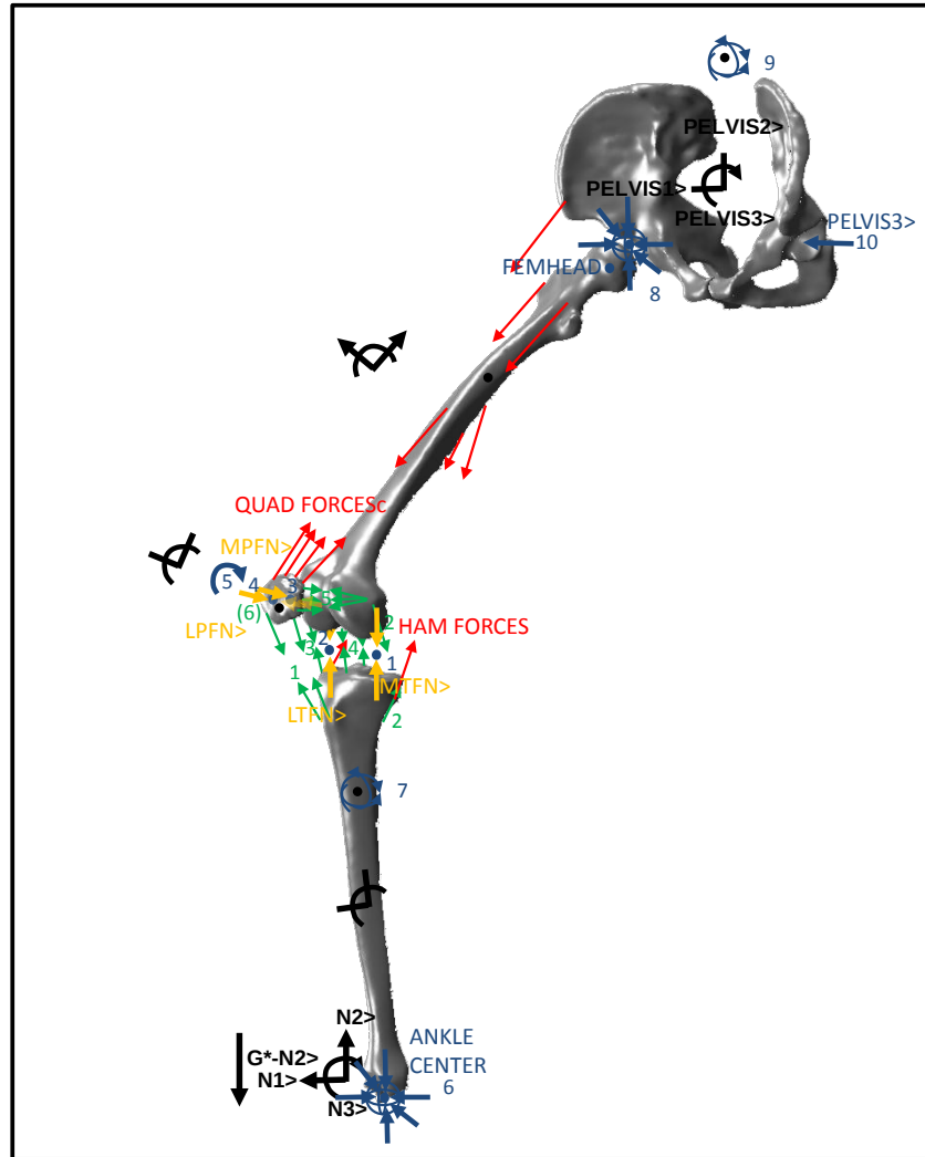
Figure 13: Free Body Diagram of the weight bearing deep knee bend model including joint constraining forces applied using geometry, ligament forces, active muscle forces, ground reaction forces, hip forces, opposite leg force in medial/lateral direction. This model includes four bodies, TIBIA, PAT, FEMUR and PELVIS (TRUNK). The TIBIA body is constrained in all three rotations and translations at the ANKLE CENTER in N. The FEMUR has three degrees of freedom although it can move in all 6 degrees of freedom. The translational speeds are constrained at the medial and lateral contact point and at the FEMORAL HEAD in the PELVIS3> direction. The PAT body representing the patella has two contact points with the FEMUR and three DOF. The ligaments forces are modeled as spring-damper systems with two spring elements per bundle. The QUAD and HAM forces are inputs to the model and are applied at attachment points on the patella and tibia, with origins on the FEMUR and PELVIS. Each force vector in this diagram represents four distributed force vectors applied to the respective bodies. The QUAD FORCES are controlled with a controller, which stabilizes the patella, embedded with a modified PID controller, which controls flexion, with an additional flexion acceleration feedback.
