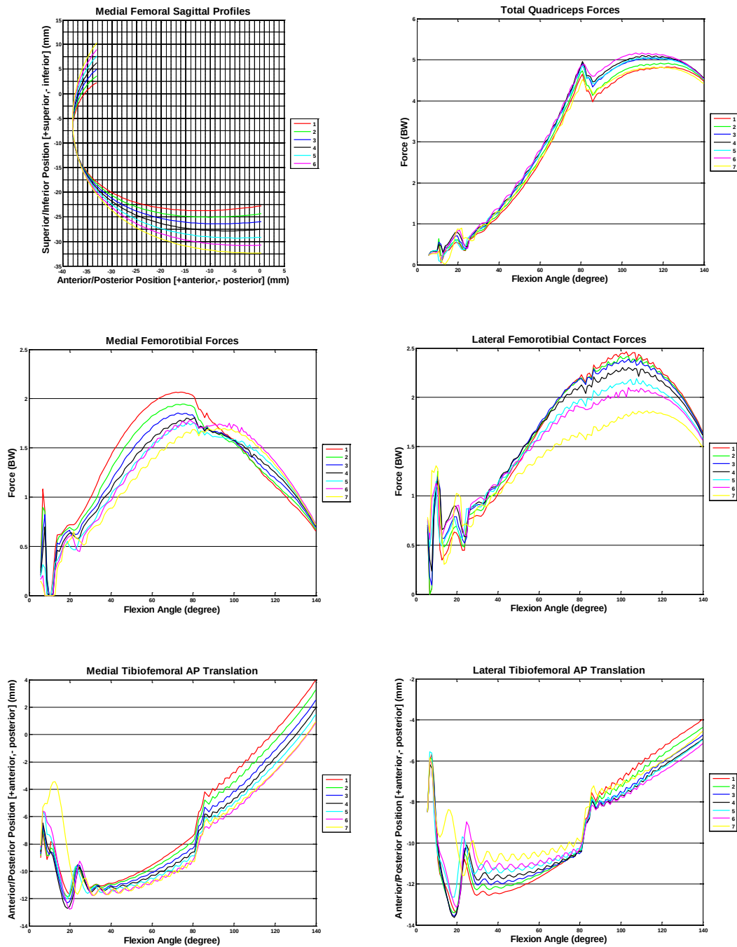
Figure 131: A second sensitivity analysis of the medial femoral sagittal profile. The sagittal profile is seen in upper left figure. The original profile of the Tibiofemoral TKA is data set 4.
