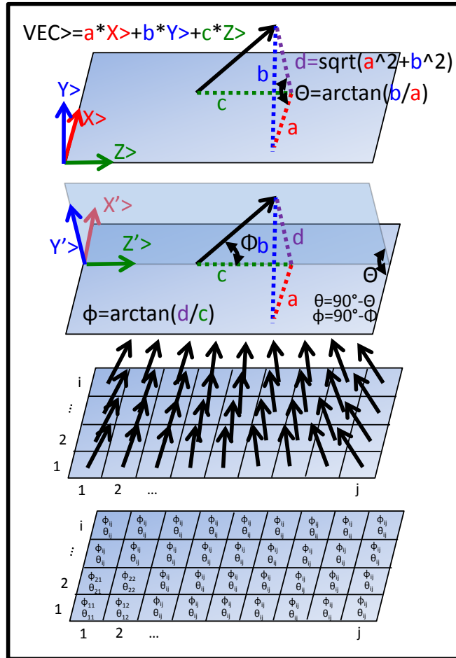
Figure 6: Demonstrating how a vector can be described using two sequential rotations, one about X and one about Y' . Multiple vectors can be expressed over a grid to represent the normal vectors from geometry. Rotations can be expressed as polynomials or spline functions.
