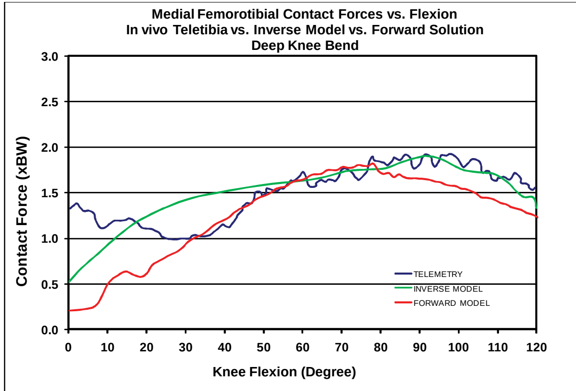
Figure 52: Comparison of the medial contact force on the tibia from in vivo data from a subject implanted with an instrumented TKA performing a deep knee bend, a validated inverse model using the in vivo motions from that subject and a forward simulation of the same activity with the same TKA geometry.
