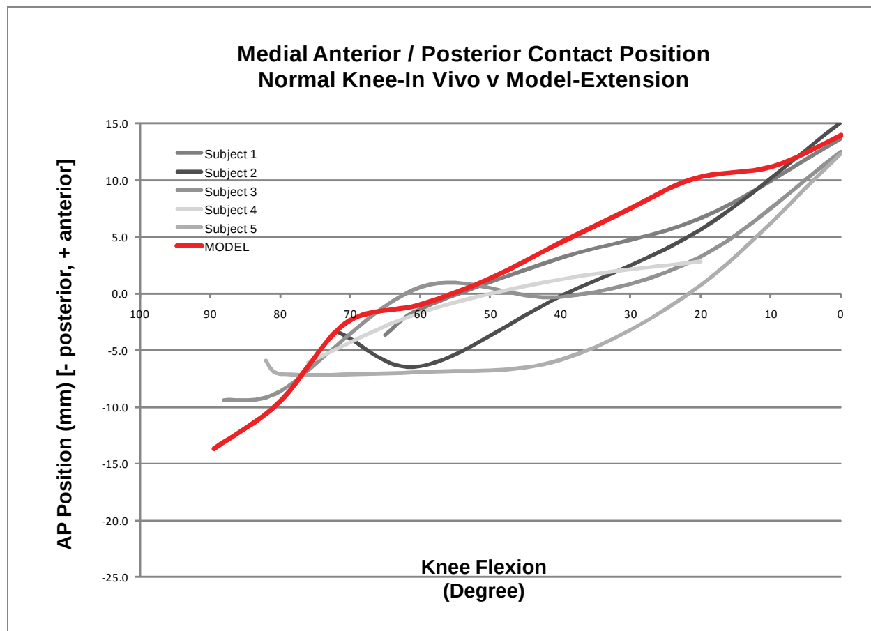
Figure 44: Medial anterior/posterior femorotibial contact position data from fluoroscopy and forward model simulation for a non-weight bearing extension activity. Geometry and soft tissue attachments were determined using models constructed from CT scans from Subject 3.
