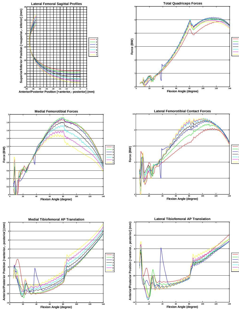
Figure 132: A second sensitivity analysis of the lateral femoral sagittal profile. The sagittal profile is seen in upper left figure. The original profile of the Tibiofemoral TKA is data set 4.
