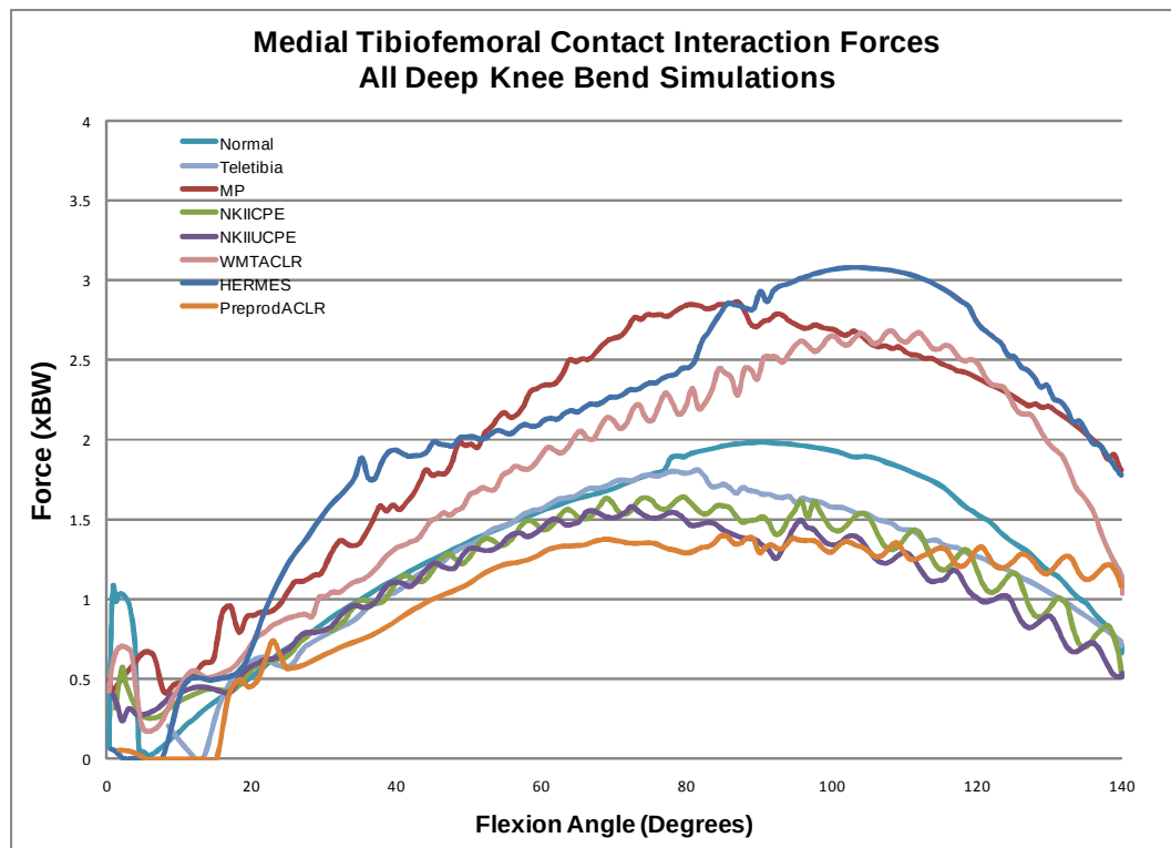
Figure 86: Medial tibiofemoral contact forces for the normal knee simulation and all TKA simulations.
