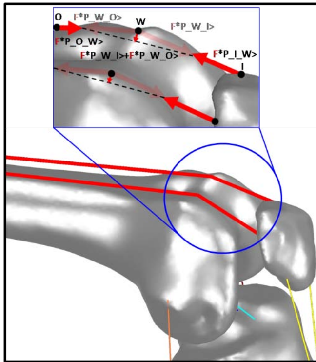
Figure 15: Close-up of the calculation of forces occurring at a wrapping point. Points O, W and I are the origin of the quad muscle, wrapping point and insertion, respectively. F is the quad muscle force and P_{I_W} and other vectors are unit vectors pointing from the first point in the name to the second. This same concept is also applied to wrapping ligaments such as the MCL.
