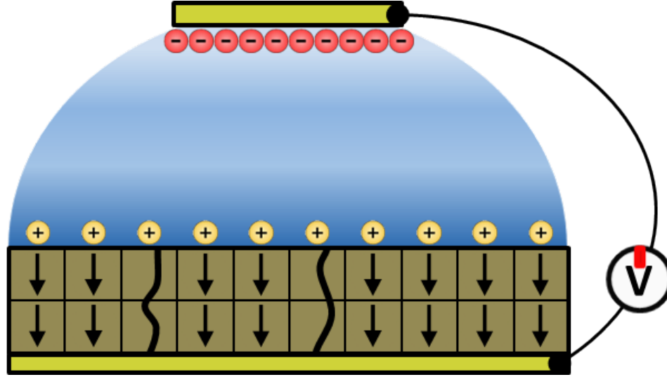
Figure 3.1: Schematic of an ionic liquid device as applied to a ferroelectric film. In this schematic a positive bias is applied, causing the negative ions to accumulate at the gate electrode, and the positive ions to accumulate at the interface of the film. These positive ions remain at the surface, despite the leakage shorts shown by the vertical curved lines. The positive ions induce a down orientation or one where the surface potential is negative.
