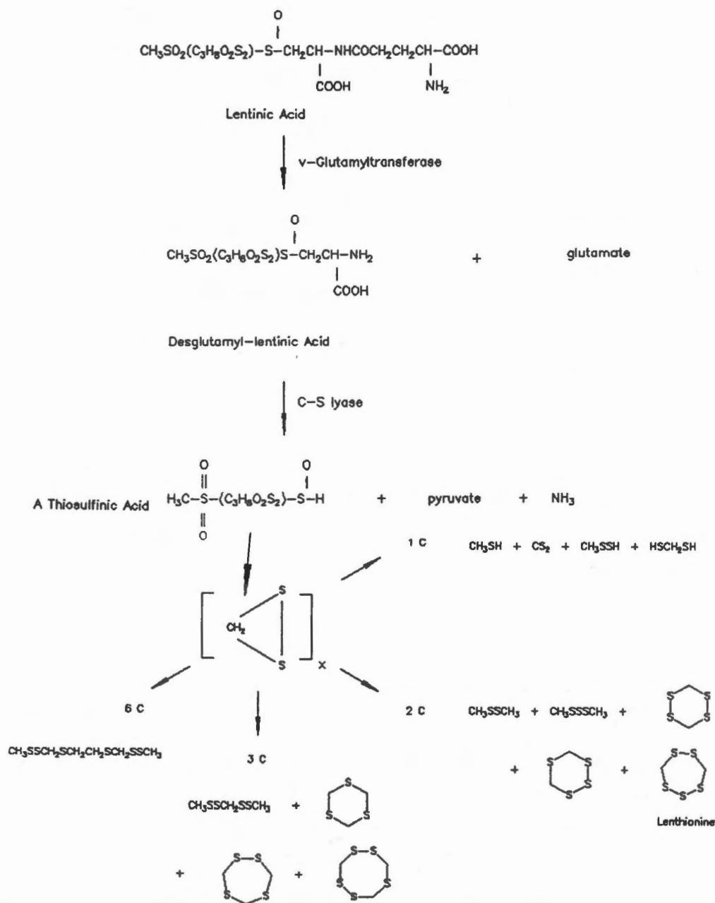
Fig. 3-Formation of sulfur volatiles in Shiitake mushrooms.
