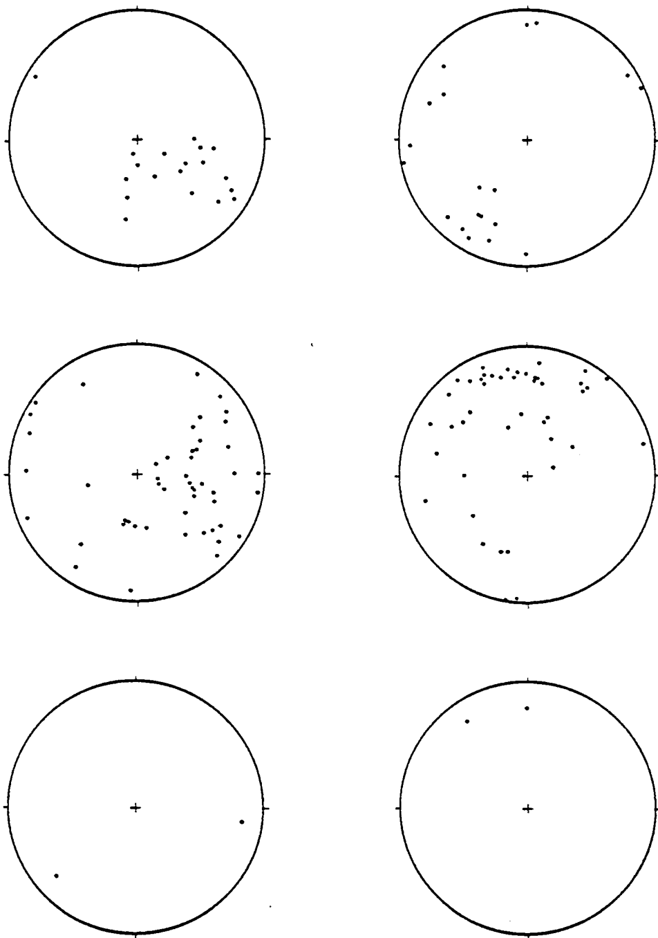
Figure 42: Domain I: Equal area plots of poles to axial surfaces (left column) and fold axes (right column) of mesoscopic folds. a. = Type 1 folds. b = Type 2 folds. c = Type 3 folds.
