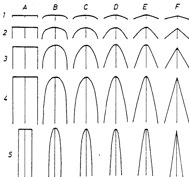
Figure 26: Fold classification scheme based on shape (A-F) and amplification (1-5) (from Ramsay and Huber, 1987; after Hudleston, 1973.)
