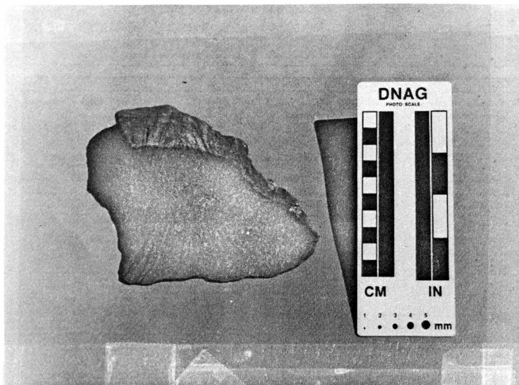
(a) Type 2 fold from Coleman River Formation, Wildcat Creek Road (Tray Mountain quadrangle).
