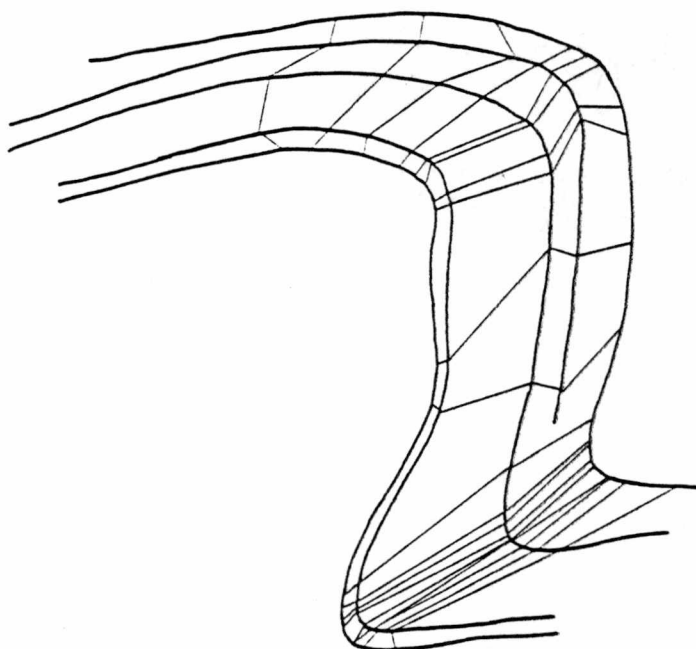
(b) Dip isogon analysis of same fold.
