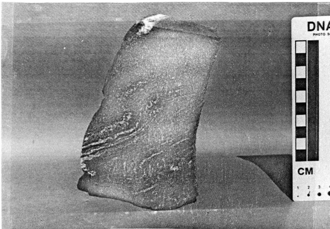
(a) Ptygmatic folds in hand sample of Coleman River metasandstone.
