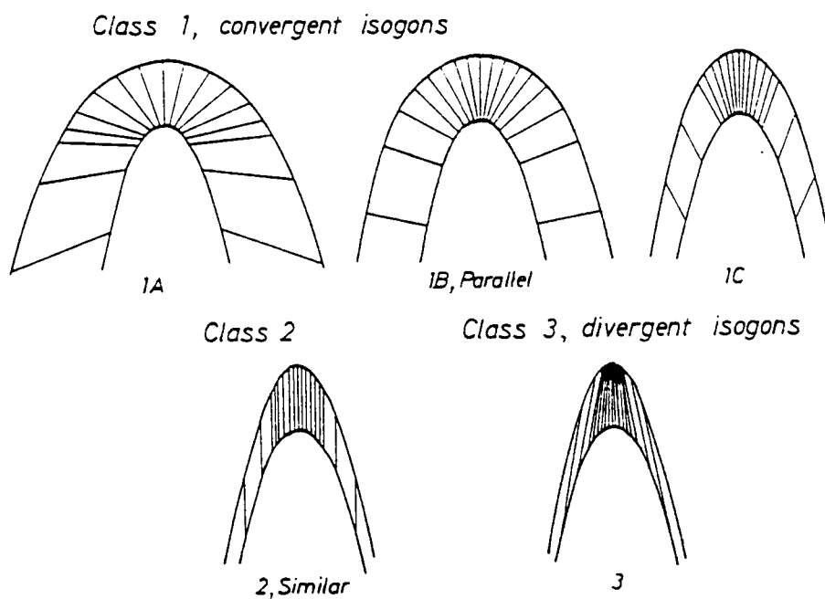
Figure 27: Dip isogon characteristics of main fold classes (after Ramsay, 1967).
