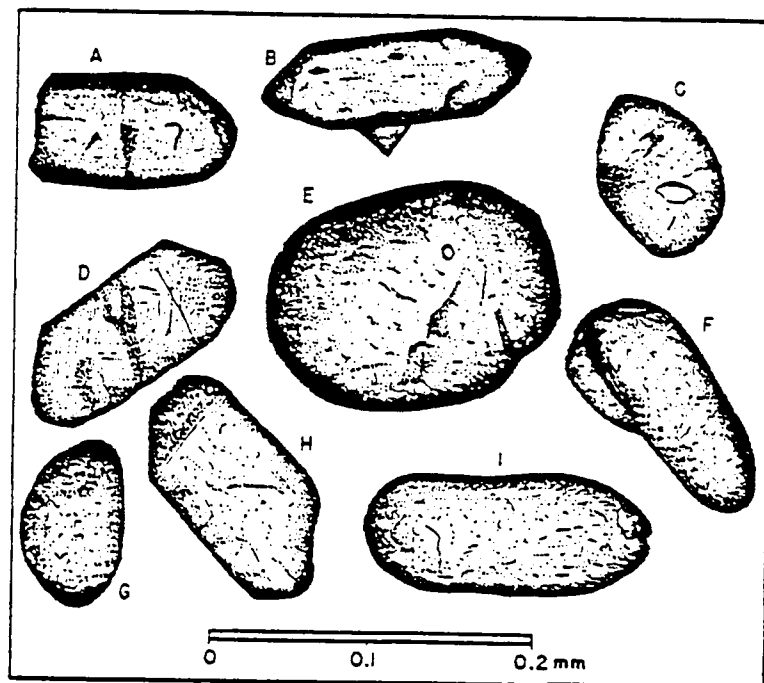
Figure 11: Typical habits of zircons in sandstones (from Poldervaart, 1955).
