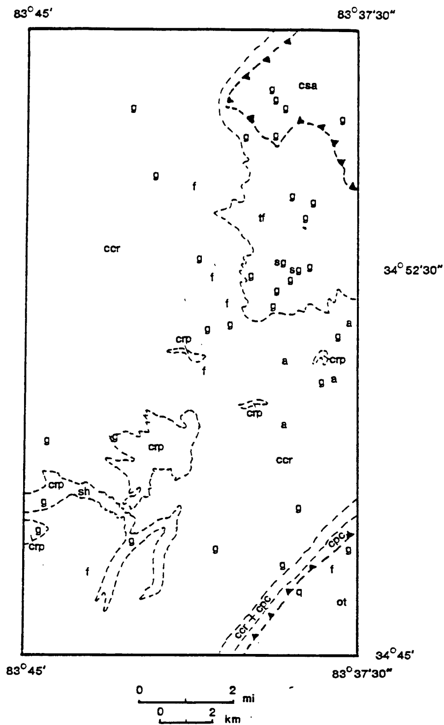
Figure 8: Distribution of sandstone types within the study area. g = greywacke; sg = subgreywacke; a = arkose; f = feldspathic sandstone; q = quartzose sandstone; sh = shale. Rocks units as in Plate II.
