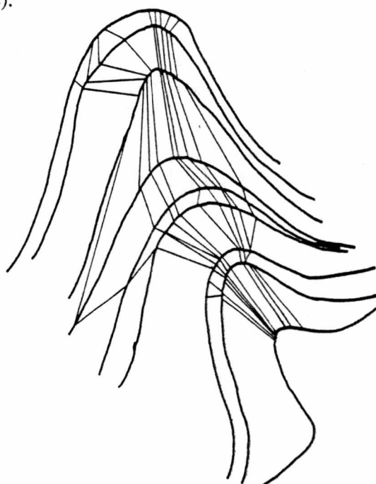
(b) Dip isogon analysis of same fold.
