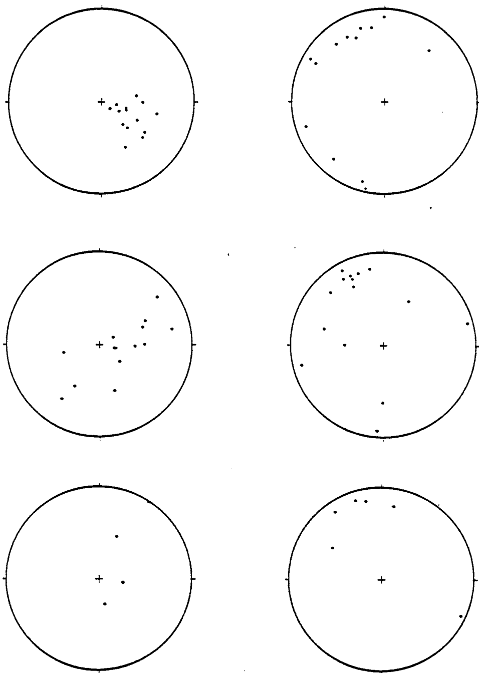
Figure 43: Domain II: Equal area plots of poles to axial surfaces (left column) and fold axes (right column) of mesoscopic folds. a. = Type 1 folds. b = Type 2 folds. c = Type 3 folds.
