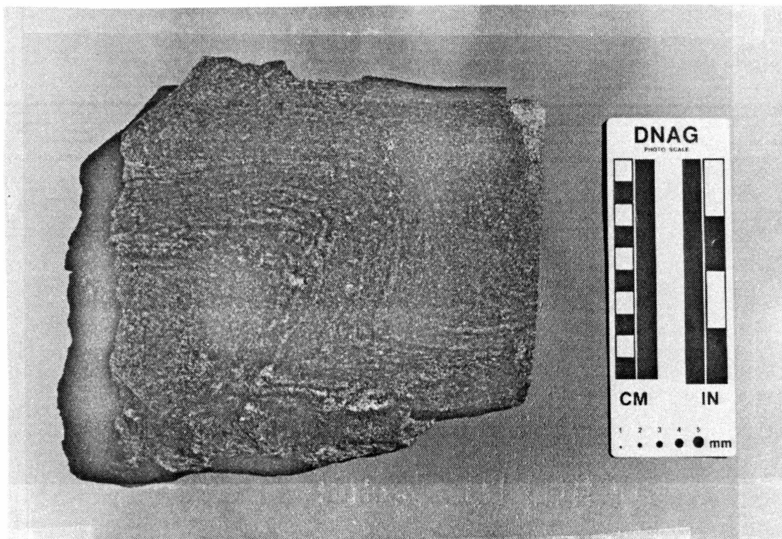
(a) Type 2 fold from Coleman River Formation, Tray Mountain.
