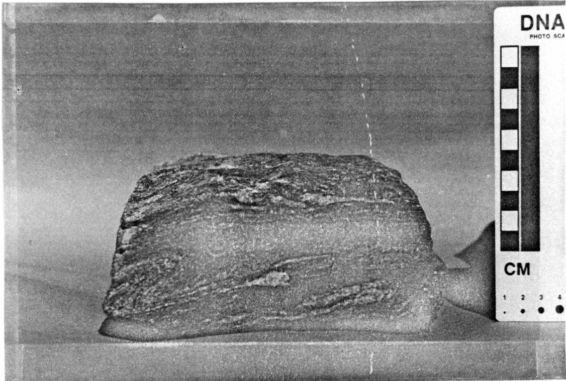
(a) Type 1 fold from Otto Formation, Wildcat Creek Road (just east of study area).
