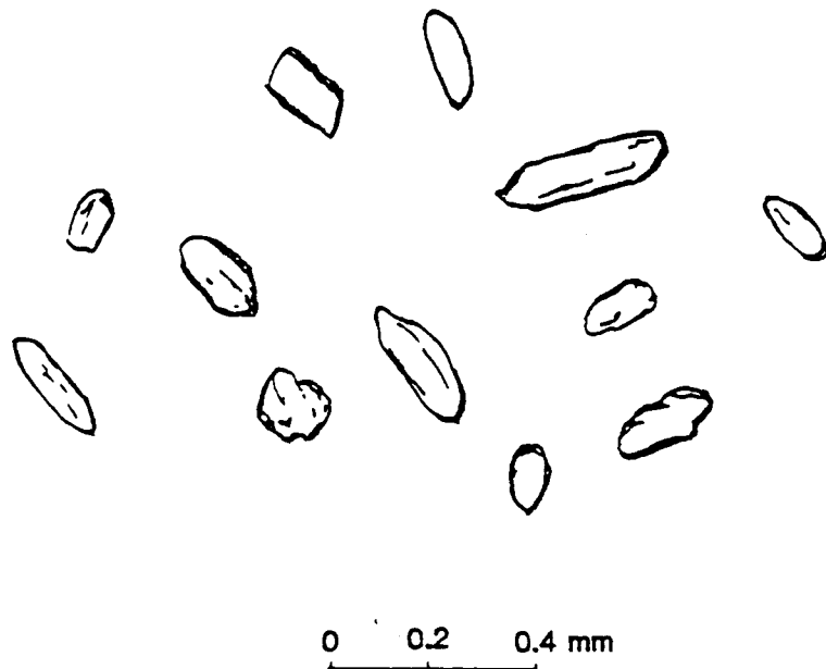
Figure 10: Typical habits of zircons from metasandstone of the Coleman River and Tallulah Falls Formations (this study).
