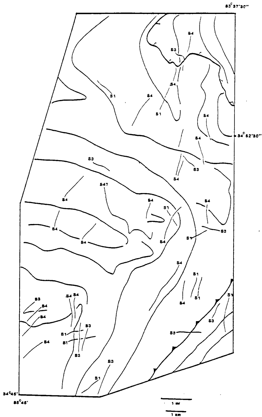
Figure 19: Orientation and observed distribution of foliations in the study area. Heavy, unlabeled lines represent the general form lines of the dominant foliation, S_2 . Lighter, labeled lines represent subordinate foliations. Heavy line with solid teeth = Soque River fault. Heavy line with open teeth = Shope Fork fault.
