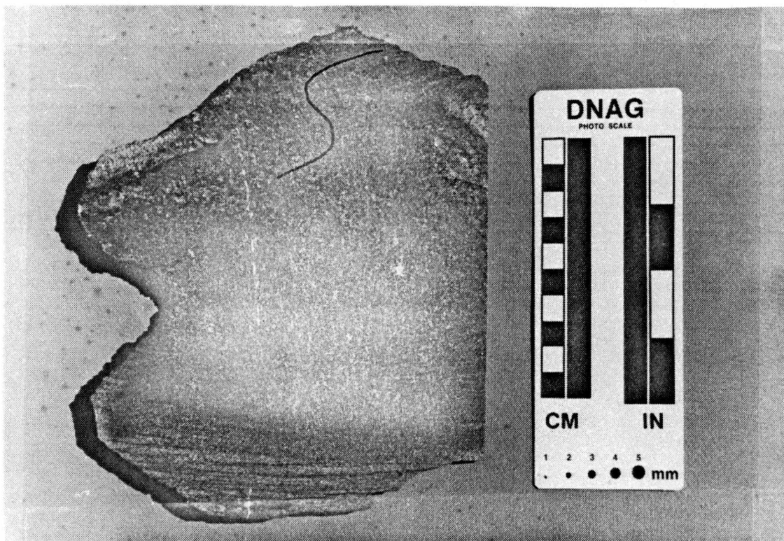
(a) Type 1 fold from Tallulah Falls Formation, Dismal Gap (Macedonia quadrangle).
