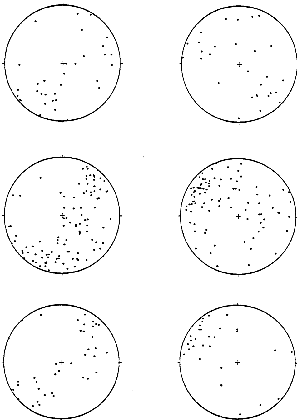
Figure 45: Domain IV: Equal area plots of poles to axial surfaces (left column) and fold axes (right column) of mesoscopic folds. a. = Type 1 folds. b = Type 2 folds. c = Type 3 folds.
