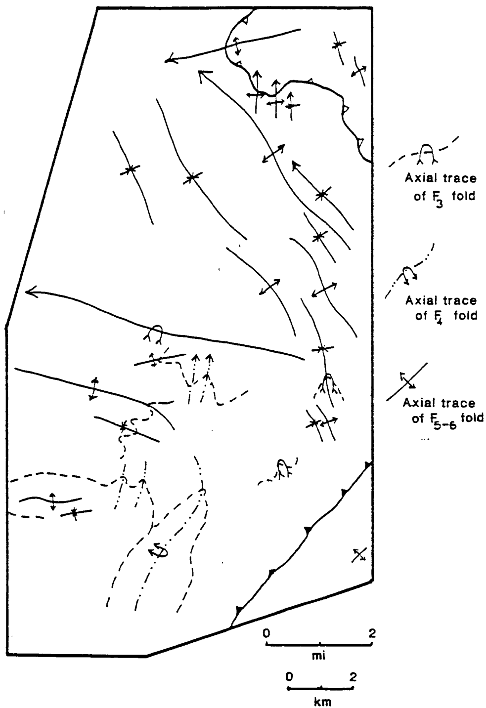
Figure 40: Distribution of map-scale folds within the study area. Heavy line with solid teeth = Soque River fault. Heavy line with open teeth = Shope Fork fault.
