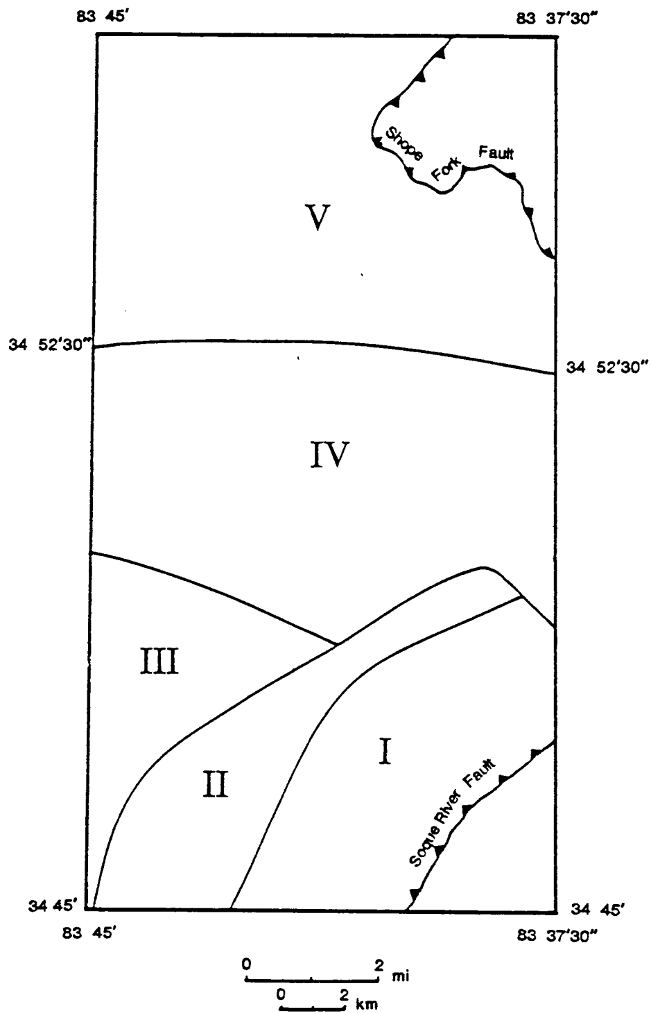
Figure 41: Map of domain boundaries for domain analysis of study area.
